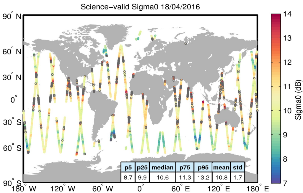
Figure 27. Geographical distribution of science-valid sigma0 data over oceans and lakes for 18/04/2016. The statistical values shown in the table refer to the sigma0 in dB and are calculated over all measurements shown in the figure. Gray circles denote records that have been rejected based on the editing criteria described in Table 4.
