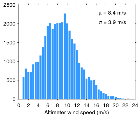
Figure 35. Histogram of science-valid wind over oceans and lakes for 18/04/2016. The mean ( \mu ) and standard deviation ( \sigma ) are also shown. Note that values larger than 24 m/s are excluded from the histogram for the sake of readability but not from the computation of \mu and \sigma .
