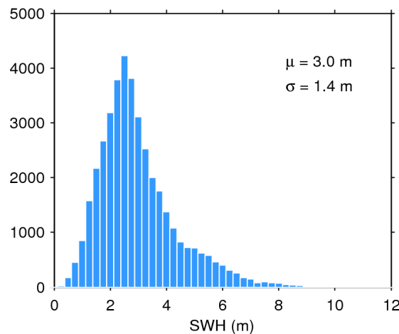
Figure 17. Histogram of flag-valid SWH over oceans and lakes for 18/04/2016. The mean ( \mu ) and standard deviation ( \sigma ) are also shown. Note that values larger than 12 m are excluded from the histogram for the sake of readability but not from the computation of \mu and \sigma .
