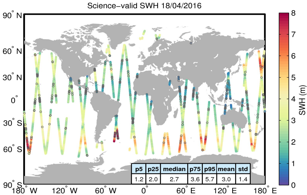
Figure 19. Geographical distribution of science-valid SWH data over oceans and lakes for 18/04/2016. The statistical values shown in the table refer to the SWH in m and are calculated over all measurements shown in the figure. Gray circles denote records that have been rejected based on the editing criteria described in Table 3.
