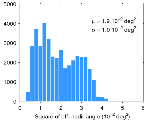
Figure 39. Histogram of flag-valid mispointing over oceans and lakes for 18/04/2016. The mean ( \mu ) and standard deviation ( \sigma ) are also shown. Note that values larger than 6 \cdot 10^{-2} \text{ deg}^2 are excluded from the histogram for the sake of readability but not from the computation of \mu and \sigma .
