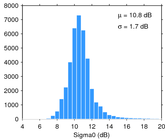
Figure 28. Histogram of science-valid sigma0 over oceans and lakes for 18/04/2016. The mean ( \mu ) and standard deviation ( \sigma ) are also shown. Note that values outside [4 20] dB are excluded from the histogram for the sake of readability but not from the computation of \mu and \sigma .
