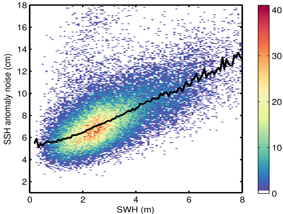
Figure 9. 2D histogram showing flag-valid SSH anomaly noise as a function of SWH for 18/04/2016. The black line denotes the median SSH anomaly noise as a function of SWH.
