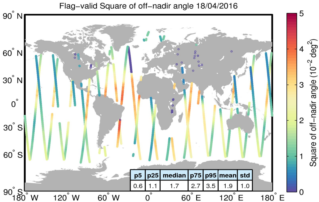
Figure 37. Geographical distribution of flag-valid mispointing data over oceans and lakes for 18/04/2016. The statistical values shown in the table refer to the mispointing in 10^{-2} \text{ deg}^2 and are calculated over all measurements shown in the figure.
