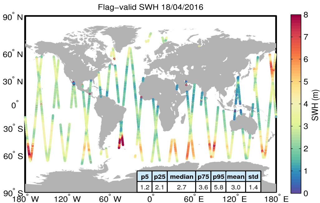
Figure 15. Geographical distribution of flag-valid SWH data over oceans and lakes for 18/04/2016. The statistical values shown in the table refer to the SWH in m and are calculated over all measurements shown in the figure.
