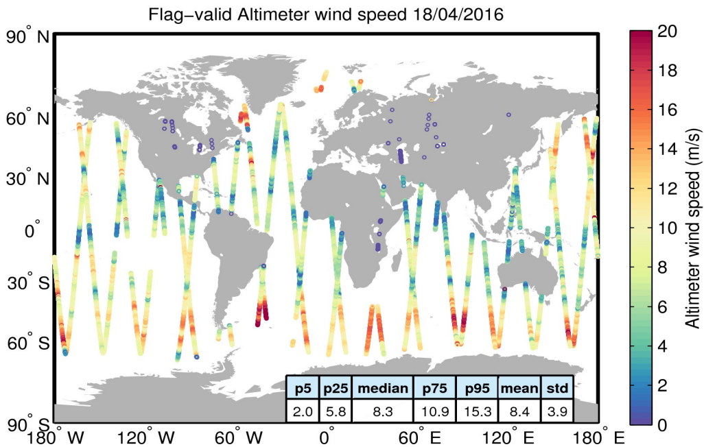
Figure 31. Geographical distribution of flag-valid wind data over oceans and lakes for 18/04/2016. The statistical values shown in the table refer to the wind in m/s and are calculated over all measurements shown in the figure.
