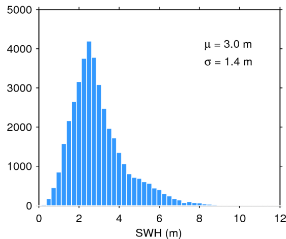
Figure 20. Histogram of science-valid SWH over oceans and lakes for 18/04/2016. The mean ( \mu ) and standard deviation ( \sigma ) are also shown. Note that values larger than 12 m are excluded from the histogram for the sake of readability but not from the computation of \mu and \sigma .
