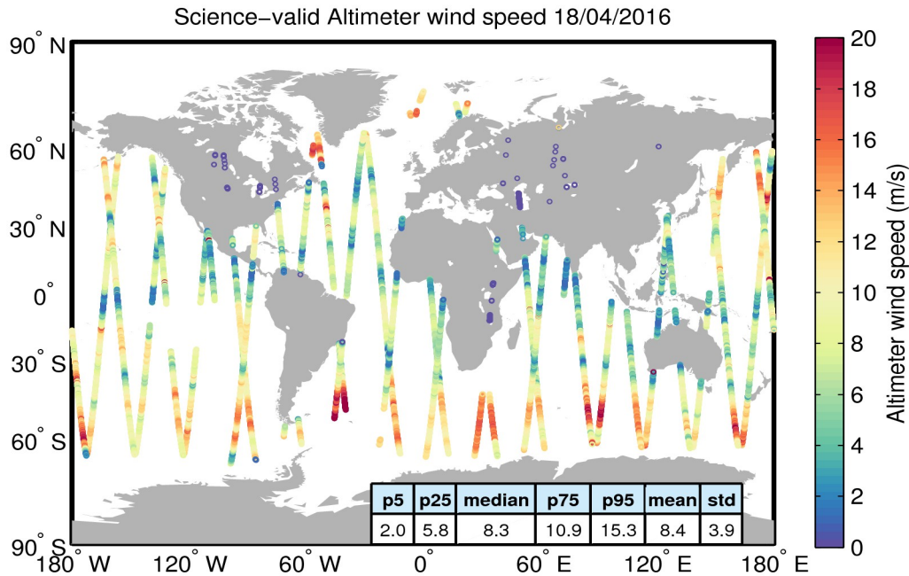
Figure 34. Geographical distribution of science-valid wind data over oceans and lakes for 18/04/2016. The statistical values shown in the table refer to the wind in m/s and are calculated over all measurements shown in the figure. Gray circles denote records that have been rejected based on the editing criteria described in Table 5.
