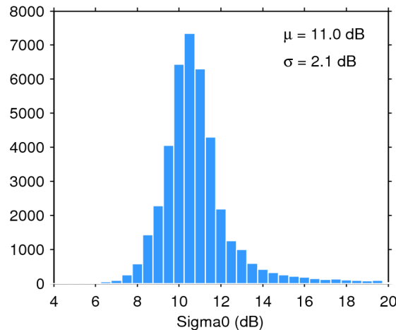
Figure 25. Histogram of flag-valid sigma0 over oceans and lakes for 18/04/2016. The mean ( \mu ) and standard deviation ( \sigma ) are also shown. Note that values outside [4 20] dB are excluded from the histogram for the sake of readability but not from the computation of \mu and \sigma .
