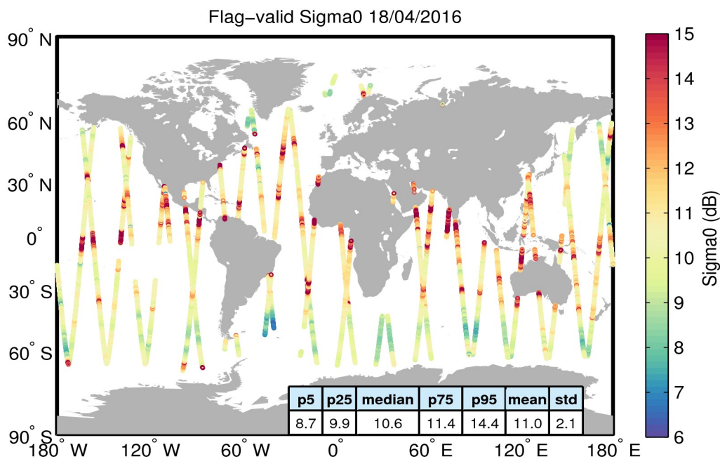
Figure 23. Geographical distribution of flag-valid sigma0 data over oceans and lakes for 18/04/2016. The statistical values shown in the table refer to the sigma0 in dB and are calculated over all measurements shown in the figure.
