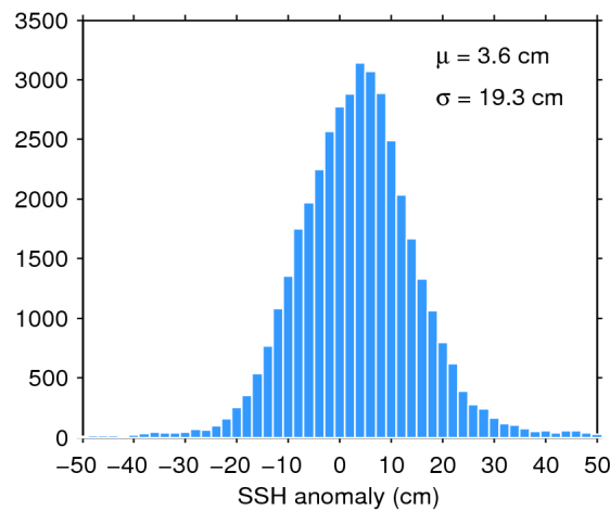
Figure 7. Histogram of flag-valid SSH anomaly over oceans and lakes for 18/04/2016. The mean ( \mu ) and standard deviation ( \sigma ) are also shown. Note that values outside [-50 50] cm are excluded from the histogram for the sake of readability but not from the computation of \mu and \sigma .
