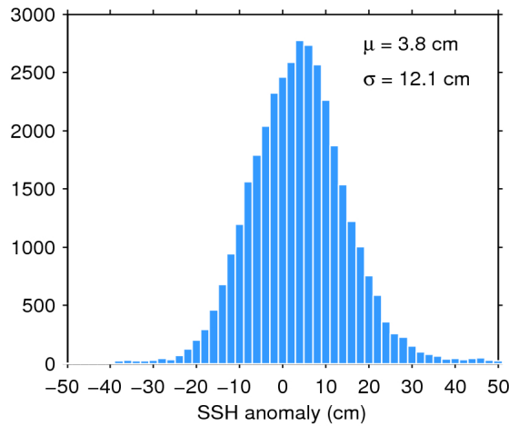
Figure 11. Histogram of science-valid SSH anomaly over oceans and lakes for 18/04/2016. The mean ( \mu ) and standard deviation ( \sigma ) are also shown. Note that values outside [-50 50] cm are excluded from the histogram for the sake of readability but not from the computation of \mu and \sigma .
