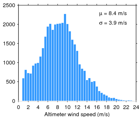
Figure 33. Histogram of flag-valid wind over oceans and lakes for 18/04/2016. The mean ( \mu ) and standard deviation ( \sigma ) are also shown. Note that values larger than 24 m/s are excluded from the histogram for the sake of readability but not from the computation of \mu and \sigma .
