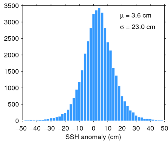
Figure 7. Histogram of flag-valid SSH anomaly over oceans and lakes for 17/04/2016. The mean ( \mu ) and standard deviation ( \sigma ) are also shown. Note that values outside [-50 50] cm are excluded from the histogram for the sake of readability but not from the computation of \mu and \sigma .
