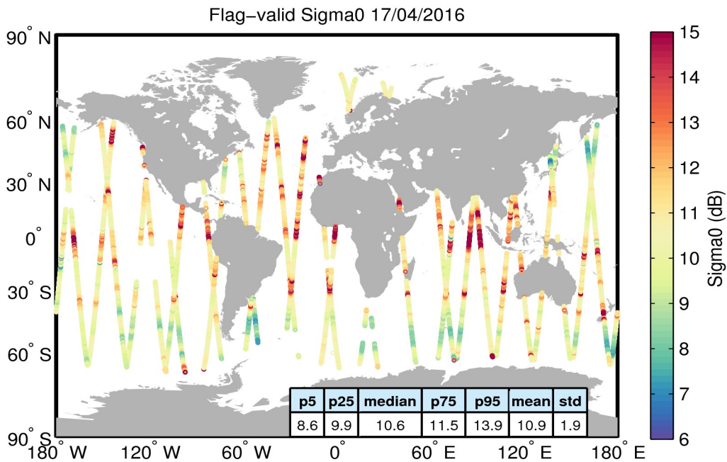
Figure 23. Geographical distribution of flag-valid sigma0 data over oceans and lakes for 17/04/2016. The statistical values shown in the table refer to the sigma0 in dB and are calculated over all measurements shown in the figure.
