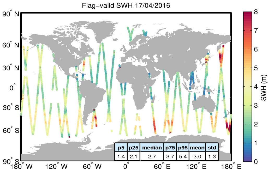
Figure 15. Geographical distribution of flag-valid SWH data over oceans and lakes for 17/04/2016. The statistical values shown in the table refer to the SWH in m and are calculated over all measurements shown in the figure.
