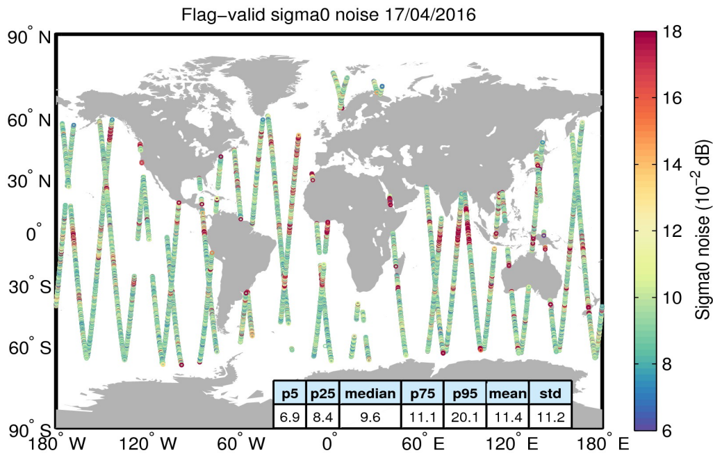
Figure 26. Geographical distribution of flag-valid 20-Hz sigma0 measurement noise over oceans and lakes for 17/04/2016. The statistical values shown in the table refer to the sigma0 noise and are calculated over all measurements shown in the figure.
