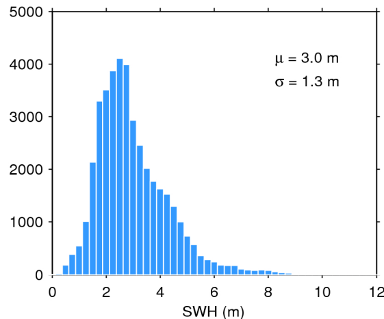
Figure 20. Histogram of science-valid SWH over oceans and lakes for 17/04/2016. The mean ( \mu ) and standard deviation ( \sigma ) are also shown. Note that values larger than 12 m are excluded from the histogram for the sake of readability but not from the computation of \mu and \sigma .
