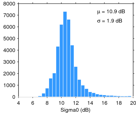
Figure 25. Histogram of flag-valid sigma0 over oceans and lakes for 17/04/2016. The mean ( \mu ) and standard deviation ( \sigma ) are also shown. Note that values outside [4 20] dB are excluded from the histogram for the sake of readability but not from the computation of \mu and \sigma .
