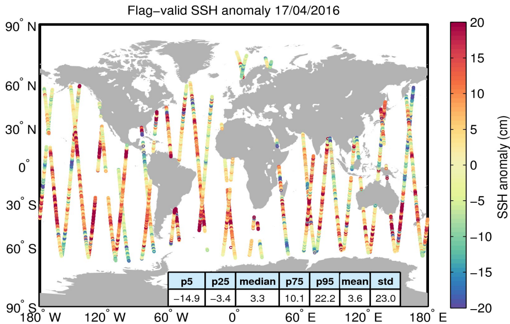
Figure 5. Geographical distribution of flag-valid 1-Hz SSH anomaly data over oceans and lakes for 17/04/2016. The statistical values shown in the table refer to the SSH anomaly in cm and are calculated over all measurements shown in the figure.
