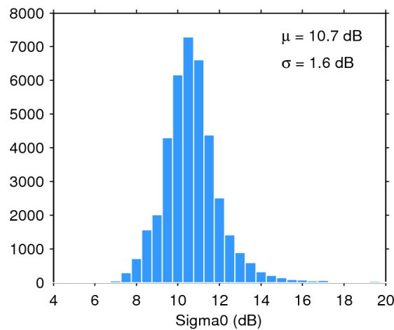
Figure 28. Histogram of science-valid sigma0 over oceans and lakes for 17/04/2016. The mean ( \mu ) and standard deviation ( \sigma ) are also shown. Note that values outside [4 20] dB are excluded from the histogram for the sake of readability but not from the computation of \mu and \sigma .
