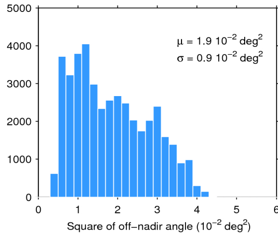
Figure 39. Histogram of flag-valid mispointing over oceans and lakes for 17/04/2016. The mean ( \mu ) and standard deviation ( \sigma ) are also shown. Note that values larger than 6 \cdot 10^{-2} \text{ deg}^2 are excluded from the histogram for the sake of readability but not from the computation of \mu and \sigma .
