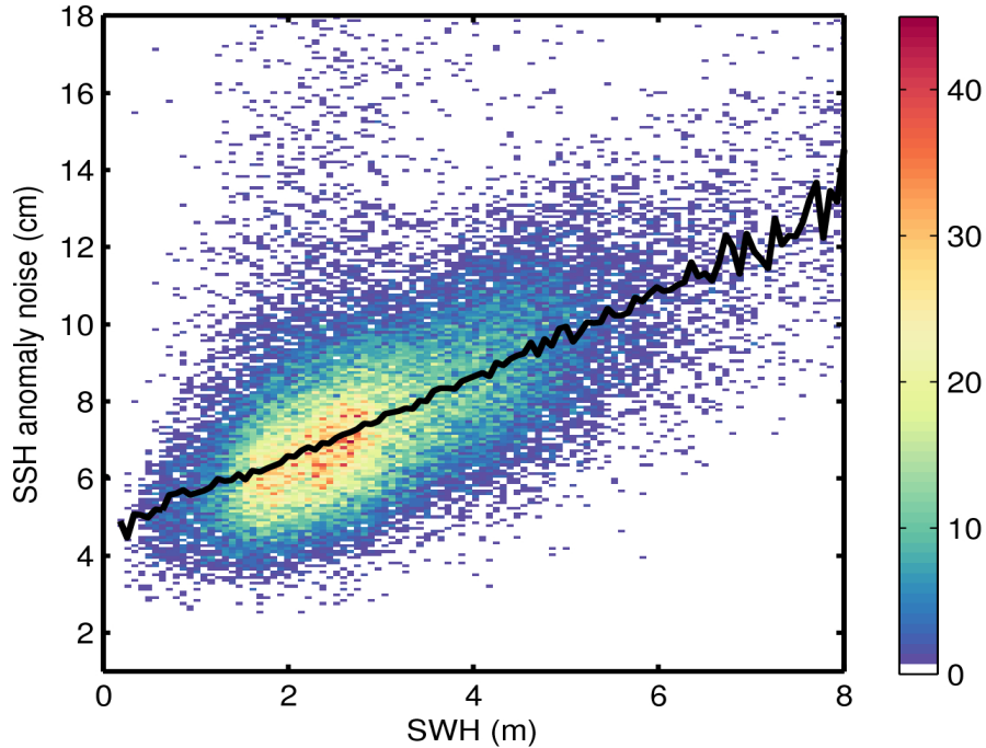
Figure 9. 2D histogram showing flag-valid SSH anomaly noise as a function of SWH for 17/04/2016. The black line denotes the median SSH anomaly noise as a function of SWH.
