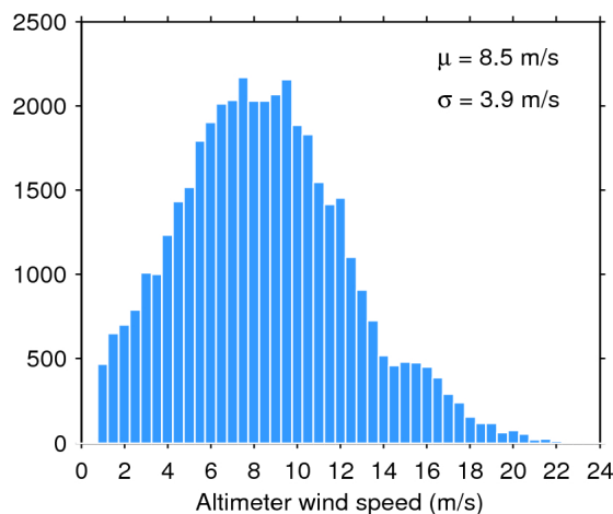
Figure 35. Histogram of science-valid wind over oceans and lakes for 17/04/2016. The mean ( \mu ) and standard deviation ( \sigma ) are also shown. Note that values larger than 24 m/s are excluded from the histogram for the sake of readability but not from the computation of \mu and \sigma .
