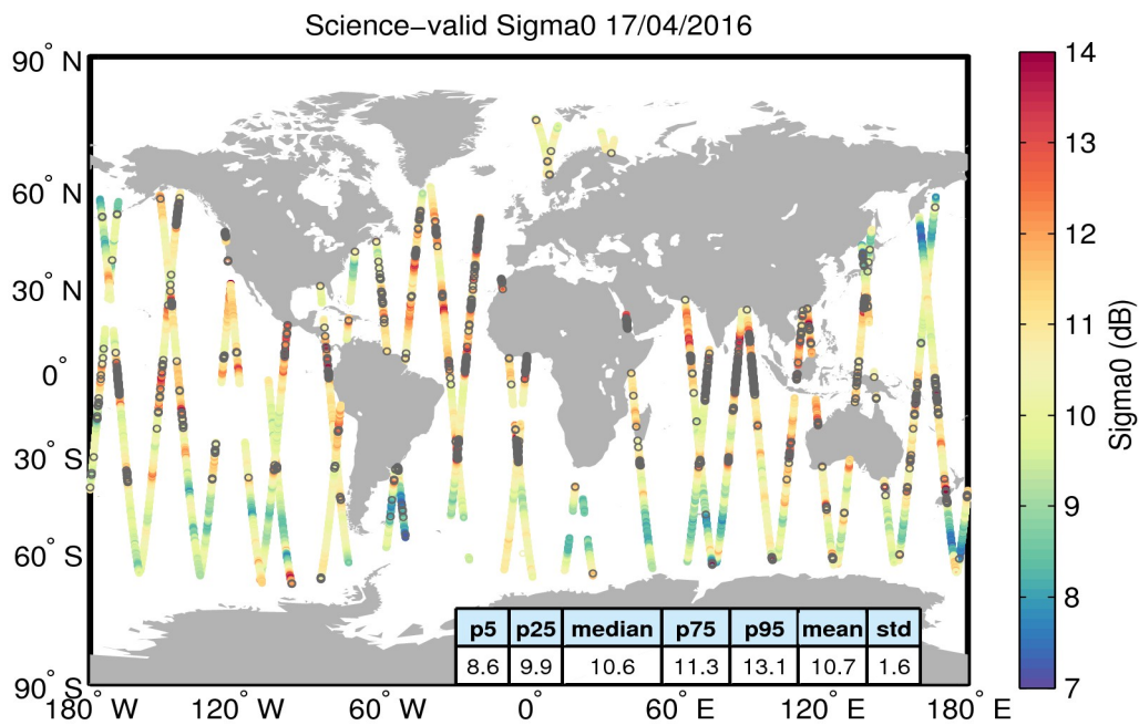
Figure 27. Geographical distribution of science-valid sigma0 data over oceans and lakes for 17/04/2016. The statistical values shown in the table refer to the sigma0 in dB and are calculated over all measurements shown in the figure. Gray circles denote records that have been rejected based on the editing criteria described in Table 4.
