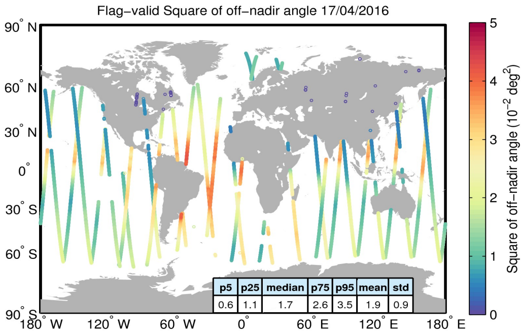
Figure 37. Geographical distribution of flag-valid mispointing data over oceans and lakes for 17/04/2016. The statistical values shown in the table refer to the mispointing in 10^{-2} \text{ deg}^2 and are calculated over all measurements shown in the figure.
