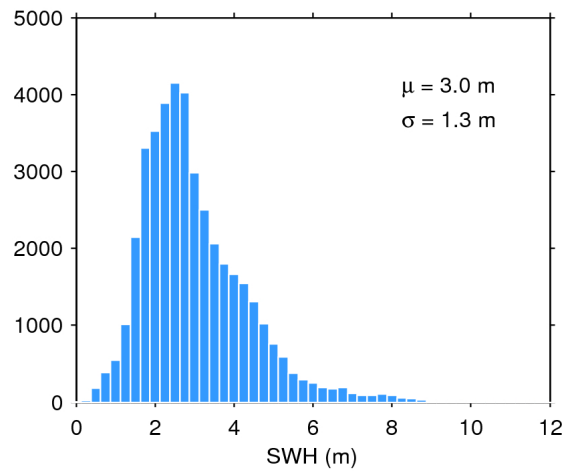
Figure 17. Histogram of flag-valid SWH over oceans and lakes for 17/04/2016. The mean ( \mu ) and standard deviation ( \sigma ) are also shown. Note that values larger than 12 m are excluded from the histogram for the sake of readability but not from the computation of \mu and \sigma .
