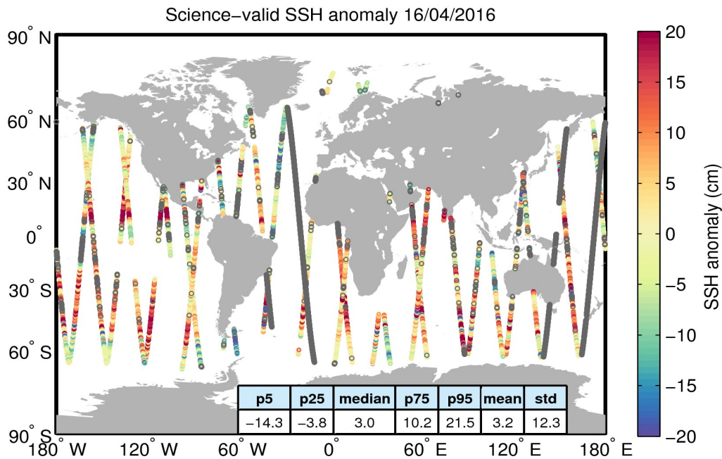
Figure 10. Geographical distribution of science-valid SSH anomaly data over oceans and lakes for 16/04/2016. The statistical values shown in the table refer to the SSH anomaly in cm and are calculated over all measurements shown in the figure. Gray circles denote records that have been rejected based on the editing criteria described in Table 2.
