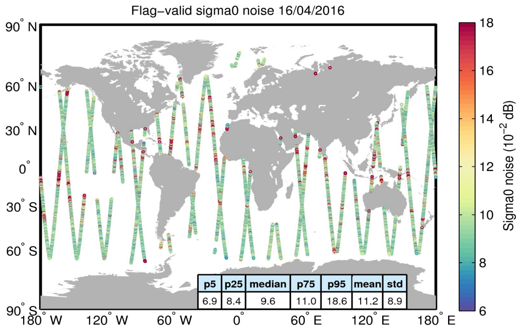
Figure 26. Geographical distribution of flag-valid 20-Hz sigma0 measurement noise over oceans and lakes for 16/04/2016. The statistical values shown in the table refer to the sigma0 noise and are calculated over all measurements shown in the figure.
