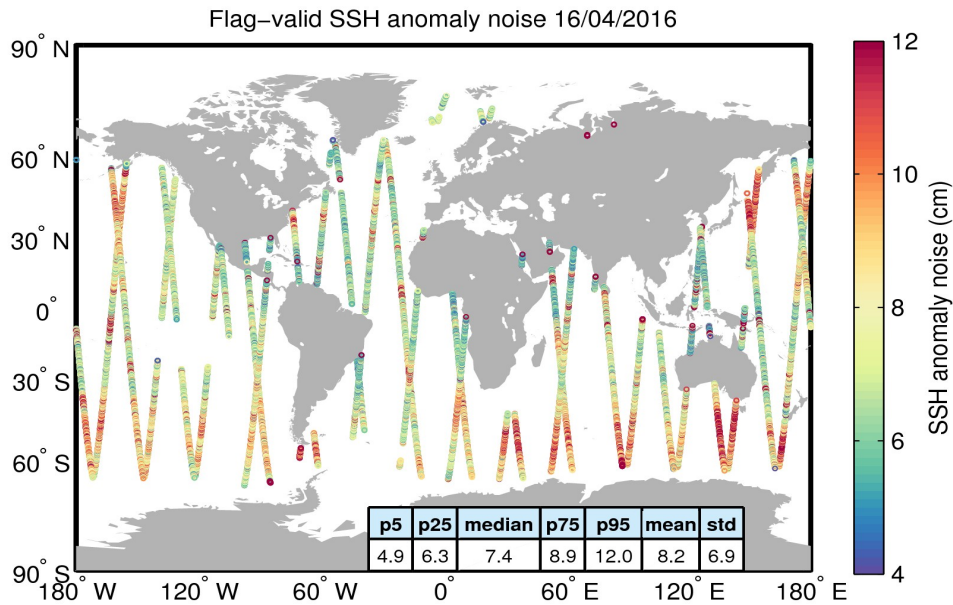
Figure 8. Geographical distribution of flag-valid 20-Hz SSH anomaly measurement noise over oceans and lakes for 16/04/2016. The statistical values shown in the table refer to the SSH anomaly noise and are calculated over all measurements shown in the figure.
