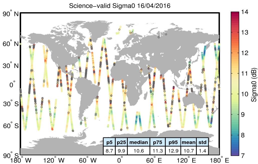
Figure 27. Geographical distribution of science-valid sigma0 data over oceans and lakes for 16/04/2016. The statistical values shown in the table refer to the sigma0 in dB and are calculated over all measurements shown in the figure. Gray circles denote records that have been rejected based on the editing criteria described in Table 4.
