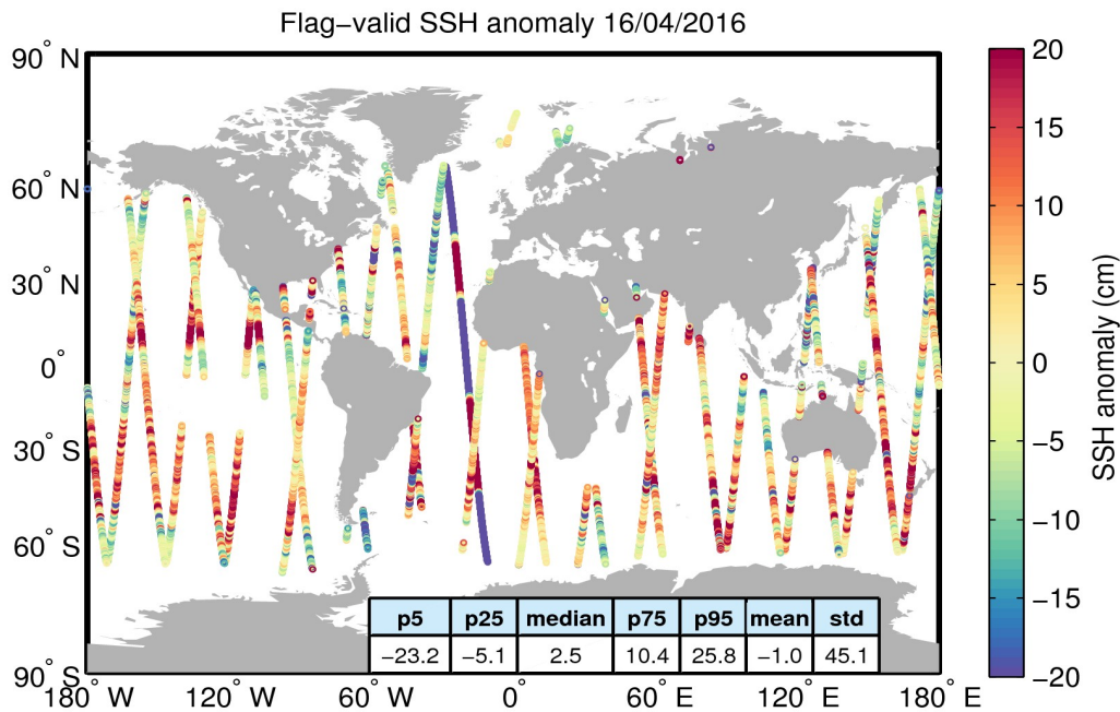
Figure 5. Geographical distribution of flag-valid 1-Hz SSH anomaly data over oceans and lakes for 16/04/2016. The statistical values shown in the table refer to the SSH anomaly in cm and are calculated over all measurements shown in the figure.
