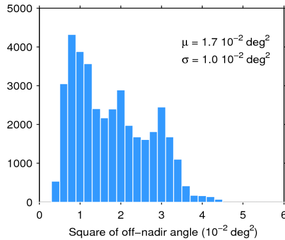
Figure 39. Histogram of flag-valid mispointing over oceans and lakes for 16/04/2016. The mean ( \mu ) and standard deviation ( \sigma ) are also shown. Note that values larger than 6 \cdot 10^{-2} \text{ deg}^2 are excluded from the histogram for the sake of readability but not from the computation of \mu and \sigma .
