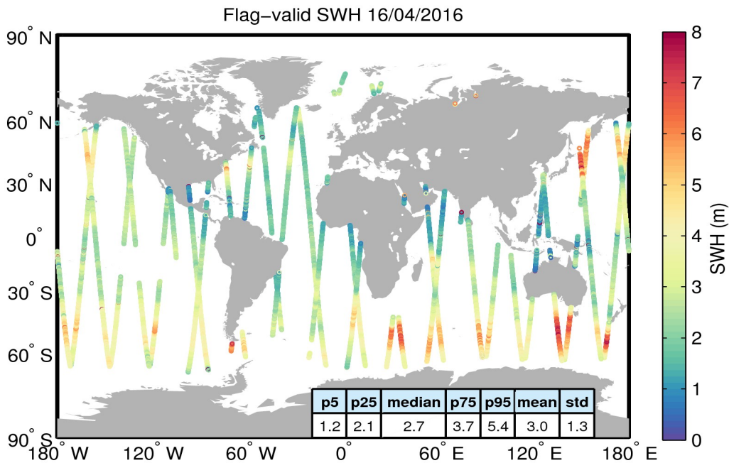
Figure 15. Geographical distribution of flag-valid SWH data over oceans and lakes for 16/04/2016. The statistical values shown in the table refer to the SWH in m and are calculated over all measurements shown in the figure.
