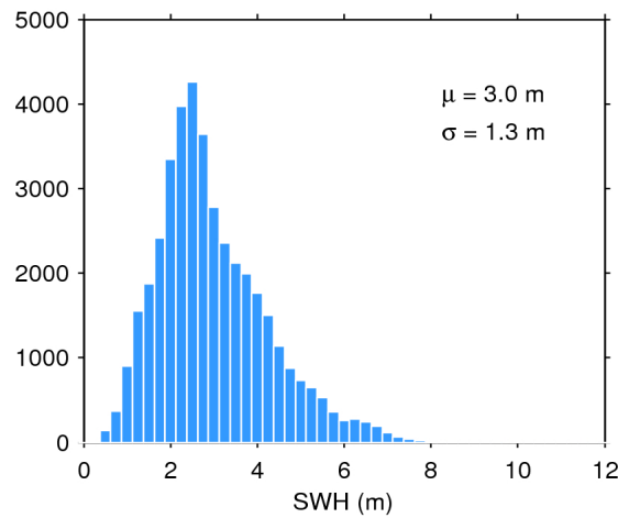
Figure 17. Histogram of flag-valid SWH over oceans and lakes for 16/04/2016. The mean ( \mu ) and standard deviation ( \sigma ) are also shown. Note that values larger than 12 m are excluded from the histogram for the sake of readability but not from the computation of \mu and \sigma .
