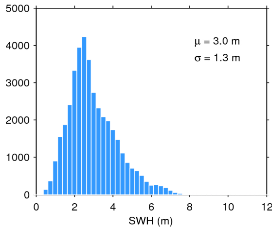
Figure 20. Histogram of science-valid SWH over oceans and lakes for 16/04/2016. The mean ( \mu ) and standard deviation ( \sigma ) are also shown. Note that values larger than 12 m are excluded from the histogram for the sake of readability but not from the computation of \mu and \sigma .
