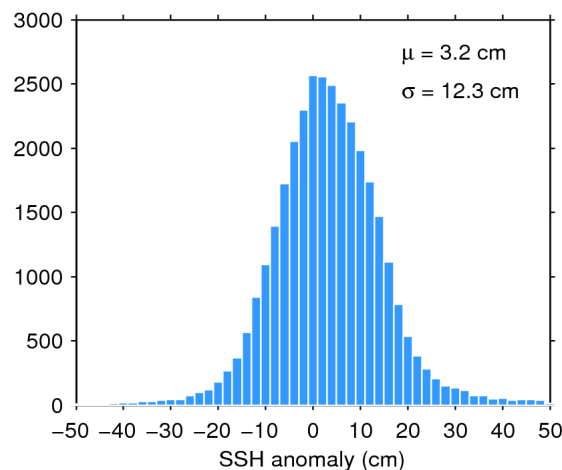
Figure 11. Histogram of science-valid SSH anomaly over oceans and lakes for 16/04/2016. The mean ( \mu ) and standard deviation ( \sigma ) are also shown. Note that values outside [-50 50] cm are excluded from the histogram for the sake of readability but not from the computation of \mu and \sigma .
