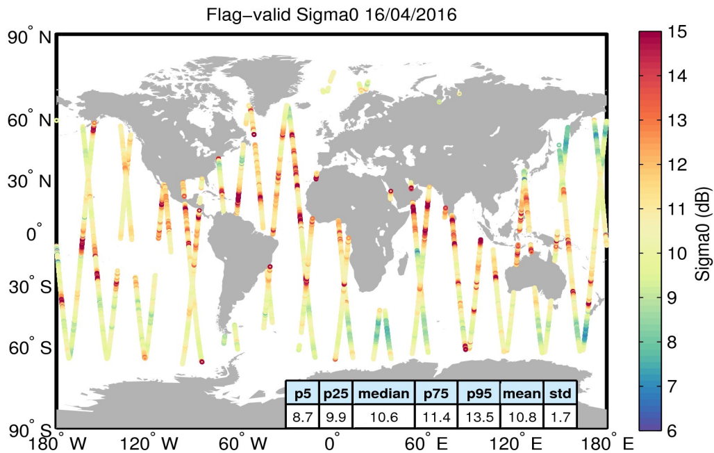
Figure 23. Geographical distribution of flag-valid sigma0 data over oceans and lakes for 16/04/2016. The statistical values shown in the table refer to the sigma0 in dB and are calculated over all measurements shown in the figure.
