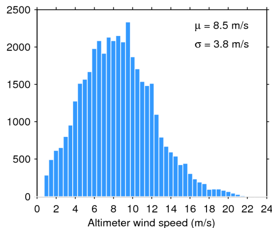
Figure 35. Histogram of science-valid wind over oceans and lakes for 16/04/2016. The mean ( \mu ) and standard deviation ( \sigma ) are also shown. Note that values larger than 24 m/s are excluded from the histogram for the sake of readability but not from the computation of \mu and \sigma .
