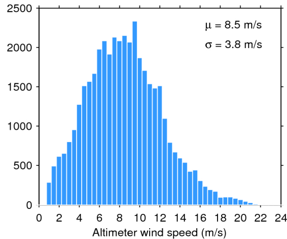
Figure 33. Histogram of flag-valid wind over oceans and lakes for 16/04/2016. The mean ( \mu ) and standard deviation ( \sigma ) are also shown. Note that values larger than 24 m/s are excluded from the histogram for the sake of readability but not from the computation of \mu and \sigma .
