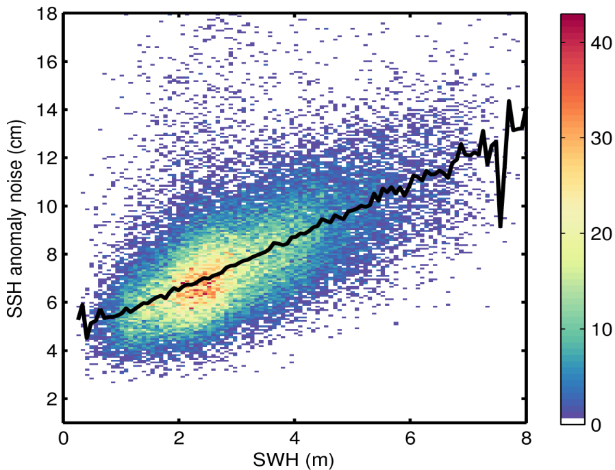
Figure 9. 2D histogram showing flag-valid SSH anomaly noise as a function of SWH for 16/04/2016. The black line denotes the median SSH anomaly noise as a function of SWH.
