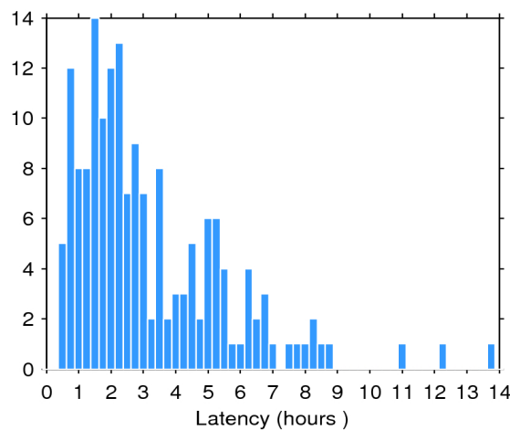
Figure 2. Histogram of the data latency for 16/04/2016. The y-axis denotes the number of files that are made available with a delay of x-hours with respect to the mean time of the records stored in the file.
