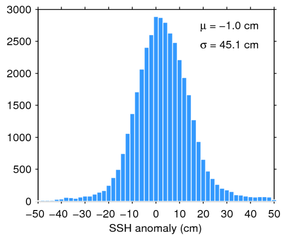
Figure 7. Histogram of flag-valid SSH anomaly over oceans and lakes for 16/04/2016. The mean ( \mu ) and standard deviation ( \sigma ) are also shown. Note that values outside [-50 50] cm are excluded from the histogram for the sake of readability but not from the computation of \mu and \sigma .
