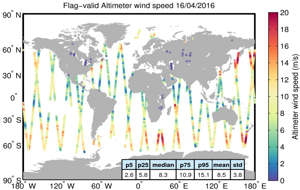
Figure 31. Geographical distribution of flag-valid wind data over oceans and lakes for 16/04/2016. The statistical values shown in the table refer to the wind in m/s and are calculated over all measurements shown in the figure.
