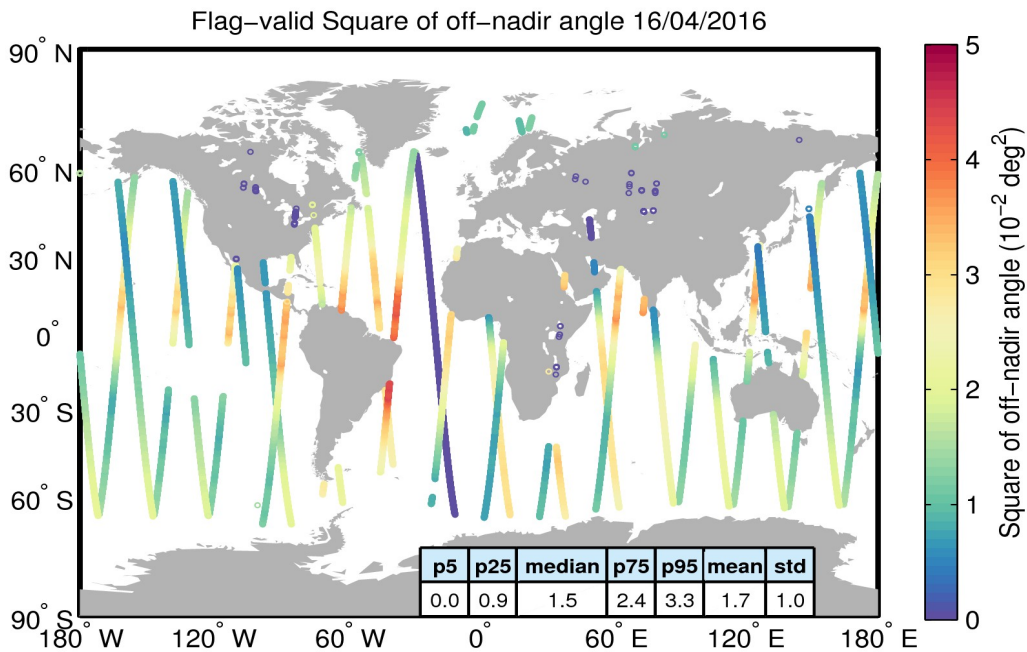
Figure 37. Geographical distribution of flag-valid mispointing data over oceans and lakes for 16/04/2016. The statistical values shown in the table refer to the mispointing in 10^{-2} \text{ deg}^2 and are calculated over all measurements shown in the figure.
