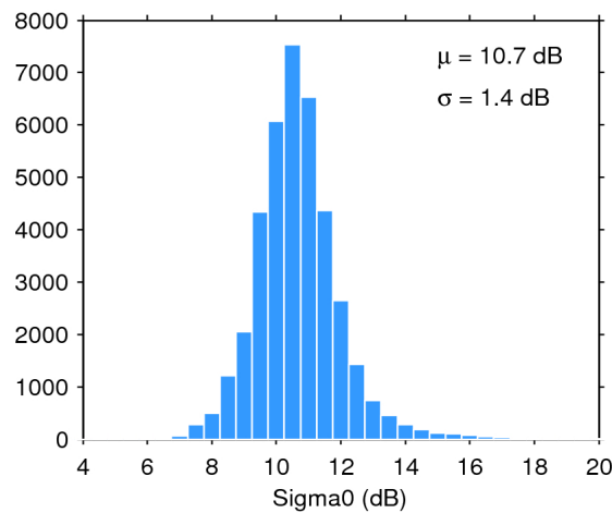
Figure 28. Histogram of science-valid sigma0 over oceans and lakes for 16/04/2016. The mean ( \mu ) and standard deviation ( \sigma ) are also shown. Note that values outside [4 20] dB are excluded from the histogram for the sake of readability but not from the computation of \mu and \sigma .
