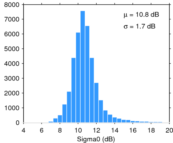
Figure 25. Histogram of flag-valid sigma0 over oceans and lakes for 16/04/2016. The mean ( \mu ) and standard deviation ( \sigma ) are also shown. Note that values outside [4 20] dB are excluded from the histogram for the sake of readability but not from the computation of \mu and \sigma .
