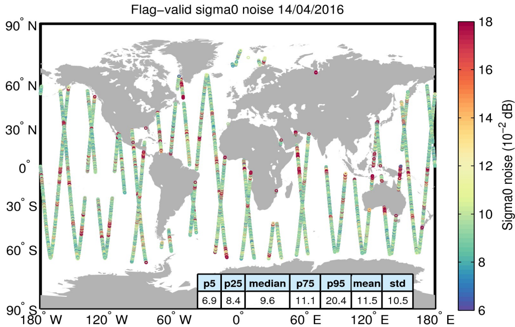
Figure 26. Geographical distribution of flag-valid 20-Hz sigma0 measurement noise over oceans and lakes for 14/04/2016. The statistical values shown in the table refer to the sigma0 noise and are calculated over all measurements shown in the figure.
