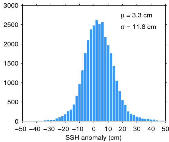
Figure 11. Histogram of science-valid SSH anomaly over oceans and lakes for 14/04/2016. The mean ( \mu ) and standard deviation ( \sigma ) are also shown. Note that values outside [-50 50] cm are excluded from the histogram for the sake of readability but not from the computation of \mu and \sigma .
