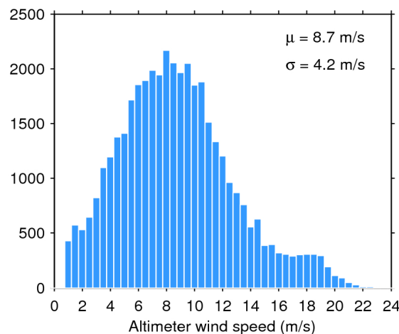
Figure 35. Histogram of science-valid wind over oceans and lakes for 14/04/2016. The mean ( \mu ) and standard deviation ( \sigma ) are also shown. Note that values larger than 24 m/s are excluded from the histogram for the sake of readability but not from the computation of \mu and \sigma .
