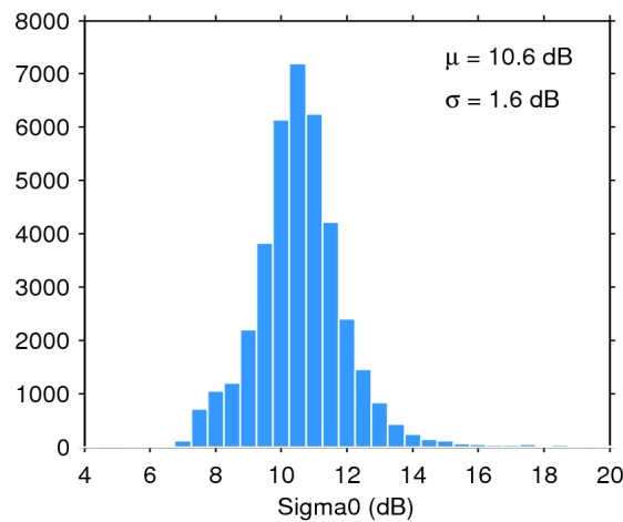
Figure 28. Histogram of science-valid sigma0 over oceans and lakes for 14/04/2016. The mean ( \mu ) and standard deviation ( \sigma ) are also shown. Note that values outside [4 20] dB are excluded from the histogram for the sake of readability but not from the computation of \mu and \sigma .
