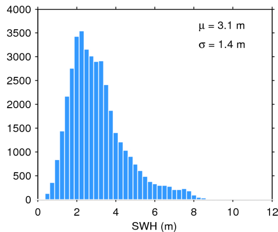
Figure 20. Histogram of science-valid SWH over oceans and lakes for 14/04/2016. The mean ( \mu ) and standard deviation ( \sigma ) are also shown. Note that values larger than 12 m are excluded from the histogram for the sake of readability but not from the computation of \mu and \sigma .
