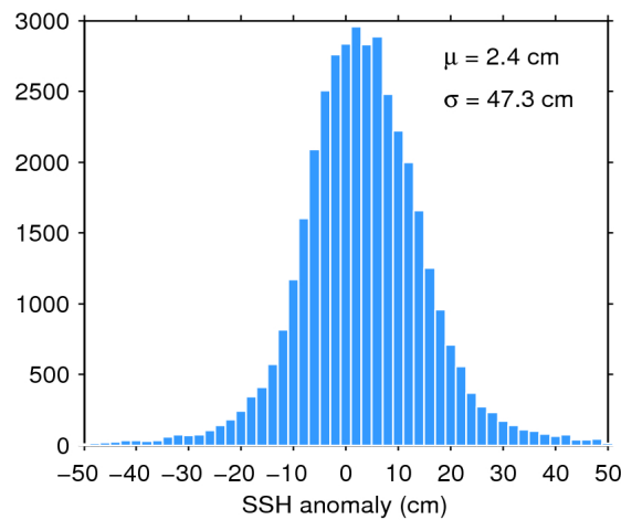
Figure 7. Histogram of flag-valid SSH anomaly over oceans and lakes for 14/04/2016. The mean ( \mu ) and standard deviation ( \sigma ) are also shown. Note that values outside [-50\ 50] cm are excluded from the histogram for the sake of readability but not from the computation of \mu and \sigma .
