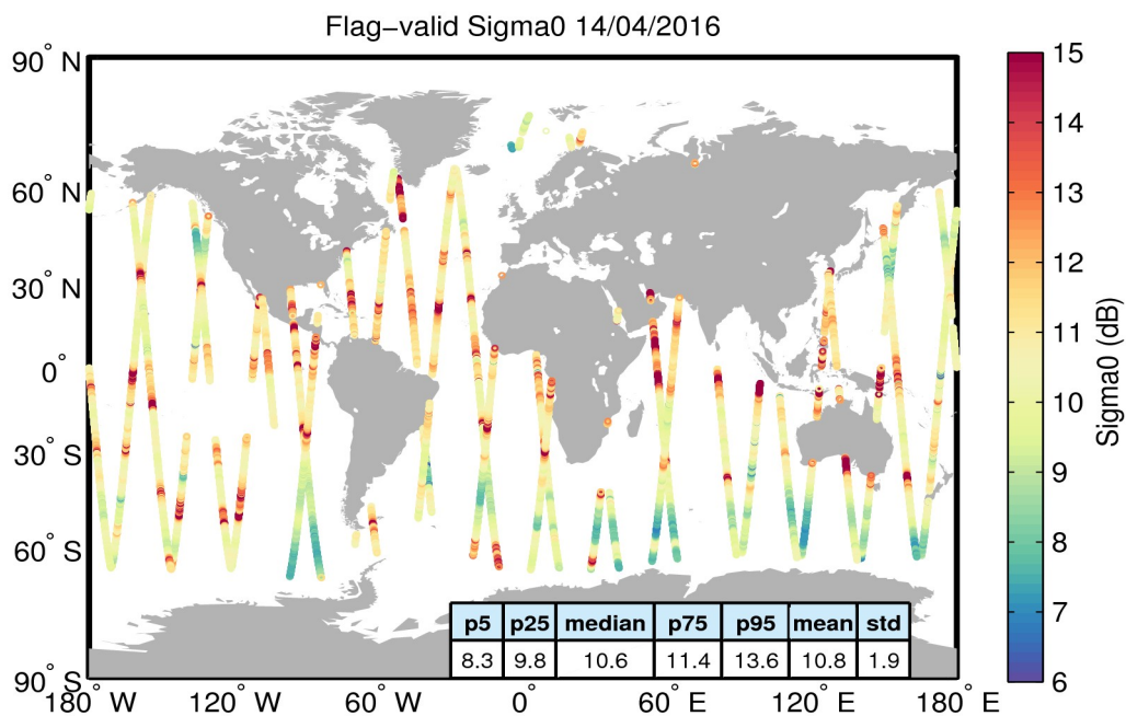
Figure 23. Geographical distribution of flag-valid sigma0 data over oceans and lakes for 14/04/2016. The statistical values shown in the table refer to the sigma0 in dB and are calculated over all measurements shown in the figure.
