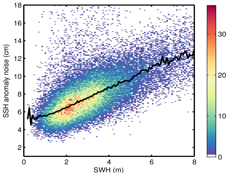
Figure 9. 2D histogram showing flag-valid SSH anomaly noise as a function of SWH for 14/04/2016. The black line denotes the median SSH anomaly noise as a function of SWH.
