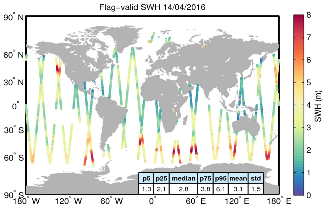
Figure 15. Geographical distribution of flag-valid SWH data over oceans and lakes for 14/04/2016. The statistical values shown in the table refer to the SWH in m and are calculated over all measurements shown in the figure.
