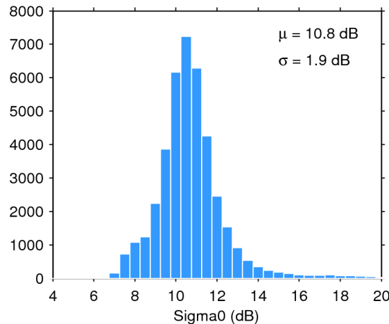
Figure 25. Histogram of flag-valid sigma0 over oceans and lakes for 14/04/2016. The mean ( \mu ) and standard deviation ( \sigma ) are also shown. Note that values outside [4 20] dB are excluded from the histogram for the sake of readability but not from the computation of \mu and \sigma .
