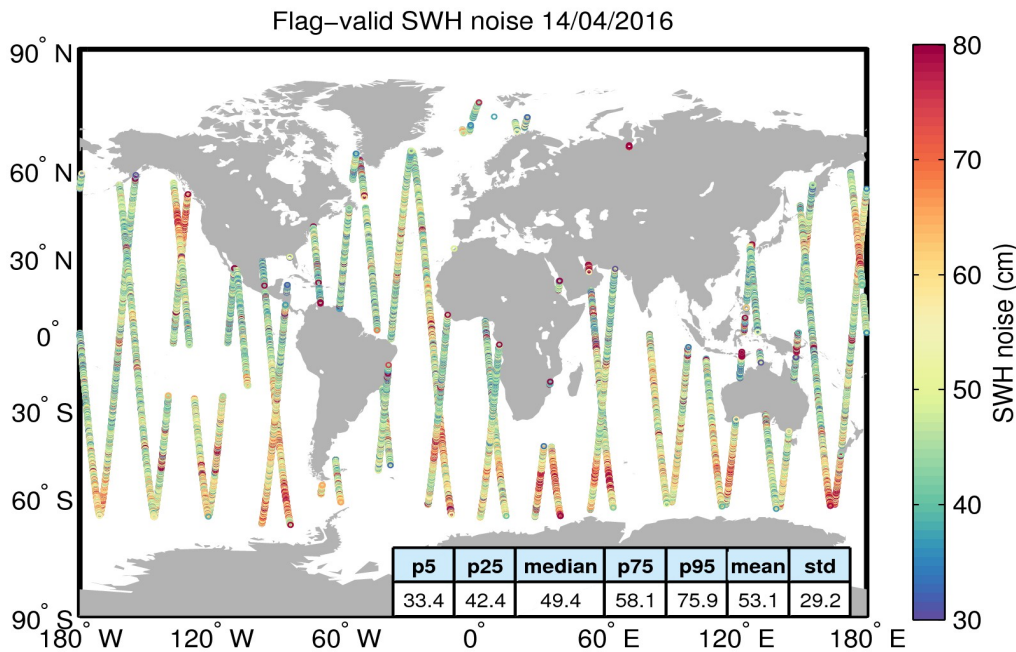
Figure 18. Geographical distribution of flag-valid 20-Hz SWH measurement noise over oceans and lakes for 14/04/2016. The statistical values shown in the table refer to the SWH noise and are calculated over all measurements shown in the figure.
