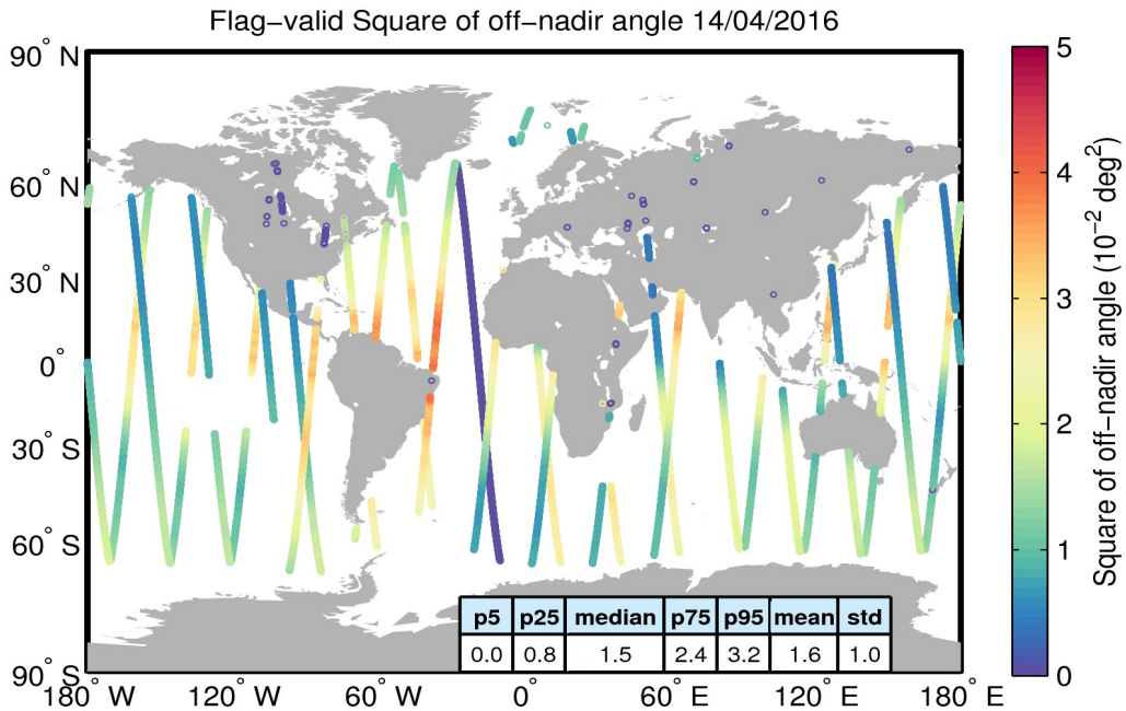
Figure 37. Geographical distribution of flag-valid mispointing data over oceans and lakes for 14/04/2016. The statistical values shown in the table refer to the mispointing in 10^{-2} deg 2 and are calculated over all measurements shown in the figure.
