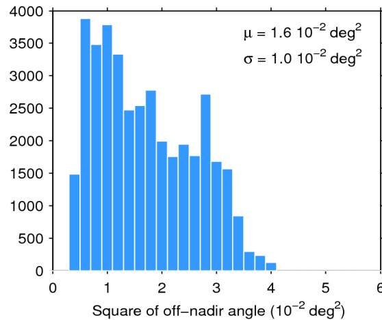
Figure 39. Histogram of flag-valid mispointing over oceans and lakes for 14/04/2016. The mean ( \mu ) and standard deviation ( \sigma ) are also shown. Note that values larger than 6 \cdot 10^{-2} \text{ deg}^2 are excluded from the histogram for the sake of readability but not from the computation of \mu and \sigma .
