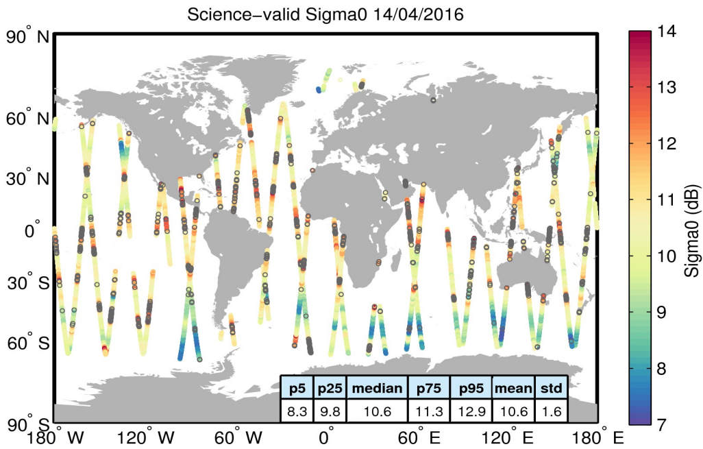
Figure 27. Geographical distribution of science-valid sigma0 data over oceans and lakes for 14/04/2016. The statistical values shown in the table refer to the sigma0 in dB and are calculated over all measurements shown in the figure. Gray circles denote records that have been rejected based on the editing criteria described in Table 4.
