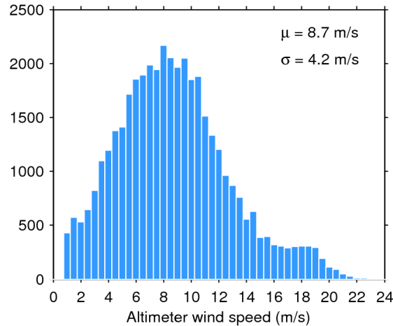
Figure 33. Histogram of flag-valid wind over oceans and lakes for 14/04/2016. The mean ( \mu ) and standard deviation ( \sigma ) are also shown. Note that values larger than 24 m/s are excluded from the histogram for the sake of readability but not from the computation of \mu and \sigma .
