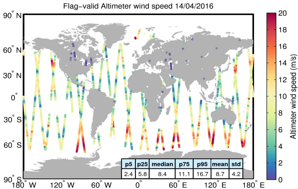
Figure 31. Geographical distribution of flag-valid wind data over oceans and lakes for 14/04/2016. The statistical values shown in the table refer to the wind in m/s and are calculated over all measurements shown in the figure.
