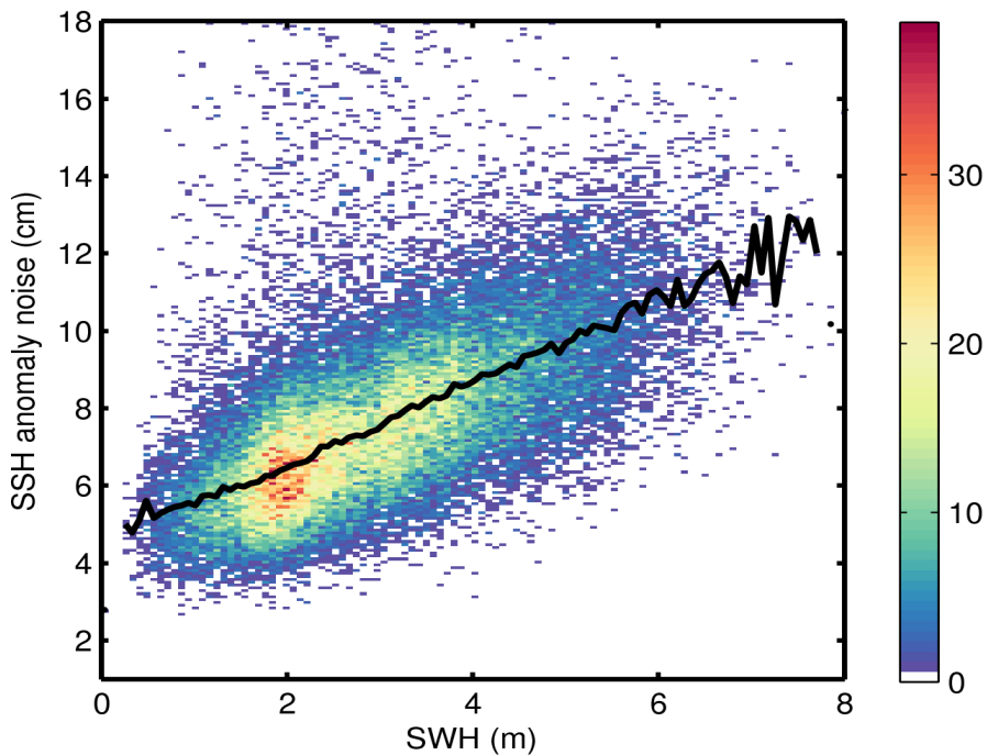
Figure 9. 2D histogram showing flag-valid SSH anomaly noise as a function of SWH for 13/04/2016. The black line denotes the median SSH anomaly noise as a function of SWH.
