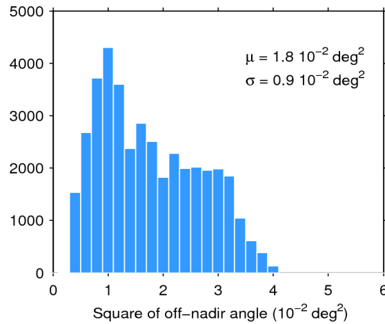
Figure 39. Histogram of flag-valid mispointing over oceans and lakes for 13/04/2016. The mean ( \mu ) and standard deviation ( \sigma ) are also shown. Note that values larger than 6 \cdot 10^{-2} \text{ deg}^2 are excluded from the histogram for the sake of readability but not from the computation of \mu and \sigma .
