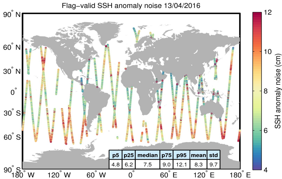
Figure 8. Geographical distribution of flag-valid 20-Hz SSH anomaly measurement noise over oceans and lakes for 13/04/2016. The statistical values shown in the table refer to the SSH anomaly noise and are calculated over all measurements shown in the figure.
