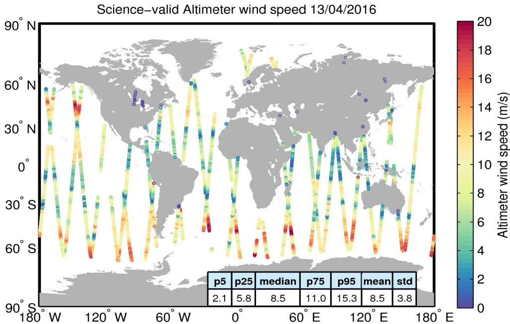
Figure 34. Geographical distribution of science-valid wind data over oceans and lakes for 13/04/2016. The statistical values shown in the table refer to the wind in m/s and are calculated over all measurements shown in the figure. Gray circles denote records that have been rejected based on the editing criteria described in Table 5.
