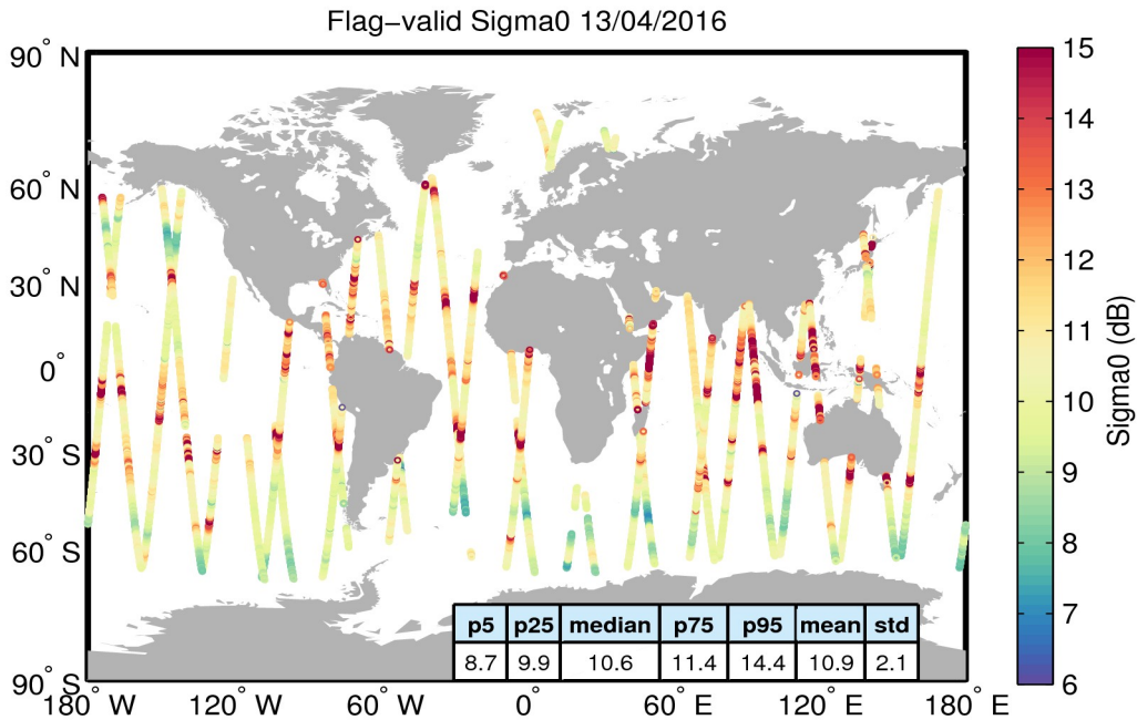
Figure 23. Geographical distribution of flag-valid sigma0 data over oceans and lakes for 13/04/2016. The statistical values shown in the table refer to the sigma0 in dB and are calculated over all measurements shown in the figure.
