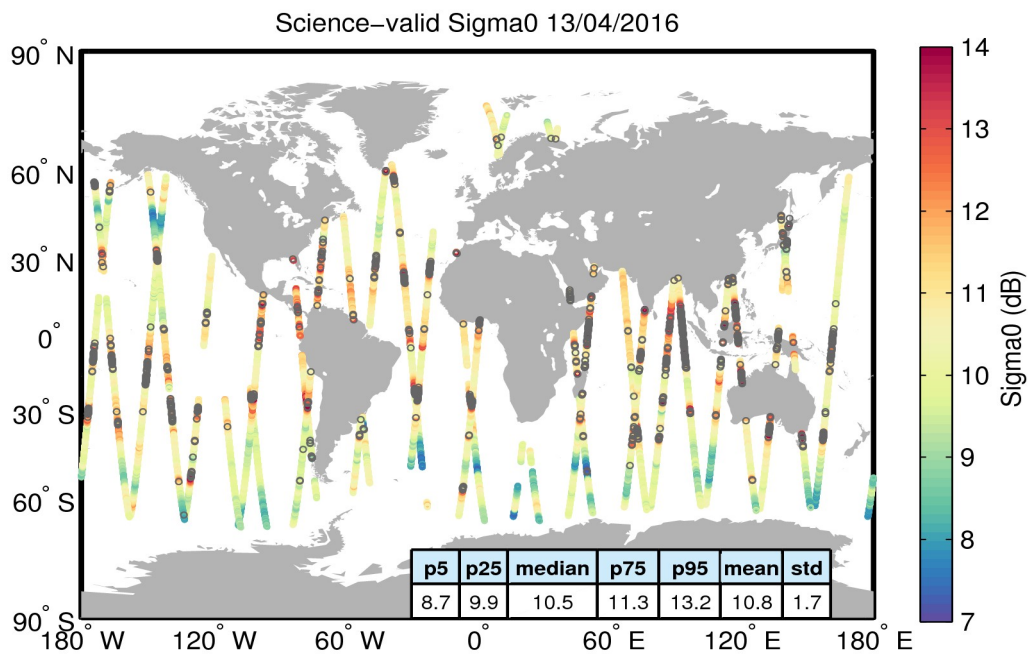
Figure 27. Geographical distribution of science-valid sigma0 data over oceans and lakes for 13/04/2016. The statistical values shown in the table refer to the sigma0 in dB and are calculated over all measurements shown in the figure. Gray circles denote records that have been rejected based on the editing criteria described in Table 4.
