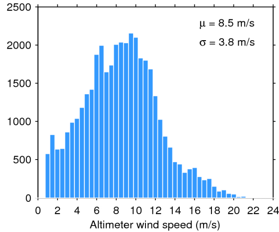
Figure 33. Histogram of flag-valid wind over oceans and lakes for 13/04/2016. The mean ( \mu ) and standard deviation ( \sigma ) are also shown. Note that values larger than 24 m/s are excluded from the histogram for the sake of readability but not from the computation of \mu and \sigma .
