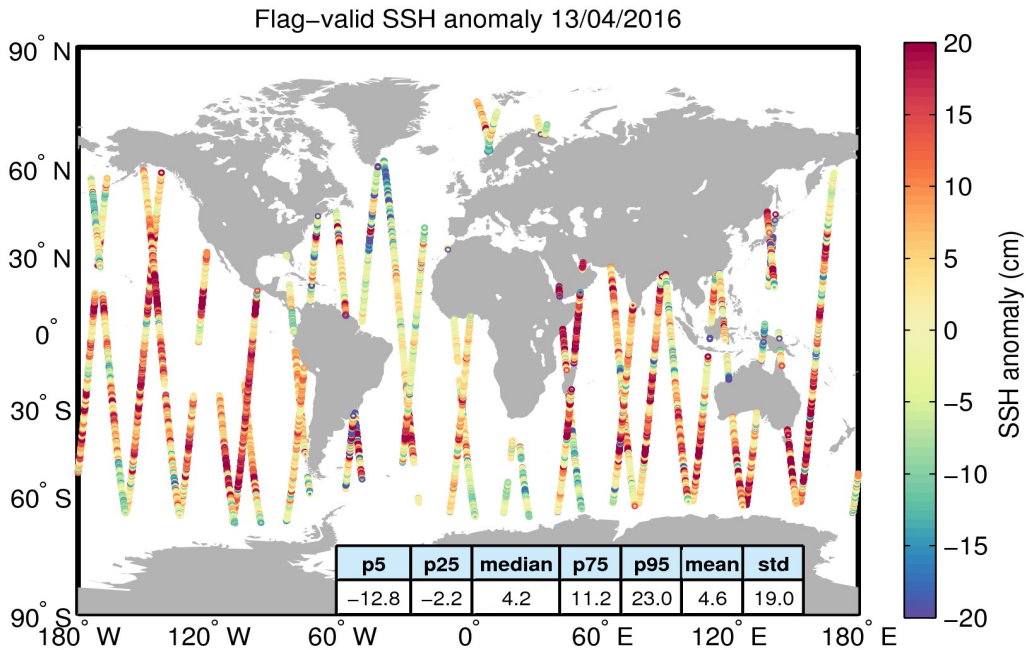
Figure 5. Geographical distribution of flag-valid 1-Hz SSH anomaly data over oceans and lakes for 13/04/2016. The statistical values shown in the table refer to the SSH anomaly in cm and are calculated over all measurements shown in the figure.
