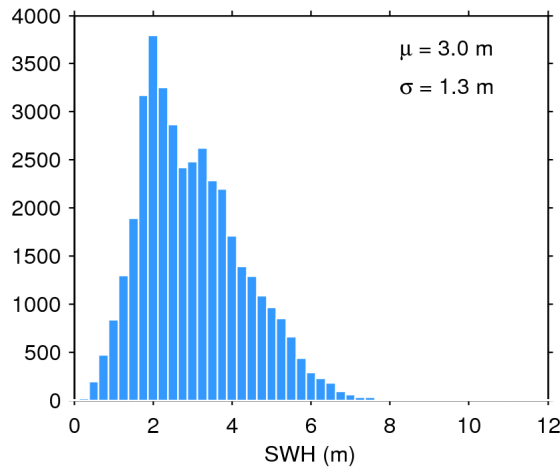
Figure 17. Histogram of flag-valid SWH over oceans and lakes for 13/04/2016. The mean ( \mu ) and standard deviation ( \sigma ) are also shown. Note that values larger than 12 m are excluded from the histogram for the sake of readability but not from the computation of \mu and \sigma .
