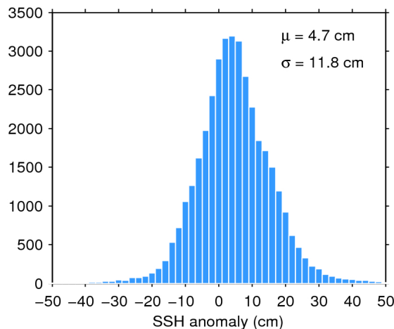
Figure 11. Histogram of science-valid SSH anomaly over oceans and lakes for 13/04/2016. The mean ( \mu ) and standard deviation ( \sigma ) are also shown. Note that values outside [-50 50] cm are excluded from the histogram for the sake of readability but not from the computation of \mu and \sigma .
