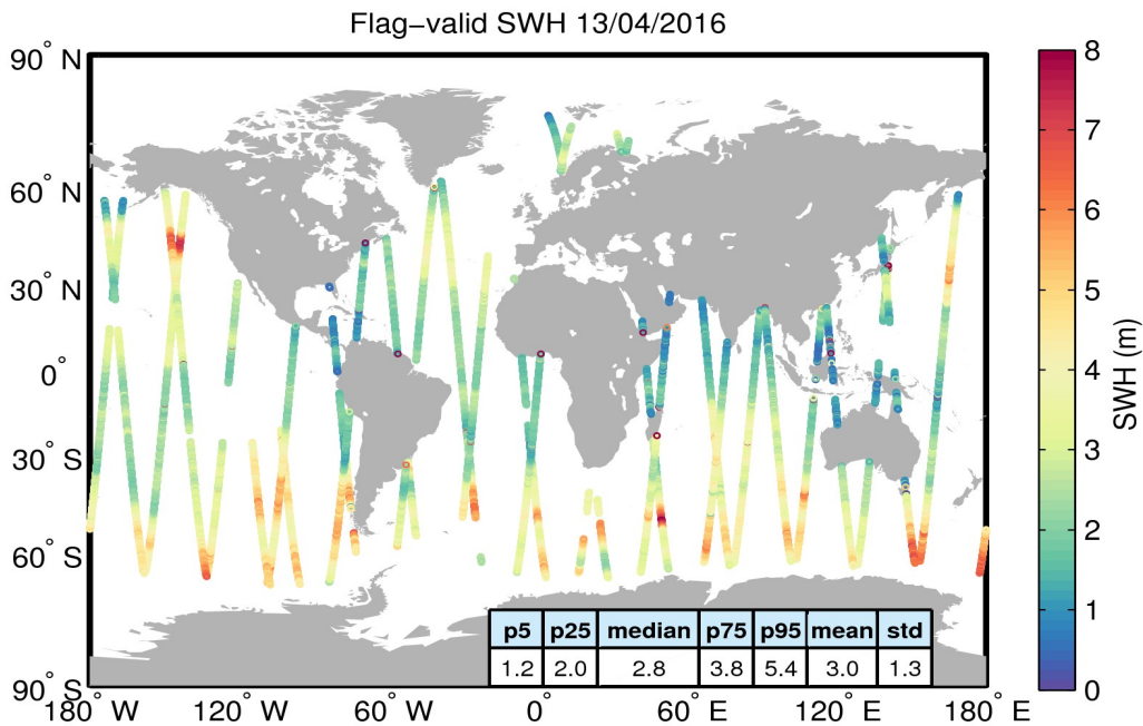
Figure 15. Geographical distribution of flag-valid SWH data over oceans and lakes for 13/04/2016. The statistical values shown in the table refer to the SWH in m and are calculated over all measurements shown in the figure.
