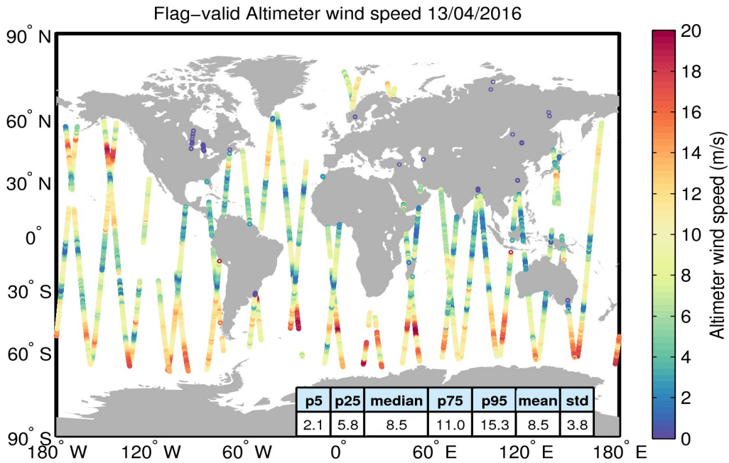
Figure 31. Geographical distribution of flag-valid wind data over oceans and lakes for 13/04/2016. The statistical values shown in the table refer to the wind in m/s and are calculated over all measurements shown in the figure.
