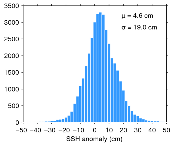
Figure 7. Histogram of flag-valid SSH anomaly over oceans and lakes for 13/04/2016. The mean ( \mu ) and standard deviation ( \sigma ) are also shown. Note that values outside [-50 50] cm are excluded from the histogram for the sake of readability but not from the computation of \mu and \sigma .
