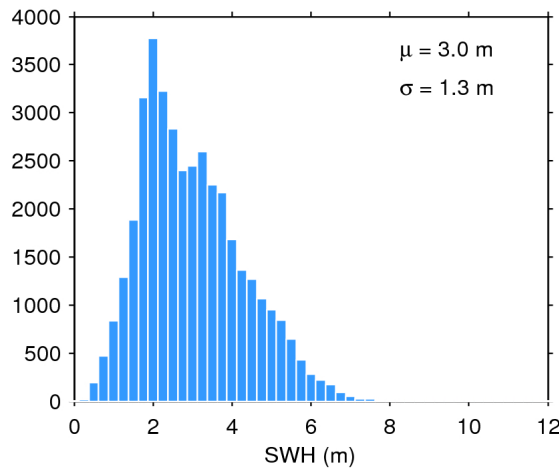
Figure 20. Histogram of science-valid SWH over oceans and lakes for 13/04/2016. The mean ( \mu ) and standard deviation ( \sigma ) are also shown. Note that values larger than 12 m are excluded from the histogram for the sake of readability but not from the computation of \mu and \sigma .
