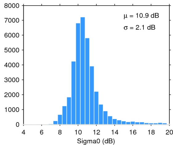
Figure 25. Histogram of flag-valid sigma0 over oceans and lakes for 13/04/2016. The mean ( \mu ) and standard deviation ( \sigma ) are also shown. Note that values outside [4 20] dB are excluded from the histogram for the sake of readability but not from the computation of \mu and \sigma .
