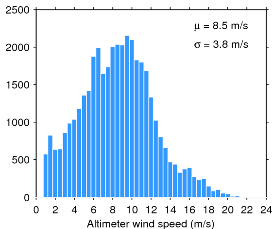
Figure 35. Histogram of science-valid wind over oceans and lakes for 13/04/2016. The mean ( \mu ) and standard deviation ( \sigma ) are also shown. Note that values larger than 24 m/s are excluded from the histogram for the sake of readability but not from the computation of \mu and \sigma .
