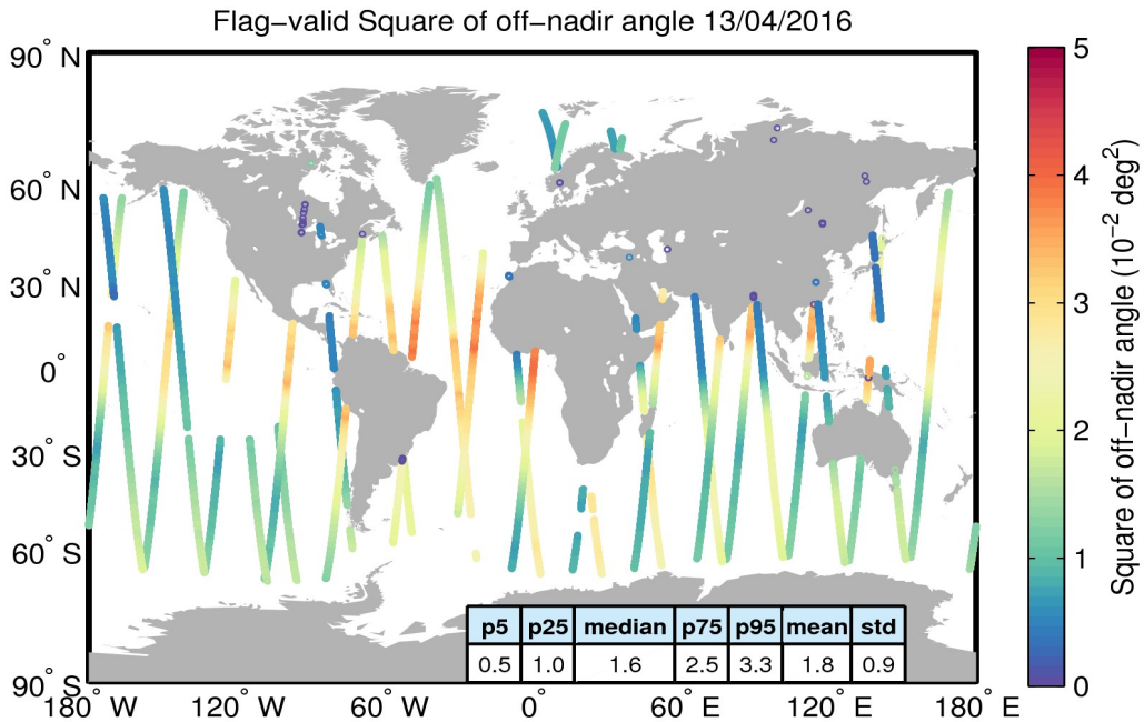
Figure 37. Geographical distribution of flag-valid mispointing data over oceans and lakes for 13/04/2016. The statistical values shown in the table refer to the mispointing in 10^{-2} \text{ deg}^2 and are calculated over all measurements shown in the figure.
