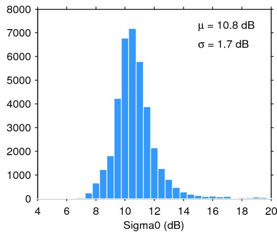
Figure 28. Histogram of science-valid sigma0 over oceans and lakes for 13/04/2016. The mean ( \mu ) and standard deviation ( \sigma ) are also shown. Note that values outside [4 20] dB are excluded from the histogram for the sake of readability but not from the computation of \mu and \sigma .
