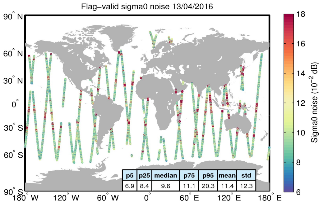
Figure 26. Geographical distribution of flag-valid 20-Hz sigma0 measurement noise over oceans and lakes for 13/04/2016. The statistical values shown in the table refer to the sigma0 noise and are calculated over all measurements shown in the figure.
