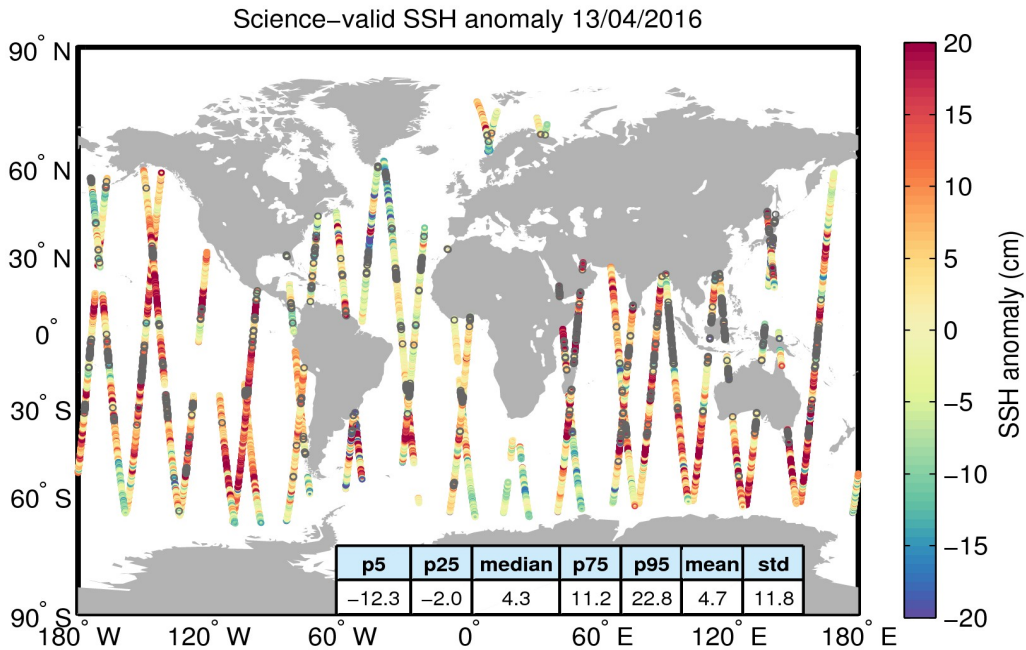
Figure 10. Geographical distribution of science-valid SSH anomaly data over oceans and lakes for 13/04/2016. The statistical values shown in the table refer to the SSH anomaly in cm and are calculated over all measurements shown in the figure. Gray circles denote records that have been rejected based on the editing criteria described in Table 2.
