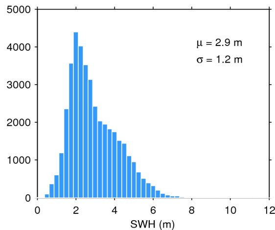
Figure 20. Histogram of science-valid SWH over oceans and lakes for 12/04/2016. The mean ( \mu ) and standard deviation ( \sigma ) are also shown. Note that values larger than 12 m are excluded from the histogram for the sake of readability but not from the computation of \mu and \sigma .
