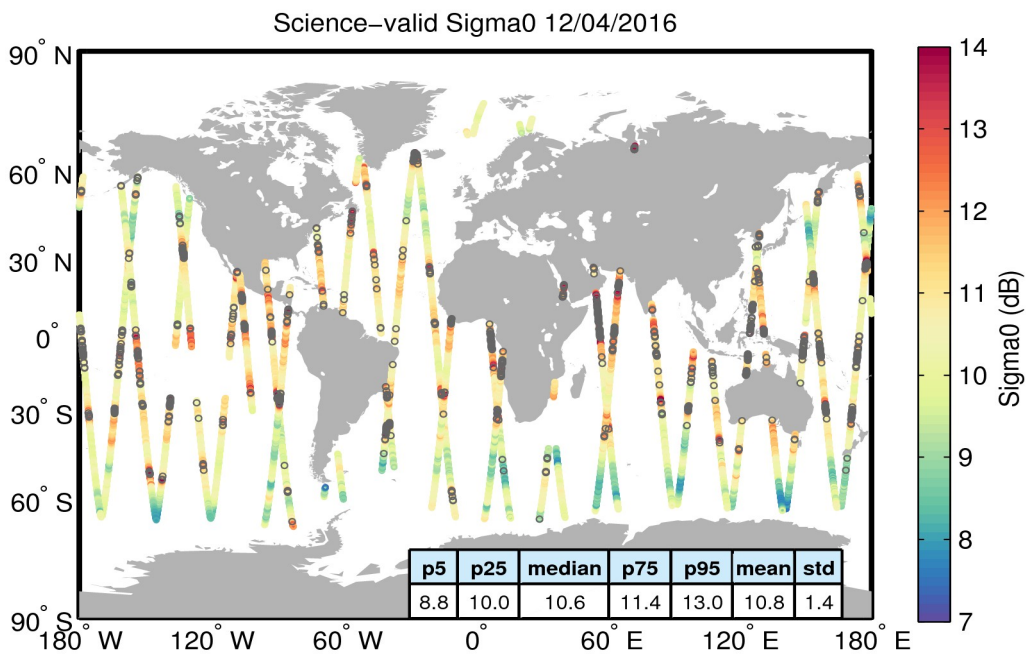
Figure 27. Geographical distribution of science-valid sigma0 data over oceans and lakes for 12/04/2016. The statistical values shown in the table refer to the sigma0 in dB and are calculated over all measurements shown in the figure. Gray circles denote records that have been rejected based on the editing criteria described in Table 4.
