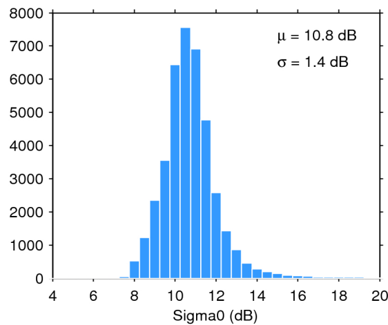
Figure 28. Histogram of science-valid sigma0 over oceans and lakes for 12/04/2016. The mean ( \mu ) and standard deviation ( \sigma ) are also shown. Note that values outside [4 20] dB are excluded from the histogram for the sake of readability but not from the computation of \mu and \sigma .
