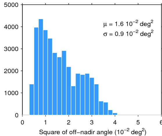
Figure 39. Histogram of flag-valid mispointing over oceans and lakes for 12/04/2016. The mean ( \mu ) and standard deviation ( \sigma ) are also shown. Note that values larger than 6 \cdot 10^{-2} \text{ deg}^2 are excluded from the histogram for the sake of readability but not from the computation of \mu and \sigma .
