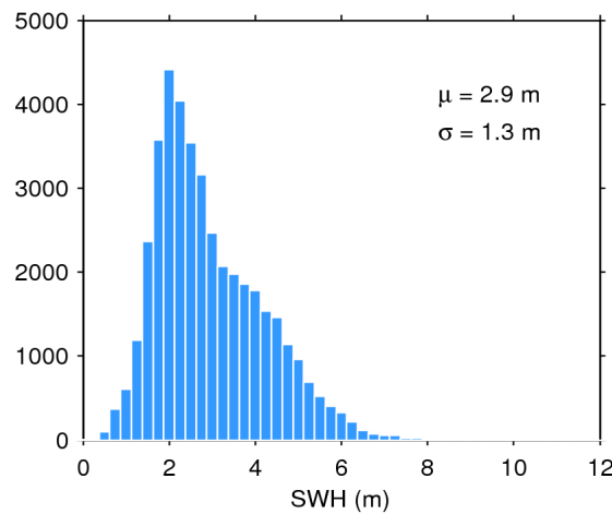
Figure 17. Histogram of flag-valid SWH over oceans and lakes for 12/04/2016. The mean ( \mu ) and standard deviation ( \sigma ) are also shown. Note that values larger than 12 m are excluded from the histogram for the sake of readability but not from the computation of \mu and \sigma .
