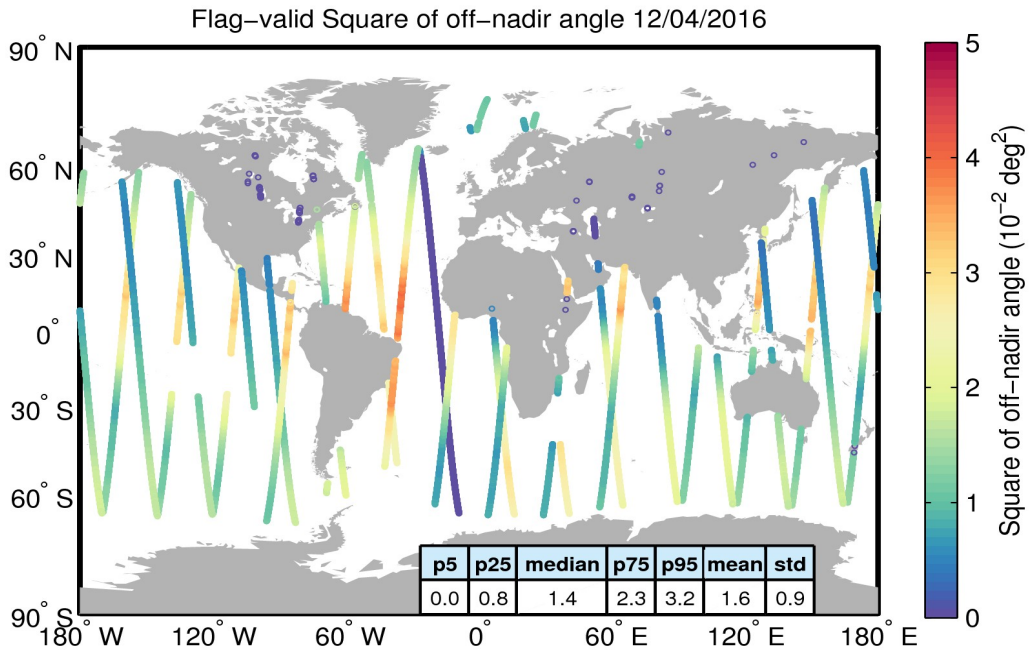
Figure 37. Geographical distribution of flag-valid mispointing data over oceans and lakes for 12/04/2016. The statistical values shown in the table refer to the mispointing in 10^{-2} deg 2 and are calculated over all measurements shown in the figure.
