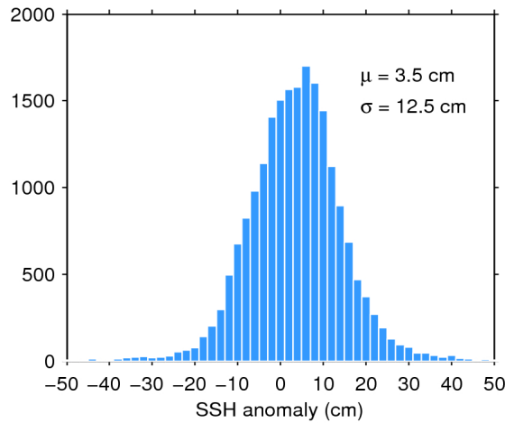
Figure 11. Histogram of science-valid SSH anomaly over oceans and lakes for 12/04/2016. The mean ( \mu ) and standard deviation ( \sigma ) are also shown. Note that values outside [-50 50] cm are excluded from the histogram for the sake of readability but not from the computation of \mu and \sigma .
