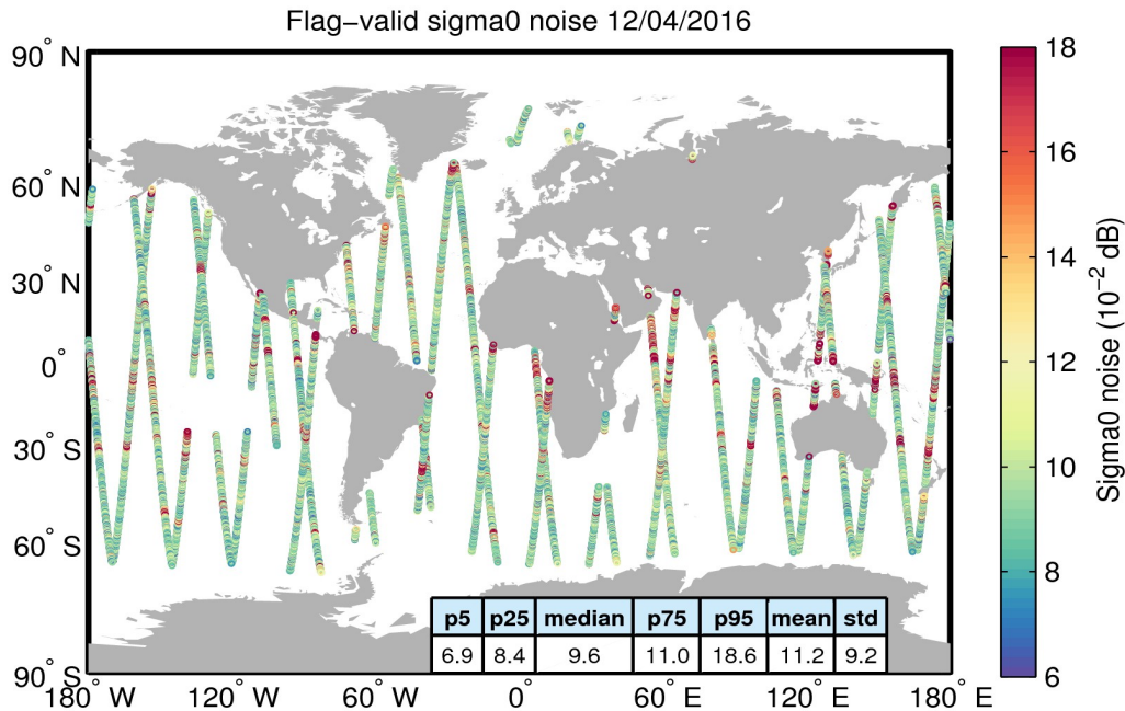
Figure 26. Geographical distribution of flag-valid 20-Hz sigma0 measurement noise over oceans and lakes for 12/04/2016. The statistical values shown in the table refer to the sigma0 noise and are calculated over all measurements shown in the figure.
