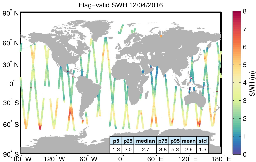
Figure 15. Geographical distribution of flag-valid SWH data over oceans and lakes for 12/04/2016. The statistical values shown in the table refer to the SWH in m and are calculated over all measurements shown in the figure.
