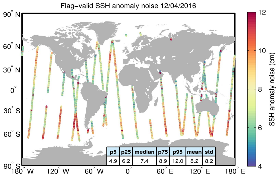
Figure 8. Geographical distribution of flag-valid 20-Hz SSH anomaly measurement noise over oceans and lakes for 12/04/2016. The statistical values shown in the table refer to the SSH anomaly noise and are calculated over all measurements shown in the figure.
