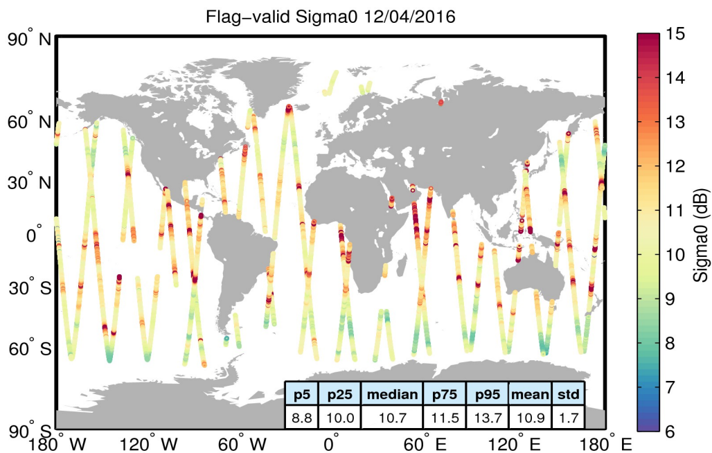
Figure 23. Geographical distribution of flag-valid sigma0 data over oceans and lakes for 12/04/2016. The statistical values shown in the table refer to the sigma0 in dB and are calculated over all measurements shown in the figure.
