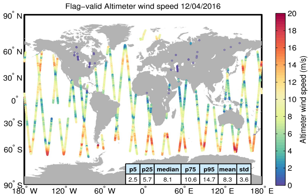
Figure 31. Geographical distribution of flag-valid wind data over oceans and lakes for 12/04/2016. The statistical values shown in the table refer to the wind in m/s and are calculated over all measurements shown in the figure.
