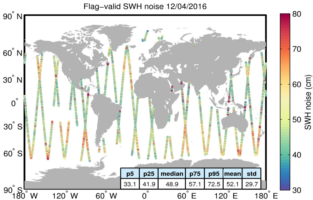
Figure 18. Geographical distribution of flag-valid 20-Hz SWH measurement noise over oceans and lakes for 12/04/2016. The statistical values shown in the table refer to the SWH noise and are calculated over all measurements shown in the figure.
