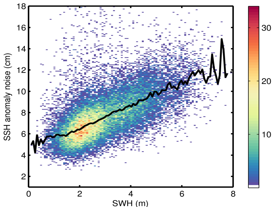
Figure 9. 2D histogram showing flag-valid SSH anomaly noise as a function of SWH for 12/04/2016. The black line denotes the median SSH anomaly noise as a function of SWH.
