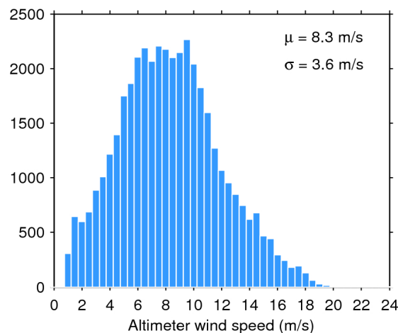
Figure 35. Histogram of science-valid wind over oceans and lakes for 12/04/2016. The mean ( \mu ) and standard deviation ( \sigma ) are also shown. Note that values larger than 24 m/s are excluded from the histogram for the sake of readability but not from the computation of \mu and \sigma .
