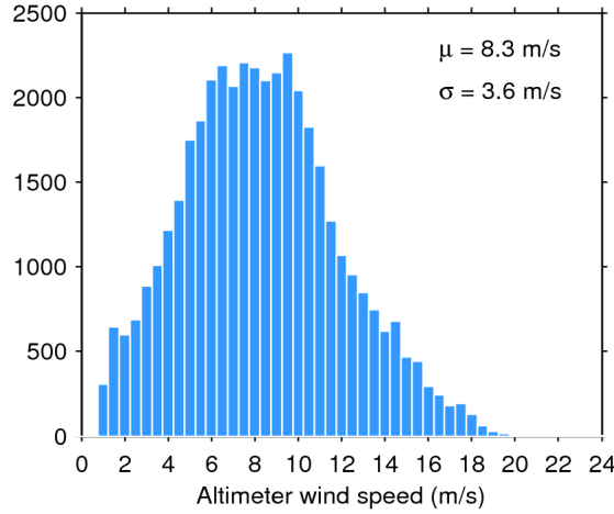
Figure 33. Histogram of flag-valid wind over oceans and lakes for 12/04/2016. The mean ( \mu ) and standard deviation ( \sigma ) are also shown. Note that values larger than 24 m/s are excluded from the histogram for the sake of readability but not from the computation of \mu and \sigma .
