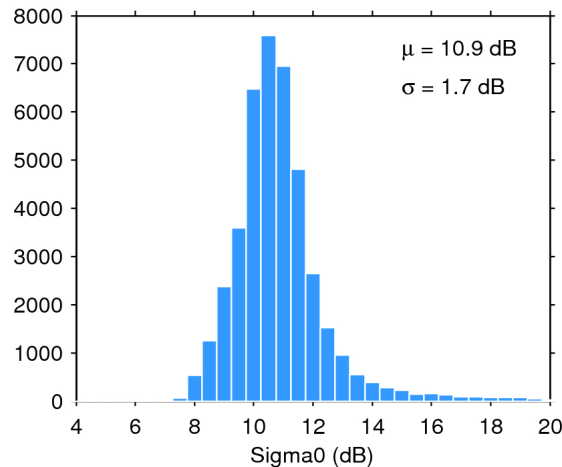
Figure 25. Histogram of flag-valid sigma0 over oceans and lakes for 12/04/2016. The mean ( \mu ) and standard deviation ( \sigma ) are also shown. Note that values outside [4 20] dB are excluded from the histogram for the sake of readability but not from the computation of \mu and \sigma .
