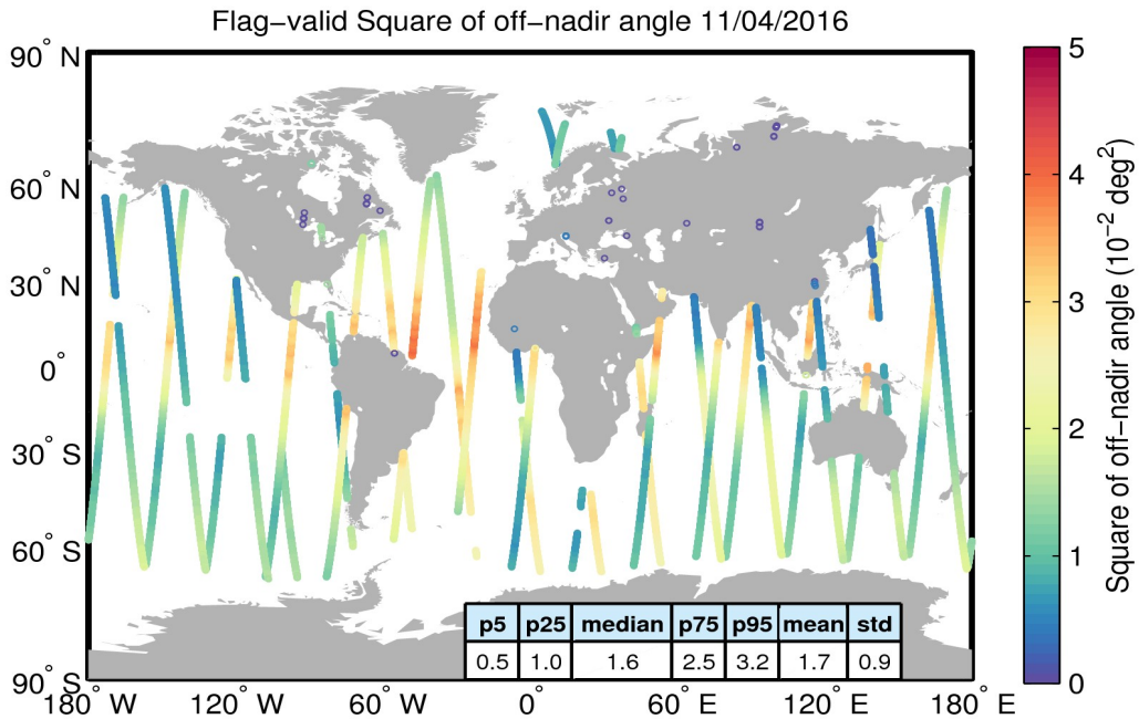
Figure 37. Geographical distribution of flag-valid mispointing data over oceans and lakes for 11/04/2016. The statistical values shown in the table refer to the mispointing in 10^{-2} \text{ deg}^2 and are calculated over all measurements shown in the figure.
