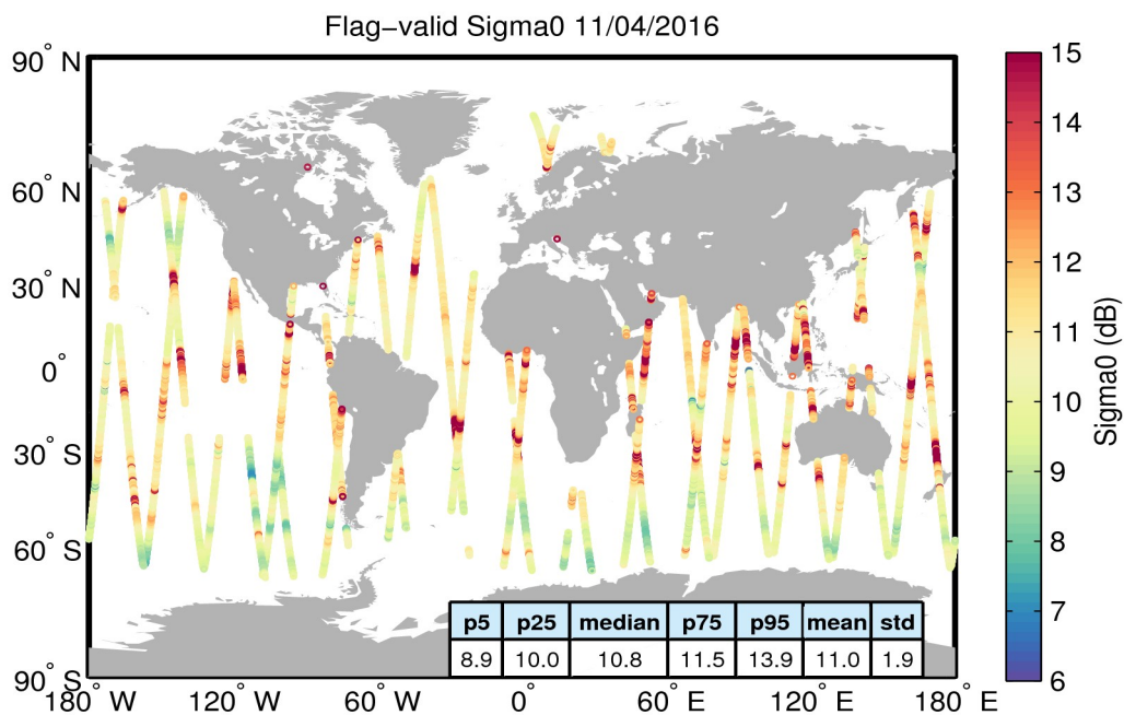
Figure 23. Geographical distribution of flag-valid sigma0 data over oceans and lakes for 11/04/2016. The statistical values shown in the table refer to the sigma0 in dB and are calculated over all measurements shown in the figure.
