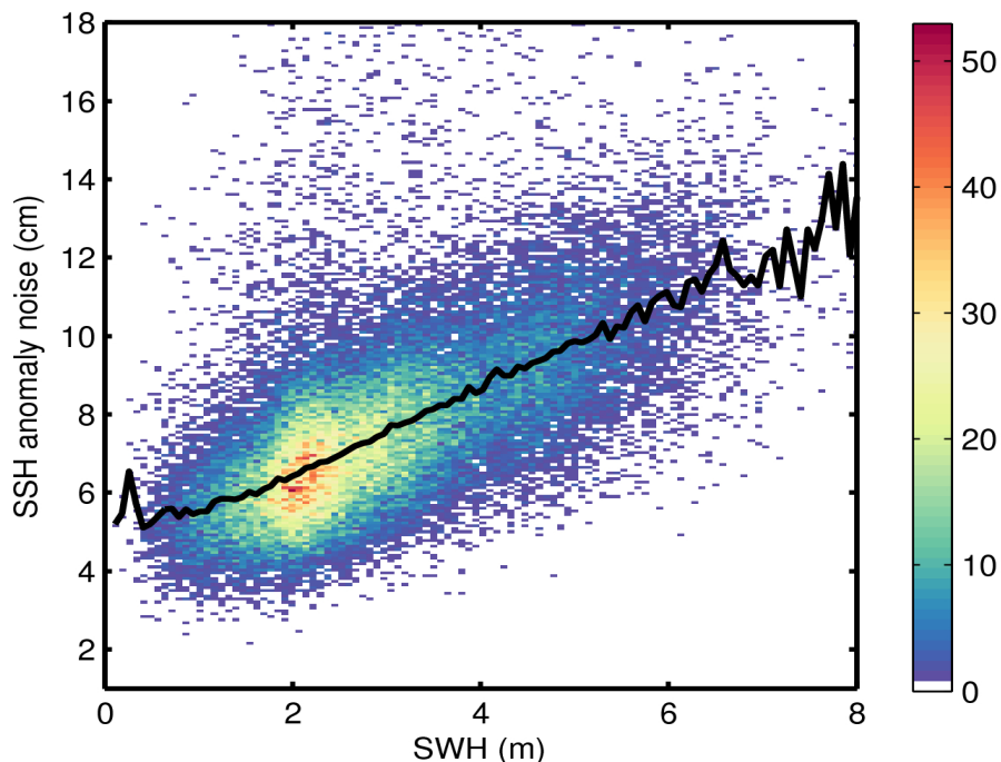
Figure 9. 2D histogram showing flag-valid SSH anomaly noise as a function of SWH for 11/04/2016. The black line denotes the median SSH anomaly noise as a function of SWH.
