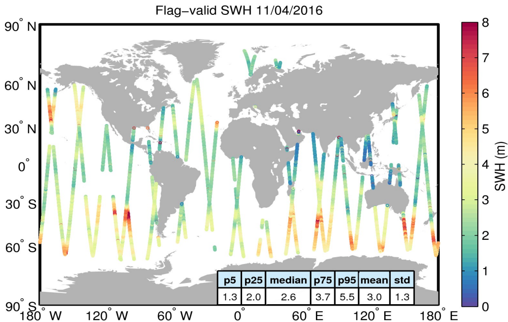
Figure 15. Geographical distribution of flag-valid SWH data over oceans and lakes for 11/04/2016. The statistical values shown in the table refer to the SWH in m and are calculated over all measurements shown in the figure.
