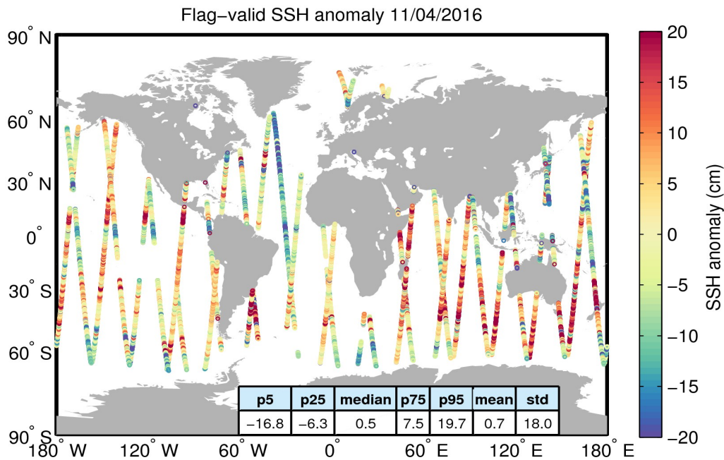
Figure 5. Geographical distribution of flag-valid 1-Hz SSH anomaly data over oceans and lakes for 11/04/2016. The statistical values shown in the table refer to the SSH anomaly in cm and are calculated over all measurements shown in the figure.
