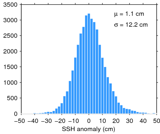
Figure 11. Histogram of science-valid SSH anomaly over oceans and lakes for 11/04/2016. The mean ( \mu ) and standard deviation ( \sigma ) are also shown. Note that values outside [-50 50] cm are excluded from the histogram for the sake of readability but not from the computation of \mu and \sigma .
