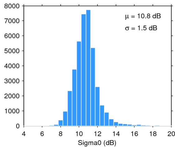
Figure 28. Histogram of science-valid sigma0 over oceans and lakes for 11/04/2016. The mean ( \mu ) and standard deviation ( \sigma ) are also shown. Note that values outside [4 20] dB are excluded from the histogram for the sake of readability but not from the computation of \mu and \sigma .
