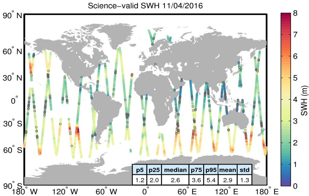
Figure 19. Geographical distribution of science-valid SWH data over oceans and lakes for 11/04/2016. The statistical values shown in the table refer to the SWH in m and are calculated over all measurements shown in the figure. Gray circles denote records that have been rejected based on the editing criteria described in Table 3.
