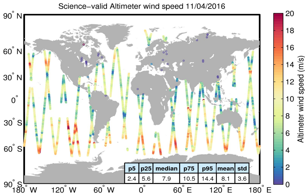
Figure 34. Geographical distribution of science-valid wind data over oceans and lakes for 11/04/2016. The statistical values shown in the table refer to the wind in m/s and are calculated over all measurements shown in the figure. Gray circles denote records that have been rejected based on the editing criteria described in Table 5.
