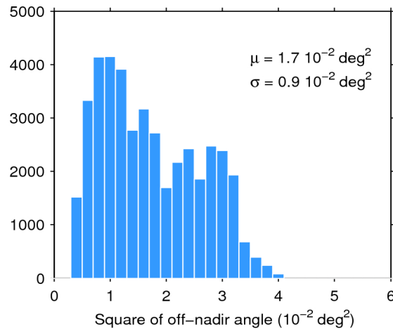
Figure 39. Histogram of flag-valid mispointing over oceans and lakes for 11/04/2016. The mean ( \mu ) and standard deviation ( \sigma ) are also shown. Note that values larger than 6 \cdot 10^{-2} \text{ deg}^2 are excluded from the histogram for the sake of readability but not from the computation of \mu and \sigma .
