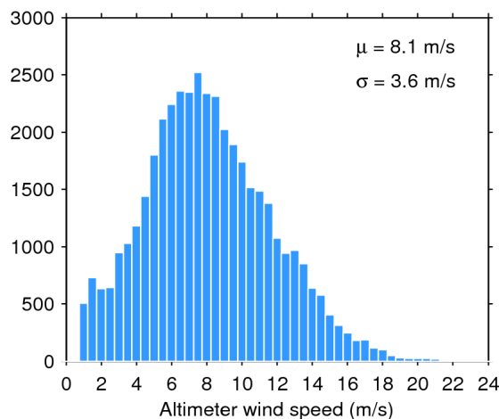
Figure 35. Histogram of science-valid wind over oceans and lakes for 11/04/2016. The mean ( \mu ) and standard deviation ( \sigma ) are also shown. Note that values larger than 24 m/s are excluded from the histogram for the sake of readability but not from the computation of \mu and \sigma .
