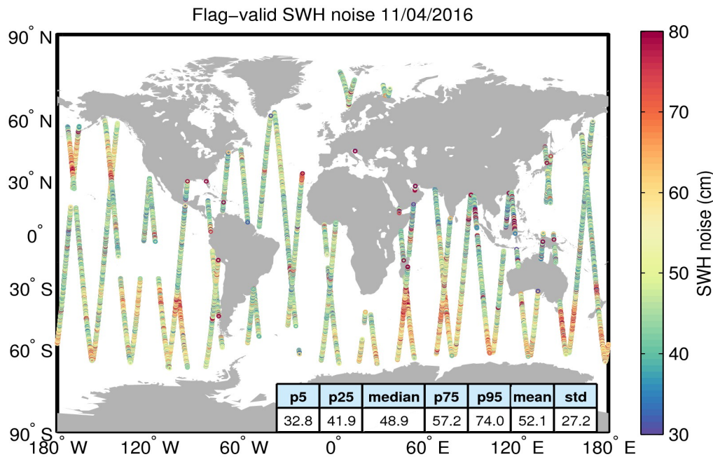
Figure 18. Geographical distribution of flag-valid 20-Hz SWH measurement noise over oceans and lakes for 11/04/2016. The statistical values shown in the figure refer to the SWH noise and are calculated over all measurements shown in the figure.
