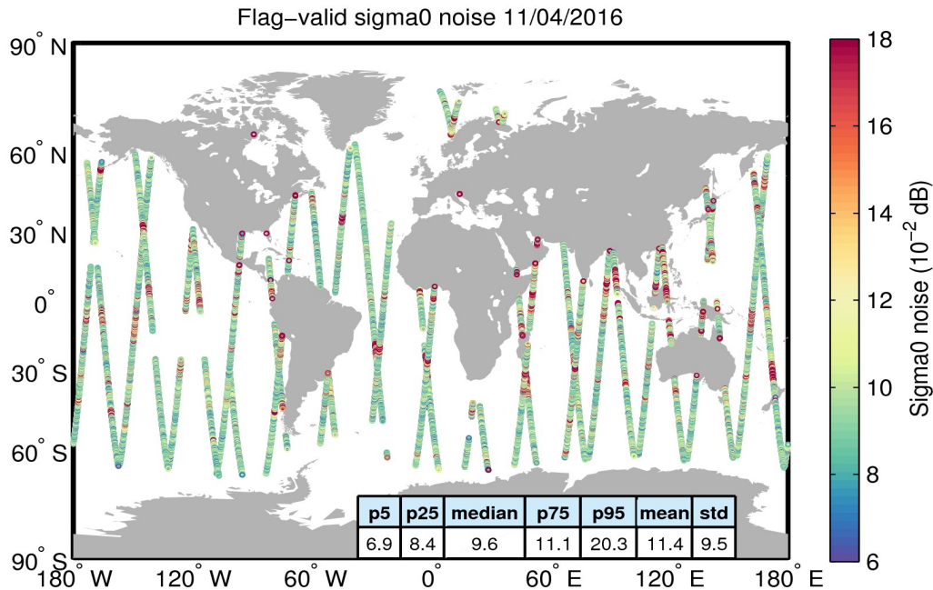
Figure 26. Geographical distribution of flag-valid 20-Hz sigma0 measurement noise over oceans and lakes for 11/04/2016. The statistical values shown in the table refer to the sigma0 noise and are calculated over all measurements shown in the figure.
