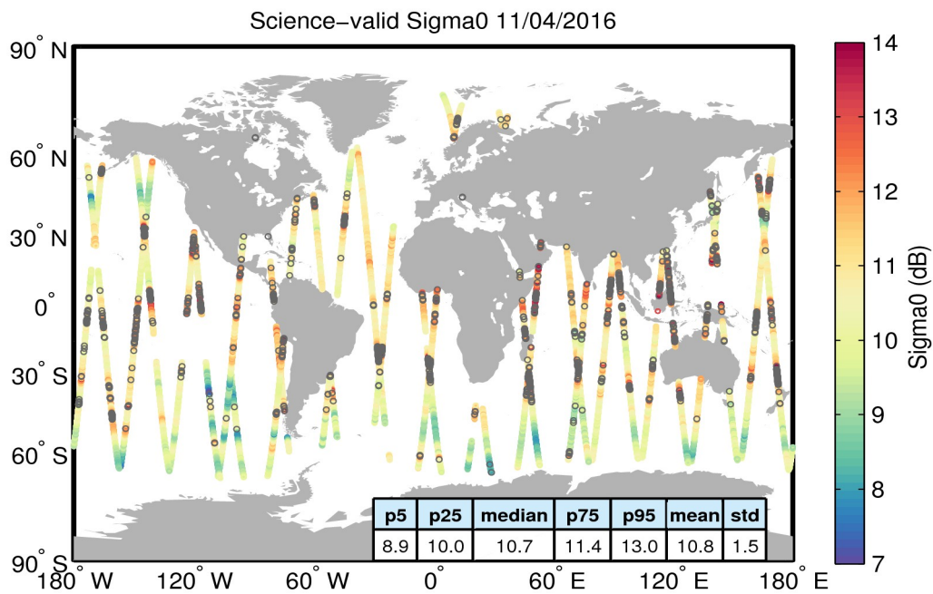
Figure 27. Geographical distribution of science-valid sigma0 data over oceans and lakes for 11/04/2016. The statistical values shown in the table refer to the sigma0 in dB and are calculated over all measurements shown in the figure. Gray circles denote records that have been rejected based on the editing criteria described in Table 4.
