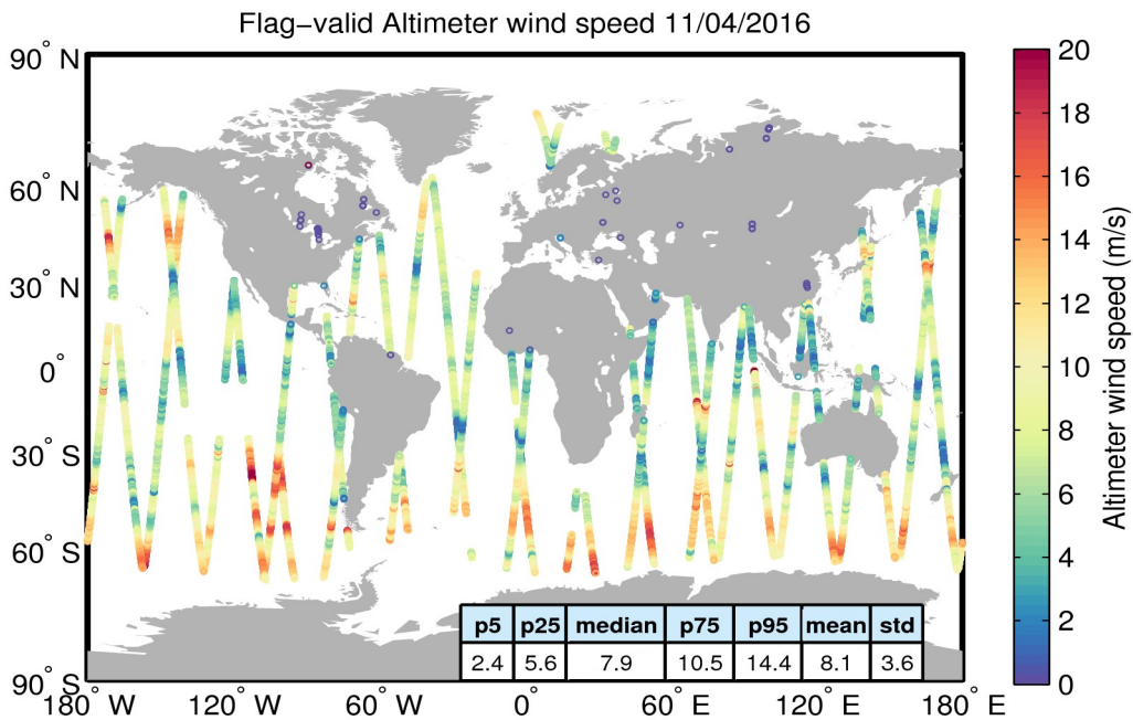
Figure 31. Geographical distribution of flag-valid wind data over oceans and lakes for 11/04/2016. The statistical values shown in the table refer to the wind in m/s and are calculated over all measurements shown in the figure.
