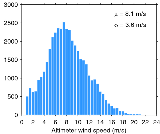
Figure 33. Histogram of flag-valid wind over oceans and lakes for 11/04/2016. The mean ( \mu ) and standard deviation ( \sigma ) are also shown. Note that values larger than 24 m/s are excluded from the histogram for the sake of readability but not from the computation of \mu and \sigma .
