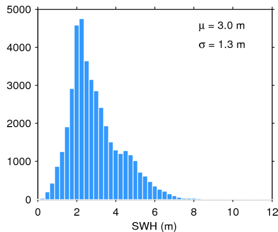
Figure 17. Histogram of flag-valid SWH over oceans and lakes for 11/04/2016. The mean ( \mu ) and standard deviation ( \sigma ) are also shown. Note that values larger than 12 m are excluded from the histogram for the sake of readability but not from the computation of \mu and \sigma .
