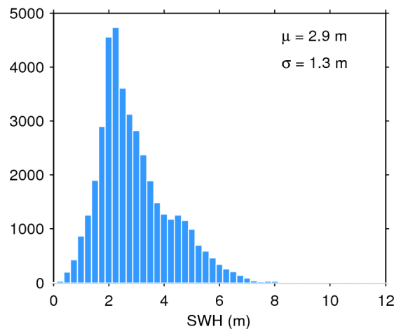
Figure 20. Histogram of science-valid SWH over oceans and lakes for 11/04/2016. The mean ( \mu ) and standard deviation ( \sigma ) are also shown. Note that values larger than 12 m are excluded from the histogram for the sake of readability but not from the computation of \mu and \sigma .
