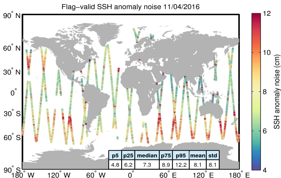
Figure 8. Geographical distribution of flag-valid 20-Hz SSH anomaly measurement noise over oceans and lakes for 11/04/2016. The statistical values shown in the table refer to the SSH anomaly noise and are calculated over all measurements shown in the figure.
