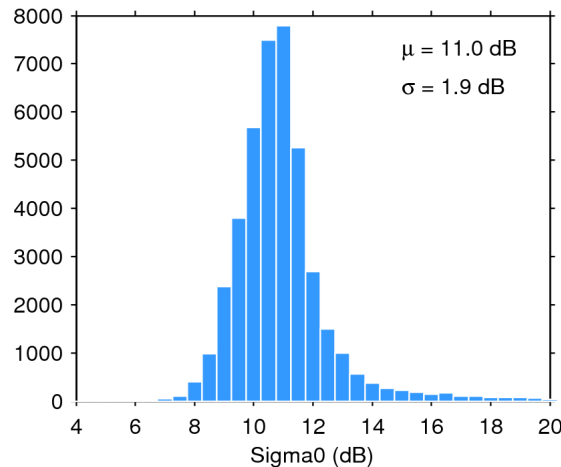
Figure 25. Histogram of flag-valid sigma0 over oceans and lakes for 11/04/2016. The mean ( \mu ) and standard deviation ( \sigma ) are also shown. Note that values outside [4 20] dB are excluded from the histogram for the sake of readability but not from the computation of \mu and \sigma .
