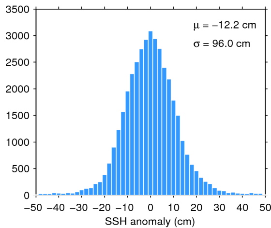
Figure 7. Histogram of flag-valid SSH anomaly over oceans and lakes for 10/04/2016. The mean ( \mu ) and standard deviation ( \sigma ) are also shown. Note that values outside [-50\ 50] cm are excluded from the histogram for the sake of readability but not from the computation of \mu and \sigma .
