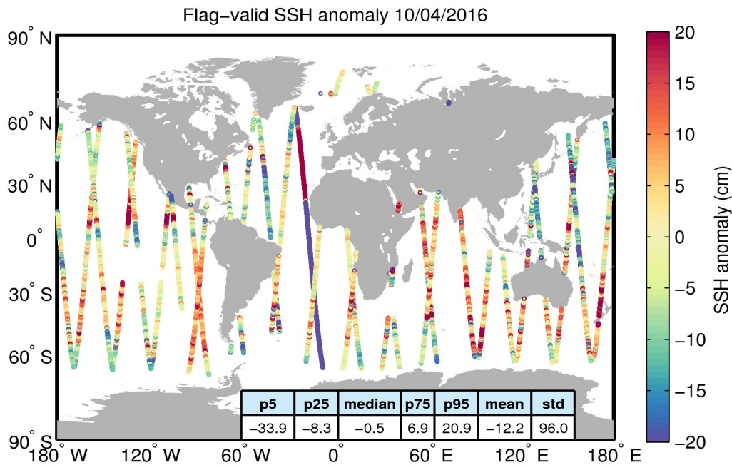
Figure 5. Geographical distribution of flag-valid 1-Hz SSH anomaly data over oceans and lakes for 10/04/2016. The statistical values shown in the table refer to the SSH anomaly in cm and are calculated over all measurements shown in the figure.
