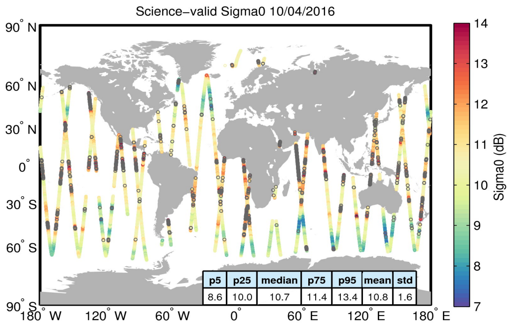
Figure 27. Geographical distribution of science-valid sigma0 data over oceans and lakes for 10/04/2016. The statistical values shown in the table refer to the sigma0 in dB and are calculated over all measurements shown in the figure. Gray circles denote records that have been rejected based on the editing criteria described in Table 4.
