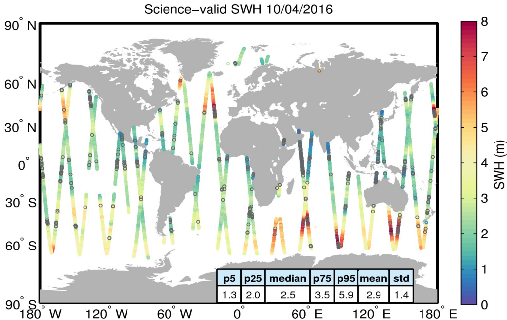
Figure 19. Geographical distribution of science-valid SWH data over oceans and lakes for 10/04/2016. The statistical values shown in the table refer to the SWH in m and are calculated over all measurements shown in the figure. Gray circles denote records that have been rejected based on the editing criteria described in Table 3.
