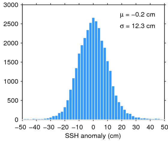
Figure 11. Histogram of science-valid SSH anomaly over oceans and lakes for 10/04/2016. The mean ( \mu ) and standard deviation ( \sigma ) are also shown. Note that values outside [-50 50] cm are excluded from the histogram for the sake of readability but not from the computation of \mu and \sigma .
