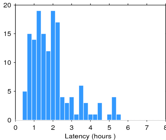
Figure 2. Histogram of the data latency for 10/04/2016. The y-axis denotes the number of files that are made available with a delay of x-hours with respect to the mean time of the records stored in the file.
