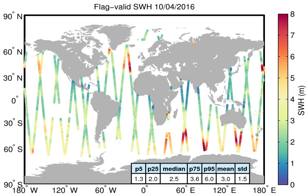
Figure 15. Geographical distribution of flag-valid SWH data over oceans and lakes for 10/04/2016. The statistical values shown in the table refer to the SWH in m and are calculated over all measurements shown in the figure.
