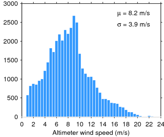
Figure 33. Histogram of flag-valid wind over oceans and lakes for 10/04/2016. The mean ( \mu ) and standard deviation ( \sigma ) are also shown. Note that values larger than 24 m/s are excluded from the histogram for the sake of readability but not from the computation of \mu and \sigma .
