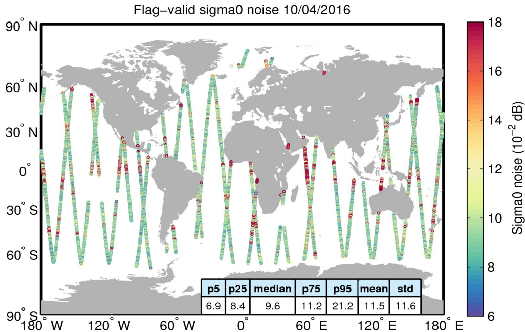
Figure 26. Geographical distribution of flag-valid 20-Hz sigma0 measurement noise over oceans and lakes for 10/04/2016. The statistical values shown in the table refer to the sigma0 noise and are calculated over all measurements shown in the figure.
