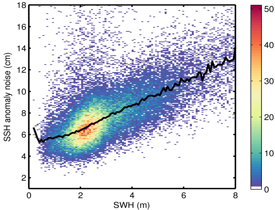
Figure 9. 2D histogram showing flag-valid SSH anomaly noise as a function of SWH for 10/04/2016. The black line denotes the median SSH anomaly noise as a function of SWH.
