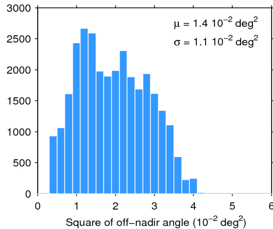
Figure 39. Histogram of flag-valid mispointing over oceans and lakes for 09/04/2016. The mean ( \mu ) and standard deviation ( \sigma ) are also shown. Note that values larger than 6 \cdot 10^{-2} \text{ deg}^2 are excluded from the histogram for the sake of readability but not from the computation of \mu and \sigma .
