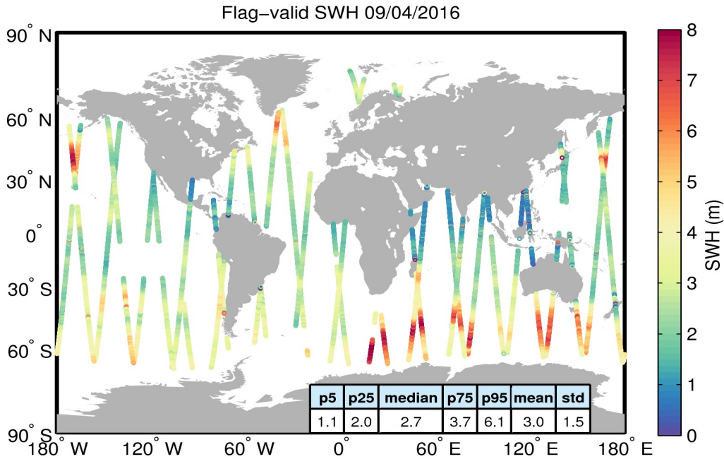
Figure 15. Geographical distribution of flag-valid SWH data over oceans and lakes for 09/04/2016. The statistical values shown in the table refer to the SWH in m and are calculated over all measurements shown in the figure.
