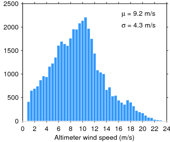
Figure 33. Histogram of flag-valid wind over oceans and lakes for 09/04/2016. The mean ( \mu ) and standard deviation ( \sigma ) are also shown. Note that values larger than 24 m/s are excluded from the histogram for the sake of readability but not from the computation of \mu and \sigma .
