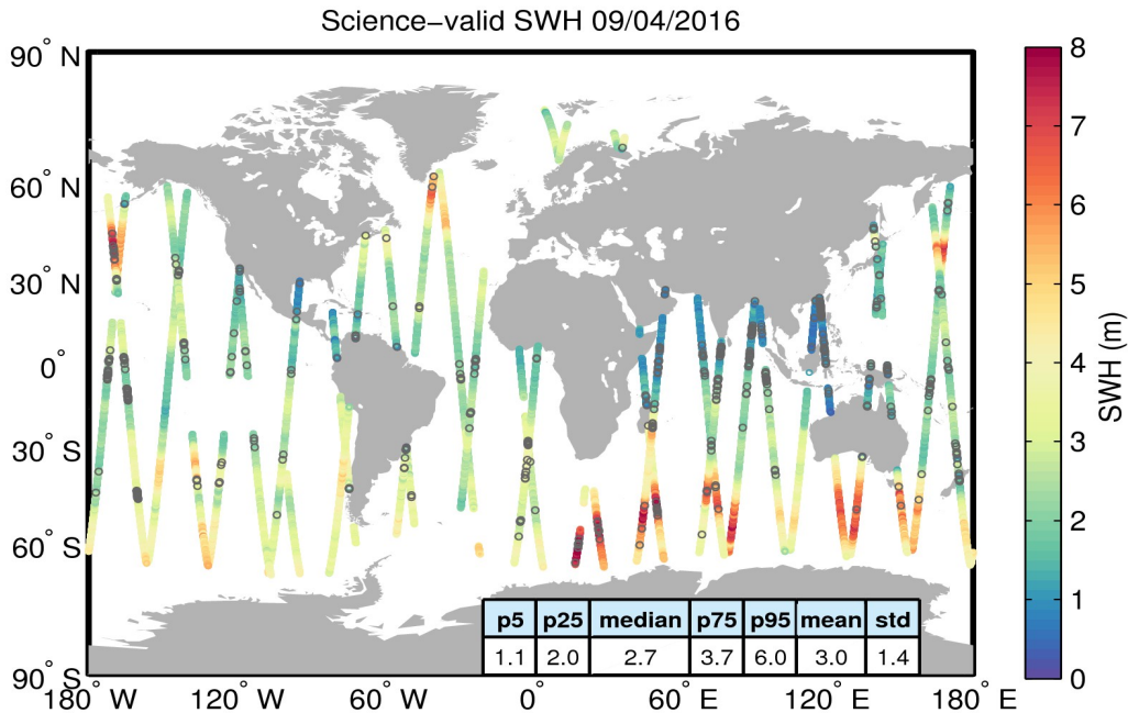
Figure 19. Geographical distribution of science-valid SWH data over oceans and lakes for 09/04/2016. The statistical values shown in the table refer to the SWH in m and are calculated over all measurements shown in the figure. Gray circles denote records that have been rejected based on the editing criteria described in Table 3.
