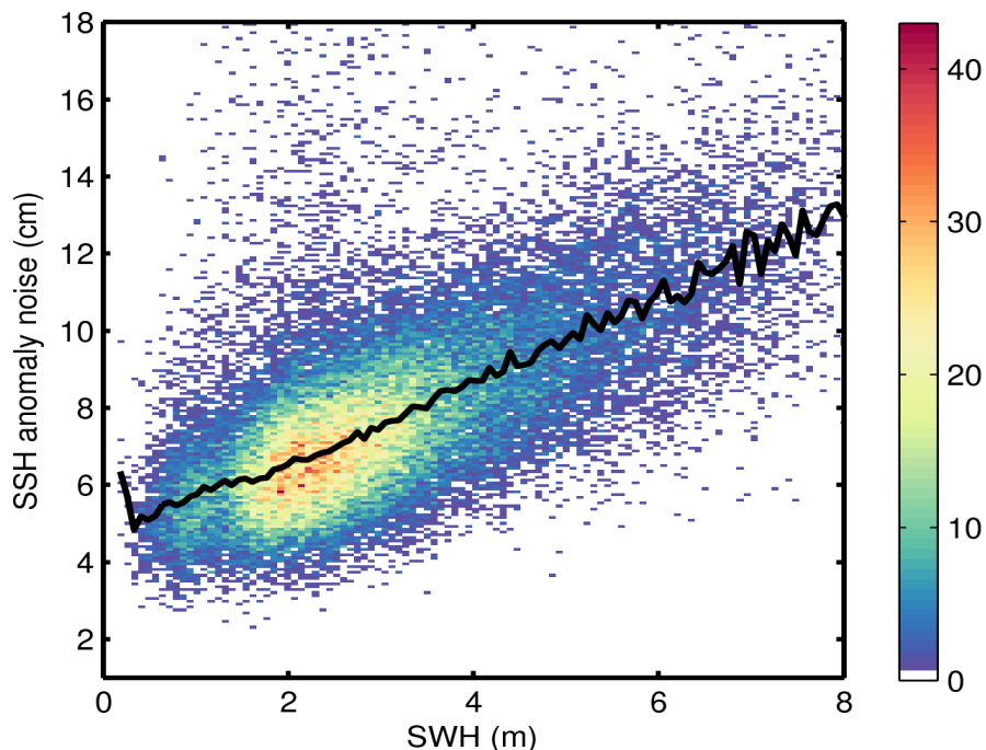
Figure 9. 2D histogram showing flag-valid SSH anomaly noise as a function of SWH for 09/04/2016. The black line denotes the median SSH anomaly noise as a function of SWH.
