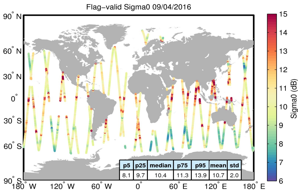
Figure 23. Geographical distribution of flag-valid sigma0 data over oceans and lakes for 09/04/2016. The statistical values shown in the table refer to the sigma0 in dB and are calculated over all measurements shown in the figure.
