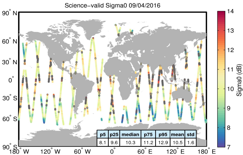
Figure 27. Geographical distribution of science-valid sigma0 data over oceans and lakes for 09/04/2016. The statistical values shown in the table refer to the sigma0 in dB and are calculated over all measurements shown in the figure. Gray circles denote records that have been rejected based on the editing criteria described in Table 4.
