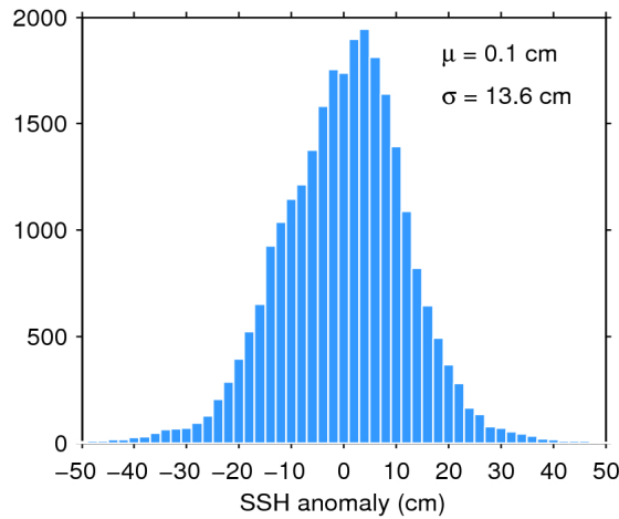
Figure 11. Histogram of science-valid SSH anomaly over oceans and lakes for 09/04/2016. The mean ( \mu ) and standard deviation ( \sigma ) are also shown. Note that values outside [-50 50] cm are excluded from the histogram for the sake of readability but not from the computation of \mu and \sigma .
