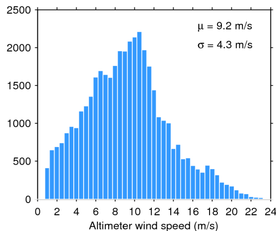
Figure 35. Histogram of science-valid wind over oceans and lakes for 09/04/2016. The mean ( \mu ) and standard deviation ( \sigma ) are also shown. Note that values larger than 24 m/s are excluded from the histogram for the sake of readability but not from the computation of \mu and \sigma .
