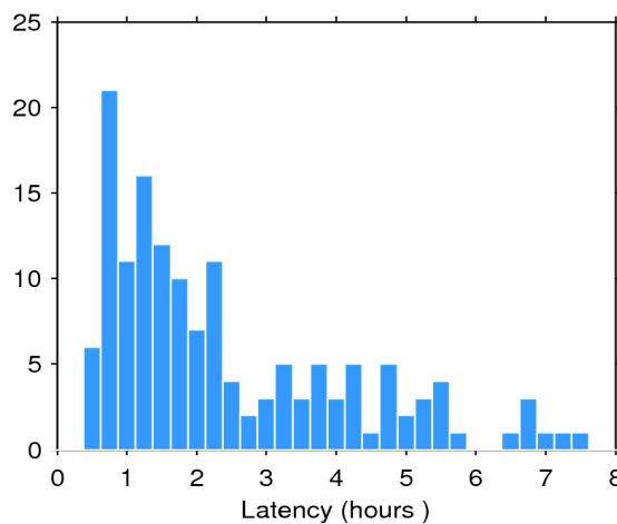
Figure 2. Histogram of the data latency for 09/04/2016. The y-axis denotes the number of files that are made available with a delay of x-hours with respect to the mean time of the records stored in the file.
