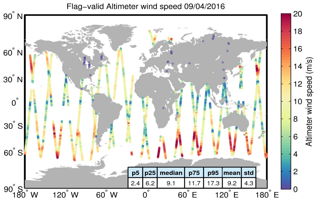
Figure 31. Geographical distribution of flag-valid wind data over oceans and lakes for 09/04/2016. The statistical values shown in the table refer to the wind in m/s and are calculated over all measurements shown in the figure.
