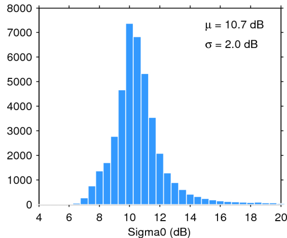
Figure 25. Histogram of flag-valid sigma0 over oceans and lakes for 09/04/2016. The mean ( \mu ) and standard deviation ( \sigma ) are also shown. Note that values outside [4 20] dB are excluded from the histogram for the sake of readability but not from the computation of \mu and \sigma .
