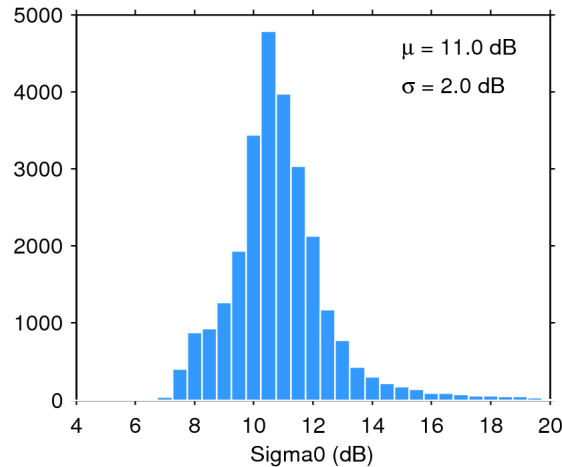
Figure 25. Histogram of flag-valid sigma0 over oceans and lakes for 08/04/2016. The mean ( \mu ) and standard deviation ( \sigma ) are also shown. Note that values outside [4 20] dB are excluded from the histogram for the sake of readability but not from the computation of \mu and \sigma .
