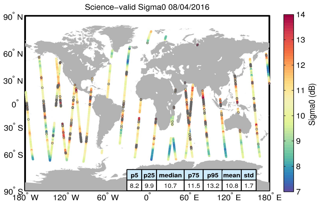
Figure 27. Geographical distribution of science-valid sigma0 data over oceans and lakes for 08/04/2016. The statistical values shown in the table refer to the sigma0 in dB and are calculated over all measurements shown in the figure. Gray circles denote records that have been rejected based on the editing criteria described in Table 4.
