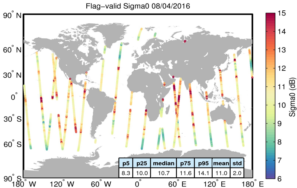
Figure 23. Geographical distribution of flag-valid sigma0 data over oceans and lakes for 08/04/2016. The statistical values shown in the table refer to the sigma0 in dB and are calculated over all measurements shown in the figure.
