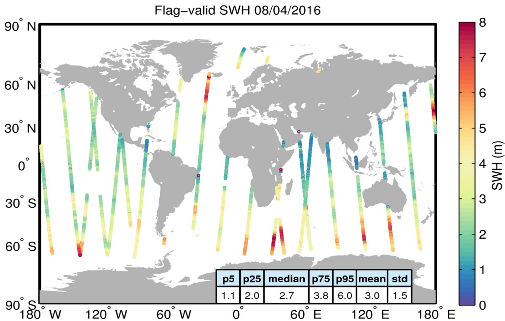
Figure 15. Geographical distribution of flag-valid SWH data over oceans and lakes for 08/04/2016. The statistical values shown in the table refer to the SWH in m and are calculated over all measurements shown in the figure.
