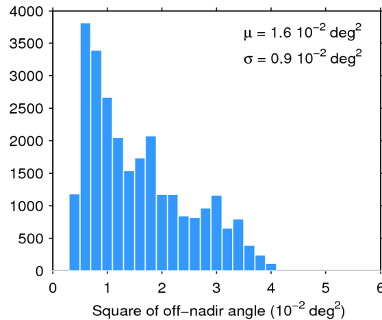
Figure 39. Histogram of flag-valid mispointing over oceans and lakes for 08/04/2016. The mean ( \mu ) and standard deviation ( \sigma ) are also shown. Note that values larger than 6 \cdot 10^{-2} \text{ deg}^2 are excluded from the histogram for the sake of readability but not from the computation of \mu and \sigma .
