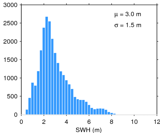
Figure 20. Histogram of science-valid SWH over oceans and lakes for 08/04/2016. The mean ( \mu ) and standard deviation ( \sigma ) are also shown. Note that values larger than 12 m are excluded from the histogram for the sake of readability but not from the computation of \mu and \sigma .
