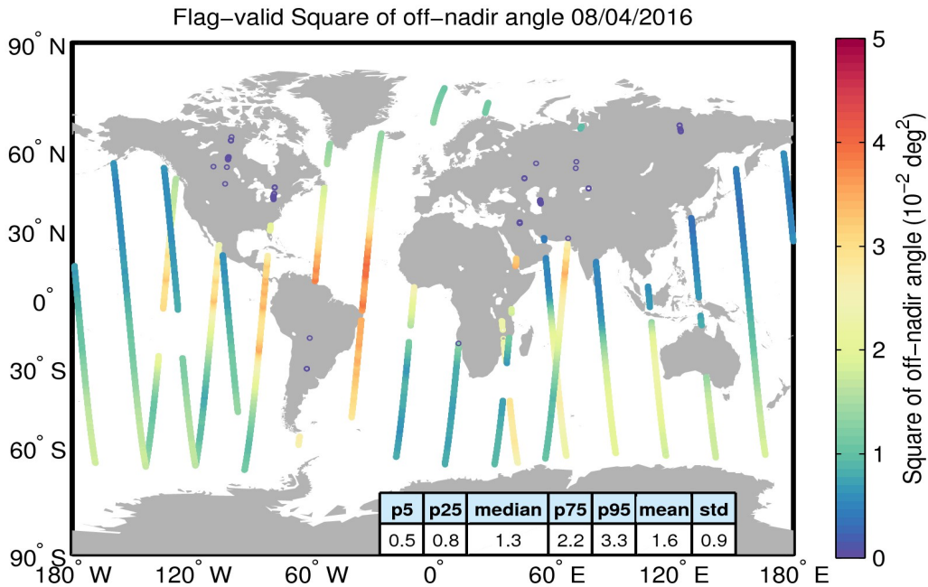
Figure 37. Geographical distribution of flag-valid mispointing data over oceans and lakes for 08/04/2016. The statistical values shown in the table refer to the mispointing in 10^{-2} \text{ deg}^2 and are calculated over all measurements shown in the figure.
