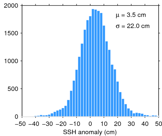
Figure 7. Histogram of flag-valid SSH anomaly over oceans and lakes for 08/04/2016. The mean ( \mu ) and standard deviation ( \sigma ) are also shown. Note that values outside [-50\ 50] cm are excluded from the histogram for the sake of readability but not from the computation of \mu and \sigma .
