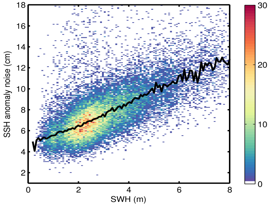
Figure 9. 2D histogram showing flag-valid SSH anomaly noise as a function of SWH for 08/04/2016. The black line denotes the median SSH anomaly noise as a function of SWH.
