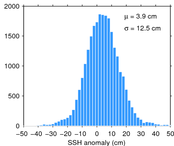
Figure 11. Histogram of science-valid SSH anomaly over oceans and lakes for 08/04/2016. The mean ( \mu ) and standard deviation ( \sigma ) are also shown. Note that values outside [-50 50] cm are excluded from the histogram for the sake of readability but not from the computation of \mu and \sigma .
