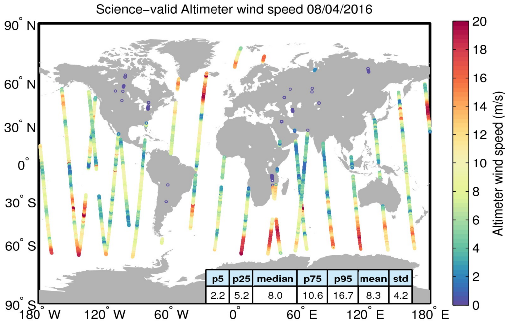
Figure 34. Geographical distribution of science-valid wind data over oceans and lakes for 08/04/2016. The statistical values shown in the table refer to the wind in m/s and are calculated over all measurements shown in the figure. Gray circles denote records that have been rejected based on the editing criteria described in Table 5.
