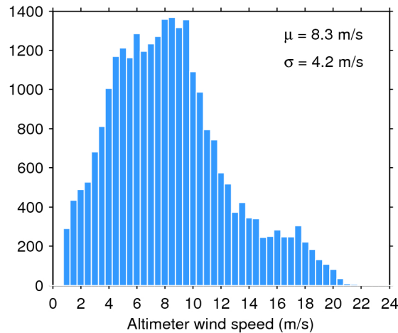
Figure 33. Histogram of flag-valid wind over oceans and lakes for 08/04/2016. The mean ( \mu ) and standard deviation ( \sigma ) are also shown. Note that values larger than 24 m/s are excluded from the histogram for the sake of readability but not from the computation of \mu and \sigma .
