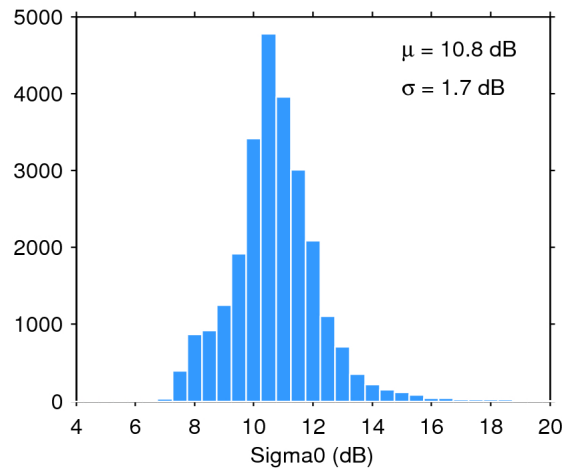
Figure 28. Histogram of science-valid sigma0 over oceans and lakes for 08/04/2016. The mean ( \mu ) and standard deviation ( \sigma ) are also shown. Note that values outside [4 20] dB are excluded from the histogram for the sake of readability but not from the computation of \mu and \sigma .
