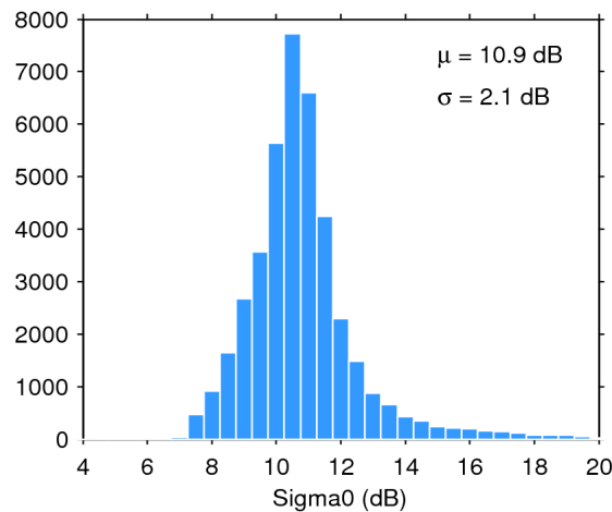
Figure 25. Histogram of flag-valid sigma0 over oceans and lakes for 07/04/2016. The mean ( \mu ) and standard deviation ( \sigma ) are also shown. Note that values outside [4 20] dB are excluded from the histogram for the sake of readability but not from the computation of \mu and \sigma .
