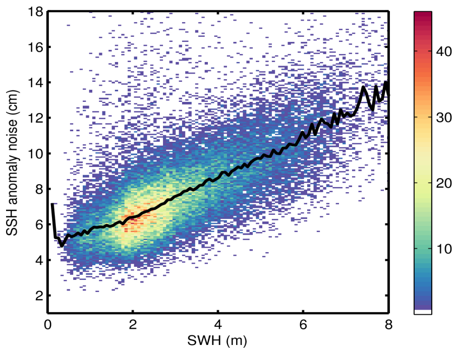
Figure 9. 2D histogram showing flag-valid SSH anomaly noise as a function of SWH for 07/04/2016. The black line denotes the median SSH anomaly noise as a function of SWH.
