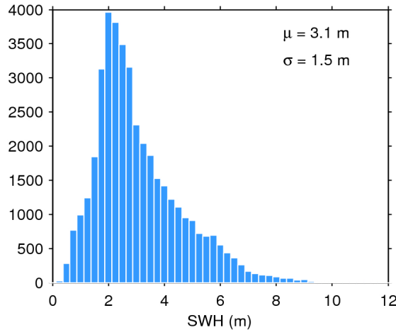
Figure 20. Histogram of science-valid SWH over oceans and lakes for 07/04/2016. The mean ( \mu ) and standard deviation ( \sigma ) are also shown. Note that values larger than 12 m are excluded from the histogram for the sake of readability but not from the computation of \mu and \sigma .
