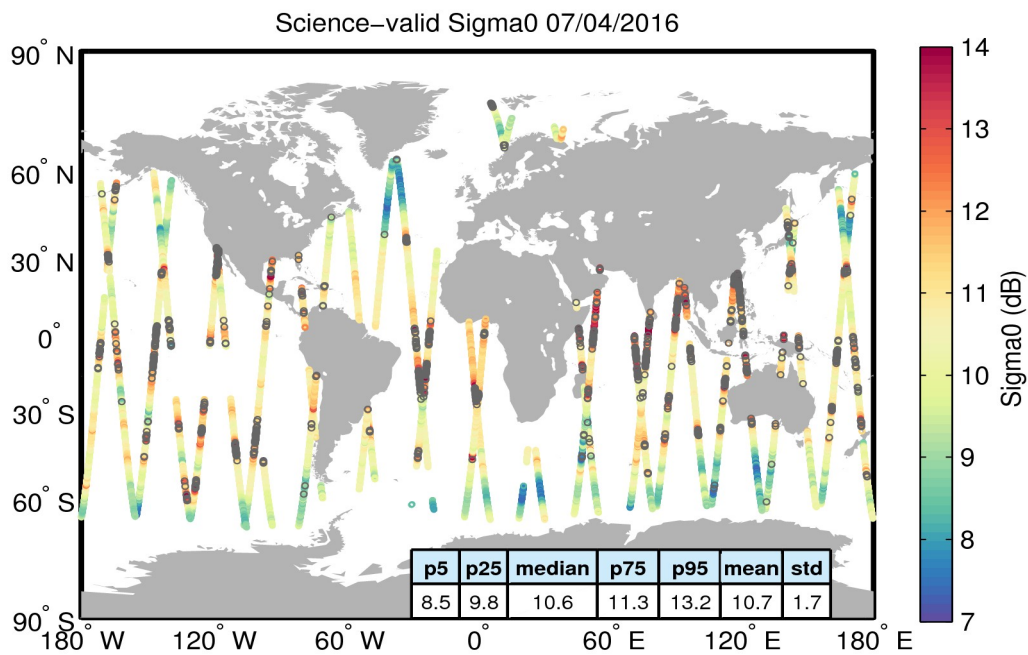
Figure 27. Geographical distribution of science-valid sigma0 data over oceans and lakes for 07/04/2016. The statistical values shown in the table refer to the sigma0 in dB and are calculated over all measurements shown in the figure. Gray circles denote records that have been rejected based on the editing criteria described in Table 4.
