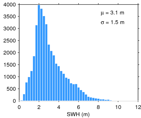
Figure 17. Histogram of flag-valid SWH over oceans and lakes for 07/04/2016. The mean ( \mu ) and standard deviation ( \sigma ) are also shown. Note that values larger than 12 m are excluded from the histogram for the sake of readability but not from the computation of \mu and \sigma .
