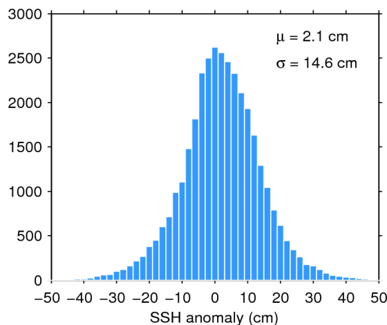
Figure 11. Histogram of science-valid SSH anomaly over oceans and lakes for 07/04/2016. The mean ( \mu ) and standard deviation ( \sigma ) are also shown. Note that values outside [-50 50] cm are excluded from the histogram for the sake of readability but not from the computation of \mu and \sigma .
