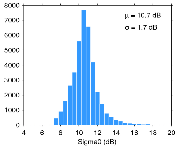
Figure 28. Histogram of science-valid sigma0 over oceans and lakes for 07/04/2016. The mean ( \mu ) and standard deviation ( \sigma ) are also shown. Note that values outside [4 20] dB are excluded from the histogram for the sake of readability but not from the computation of \mu and \sigma .
