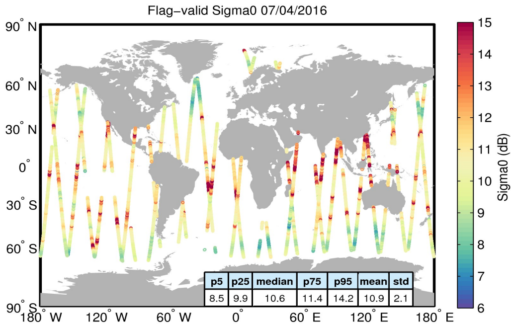
Figure 23. Geographical distribution of flag-valid sigma0 data over oceans and lakes for 07/04/2016. The statistical values shown in the table refer to the sigma0 in dB and are calculated over all measurements shown in the figure.
