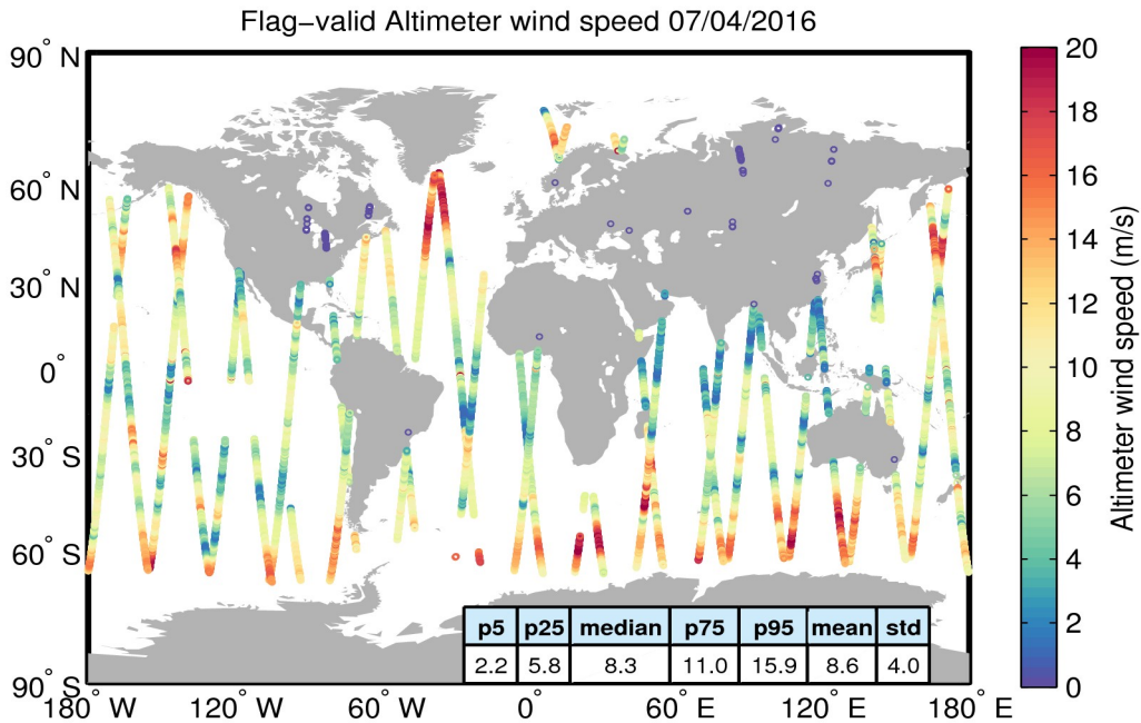
Figure 31. Geographical distribution of flag-valid wind data over oceans and lakes for 07/04/2016. The statistical values shown in the table refer to the wind in m/s and are calculated over all measurements shown in the figure.
