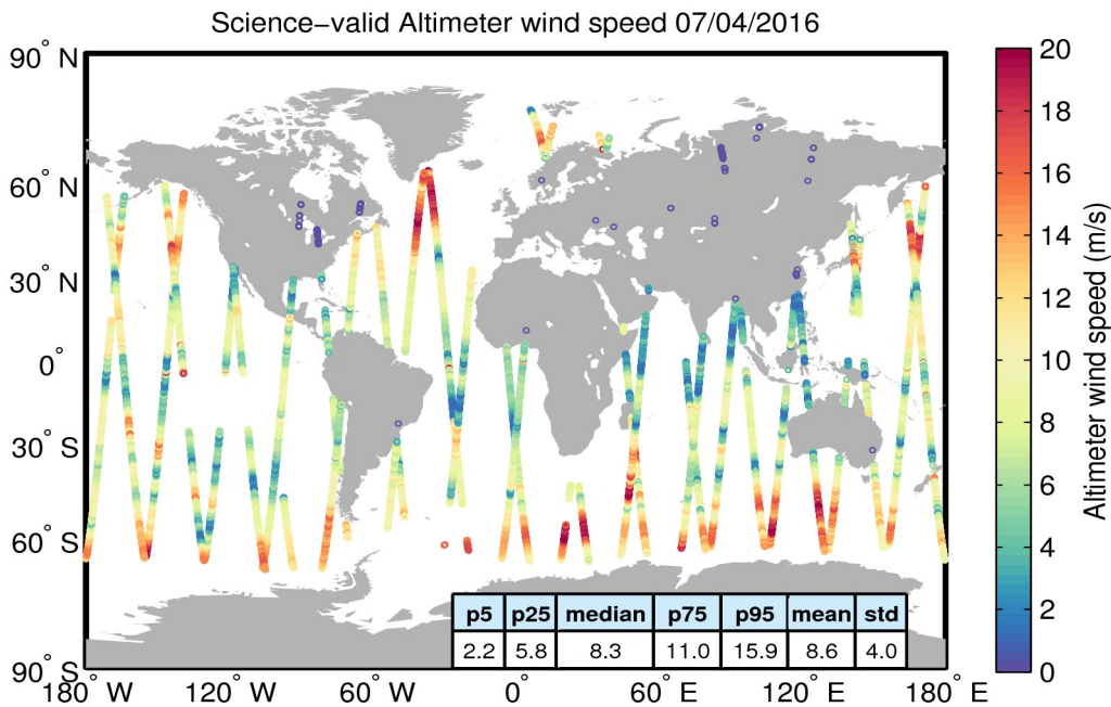
Figure 34. Geographical distribution of science-valid wind data over oceans and lakes for 07/04/2016. The statistical values shown in the table refer to the wind in m/s and are calculated over all measurements shown in the figure. Gray circles denote records that have been rejected based on the editing criteria described in Table 5.
