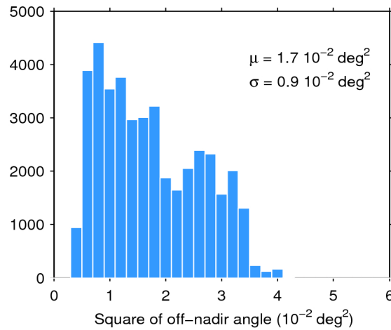
Figure 39. Histogram of flag-valid mispointing over oceans and lakes for 07/04/2016. The mean ( \mu ) and standard deviation ( \sigma ) are also shown. Note that values larger than 6 \cdot 10^{-2} \text{ deg}^2 are excluded from the histogram for the sake of readability but not from the computation of \mu and \sigma .
