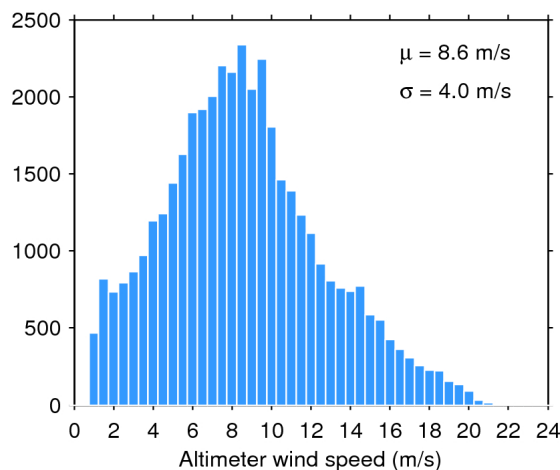
Figure 35. Histogram of science-valid wind over oceans and lakes for 07/04/2016. The mean ( \mu ) and standard deviation ( \sigma ) are also shown. Note that values larger than 24 m/s are excluded from the histogram for the sake of readability but not from the computation of \mu and \sigma .
