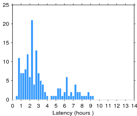
Figure 2. Histogram of the data latency for 07/04/2016. The y-axis denotes the number of files that are made available with a delay of x-hours with respect to the mean time of the records stored in the file.
