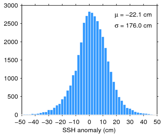
Figure 7. Histogram of flag-valid SSH anomaly over oceans and lakes for 07/04/2016. The mean ( \mu ) and standard deviation ( \sigma ) are also shown. Note that values outside [-50 50] cm are excluded from the histogram for the sake of readability but not from the computation of \mu and \sigma .
