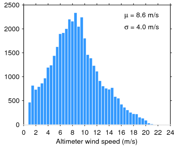
Figure 33. Histogram of flag-valid wind over oceans and lakes for 07/04/2016. The mean ( \mu ) and standard deviation ( \sigma ) are also shown. Note that values larger than 24 m/s are excluded from the histogram for the sake of readability but not from the computation of \mu and \sigma .
