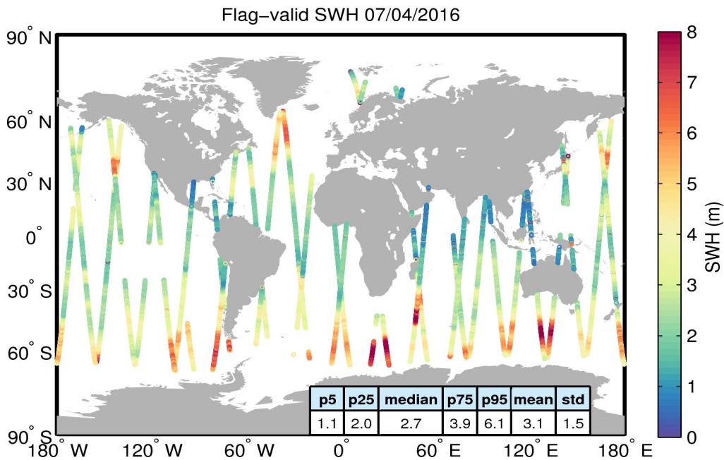
Figure 15. Geographical distribution of flag-valid SWH data over oceans and lakes for 07/04/2016. The statistical values shown in the table refer to the SWH in m and are calculated over all measurements shown in the figure.
