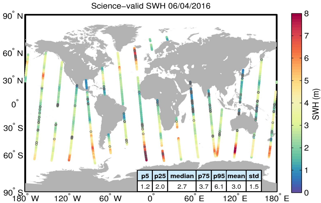
Figure 19. Geographical distribution of science-valid SWH data over oceans and lakes for 06/04/2016. The statistical values shown in the table refer to the SWH in m and are calculated over all measurements shown in the figure. Gray circles denote records that have been rejected based on the editing criteria described in Table 3.
