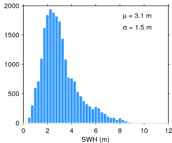
Figure 17. Histogram of flag-valid SWH over oceans and lakes for 06/04/2016. The mean ( \mu ) and standard deviation ( \sigma ) are also shown. Note that values larger than 12 m are excluded from the histogram for the sake of readability but not from the computation of \mu and \sigma .
