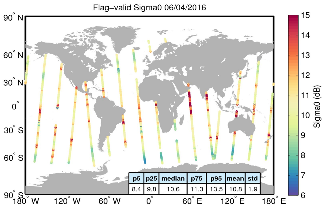
Figure 23. Geographical distribution of flag-valid sigma0 data over oceans and lakes for 06/04/2016. The statistical values shown in the table refer to the sigma0 in dB and are calculated over all measurements shown in the figure.
