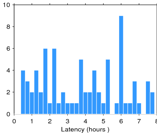
Figure 2. Histogram of the data latency for 06/04/2016. The y-axis denotes the number of files that are made available with a delay of x-hours with respect to the mean time of the records stored in the file.
