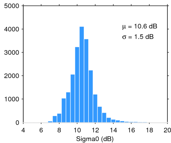
Figure 28. Histogram of science-valid sigma0 over oceans and lakes for 06/04/2016. The mean ( \mu ) and standard deviation ( \sigma ) are also shown. Note that values outside [4 20] dB are excluded from the histogram for the sake of readability but not from the computation of \mu and \sigma .
