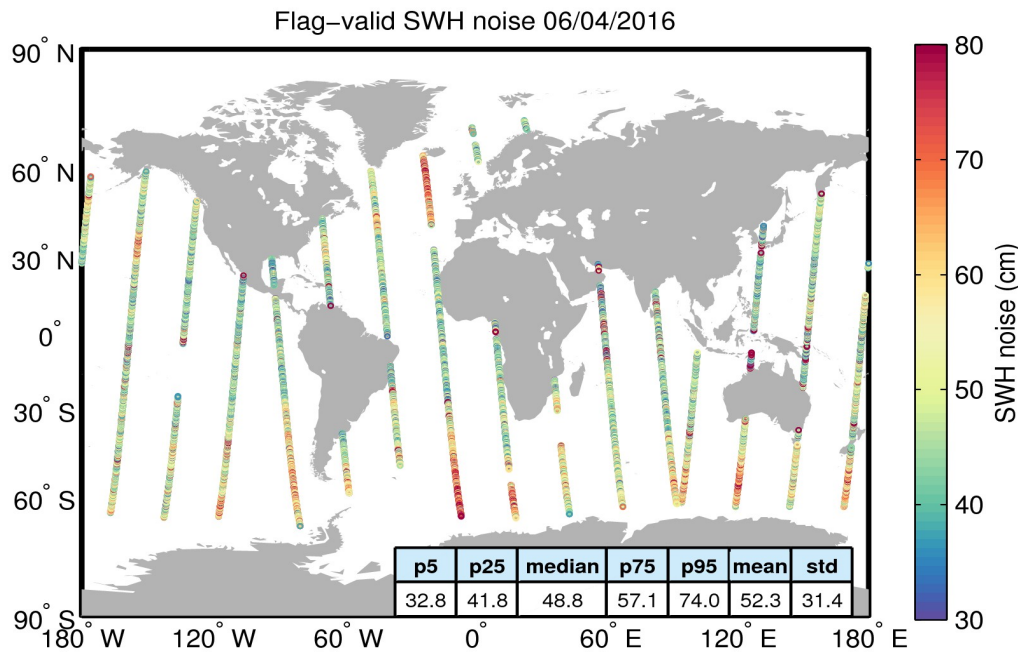
Figure 18. Geographical distribution of flag-valid 20-Hz SWH measurement noise over oceans and lakes for 06/04/2016. The statistical values shown in the figure refer to the SWH noise and are calculated over all measurements shown in the figure.
