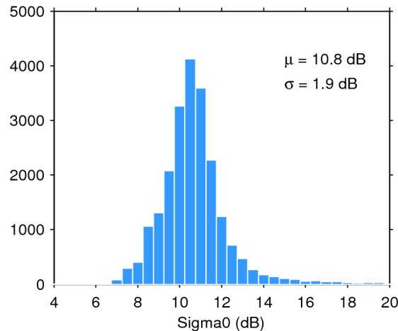
Figure 25. Histogram of flag-valid sigma0 over oceans and lakes for 06/04/2016. The mean ( \mu ) and standard deviation ( \sigma ) are also shown. Note that values outside [4 20] dB are excluded from the histogram for the sake of readability but not from the computation of \mu and \sigma .
