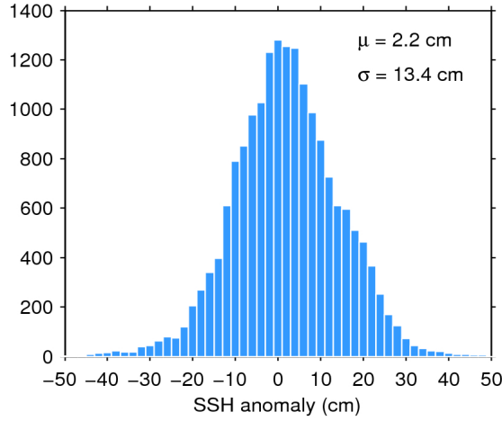
Figure 11. Histogram of science-valid SSH anomaly over oceans and lakes for 06/04/2016. The mean ( \mu ) and standard deviation ( \sigma ) are also shown. Note that values outside [-50 50] cm are excluded from the histogram for the sake of readability but not from the computation of \mu and \sigma .
