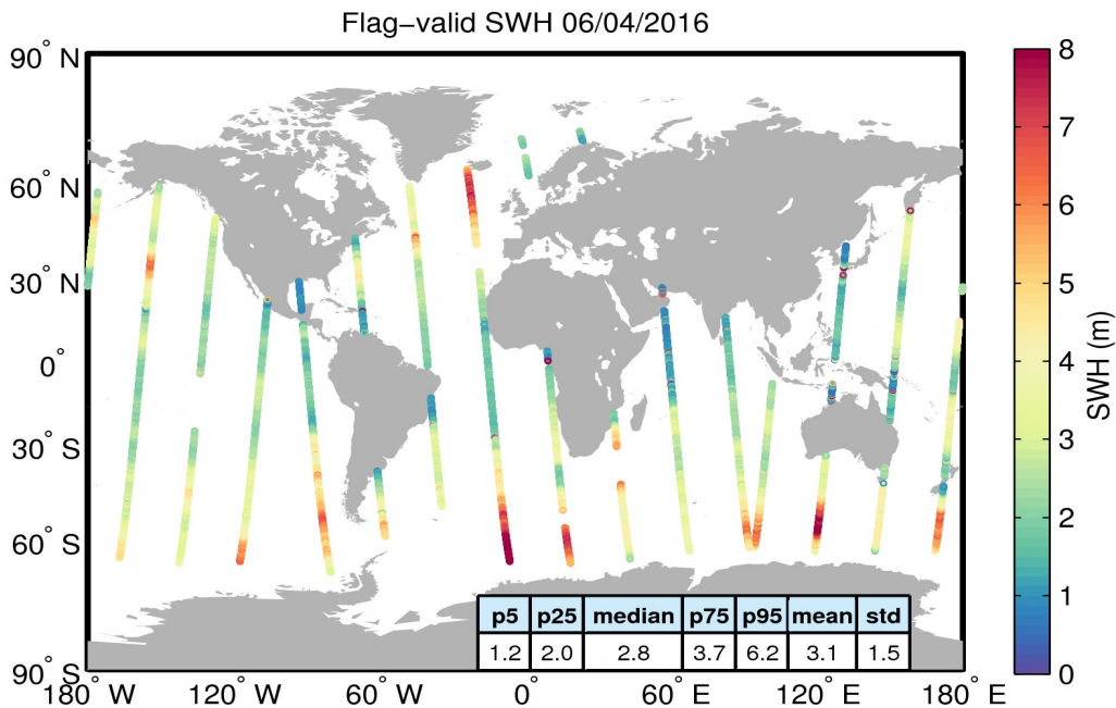
Figure 15. Geographical distribution of flag-valid SWH data over oceans and lakes for 06/04/2016. The statistical values shown in the table refer to the SWH in m and are calculated over all measurements shown in the figure.
