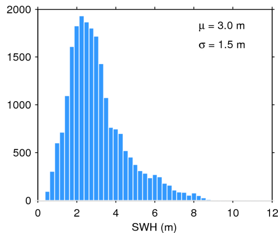
Figure 20. Histogram of science-valid SWH over oceans and lakes for 06/04/2016. The mean ( \mu ) and standard deviation ( \sigma ) are also shown. Note that values larger than 12 m are excluded from the histogram for the sake of readability but not from the computation of \mu and \sigma .
