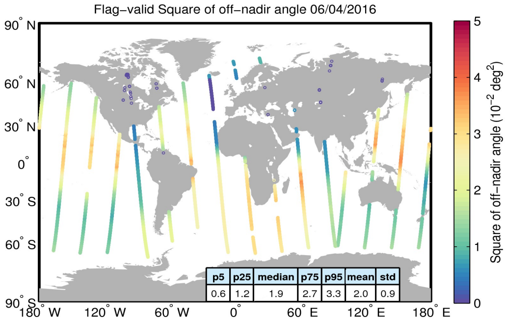
Figure 37. Geographical distribution of flag-valid mispointing data over oceans and lakes for 06/04/2016. The statistical values shown in the table refer to the mispointing in 10^{-2} \text{ deg}^2 and are calculated over all measurements shown in the figure.
