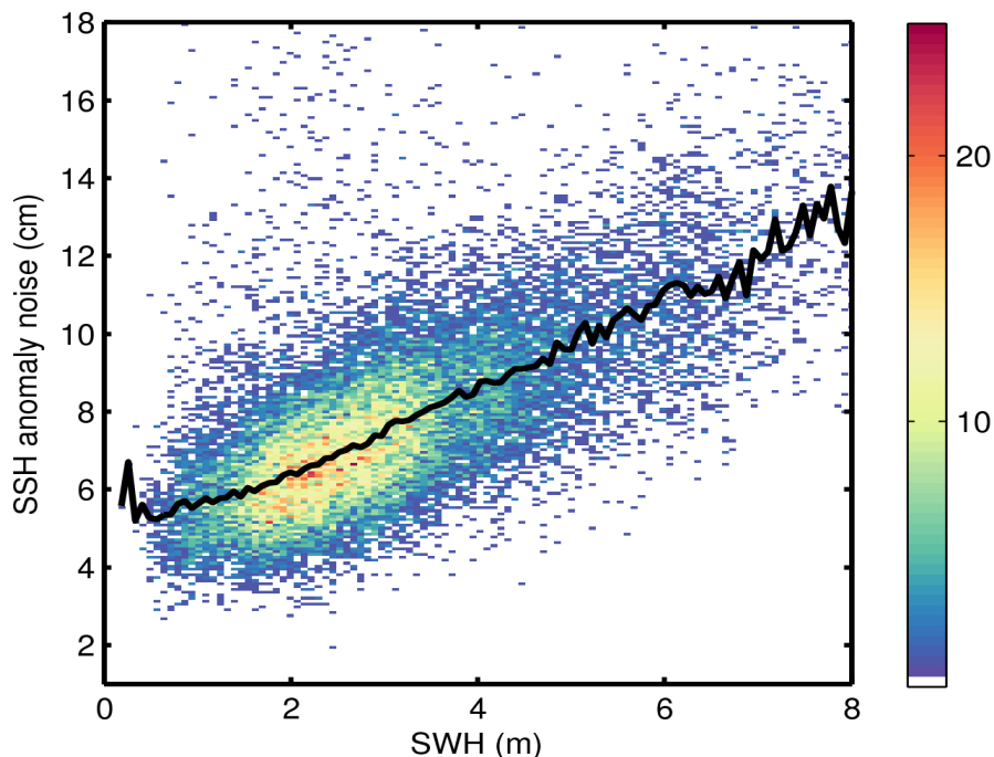
Figure 9. 2D histogram showing flag-valid SSH anomaly noise as a function of SWH for 06/04/2016. The black line denotes the median SSH anomaly noise as a function of SWH.
