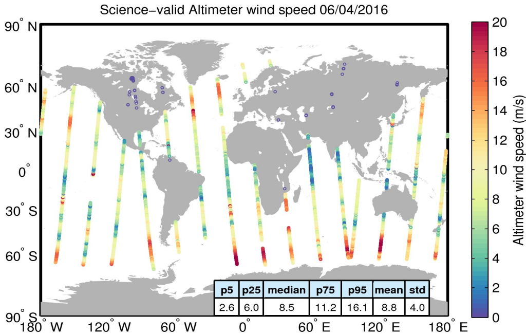
Figure 34. Geographical distribution of science-valid wind data over oceans and lakes for 06/04/2016. The statistical values shown in the table refer to the wind in m/s and are calculated over all measurements shown in the figure. Gray circles denote records that have been rejected based on the editing criteria described in Table 5.
