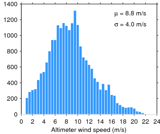
Figure 33. Histogram of flag-valid wind over oceans and lakes for 06/04/2016. The mean ( \mu ) and standard deviation ( \sigma ) are also shown. Note that values larger than 24 m/s are excluded from the histogram for the sake of readability but not from the computation of \mu and \sigma .
