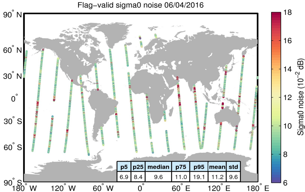
Figure 26. Geographical distribution of flag-valid 20-Hz sigma0 measurement noise over oceans and lakes for 06/04/2016. The statistical values shown in the table refer to the sigma0 noise and are calculated over all measurements shown in the figure.
