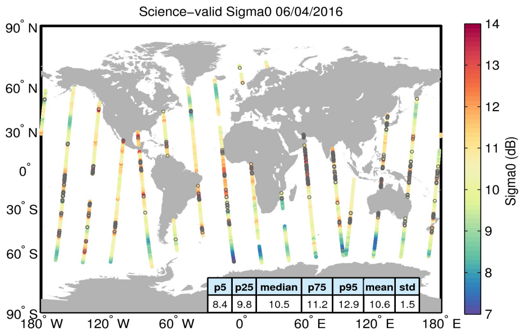
Figure 27. Geographical distribution of science-valid sigma0 data over oceans and lakes for 06/04/2016. The statistical values shown in the table refer to the sigma0 in dB and are calculated over all measurements shown in the figure. Gray circles denote records that have been rejected based on the editing criteria described in Table 4.
