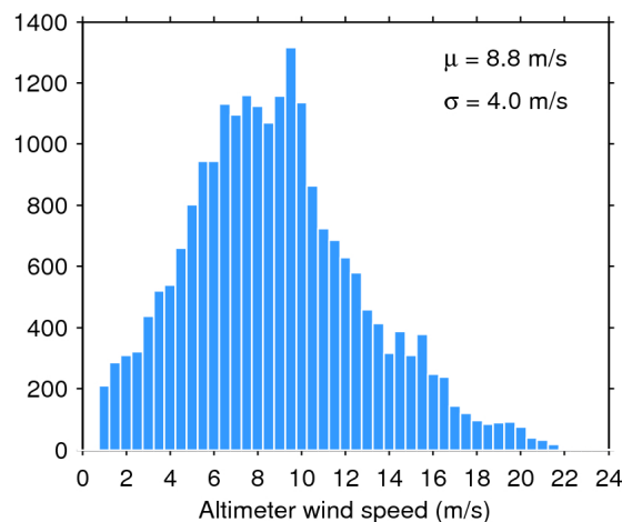
Figure 35. Histogram of science-valid wind over oceans and lakes for 06/04/2016. The mean ( \mu ) and standard deviation ( \sigma ) are also shown. Note that values larger than 24 m/s are excluded from the histogram for the sake of readability but not from the computation of \mu and \sigma .
