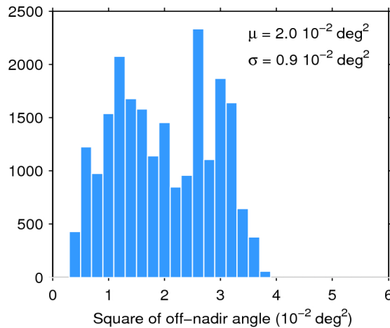
Figure 39. Histogram of flag-valid mispointing over oceans and lakes for 06/04/2016. The mean ( \mu ) and standard deviation ( \sigma ) are also shown. Note that values larger than 6 \cdot 10^{-2} \text{ deg}^2 are excluded from the histogram for the sake of readability but not from the computation of \mu and \sigma .
