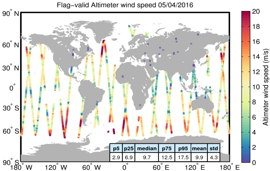
Figure 31. Geographical distribution of flag-valid wind data over oceans and lakes for 05/04/2016. The statistical values shown in the table refer to the wind in m/s and are calculated over all measurements shown in the figure.
