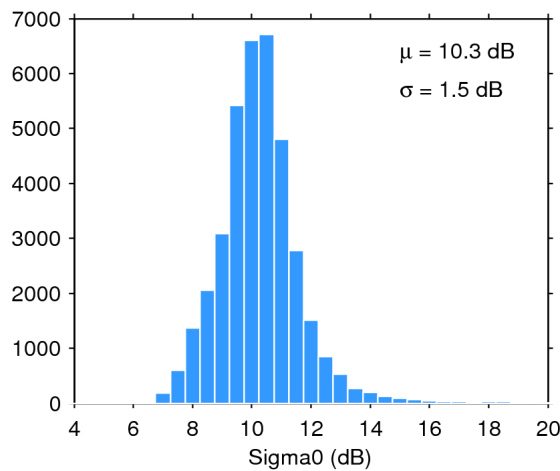
Figure 28. Histogram of science-valid sigma0 over oceans and lakes for 05/04/2016. The mean ( \mu ) and standard deviation ( \sigma ) are also shown. Note that values outside [4 20] dB are excluded from the histogram for the sake of readability but not from the computation of \mu and \sigma .
