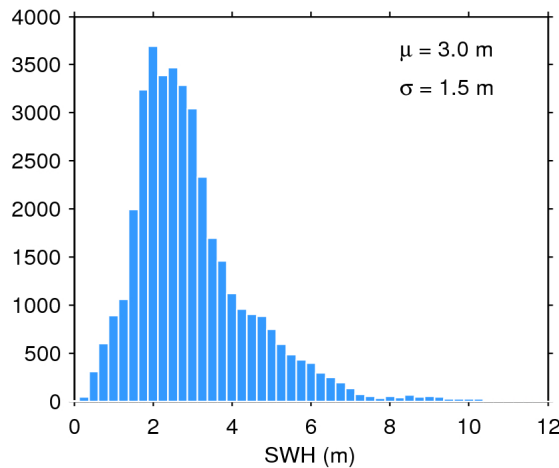
Figure 20. Histogram of science-valid SWH over oceans and lakes for 05/04/2016. The mean ( \mu ) and standard deviation ( \sigma ) are also shown. Note that values larger than 12 m are excluded from the histogram for the sake of readability but not from the computation of \mu and \sigma .
