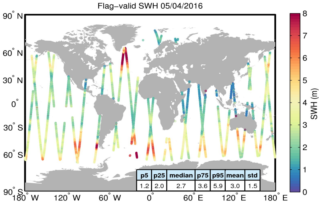
Figure 15. Geographical distribution of flag-valid SWH data over oceans and lakes for 05/04/2016. The statistical values shown in the table refer to the SWH in m and are calculated over all measurements shown in the figure.
