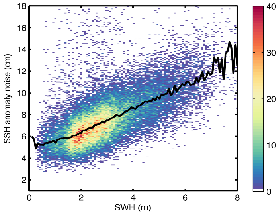
Figure 9. 2D histogram showing flag-valid SSH anomaly noise as a function of SWH for 05/04/2016. The black line denotes the median SSH anomaly noise as a function of SWH.
