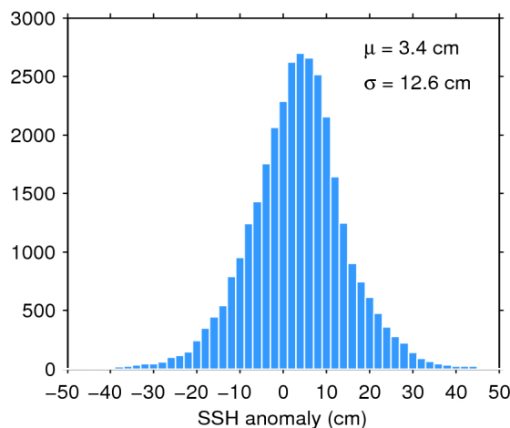
Figure 11. Histogram of science-valid SSH anomaly over oceans and lakes for 05/04/2016. The mean ( \mu ) and standard deviation ( \sigma ) are also shown. Note that values outside [-50 50] cm are excluded from the histogram for the sake of readability but not from the computation of \mu and \sigma .
