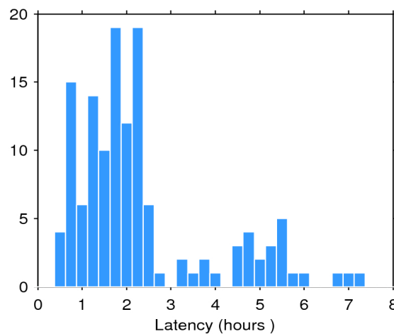
Figure 2. Histogram of the data latency for 05/04/2016. The y-axis denotes the number of files that are made available with a delay of x-hours with respect to the mean time of the records stored in the file.
