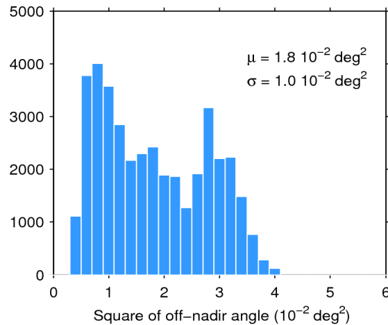
Figure 39. Histogram of flag-valid mispointing over oceans and lakes for 05/04/2016. The mean ( \mu ) and standard deviation ( \sigma ) are also shown. Note that values larger than 6 \cdot 10^{-2} \text{ deg}^2 are excluded from the histogram for the sake of readability but not from the computation of \mu and \sigma .
