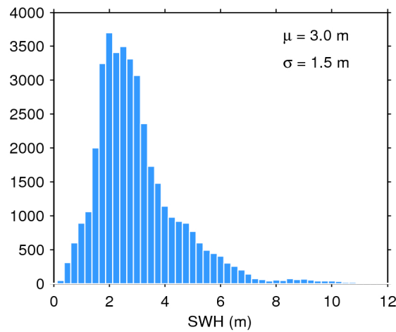
Figure 17. Histogram of flag-valid SWH over oceans and lakes for 05/04/2016. The mean ( \mu ) and standard deviation ( \sigma ) are also shown. Note that values larger than 12 m are excluded from the histogram for the sake of readability but not from the computation of \mu and \sigma .
