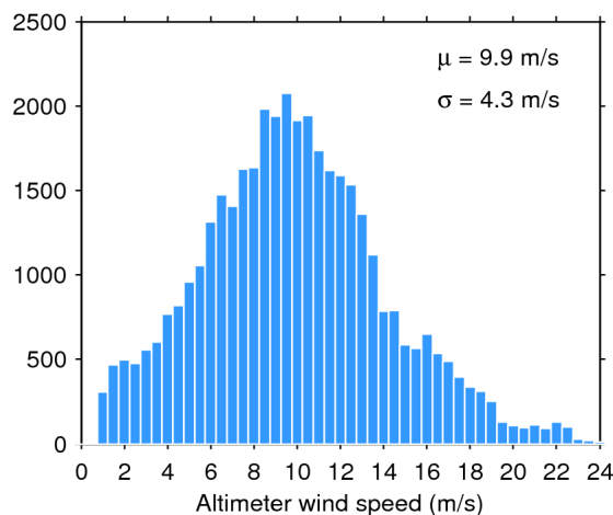
Figure 35. Histogram of science-valid wind over oceans and lakes for 05/04/2016. The mean ( \mu ) and standard deviation ( \sigma ) are also shown. Note that values larger than 24 m/s are excluded from the histogram for the sake of readability but not from the computation of \mu and \sigma .
