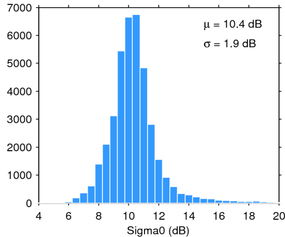
Figure 25. Histogram of flag-valid sigma0 over oceans and lakes for 05/04/2016. The mean ( \mu ) and standard deviation ( \sigma ) are also shown. Note that values outside [4 20] dB are excluded from the histogram for the sake of readability but not from the computation of \mu and \sigma .
