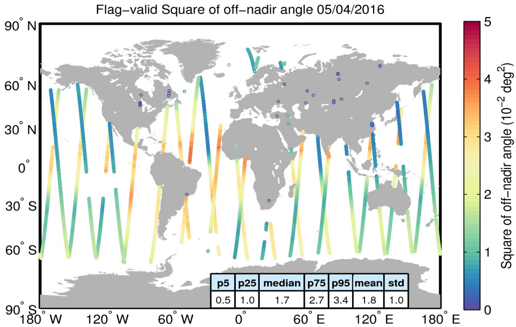
Figure 37. Geographical distribution of flag-valid mispointing data over oceans and lakes for 05/04/2016. The statistical values shown in the table refer to the mispointing in 10^{-2} \text{ deg}^2 and are calculated over all measurements shown in the figure.
