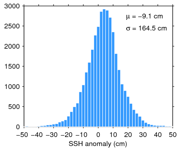
Figure 7. Histogram of flag-valid SSH anomaly over oceans and lakes for 05/04/2016. The mean ( \mu ) and standard deviation ( \sigma ) are also shown. Note that values outside [-50 50] cm are excluded from the histogram for the sake of readability but not from the computation of \mu and \sigma .
