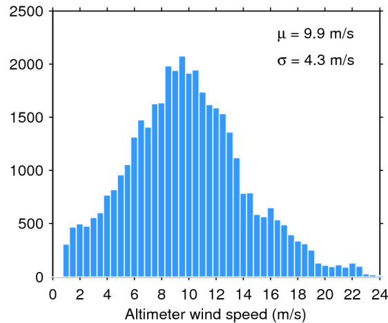
Figure 33. Histogram of flag-valid wind over oceans and lakes for 05/04/2016. The mean ( \mu ) and standard deviation ( \sigma ) are also shown. Note that values larger than 24 m/s are excluded from the histogram for the sake of readability but not from the computation of \mu and \sigma .
