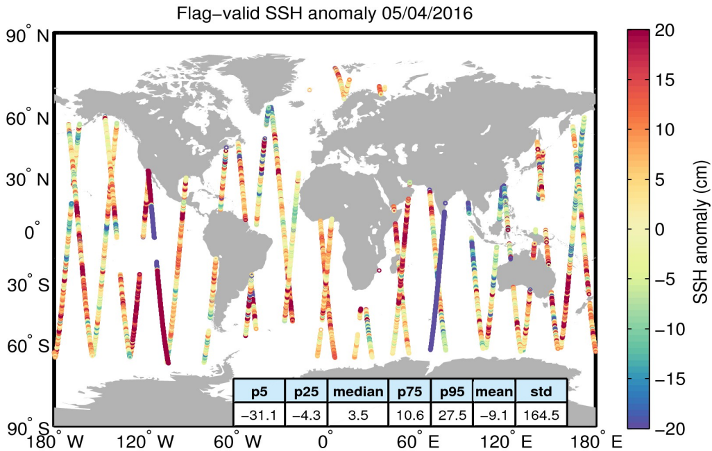
Figure 5. Geographical distribution of flag-valid 1-Hz SSH anomaly data over oceans and lakes for 05/04/2016. The statistical values shown in the table refer to the SSH anomaly in cm and are calculated over all measurements shown in the figure.
