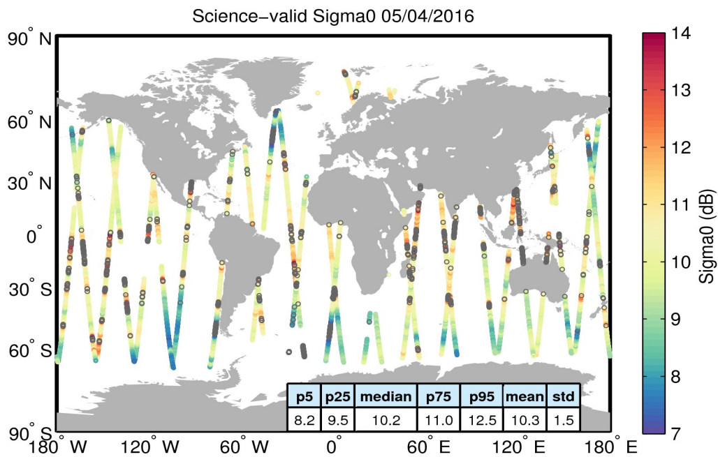
Figure 27. Geographical distribution of science-valid sigma0 data over oceans and lakes for 05/04/2016. The statistical values shown in the table refer to the sigma0 in dB and are calculated over all measurements shown in the figure. Gray circles denote records that have been rejected based on the editing criteria described in Table 4.
