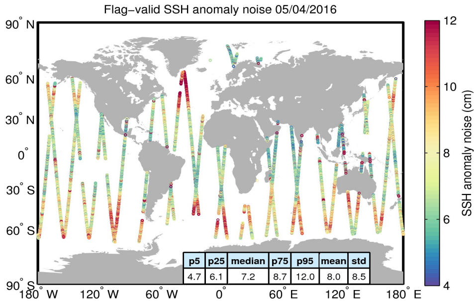
Figure 8. Geographical distribution of flag-valid 20-Hz SSH anomaly measurement noise over oceans and lakes for 05/04/2016. The statistical values shown in the table refer to the SSH anomaly noise and are calculated over all measurements shown in the figure.
