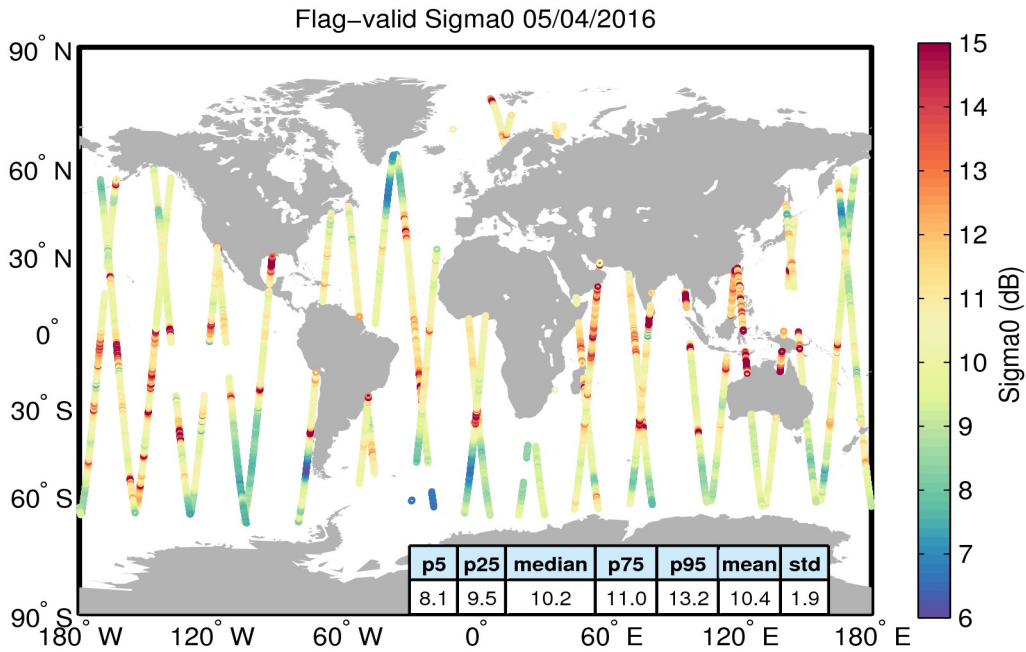
Figure 23. Geographical distribution of flag-valid sigma0 data over oceans and lakes for 05/04/2016. The statistical values shown in the table refer to the sigma0 in dB and are calculated over all measurements shown in the figure.
