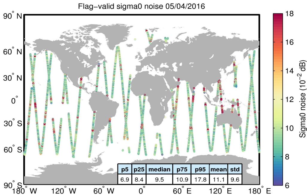
Figure 26. Geographical distribution of flag-valid 20-Hz sigma0 measurement noise over oceans and lakes for 05/04/2016. The statistical values shown in the table refer to the sigma0 noise and are calculated over all measurements shown in the figure.
