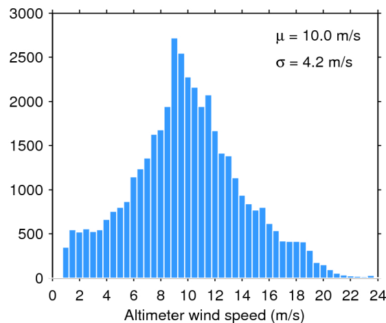
Figure 35. Histogram of science-valid wind over oceans and lakes for 03/04/2016. The mean ( \mu ) and standard deviation ( \sigma ) are also shown. Note that values larger than 24 m/s are excluded from the histogram for the sake of readability but not from the computation of \mu and \sigma .
