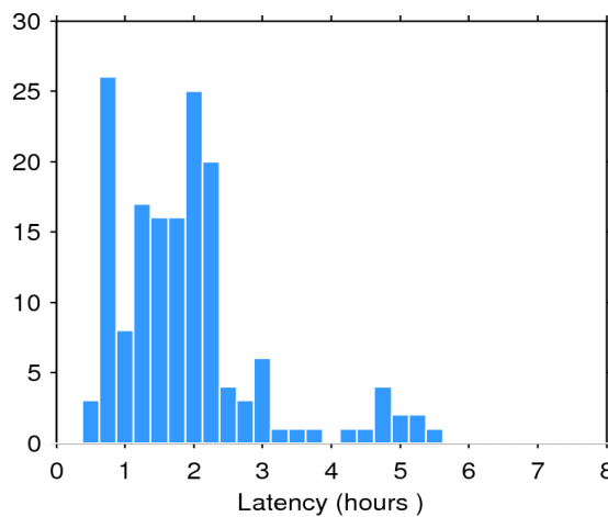
Figure 2. Histogram of the data latency for 03/04/2016. The y-axis denotes the number of files that are made available with a delay of x-hours with respect to the mean time of the records stored in the file.
