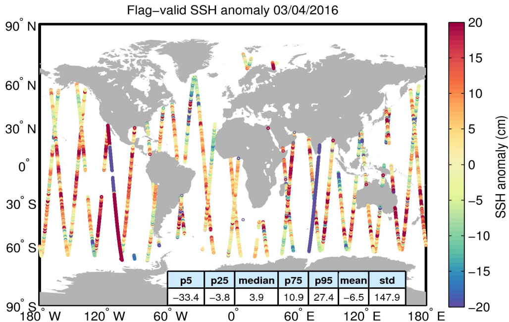
Figure 5. Geographical distribution of flag-valid 1-Hz SSH anomaly data over oceans and lakes for 03/04/2016. The statistical values shown in the table refer to the SSH anomaly in cm and are calculated over all measurements shown in the figure.
