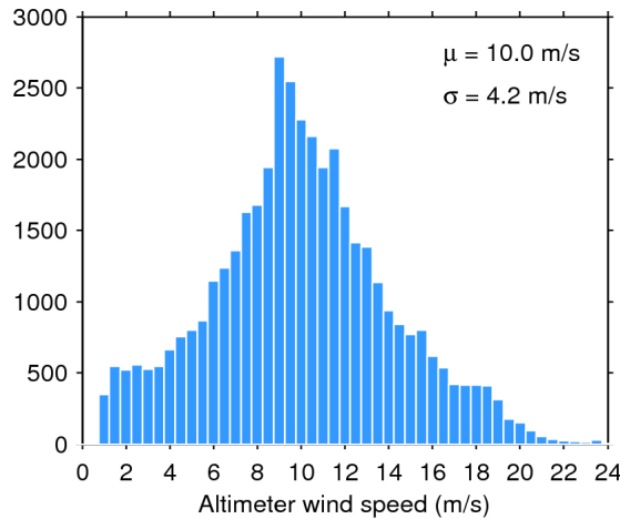
Figure 33. Histogram of flag-valid wind over oceans and lakes for 03/04/2016. The mean ( \mu ) and standard deviation ( \sigma ) are also shown. Note that values larger than 24 m/s are excluded from the histogram for the sake of readability but not from the computation of \mu and \sigma .
