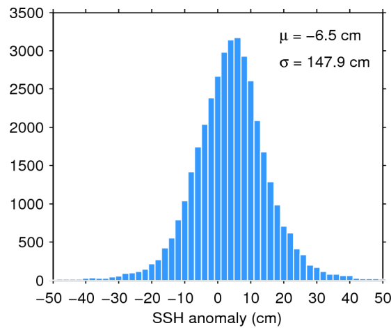
Figure 7. Histogram of flag-valid SSH anomaly over oceans and lakes for 03/04/2016. The mean ( \mu ) and standard deviation ( \sigma ) are also shown. Note that values outside [-50\ 50] cm are excluded from the histogram for the sake of readability but not from the computation of \mu and \sigma .
