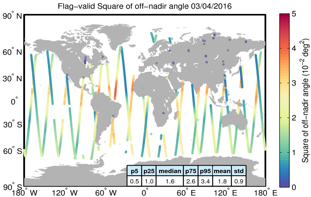
Figure 37. Geographical distribution of flag-valid mispointing data over oceans and lakes for 03/04/2016. The statistical values shown in the table refer to the mispointing in 10^{-2} deg 2 and are calculated over all measurements shown in the figure.
