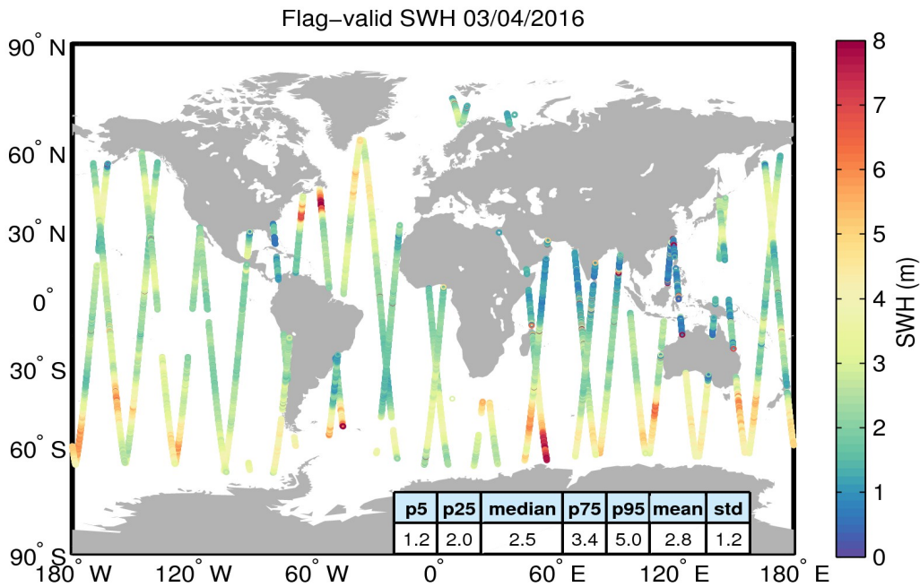
Figure 15. Geographical distribution of flag-valid SWH data over oceans and lakes for 03/04/2016. The statistical values shown in the table refer to the SWH in m and are calculated over all measurements shown in the figure.
