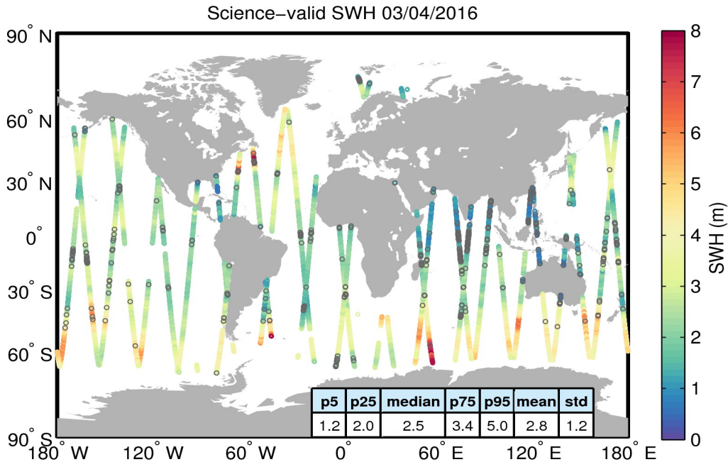
Figure 19. Geographical distribution of science-valid SWH data over oceans and lakes for 03/04/2016. The statistical values shown in the table refer to the SWH in m and are calculated over all measurements shown in the figure. Gray circles denote records that have been rejected based on the editing criteria described in Table 3.
