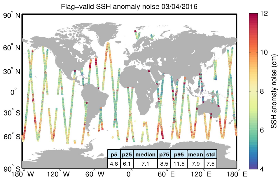
Figure 8. Geographical distribution of flag-valid 20-Hz SSH anomaly measurement noise over oceans and lakes for 03/04/2016. The statistical values shown in the table refer to the SSH anomaly noise and are calculated over all measurements shown in the figure.
