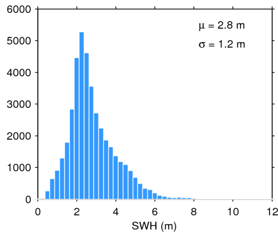
Figure 17. Histogram of flag-valid SWH over oceans and lakes for 03/04/2016. The mean ( \mu ) and standard deviation ( \sigma ) are also shown. Note that values larger than 12 m are excluded from the histogram for the sake of readability but not from the computation of \mu and \sigma .
