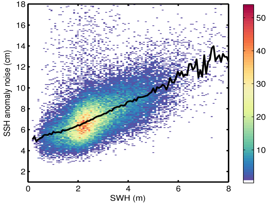
Figure 9. 2D histogram showing flag-valid SSH anomaly noise as a function of SWH for 03/04/2016. The black line denotes the median SSH anomaly noise as a function of SWH.
