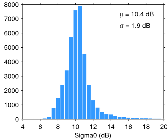
Figure 25. Histogram of flag-valid sigma0 over oceans and lakes for 03/04/2016. The mean ( \mu ) and standard deviation ( \sigma ) are also shown. Note that values outside [4 20] dB are excluded from the histogram for the sake of readability but not from the computation of \mu and \sigma .
