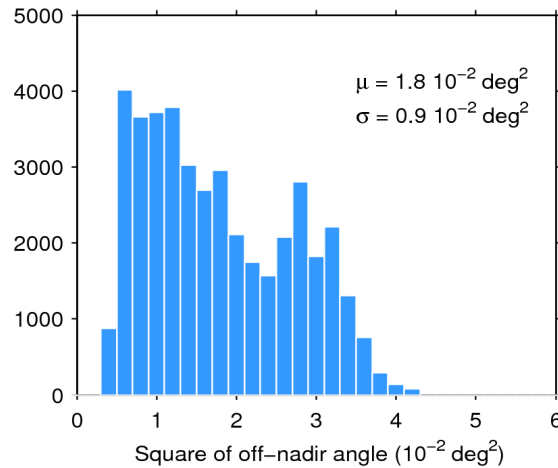
Figure 39. Histogram of flag-valid mispointing over oceans and lakes for 03/04/2016. The mean ( \mu ) and standard deviation ( \sigma ) are also shown. Note that values larger than 6 \cdot 10^{-2} \text{ deg}^2 are excluded from the histogram for the sake of readability but not from the computation of \mu and \sigma .
