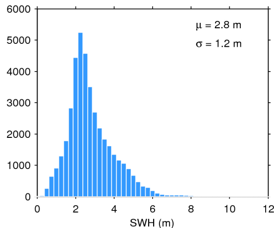
Figure 20. Histogram of science-valid SWH over oceans and lakes for 03/04/2016. The mean ( \mu ) and standard deviation ( \sigma ) are also shown. Note that values larger than 12 m are excluded from the histogram for the sake of readability but not from the computation of \mu and \sigma .
