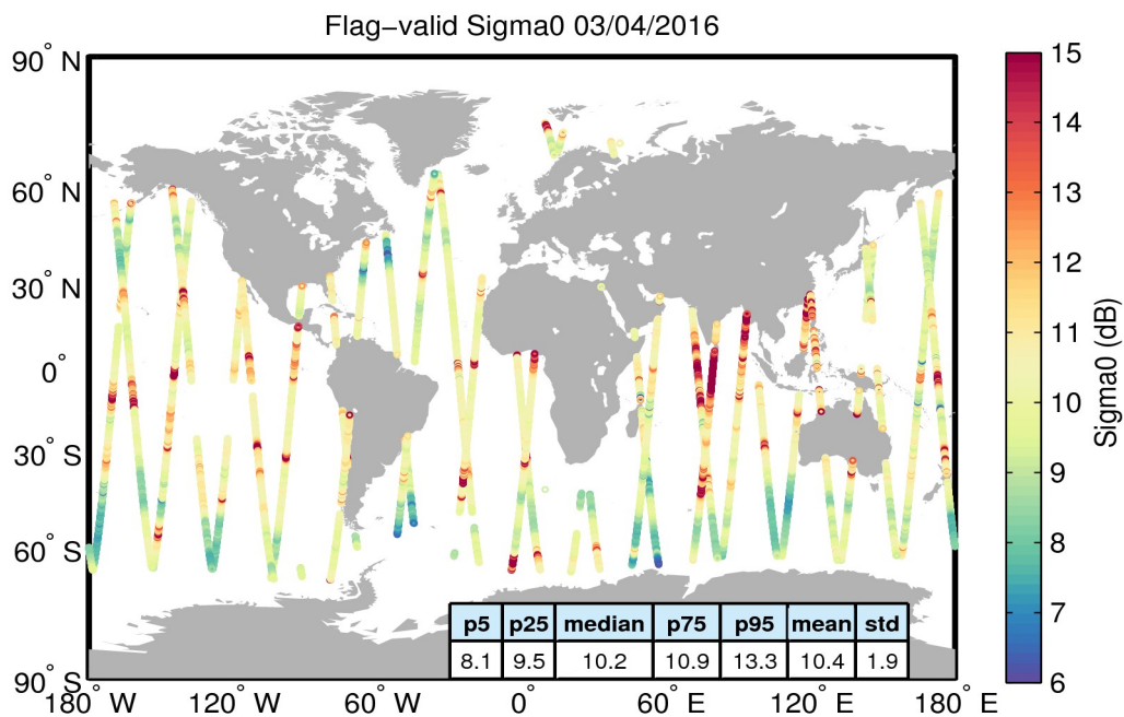
Figure 23. Geographical distribution of flag-valid sigma0 data over oceans and lakes for 03/04/2016. The statistical values shown in the table refer to the sigma0 in dB and are calculated over all measurements shown in the figure.
