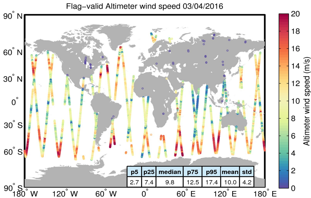
Figure 31. Geographical distribution of flag-valid wind data over oceans and lakes for 03/04/2016. The statistical values shown in the table refer to the wind in m/s and are calculated over all measurements shown in the figure.
