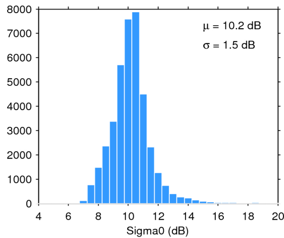
Figure 28. Histogram of science-valid sigma0 over oceans and lakes for 03/04/2016. The mean ( \mu ) and standard deviation ( \sigma ) are also shown. Note that values outside [4 20] dB are excluded from the histogram for the sake of readability but not from the computation of \mu and \sigma .
