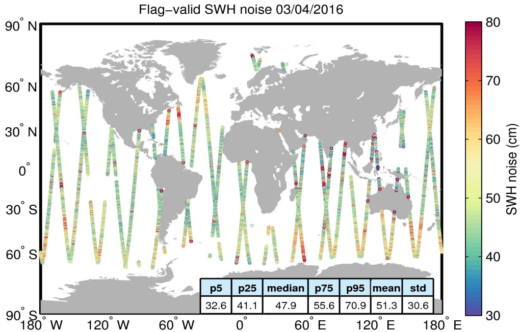
Figure 18. Geographical distribution of flag-valid 20-Hz SWH measurement noise over oceans and lakes for 03/04/2016. The statistical values shown in the figure refer to the SWH noise and are calculated over all measurements shown in the figure.
