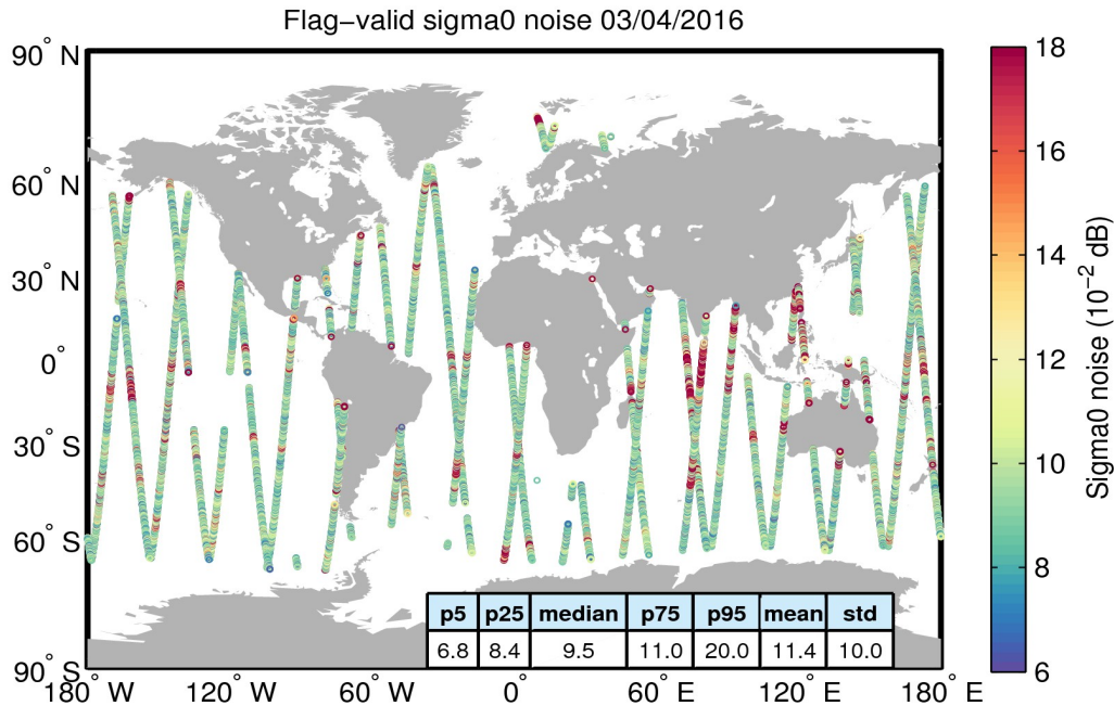
Figure 26. Geographical distribution of flag-valid 20-Hz sigma0 measurement noise over oceans and lakes for 03/04/2016. The statistical values shown in the table refer to the sigma0 noise and are calculated over all measurements shown in the figure.
