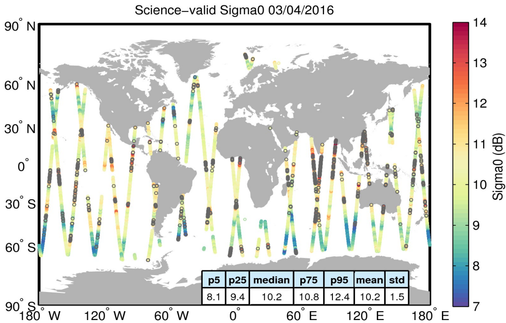
Figure 27. Geographical distribution of science-valid sigma0 data over oceans and lakes for 03/04/2016. The statistical values shown in the table refer to the sigma0 in dB and are calculated over all measurements shown in the figure. Gray circles denote records that have been rejected based on the editing criteria described in Table 4.
