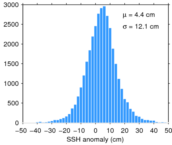
Figure 11. Histogram of science-valid SSH anomaly over oceans and lakes for 03/04/2016. The mean ( \mu ) and standard deviation ( \sigma ) are also shown. Note that values outside [-50 50] cm are excluded from the histogram for the sake of readability but not from the computation of \mu and \sigma .
