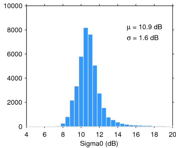
Figure 28. Histogram of science-valid sigma0 over oceans and lakes for 02/04/2016. The mean ( \mu ) and standard deviation ( \sigma ) are also shown. Note that values outside [4 20] dB are excluded from the histogram for the sake of readability but not from the computation of \mu and \sigma .
