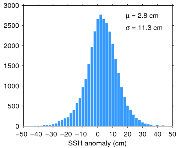
Figure 11. Histogram of science-valid SSH anomaly over oceans and lakes for 02/04/2016. The mean ( \mu ) and standard deviation ( \sigma ) are also shown. Note that values outside [-50 50] cm are excluded from the histogram for the sake of readability but not from the computation of \mu and \sigma .
