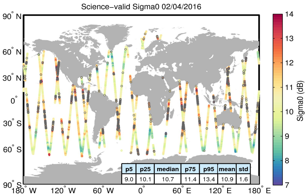
Figure 27. Geographical distribution of science-valid sigma0 data over oceans and lakes for 02/04/2016. The statistical values shown in the table refer to the sigma0 in dB and are calculated over all measurements shown in the figure. Gray circles denote records that have been rejected based on the editing criteria described in Table 4.
