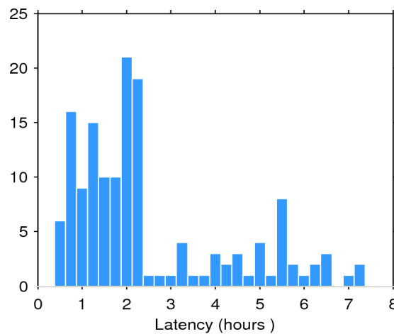
Figure 2. Histogram of the data latency for 02/04/2016. The y-axis denotes the number of files that are made available with a delay of x-hours with respect to the mean time of the records stored in the file.
