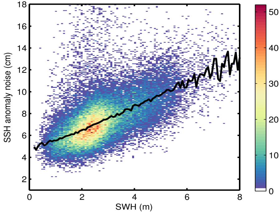
Figure 9. 2D histogram showing flag-valid SSH anomaly noise as a function of SWH for 02/04/2016. The black line denotes the median SSH anomaly noise as a function of SWH.
