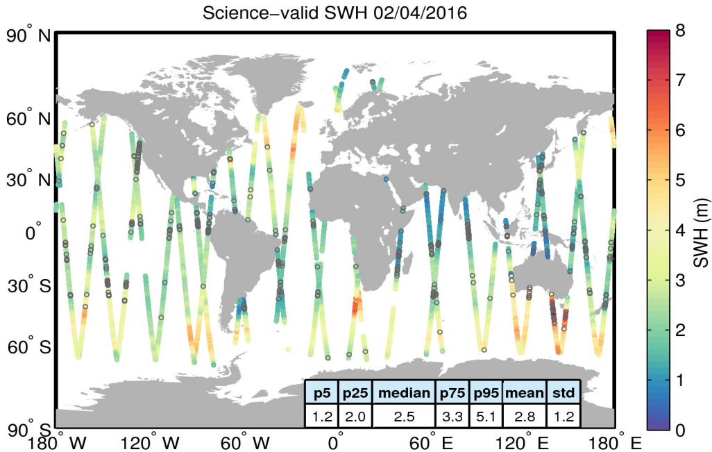
Figure 19. Geographical distribution of science-valid SWH data over oceans and lakes for 02/04/2016. The statistical values shown in the table refer to the SWH in m and are calculated over all measurements shown in the figure. Gray circles denote records that have been rejected based on the editing criteria described in Table 3.
