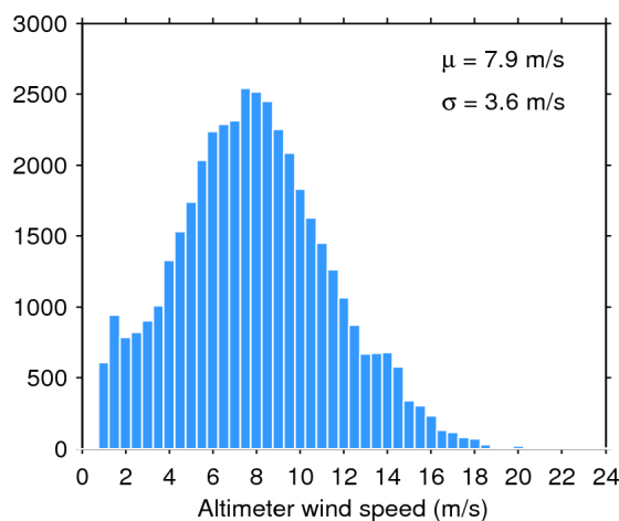
Figure 35. Histogram of science-valid wind over oceans and lakes for 02/04/2016. The mean ( \mu ) and standard deviation ( \sigma ) are also shown. Note that values larger than 24 m/s are excluded from the histogram for the sake of readability but not from the computation of \mu and \sigma .
