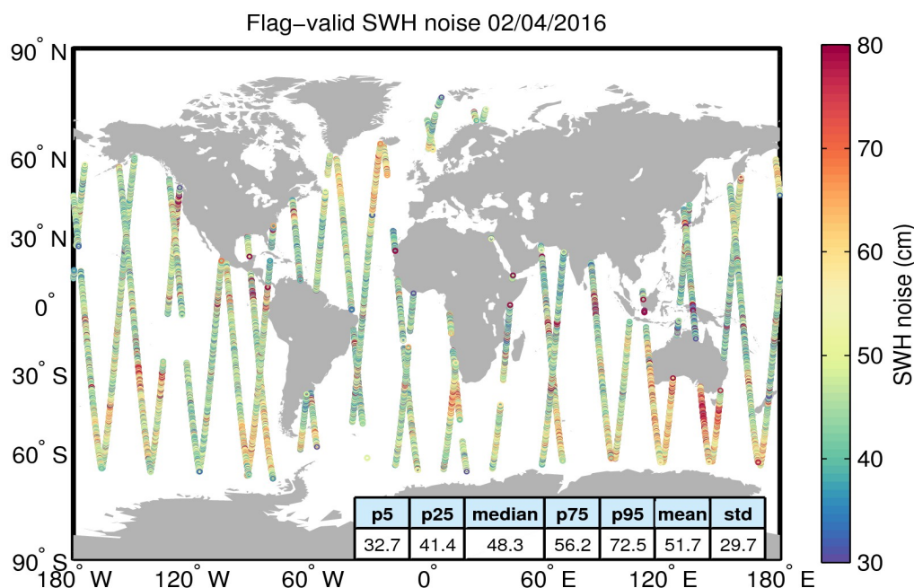
Figure 18. Geographical distribution of flag-valid 20-Hz SWH measurement noise over oceans and lakes for 02/04/2016. The statistical values shown in the table refer to the SWH noise and are calculated over all measurements shown in the figure.
