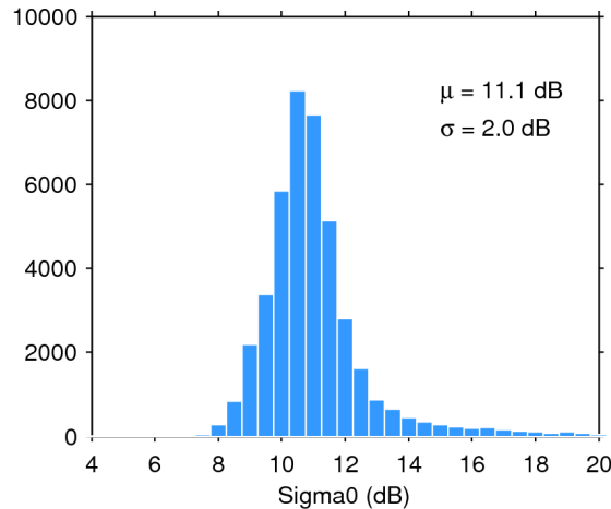
Figure 25. Histogram of flag-valid sigma0 over oceans and lakes for 02/04/2016. The mean ( \mu ) and standard deviation ( \sigma ) are also shown. Note that values outside [4 20] dB are excluded from the histogram for the sake of readability but not from the computation of \mu and \sigma .
