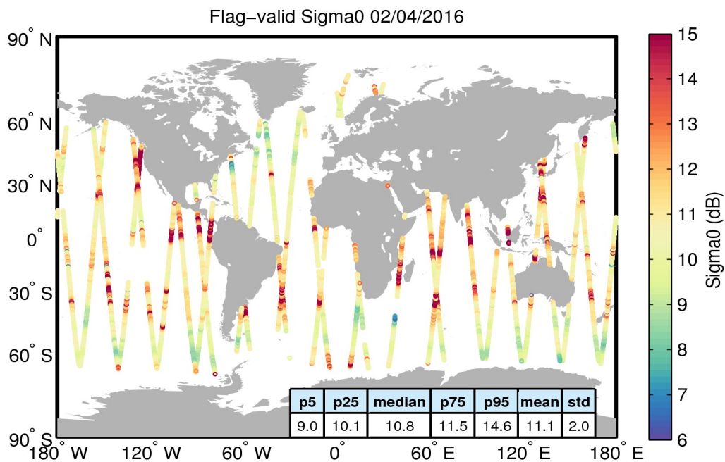
Figure 23. Geographical distribution of flag-valid sigma0 data over oceans and lakes for 02/04/2016. The statistical values shown in the table refer to the sigma0 in dB and are calculated over all measurements shown in the figure.
