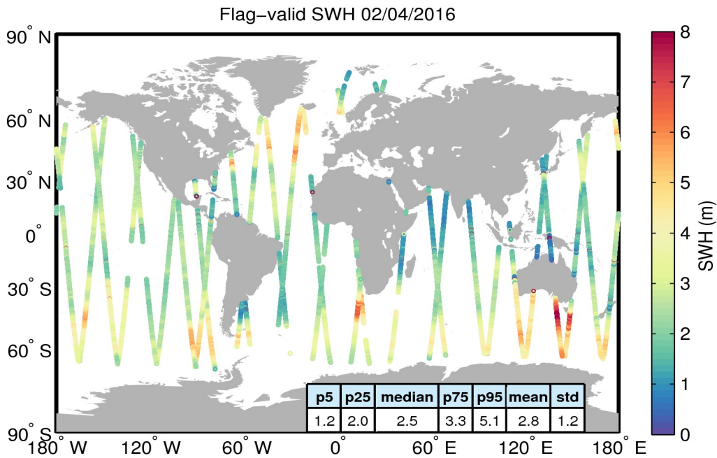
Figure 15. Geographical distribution of flag-valid SWH data over oceans and lakes for 02/04/2016. The statistical values shown in the table refer to the SWH in m and are calculated over all measurements shown in the figure.
