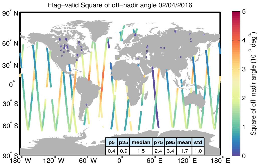
Figure 37. Geographical distribution of flag-valid mispointing data over oceans and lakes for 02/04/2016. The statistical values shown in the table refer to the mispointing in 10^{-2} \text{ deg}^2 and are calculated over all measurements shown in the figure.
