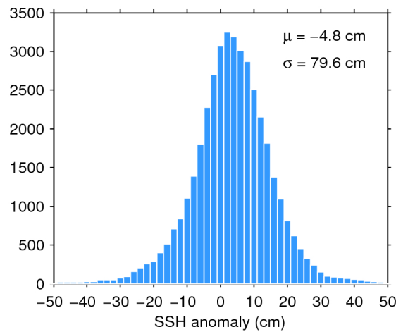
Figure 7. Histogram of flag-valid SSH anomaly over oceans and lakes for 02/04/2016. The mean ( \mu ) and standard deviation ( \sigma ) are also shown. Note that values outside [-50 50] cm are excluded from the histogram for the sake of readability but not from the computation of \mu and \sigma .
