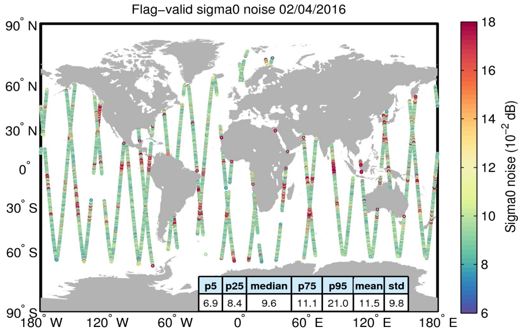
Figure 26. Geographical distribution of flag-valid 20-Hz sigma0 measurement noise over oceans and lakes for 02/04/2016. The statistical values shown in the table refer to the sigma0 noise and are calculated over all measurements shown in the figure.
