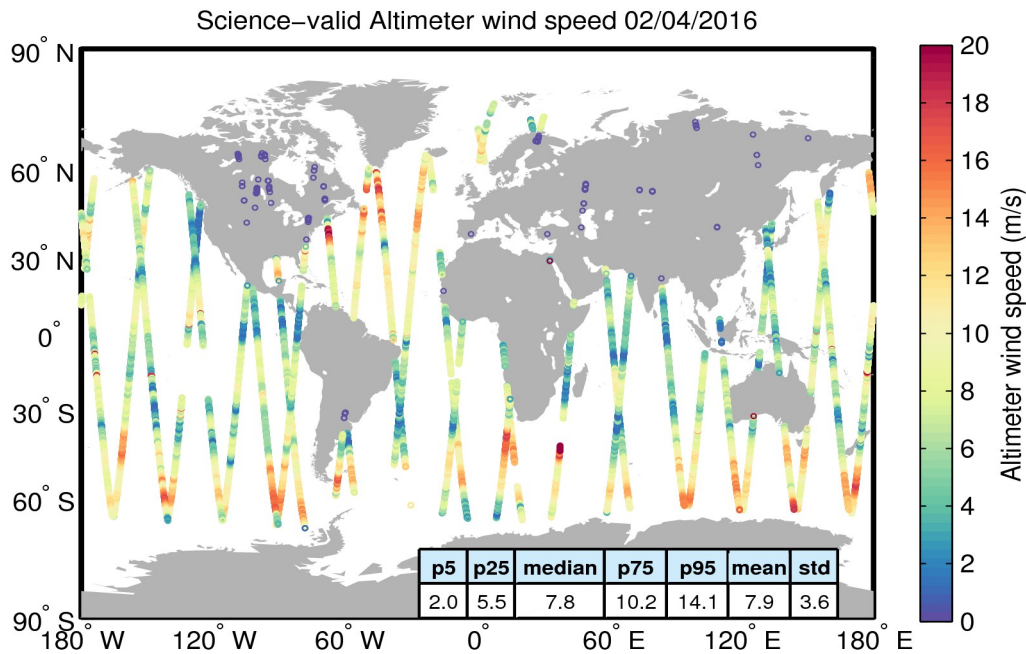
Figure 34. Geographical distribution of science-valid wind data over oceans and lakes for 02/04/2016. The statistical values shown in the table refer to the wind in m/s and are calculated over all measurements shown in the figure. Gray circles denote records that have been rejected based on the editing criteria described in Table 5.
