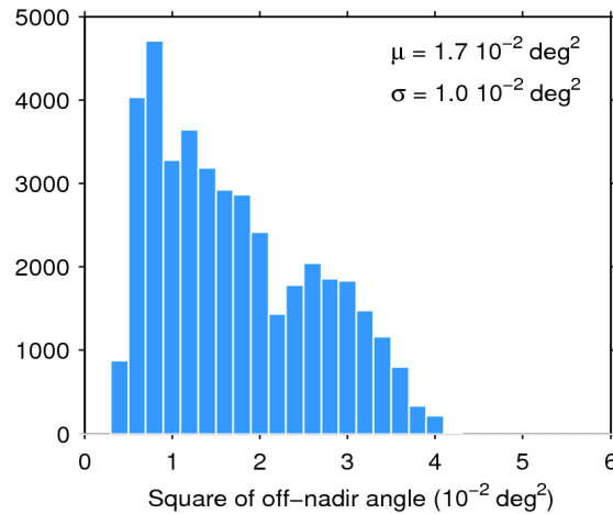
Figure 39. Histogram of flag-valid mispointing over oceans and lakes for 02/04/2016. The mean ( \mu ) and standard deviation ( \sigma ) are also shown. Note that values larger than 6 \cdot 10^{-2} \text{ deg}^2 are excluded from the histogram for the sake of readability but not from the computation of \mu and \sigma .
