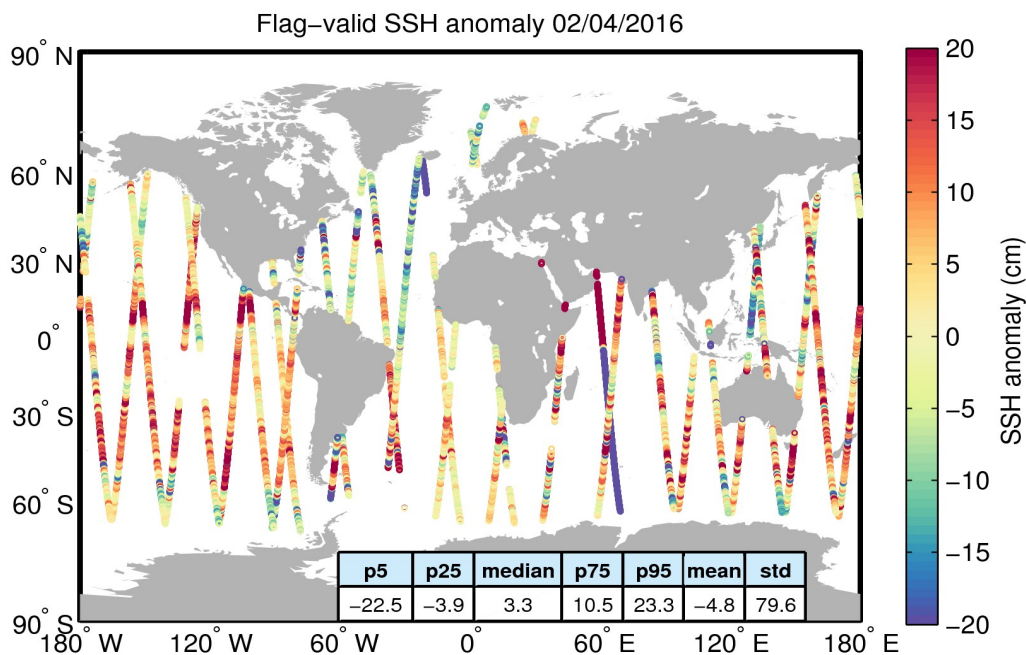
Figure 5. Geographical distribution of flag-valid 1-Hz SSH anomaly data over oceans and lakes for 02/04/2016. The statistical values shown in the table refer to the SSH anomaly in cm and are calculated over all measurements shown in the figure.
