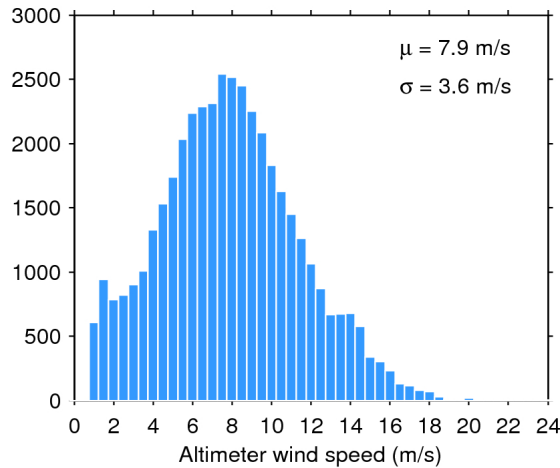
Figure 33. Histogram of flag-valid wind over oceans and lakes for 02/04/2016. The mean ( \mu ) and standard deviation ( \sigma ) are also shown. Note that values larger than 24 m/s are excluded from the histogram for the sake of readability but not from the computation of \mu and \sigma .
