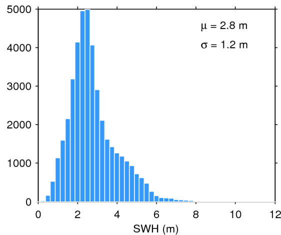
Figure 17. Histogram of flag-valid SWH over oceans and lakes for 02/04/2016. The mean ( \mu ) and standard deviation ( \sigma ) are also shown. Note that values larger than 12 m are excluded from the histogram for the sake of readability but not from the computation of \mu and \sigma .
