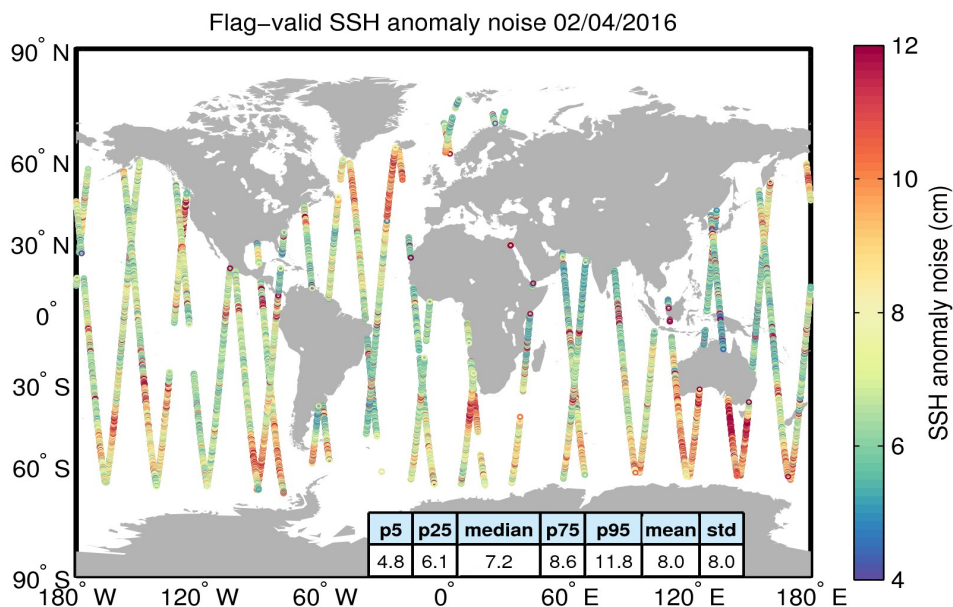
Figure 8. Geographical distribution of flag-valid 20-Hz SSH anomaly measurement noise over oceans and lakes for 02/04/2016. The statistical values shown in the table refer to the SSH anomaly noise and are calculated over all measurements shown in the figure.
