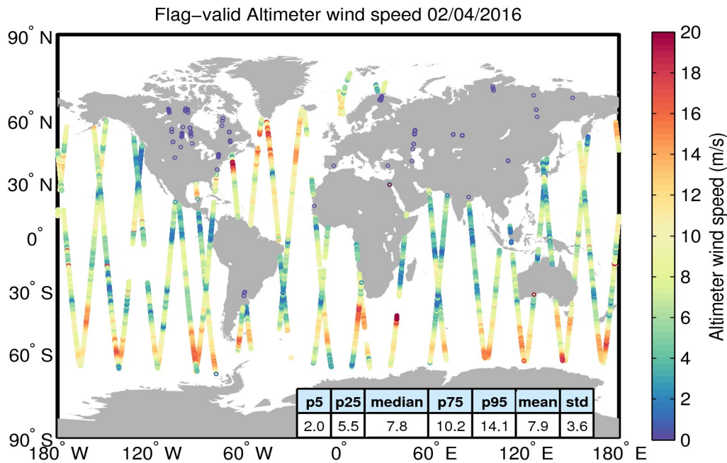
Figure 31. Geographical distribution of flag-valid wind data over oceans and lakes for 02/04/2016. The statistical values shown in the table refer to the wind in m/s and are calculated over all measurements shown in the figure.
