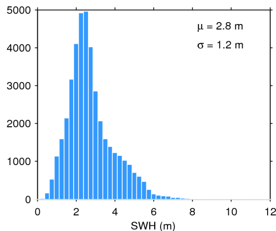
Figure 20. Histogram of science-valid SWH over oceans and lakes for 02/04/2016. The mean ( \mu ) and standard deviation ( \sigma ) are also shown. Note that values larger than 12 m are excluded from the histogram for the sake of readability but not from the computation of \mu and \sigma .
