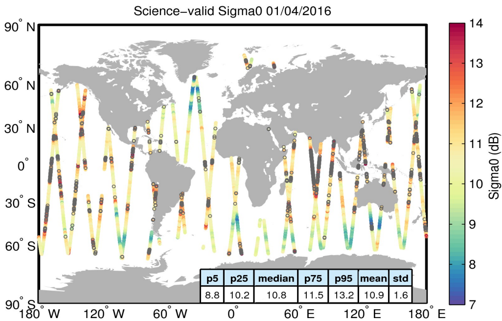
Figure 27. Geographical distribution of science-valid sigma0 data over oceans and lakes for 01/04/2016. The statistical values shown in the table refer to the sigma0 in dB and are calculated over all measurements shown in the figure. Gray circles denote records that have been rejected based on the editing criteria described in Table 4.
