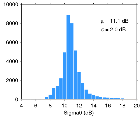
Figure 25. Histogram of flag-valid sigma0 over oceans and lakes for 01/04/2016. The mean ( \mu ) and standard deviation ( \sigma ) are also shown. Note that values outside [4 20] dB are excluded from the histogram for the sake of readability but not from the computation of \mu and \sigma .
