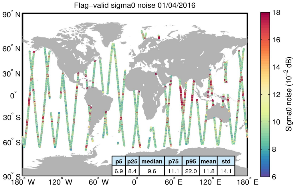
Figure 26. Geographical distribution of flag-valid 20-Hz sigma0 measurement noise over oceans and lakes for 01/04/2016. The statistical values shown in the table refer to the sigma0 noise and are calculated over all measurements shown in the figure.
