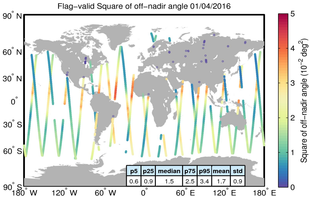
Figure 37. Geographical distribution of flag-valid mispointing data over oceans and lakes for 01/04/2016. The statistical values shown in the table refer to the mispointing in 10^{-2} deg 2 and are calculated over all measurements shown in the figure.
