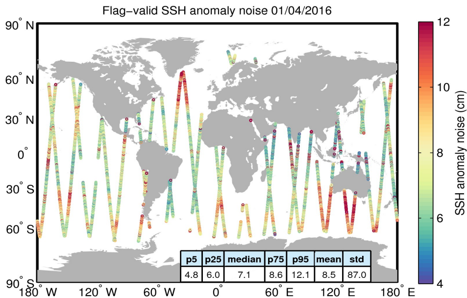
Figure 8. Geographical distribution of flag-valid 20-Hz SSH anomaly measurement noise over oceans and lakes for 01/04/2016. The statistical values shown in the table refer to the SSH anomaly noise and are calculated over all measurements shown in the figure.
