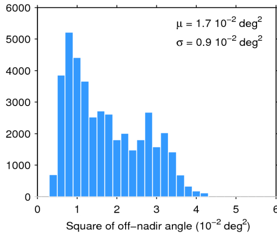
Figure 39. Histogram of flag-valid mispointing over oceans and lakes for 01/04/2016. The mean ( \mu ) and standard deviation ( \sigma ) are also shown. Note that values larger than 6 \cdot 10^{-2} \text{ deg}^2 are excluded from the histogram for the sake of readability but not from the computation of \mu and \sigma .
