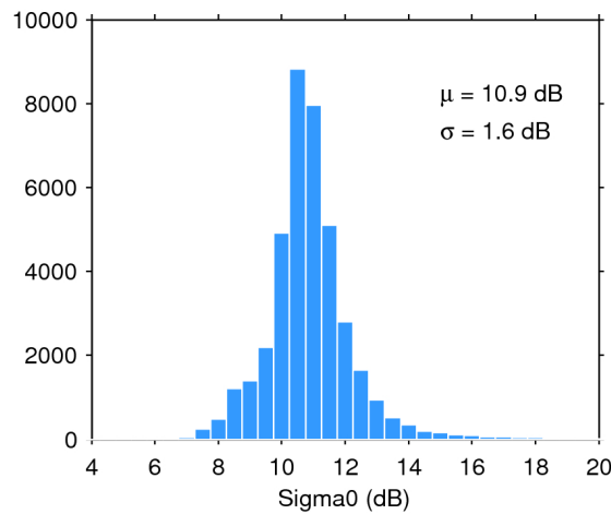
Figure 28. Histogram of science-valid sigma0 over oceans and lakes for 01/04/2016. The mean ( \mu ) and standard deviation ( \sigma ) are also shown. Note that values outside [4 20] dB are excluded from the histogram for the sake of readability but not from the computation of \mu and \sigma .
