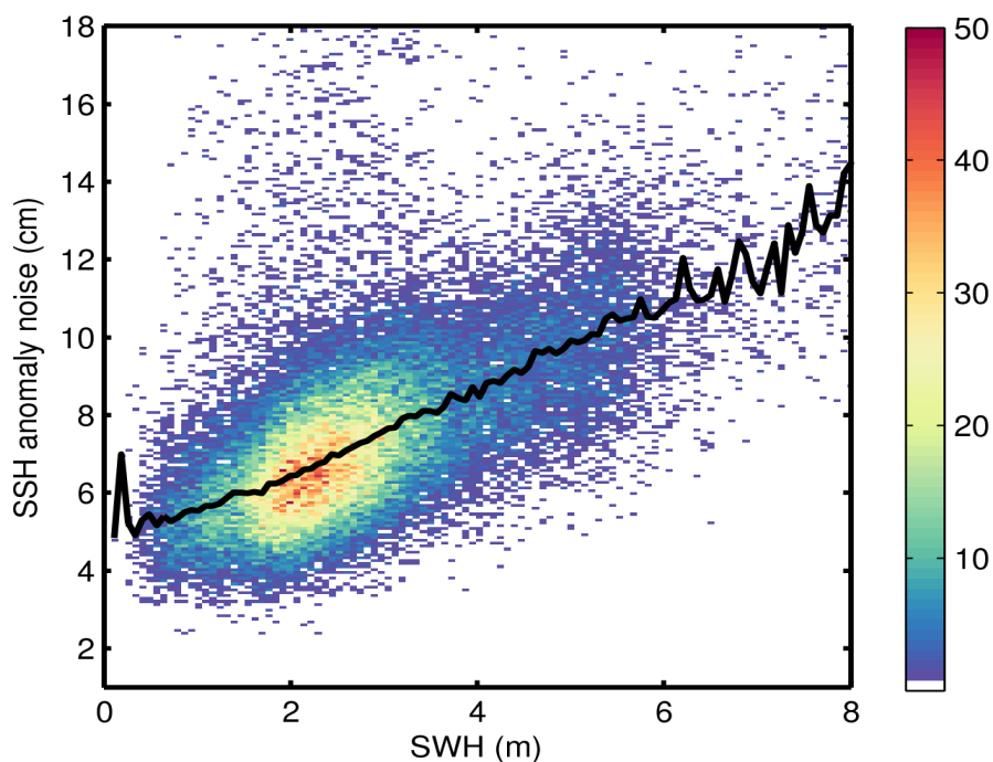
Figure 9. 2D histogram showing flag-valid SSH anomaly noise as a function of SWH for 01/04/2016. The black line denotes the median SSH anomaly noise as a function of SWH.
