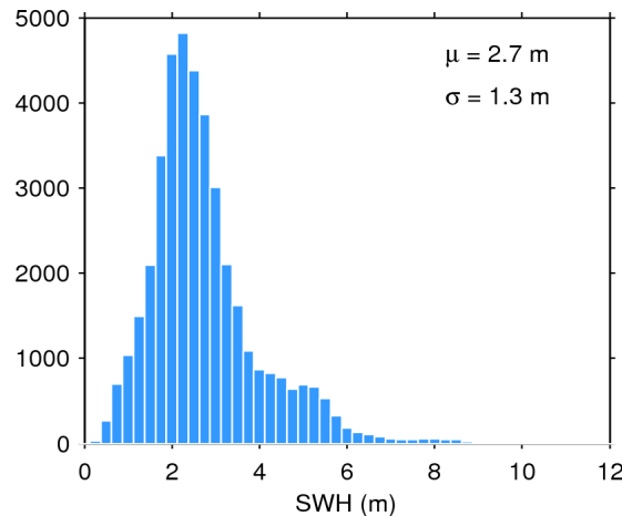
Figure 20. Histogram of science-valid SWH over oceans and lakes for 01/04/2016. The mean ( \mu ) and standard deviation ( \sigma ) are also shown. Note that values larger than 12 m are excluded from the histogram for the sake of readability but not from the computation of \mu and \sigma .
