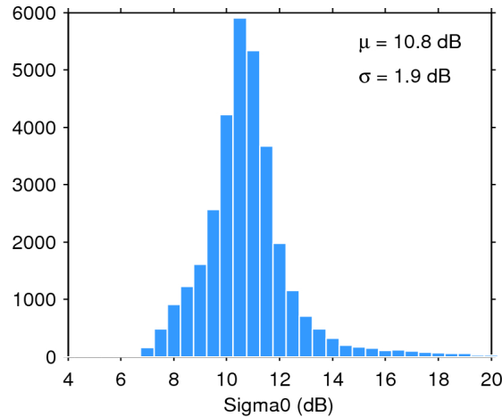
Figure 25. Histogram of flag-valid sigma0 over oceans and lakes for 30/03/2016. The mean ( \mu ) and standard deviation ( \sigma ) are also shown. Note that values outside [4 20] dB are excluded from the histogram for the sake of readability but not from the computation of \mu and \sigma .
