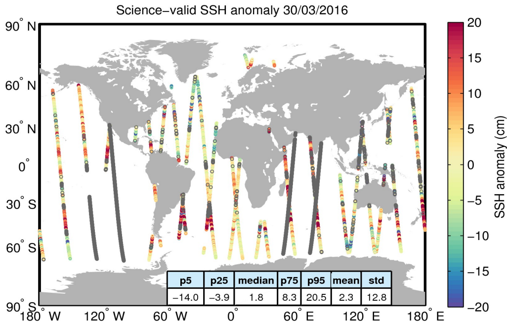
Figure 10. Geographical distribution of science-valid SSH anomaly data over oceans and lakes for 30/03/2016. The statistical values shown in the table refer to the SSH anomaly in cm and are calculated over all measurements shown in the figure. Gray circles denote records that have been rejected based on the editing criteria described in Table 2.
