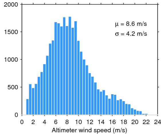
Figure 33. Histogram of flag-valid wind over oceans and lakes for 30/03/2016. The mean ( \mu ) and standard deviation ( \sigma ) are also shown. Note that values larger than 24 m/s are excluded from the histogram for the sake of readability but not from the computation of \mu and \sigma .
