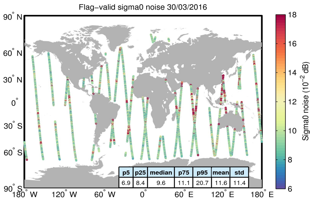
Figure 26. Geographical distribution of flag-valid 20-Hz sigma0 measurement noise over oceans and lakes for 30/03/2016. The statistical values shown in the table refer to the sigma0 noise and are calculated over all measurements shown in the figure.
