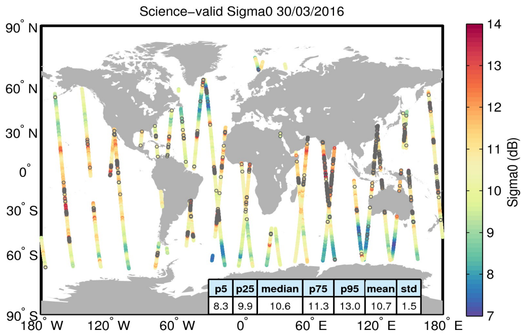
Figure 27. Geographical distribution of science-valid sigma0 data over oceans and lakes for 30/03/2016. The statistical values shown in the table refer to the sigma0 in dB and are calculated over all measurements shown in the figure. Gray circles denote records that have been rejected based on the editing criteria described in Table 4.
