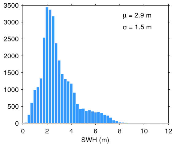
Figure 17. Histogram of flag-valid SWH over oceans and lakes for 30/03/2016. The mean ( \mu ) and standard deviation ( \sigma ) are also shown. Note that values larger than 12 m are excluded from the histogram for the sake of readability but not from the computation of \mu and \sigma .
