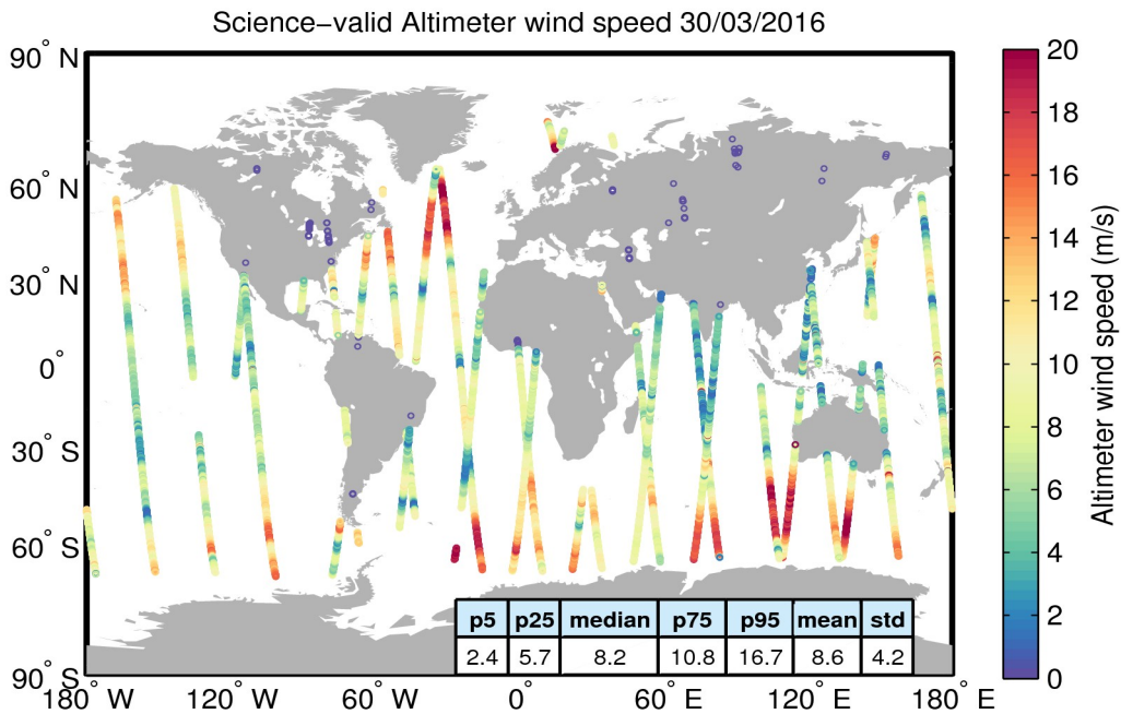
Figure 34. Geographical distribution of science-valid wind data over oceans and lakes for 30/03/2016. The statistical values shown in the table refer to the wind in m/s and are calculated over all measurements shown in the figure. Gray circles denote records that have been rejected based on the editing criteria described in Table 5.
