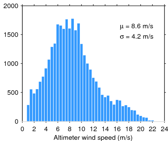
Figure 35. Histogram of science-valid wind over oceans and lakes for 30/03/2016. The mean ( \mu ) and standard deviation ( \sigma ) are also shown. Note that values larger than 24 m/s are excluded from the histogram for the sake of readability but not from the computation of \mu and \sigma .
