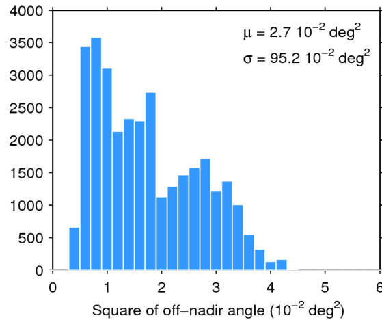
Figure 39. Histogram of flag-valid mispointing over oceans and lakes for 30/03/2016. The mean ( \mu ) and standard deviation ( \sigma ) are also shown. Note that values larger than 6 \cdot 10^{-2} \text{ deg}^2 are excluded from the histogram for the sake of readability but not from the computation of \mu and \sigma .
