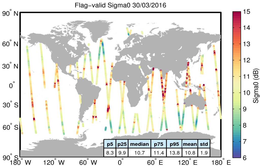
Figure 23. Geographical distribution of flag-valid sigma0 data over oceans and lakes for 30/03/2016. The statistical values shown in the table refer to the sigma0 in dB and are calculated over all measurements shown in the figure.
