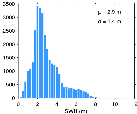
Figure 20. Histogram of science-valid SWH over oceans and lakes for 30/03/2016. The mean ( \mu ) and standard deviation ( \sigma ) are also shown. Note that values larger than 12 m are excluded from the histogram for the sake of readability but not from the computation of \mu and \sigma .
