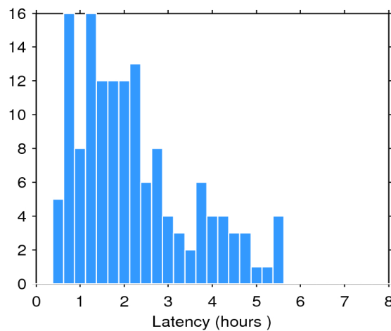
Figure 2. Histogram of the data latency for 30/03/2016. The y-axis denotes the number of files that are made available with a delay of x-hours with respect to the mean time of the records stored in the file.
