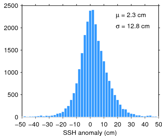
Figure 11. Histogram of science-valid SSH anomaly over oceans and lakes for 30/03/2016. The mean ( \mu ) and standard deviation ( \sigma ) are also shown. Note that values outside [-50 50] cm are excluded from the histogram for the sake of readability but not from the computation of \mu and \sigma .
