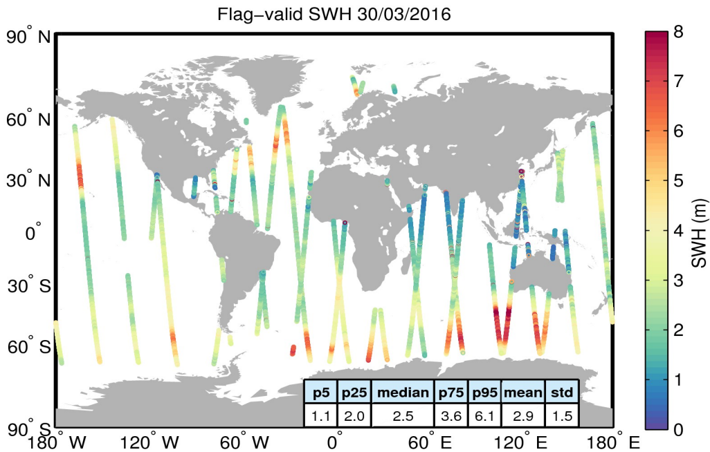
Figure 15. Geographical distribution of flag-valid SWH data over oceans and lakes for 30/03/2016. The statistical values shown in the table refer to the SWH in m and are calculated over all measurements shown in the figure.
