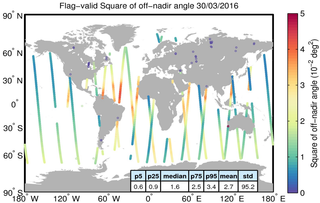
Figure 37. Geographical distribution of flag-valid mispointing data over oceans and lakes for 30/03/2016. The statistical values shown in the table refer to the mispointing in 10^{-2} \text{deg}^2 and are calculated over all measurements shown in the figure.
