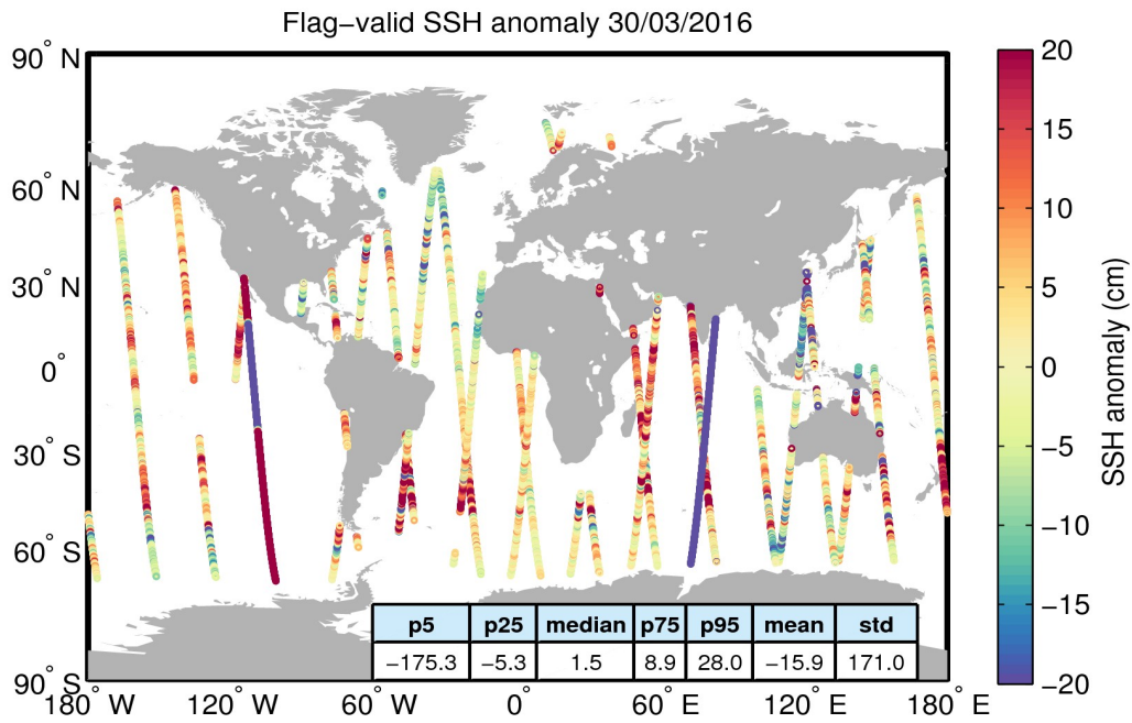
Figure 5. Geographical distribution of flag-valid 1-Hz SSH anomaly data over oceans and lakes for 30/03/2016. The statistical values shown in the table refer to the SSH anomaly in cm and are calculated over all measurements shown in the figure.
