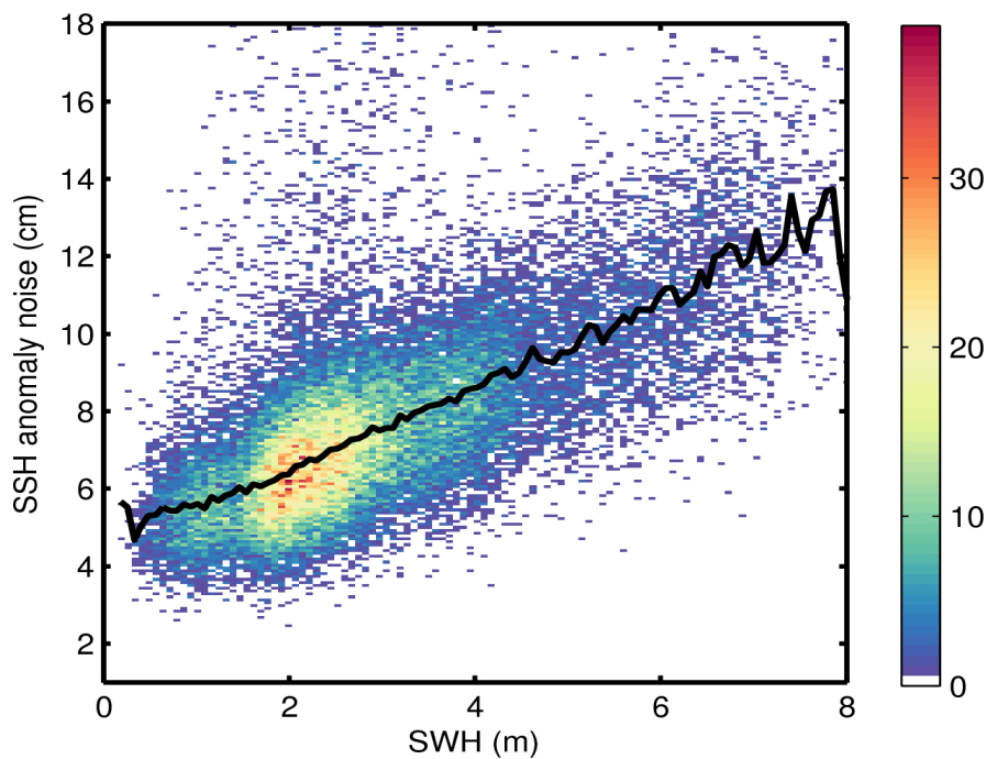
Figure 9. 2D histogram showing flag-valid SSH anomaly noise as a function of SWH for 30/03/2016. The black line denotes the median SSH anomaly noise as a function of SWH.
