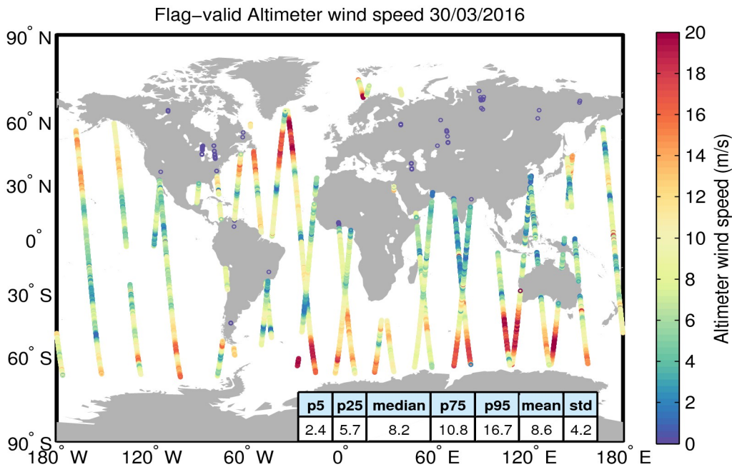
Figure 31. Geographical distribution of flag-valid wind data over oceans and lakes for 30/03/2016. The statistical values shown in the table refer to the wind in m/s and are calculated over all measurements shown in the figure.
