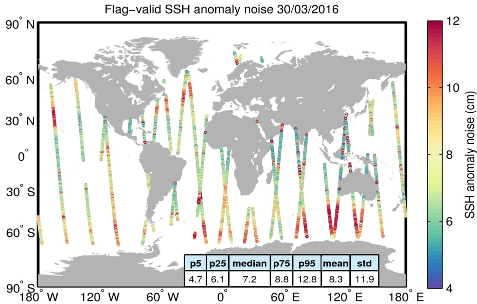
Figure 8. Geographical distribution of flag-valid 20-Hz SSH anomaly measurement noise over oceans and lakes for 30/03/2016. The statistical values shown in the table refer to the SSH anomaly noise and are calculated over all measurements shown in the figure.
