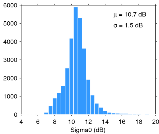
Figure 28. Histogram of science-valid sigma0 over oceans and lakes for 30/03/2016. The mean ( \mu ) and standard deviation ( \sigma ) are also shown. Note that values outside [4 20] dB are excluded from the histogram for the sake of readability but not from the computation of \mu and \sigma .
