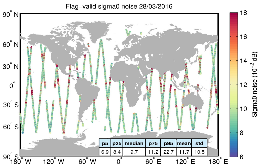
Figure 26. Geographical distribution of flag-valid 20-Hz sigma0 measurement noise over oceans and lakes for 28/03/2016. The statistical values shown in the table refer to the sigma0 noise and are calculated over all measurements shown in the figure.
