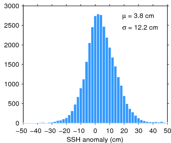
Figure 11. Histogram of science-valid SSH anomaly over oceans and lakes for 28/03/2016. The mean ( \mu ) and standard deviation ( \sigma ) are also shown. Note that values outside [-50 50] cm are excluded from the histogram for the sake of readability but not from the computation of \mu and \sigma .
