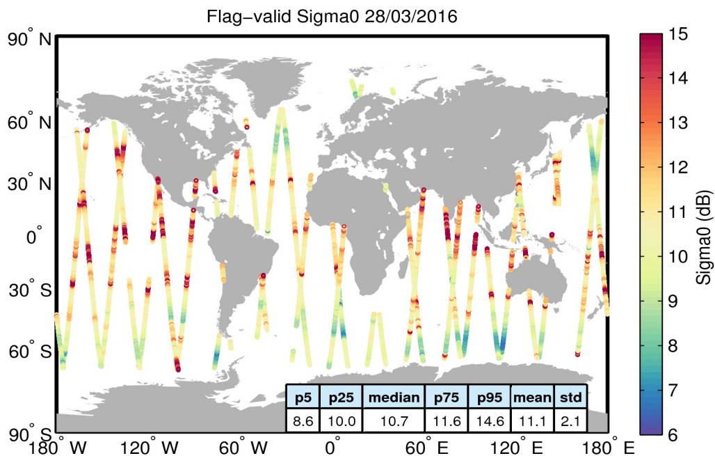
Figure 23. Geographical distribution of flag-valid sigma0 data over oceans and lakes for 28/03/2016. The statistical values shown in the table refer to the sigma0 in dB and are calculated over all measurements shown in the figure.
