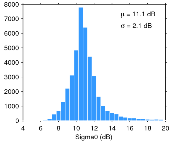
Figure 25. Histogram of flag-valid sigma0 over oceans and lakes for 28/03/2016. The mean ( \mu ) and standard deviation ( \sigma ) are also shown. Note that values outside [4 20] dB are excluded from the histogram for the sake of readability but not from the computation of \mu and \sigma .
