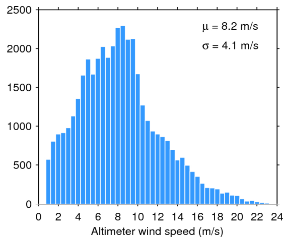
Figure 35. Histogram of science-valid wind over oceans and lakes for 28/03/2016. The mean ( \mu ) and standard deviation ( \sigma ) are also shown. Note that values larger than 24 m/s are excluded from the histogram for the sake of readability but not from the computation of \mu and \sigma .
