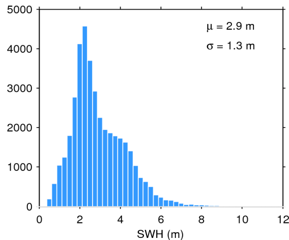
Figure 20. Histogram of science-valid SWH over oceans and lakes for 28/03/2016. The mean ( \mu ) and standard deviation ( \sigma ) are also shown. Note that values larger than 12 m are excluded from the histogram for the sake of readability but not from the computation of \mu and \sigma .
