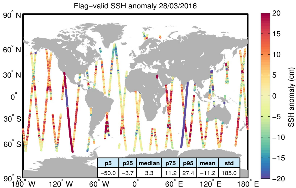
Figure 5. Geographical distribution of flag-valid 1-Hz SSH anomaly data over oceans and lakes for 28/03/2016. The statistical values shown in the table refer to the SSH anomaly in cm and are calculated over all measurements shown in the figure.
