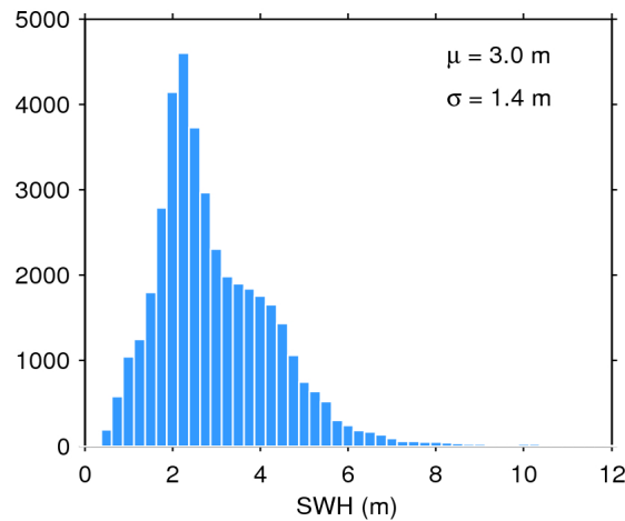
Figure 17. Histogram of flag-valid SWH over oceans and lakes for 28/03/2016. The mean ( \mu ) and standard deviation ( \sigma ) are also shown. Note that values larger than 12 m are excluded from the histogram for the sake of readability but not from the computation of \mu and \sigma .
