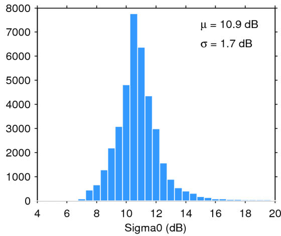
Figure 28. Histogram of science-valid sigma0 over oceans and lakes for 28/03/2016. The mean ( \mu ) and standard deviation ( \sigma ) are also shown. Note that values outside [4 20] dB are excluded from the histogram for the sake of readability but not from the computation of \mu and \sigma .
