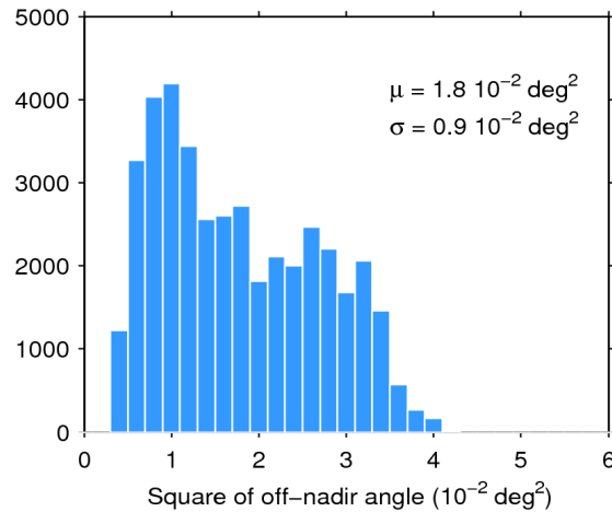
Figure 39. Histogram of flag-valid mispointing over oceans and lakes for 28/03/2016. The mean ( \mu ) and standard deviation ( \sigma ) are also shown. Note that values larger than 6 \cdot 10^{-2} \text{ deg}^2 are excluded from the histogram for the sake of readability but not from the computation of \mu and \sigma .
