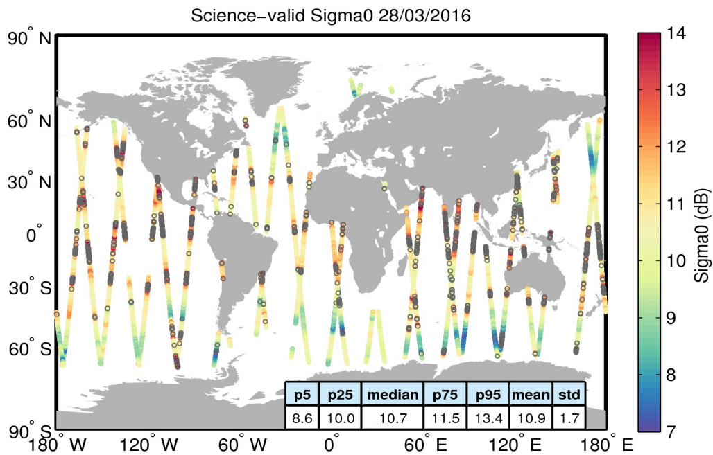
Figure 27. Geographical distribution of science-valid sigma0 data over oceans and lakes for 28/03/2016. The statistical values shown in the table refer to the sigma0 in dB and are calculated over all measurements shown in the figure. Gray circles denote records that have been rejected based on the editing criteria described in Table 4.
