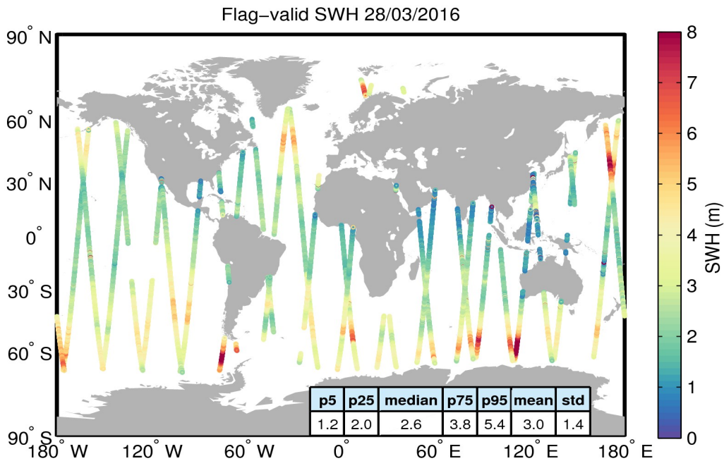
Figure 15. Geographical distribution of flag-valid SWH data over oceans and lakes for 28/03/2016. The statistical values shown in the table refer to the SWH in m and are calculated over all measurements shown in the figure.
