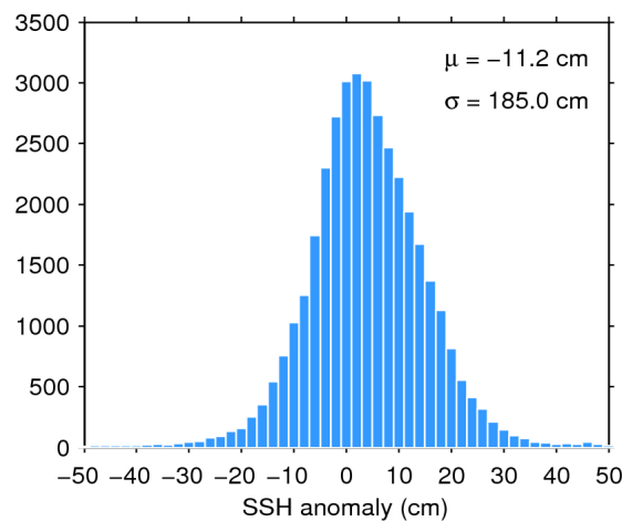
Figure 7. Histogram of flag-valid SSH anomaly over oceans and lakes for 28/03/2016. The mean ( \mu ) and standard deviation ( \sigma ) are also shown. Note that values outside [-50 50] cm are excluded from the histogram for the sake of readability but not from the computation of \mu and \sigma .
