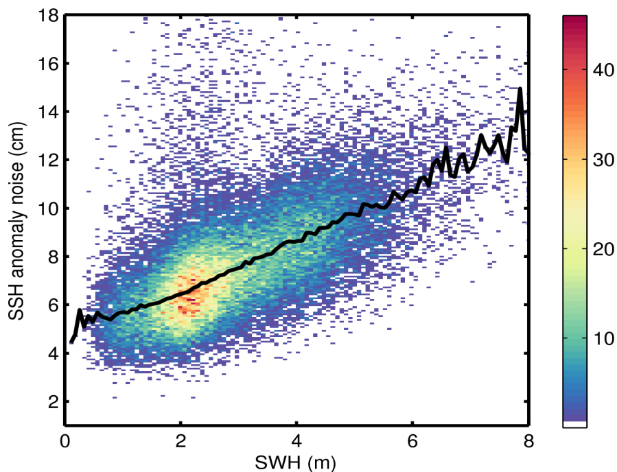
Figure 9. 2D histogram showing flag-valid SSH anomaly noise as a function of SWH for 28/03/2016. The black line denotes the median SSH anomaly noise as a function of SWH.
