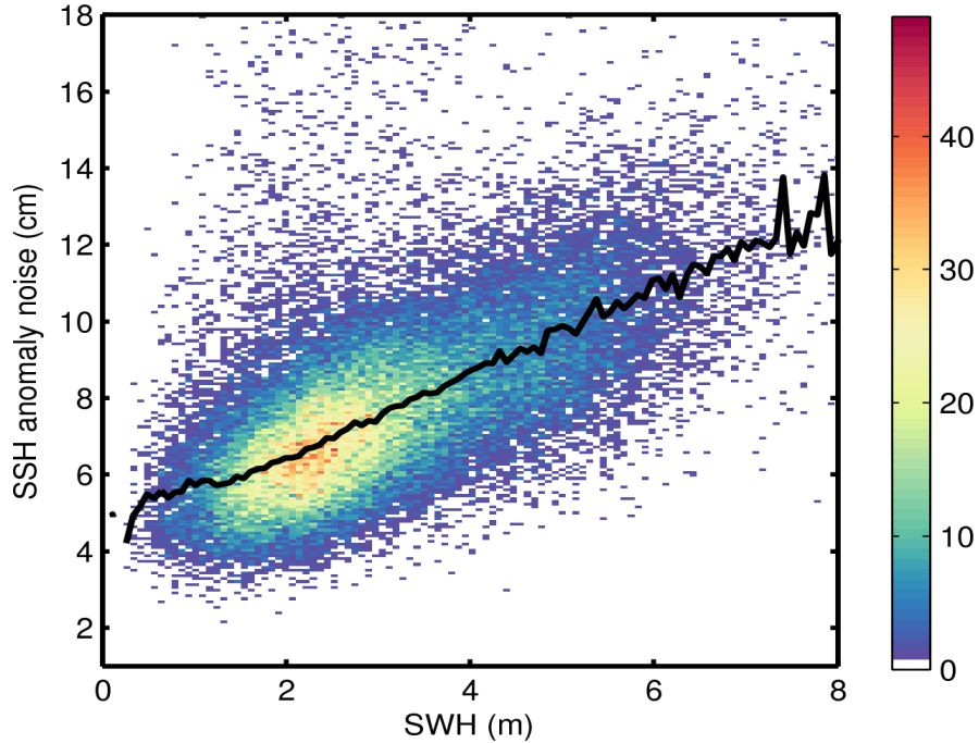
Figure 9. 2D histogram showing flag-valid SSH anomaly noise as a function of SWH for 27/03/2016. The black line denotes the median SSH anomaly noise as a function of SWH.
