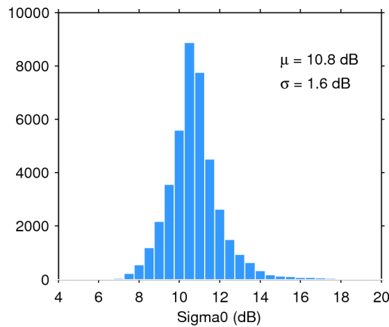
Figure 28. Histogram of science-valid sigma0 over oceans and lakes for 27/03/2016. The mean ( \mu ) and standard deviation ( \sigma ) are also shown. Note that values outside [4 20] dB are excluded from the histogram for the sake of readability but not from the computation of \mu and \sigma .
