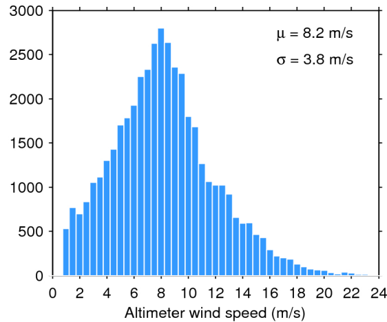
Figure 33. Histogram of flag-valid wind over oceans and lakes for 27/03/2016. The mean ( \mu ) and standard deviation ( \sigma ) are also shown. Note that values larger than 24 m/s are excluded from the histogram for the sake of readability but not from the computation of \mu and \sigma .
