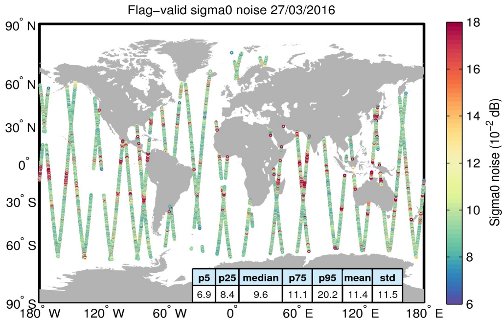
Figure 26. Geographical distribution of flag-valid 20-Hz sigma0 measurement noise over oceans and lakes for 27/03/2016. The statistical values shown in the table refer to the sigma0 noise and are calculated over all measurements shown in the figure.
