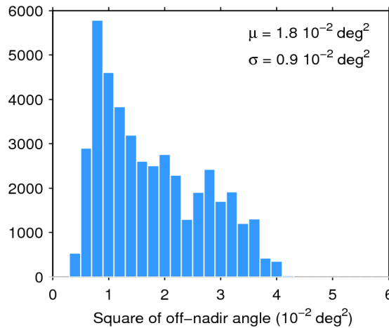
Figure 39. Histogram of flag-valid mispointing over oceans and lakes for 27/03/2016. The mean ( \mu ) and standard deviation ( \sigma ) are also shown. Note that values larger than 6 \cdot 10^{-2} \text{ deg}^2 are excluded from the histogram for the sake of readability but not from the computation of \mu and \sigma .
