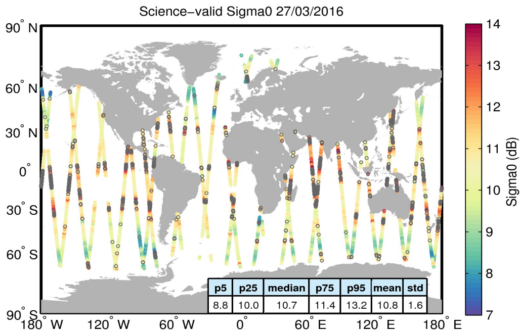
Figure 27. Geographical distribution of science-valid sigma0 data over oceans and lakes for 27/03/2016. The statistical values shown in the table refer to the sigma0 in dB and are calculated over all measurements shown in the figure. Gray circles denote records that have been rejected based on the editing criteria described in Table 4.
