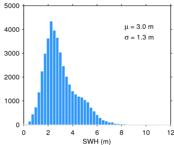
Figure 20. Histogram of science-valid SWH over oceans and lakes for 27/03/2016. The mean ( \mu ) and standard deviation ( \sigma ) are also shown. Note that values larger than 12 m are excluded from the histogram for the sake of readability but not from the computation of \mu and \sigma .
