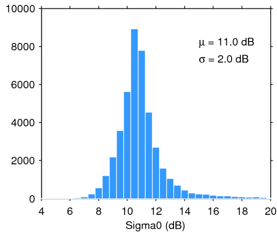
Figure 25. Histogram of flag-valid sigma0 over oceans and lakes for 27/03/2016. The mean ( \mu ) and standard deviation ( \sigma ) are also shown. Note that values outside [4 20] dB are excluded from the histogram for the sake of readability but not from the computation of \mu and \sigma .
