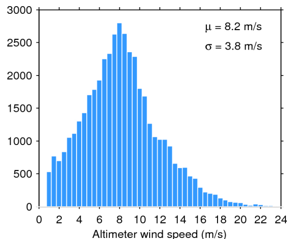
Figure 35. Histogram of science-valid wind over oceans and lakes for 27/03/2016. The mean ( \mu ) and standard deviation ( \sigma ) are also shown. Note that values larger than 24 m/s are excluded from the histogram for the sake of readability but not from the computation of \mu and \sigma .
