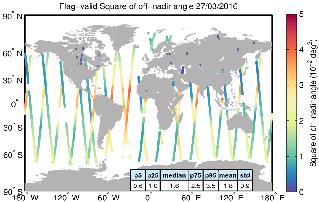
Figure 37. Geographical distribution of flag-valid mispointing data over oceans and lakes for 27/03/2016. The statistical values shown in the table refer to the mispointing in 10^{-2} \text{deg}^2 and are calculated over all measurements shown in the figure.
