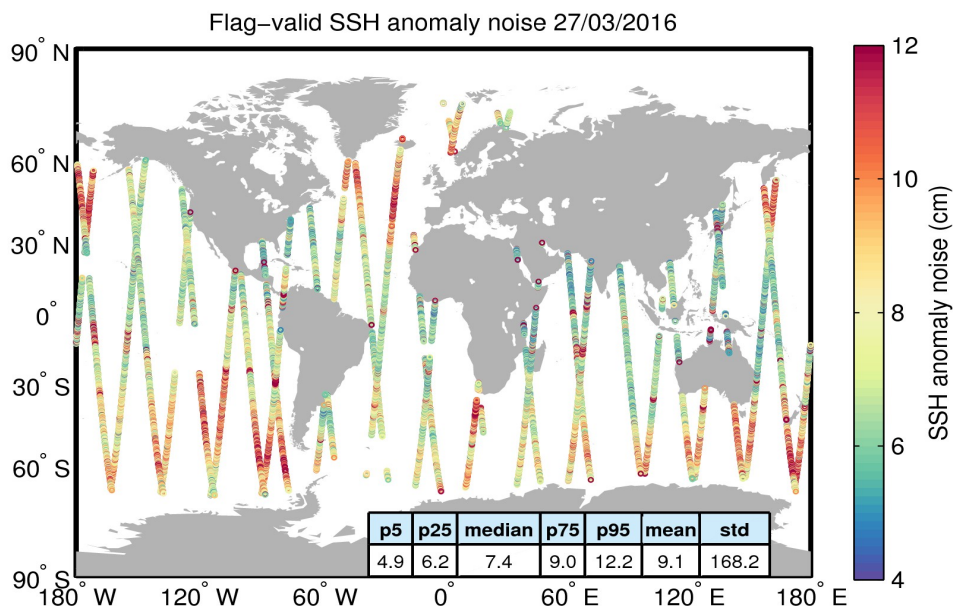
Figure 8. Geographical distribution of flag-valid 20-Hz SSH anomaly measurement noise over oceans and lakes for 27/03/2016. The statistical values shown in the table refer to the SSH anomaly noise and are calculated over all measurements shown in the figure.
