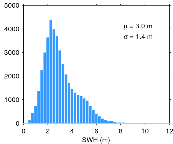
Figure 17. Histogram of flag-valid SWH over oceans and lakes for 27/03/2016. The mean ( \mu ) and standard deviation ( \sigma ) are also shown. Note that values larger than 12 m are excluded from the histogram for the sake of readability but not from the computation of \mu and \sigma .
