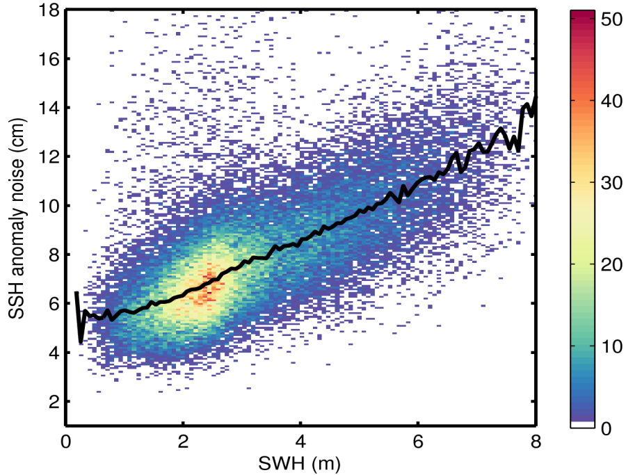
Figure 9. 2D histogram showing flag-valid SSH anomaly noise as a function of SWH for 26/03/2016. The black line denotes the median SSH anomaly noise as a function of SWH.
