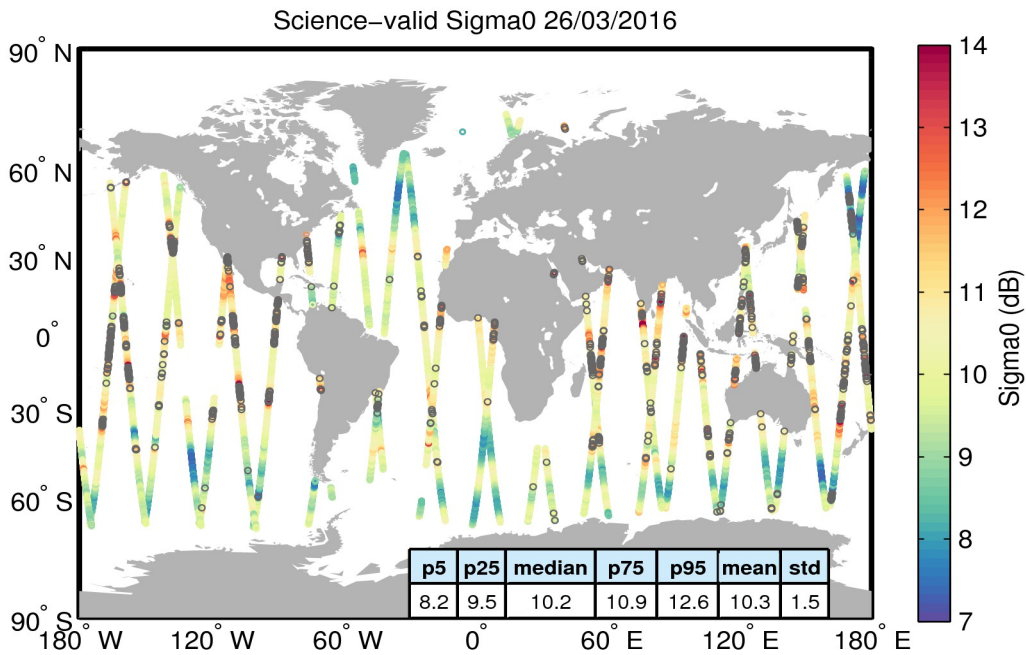
Figure 27. Geographical distribution of science-valid sigma0 data over oceans and lakes for 26/03/2016. The statistical values shown in the table refer to the sigma0 in dB and are calculated over all measurements shown in the figure. Gray circles denote records that have been rejected based on the editing criteria described in Table 4.
