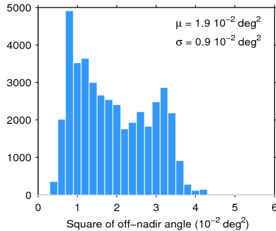
Figure 39. Histogram of flag-valid mispointing over oceans and lakes for 26/03/2016. The mean ( \mu ) and standard deviation ( \sigma ) are also shown. Note that values larger than 6 \cdot 10^{-2} \text{ deg}^2 are excluded from the histogram for the sake of readability but not from the computation of \mu and \sigma .
