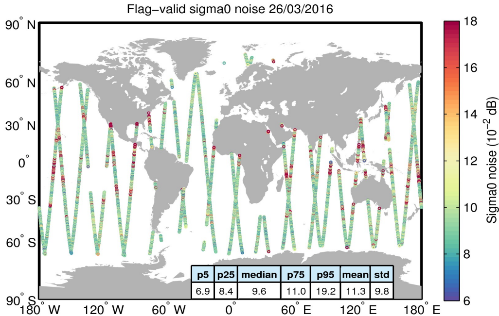
Figure 26. Geographical distribution of flag-valid 20-Hz sigma0 measurement noise over oceans and lakes for 26/03/2016. The statistical values shown in the table refer to the sigma0 noise and are calculated over all measurements shown in the figure.
