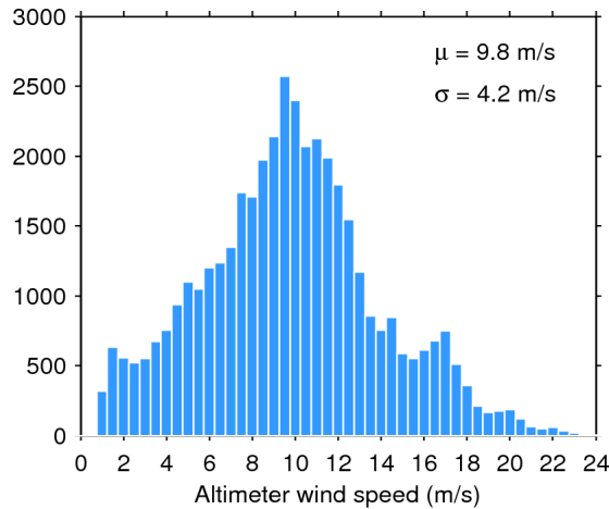
Figure 33. Histogram of flag-valid wind over oceans and lakes for 26/03/2016. The mean ( \mu ) and standard deviation ( \sigma ) are also shown. Note that values larger than 24 m/s are excluded from the histogram for the sake of readability but not from the computation of \mu and \sigma .
