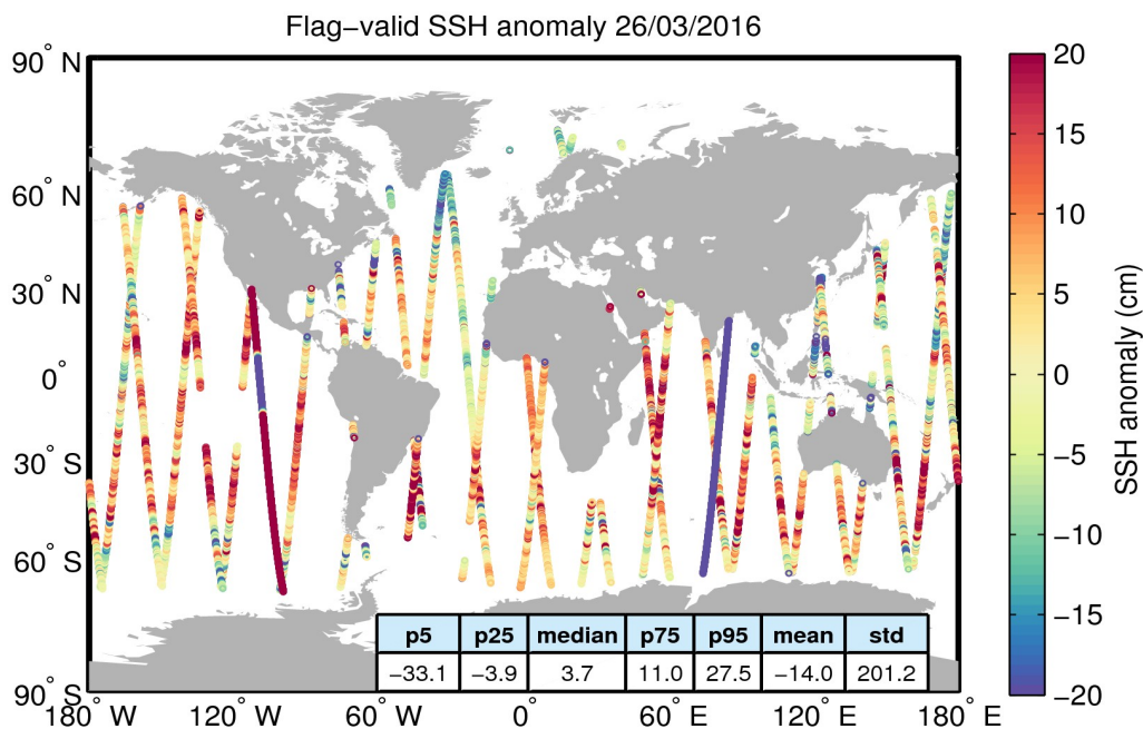
Figure 5. Geographical distribution of flag-valid 1-Hz SSH anomaly data over oceans and lakes for 26/03/2016. The statistical values shown in the table refer to the SSH anomaly in cm and are calculated over all measurements shown in the figure.
