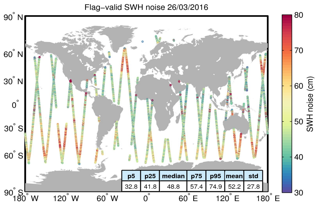
Figure 18. Geographical distribution of flag-valid 20-Hz SWH measurement noise over oceans and lakes for 26/03/2016. The statistical values shown in the table refer to the SWH noise and are calculated over all measurements shown in the figure.
