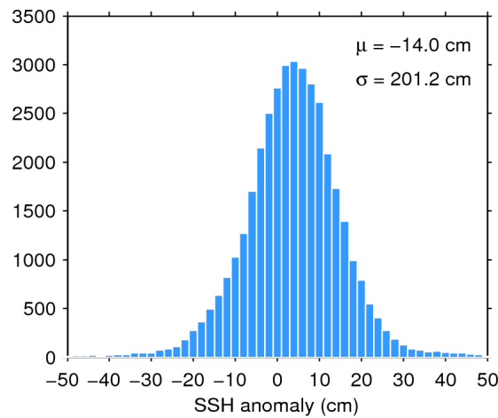
Figure 7. Histogram of flag-valid SSH anomaly over oceans and lakes for 26/03/2016. The mean ( \mu ) and standard deviation ( \sigma ) are also shown. Note that values outside [-50\ 50] cm are excluded from the histogram for the sake of readability but not from the computation of \mu and \sigma .
