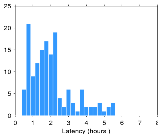
Figure 2. Histogram of the data latency for 26/03/2016. The y-axis denotes the number of files that are made available with a delay of x-hours with respect to the mean time of the records stored in the file.
