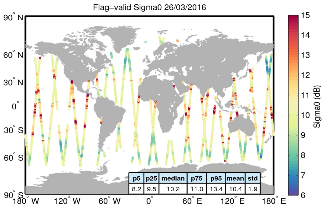
Figure 23. Geographical distribution of flag-valid sigma0 data over oceans and lakes for 26/03/2016. The statistical values shown in the table refer to the sigma0 in dB and are calculated over all measurements shown in the figure.
