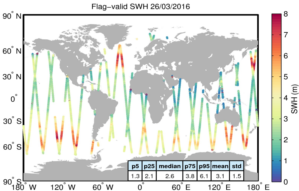
Figure 15. Geographical distribution of flag-valid SWH data over oceans and lakes for 26/03/2016. The statistical values shown in the table refer to the SWH in m and are calculated over all measurements shown in the figure.
