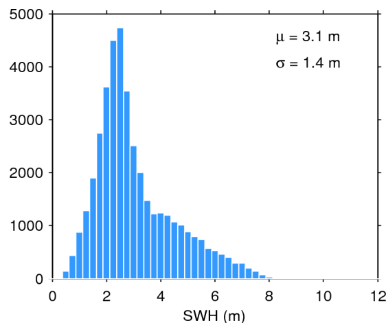
Figure 20. Histogram of science-valid SWH over oceans and lakes for 26/03/2016. The mean ( \mu ) and standard deviation ( \sigma ) are also shown. Note that values larger than 12 m are excluded from the histogram for the sake of readability but not from the computation of \mu and \sigma .
