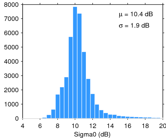
Figure 25. Histogram of flag-valid sigma0 over oceans and lakes for 26/03/2016. The mean ( \mu ) and standard deviation ( \sigma ) are also shown. Note that values outside [4 20] dB are excluded from the histogram for the sake of readability but not from the computation of \mu and \sigma .
