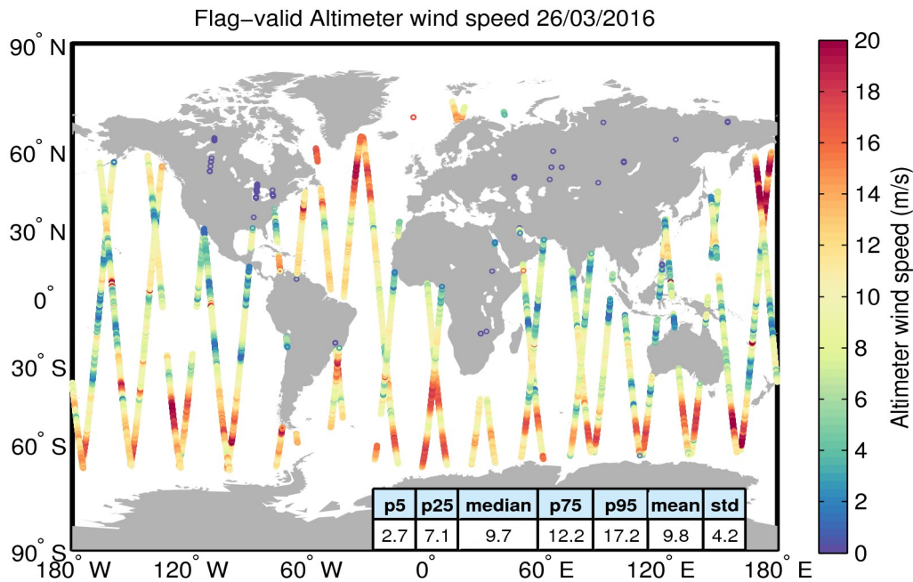
Figure 31. Geographical distribution of flag-valid wind data over oceans and lakes for 26/03/2016. The statistical values shown in the table refer to the wind in m/s and are calculated over all measurements shown in the figure.
