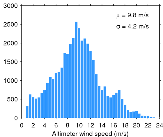
Figure 35. Histogram of science-valid wind over oceans and lakes for 26/03/2016. The mean ( \mu ) and standard deviation ( \sigma ) are also shown. Note that values larger than 24 m/s are excluded from the histogram for the sake of readability but not from the computation of \mu and \sigma .
