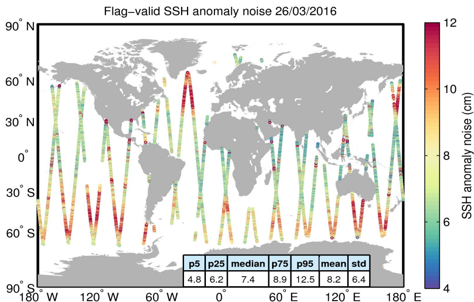
Figure 8. Geographical distribution of flag-valid 20-Hz SSH anomaly measurement noise over oceans and lakes for 26/03/2016. The statistical values shown in the table refer to the SSH anomaly noise and are calculated over all measurements shown in the figure.
