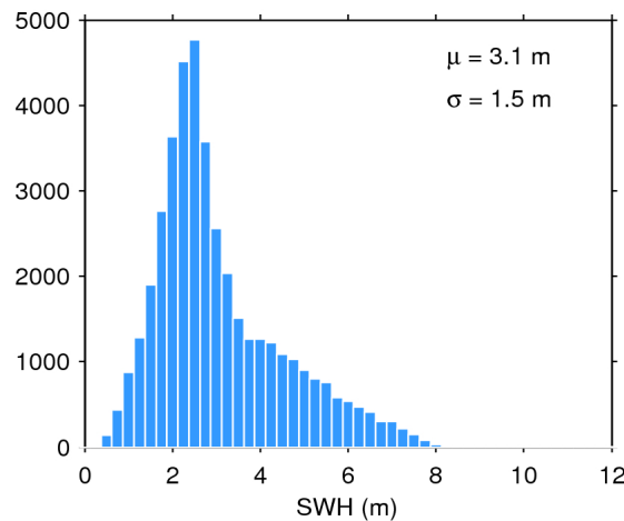
Figure 17. Histogram of flag-valid SWH over oceans and lakes for 26/03/2016. The mean ( \mu ) and standard deviation ( \sigma ) are also shown. Note that values larger than 12 m are excluded from the histogram for the sake of readability but not from the computation of \mu and \sigma .
