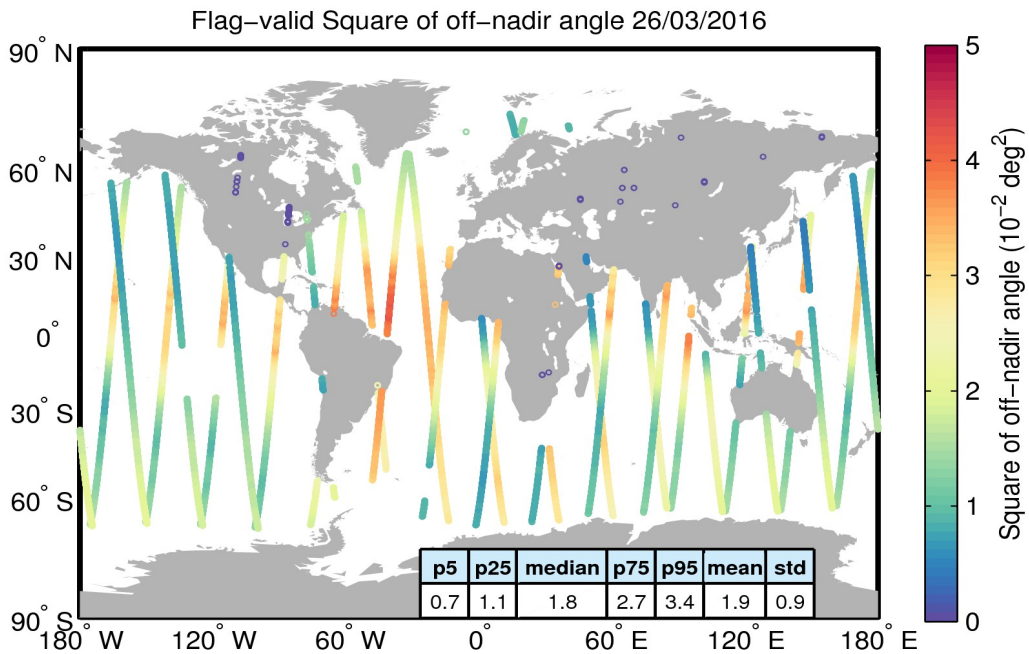
Figure 37. Geographical distribution of flag-valid mispointing data over oceans and lakes for 26/03/2016. The statistical values shown in the table refer to the mispointing in 10^{-2} deg 2 and are calculated over all measurements shown in the figure.
