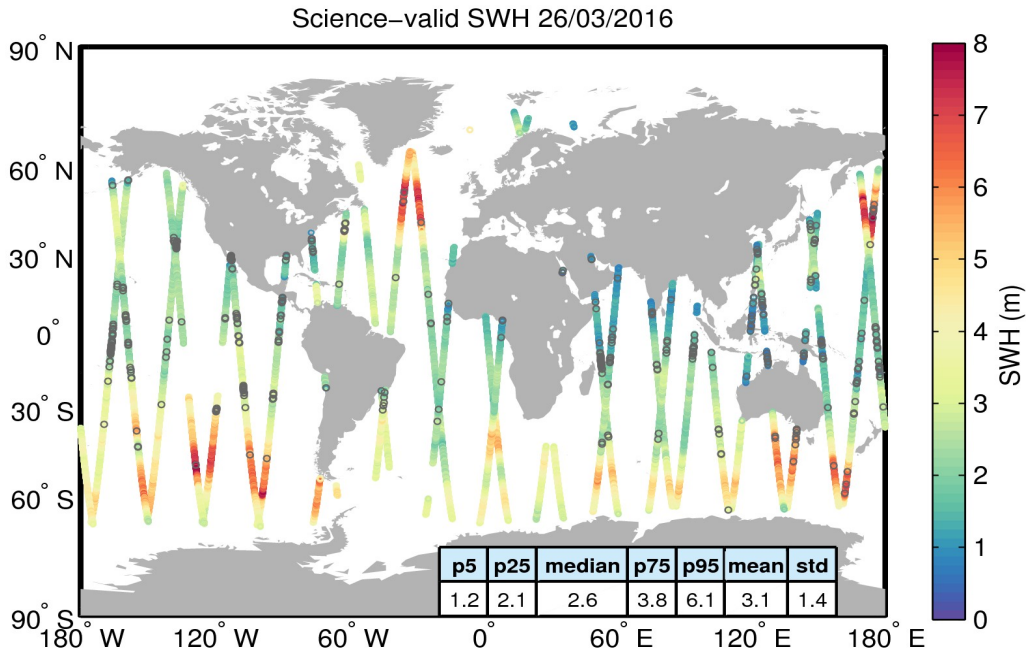
Figure 19. Geographical distribution of science-valid SWH data over oceans and lakes for 26/03/2016. The statistical values shown in the table refer to the SWH in m and are calculated over all measurements shown in the figure. Gray circles denote records that have been rejected based on the editing criteria described in Table 3.
