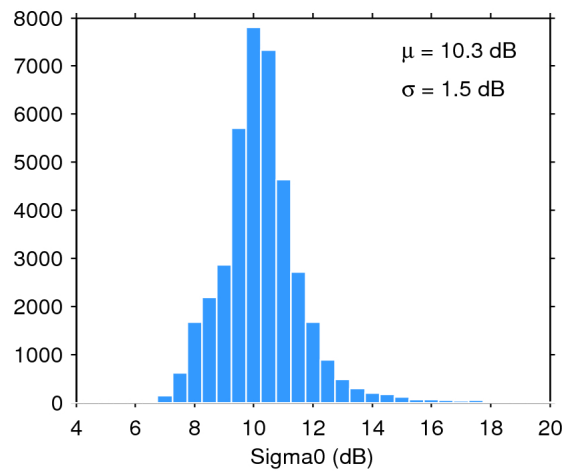
Figure 28. Histogram of science-valid sigma0 over oceans and lakes for 26/03/2016. The mean ( \mu ) and standard deviation ( \sigma ) are also shown. Note that values outside [4 20] dB are excluded from the histogram for the sake of readability but not from the computation of \mu and \sigma .
