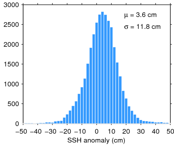
Figure 11. Histogram of science-valid SSH anomaly over oceans and lakes for 26/03/2016. The mean ( \mu ) and standard deviation ( \sigma ) are also shown. Note that values outside [-50 50] cm are excluded from the histogram for the sake of readability but not from the computation of \mu and \sigma .
