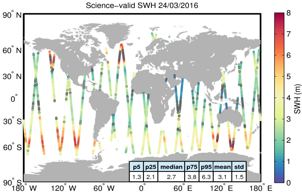
Figure 19. Geographical distribution of science-valid SWH data over oceans and lakes for 24/03/2016. The statistical values shown in the table refer to the SWH in m and are calculated over all measurements shown in the figure. Gray circles denote records that have been rejected based on the editing criteria described in Table 3.
