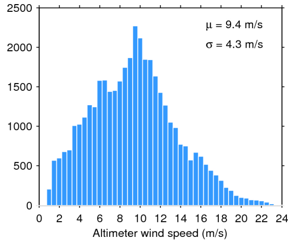
Figure 33. Histogram of flag-valid wind over oceans and lakes for 24/03/2016. The mean ( \mu ) and standard deviation ( \sigma ) are also shown. Note that values larger than 24 m/s are excluded from the histogram for the sake of readability but not from the computation of \mu and \sigma .
