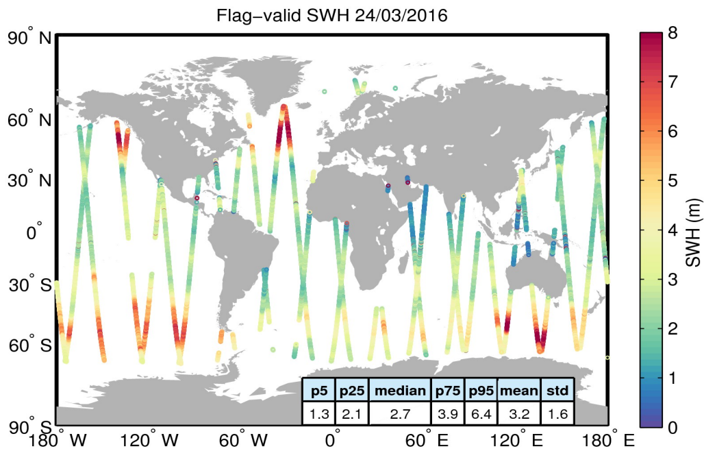
Figure 15. Geographical distribution of flag-valid SWH data over oceans and lakes for 24/03/2016. The statistical values shown in the table refer to the SWH in m and are calculated over all measurements shown in the figure.
