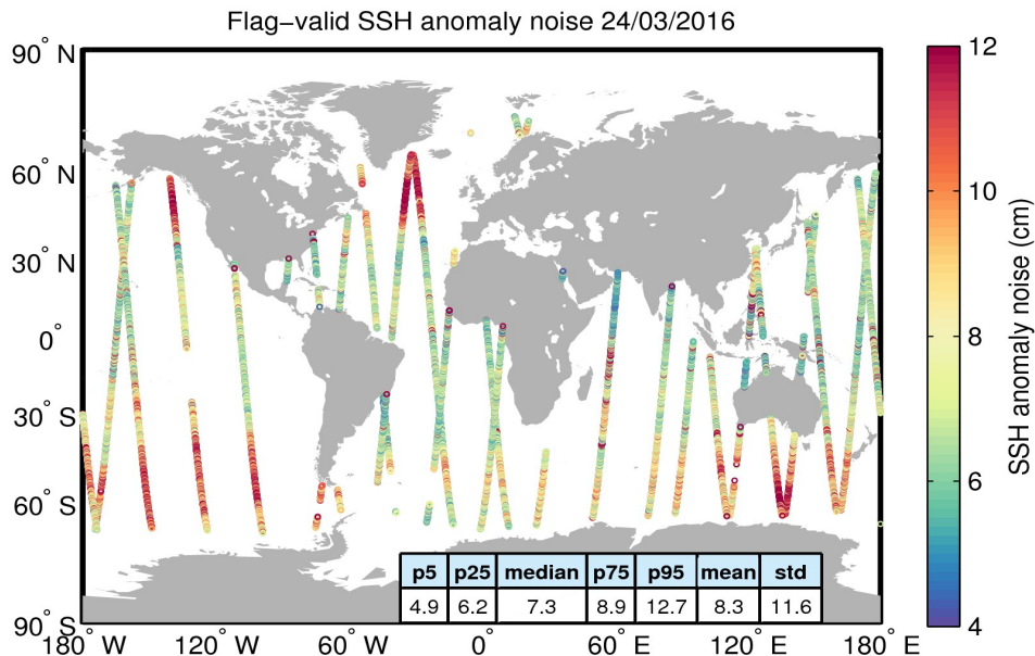
Figure 8. Geographical distribution of flag-valid 20-Hz SSH anomaly measurement noise over oceans and lakes for 24/03/2016. The statistical values shown in the table refer to the SSH anomaly noise and are calculated over all measurements shown in the figure.
