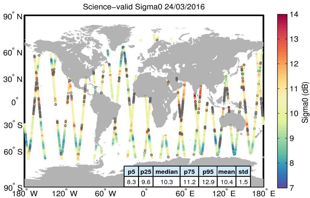
Figure 27. Geographical distribution of science-valid sigma0 data over oceans and lakes for 24/03/2016. The statistical values shown in the table refer to the sigma0 in dB and are calculated over all measurements shown in the figure. Gray circles denote records that have been rejected based on the editing criteria described in Table 4.
