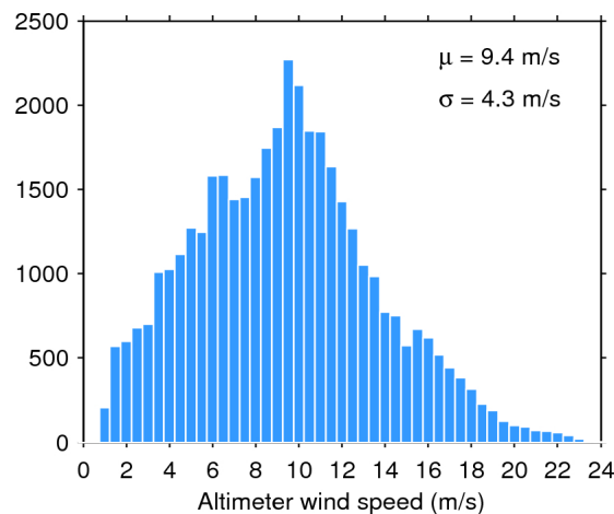
Figure 35. Histogram of science-valid wind over oceans and lakes for 24/03/2016. The mean ( \mu ) and standard deviation ( \sigma ) are also shown. Note that values larger than 24 m/s are excluded from the histogram for the sake of readability but not from the computation of \mu and \sigma .
