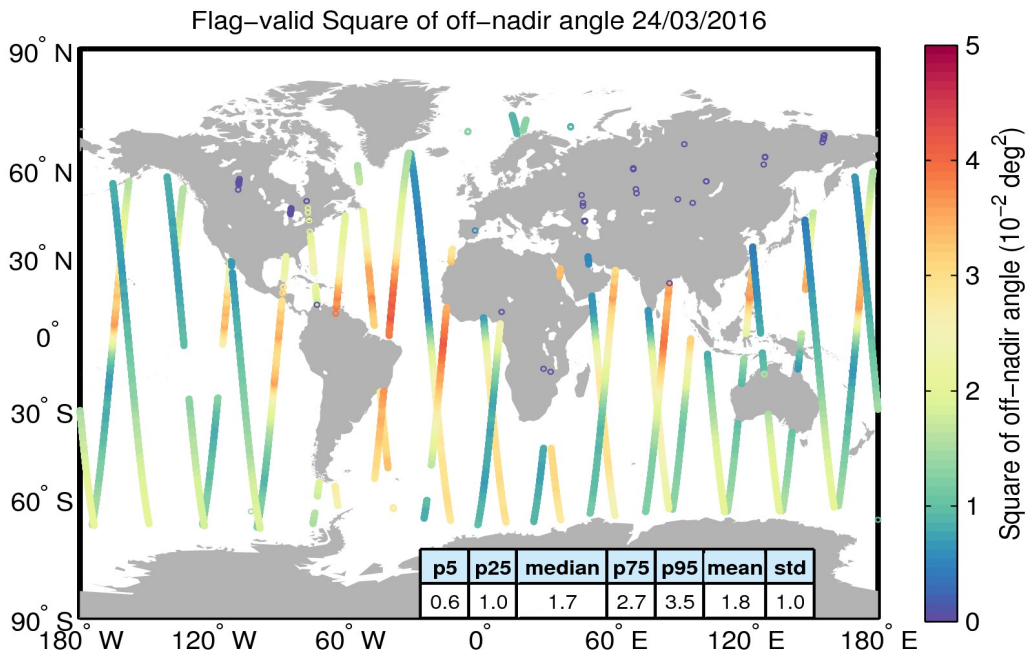
Figure 37. Geographical distribution of flag-valid mispointing data over oceans and lakes for 24/03/2016. The statistical values shown in the table refer to the mispointing in 10^{-2} \text{ deg}^2 and are calculated over all measurements shown in the figure.
