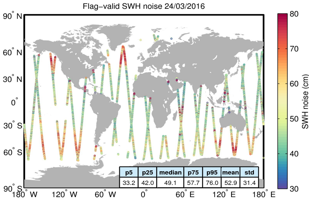
Figure 18. Geographical distribution of flag-valid 20-Hz SWH measurement noise over oceans and lakes for 24/03/2016. The statistical values shown in the figure refer to the SWH noise and are calculated over all measurements shown in the figure.
