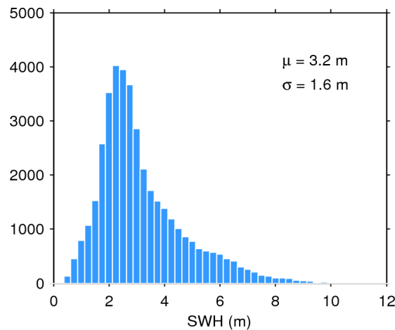
Figure 17. Histogram of flag-valid SWH over oceans and lakes for 24/03/2016. The mean ( \mu ) and standard deviation ( \sigma ) are also shown. Note that values larger than 12 m are excluded from the histogram for the sake of readability but not from the computation of \mu and \sigma .
