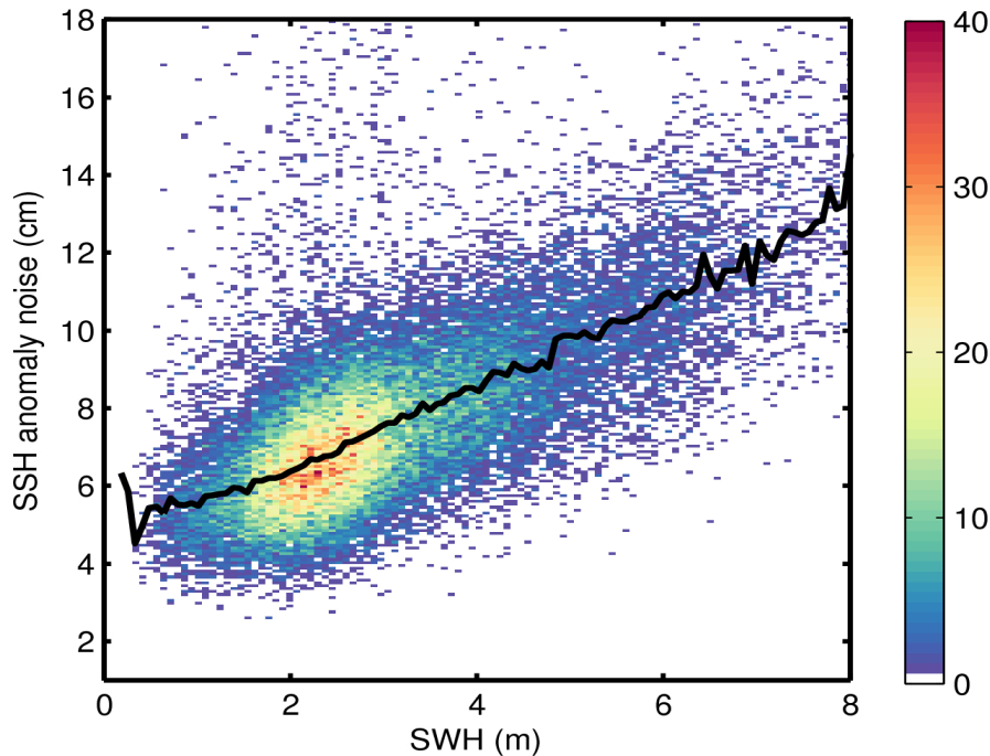
Figure 9. 2D histogram showing flag-valid SSH anomaly noise as a function of SWH for 24/03/2016. The black line denotes the median SSH anomaly noise as a function of SWH.
