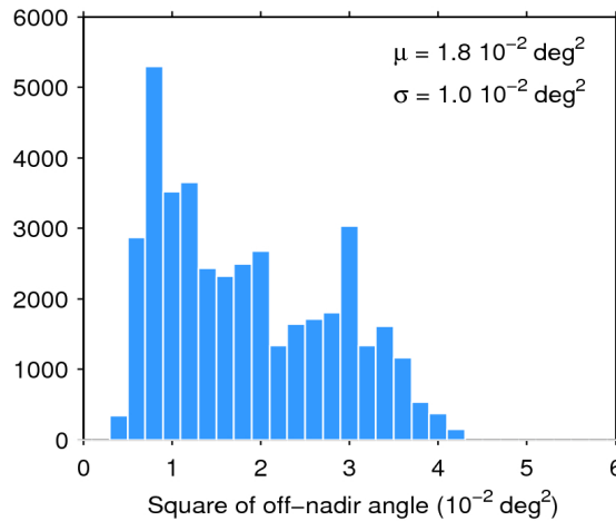
Figure 39. Histogram of flag-valid mispointing over oceans and lakes for 24/03/2016. The mean ( \mu ) and standard deviation ( \sigma ) are also shown. Note that values larger than 6 \cdot 10^{-2} \text{ deg}^2 are excluded from the histogram for the sake of readability but not from the computation of \mu and \sigma .
