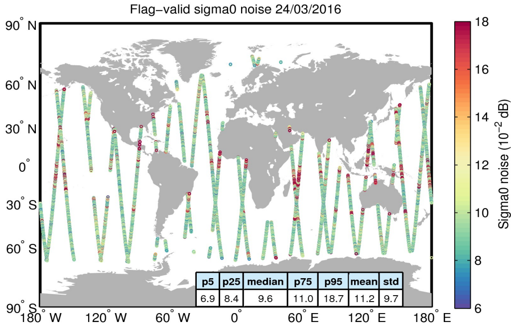
Figure 26. Geographical distribution of flag-valid 20-Hz sigma0 measurement noise over oceans and lakes for 24/03/2016. The statistical values shown in the table refer to the sigma0 noise and are calculated over all measurements shown in the figure.
