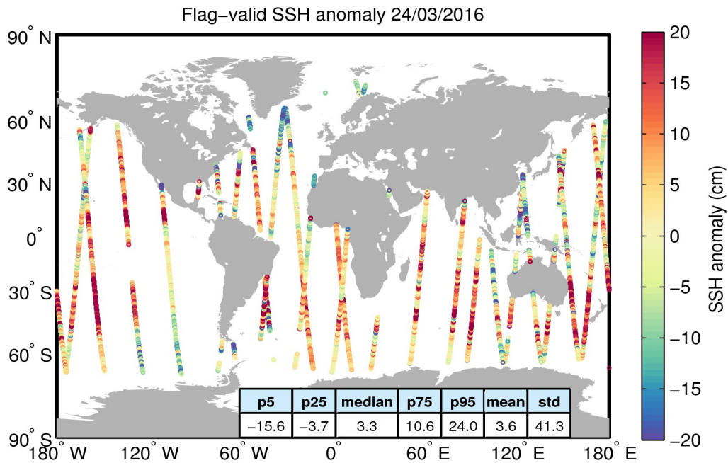
Figure 5. Geographical distribution of flag-valid 1-Hz SSH anomaly data over oceans and lakes for 24/03/2016. The statistical values shown in the table refer to the SSH anomaly in cm and are calculated over all measurements shown in the figure.
