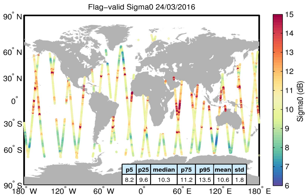
Figure 23. Geographical distribution of flag-valid sigma0 data over oceans and lakes for 24/03/2016. The statistical values shown in the table refer to the sigma0 in dB and are calculated over all measurements shown in the figure.
