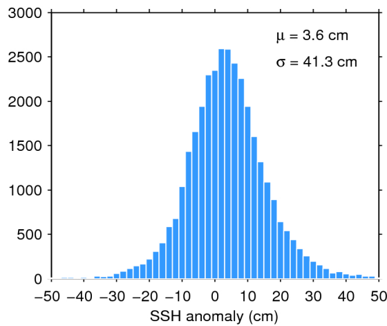
Figure 7. Histogram of flag-valid SSH anomaly over oceans and lakes for 24/03/2016. The mean ( \mu ) and standard deviation ( \sigma ) are also shown. Note that values outside [-50\ 50] cm are excluded from the histogram for the sake of readability but not from the computation of \mu and \sigma .
