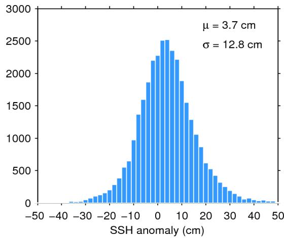
Figure 11. Histogram of science-valid SSH anomaly over oceans and lakes for 24/03/2016. The mean ( \mu ) and standard deviation ( \sigma ) are also shown. Note that values outside [-50 50] cm are excluded from the histogram for the sake of readability but not from the computation of \mu and \sigma .
