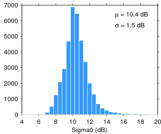
Figure 28. Histogram of science-valid sigma0 over oceans and lakes for 24/03/2016. The mean ( \mu ) and standard deviation ( \sigma ) are also shown. Note that values outside [4 20] dB are excluded from the histogram for the sake of readability but not from the computation of \mu and \sigma .
