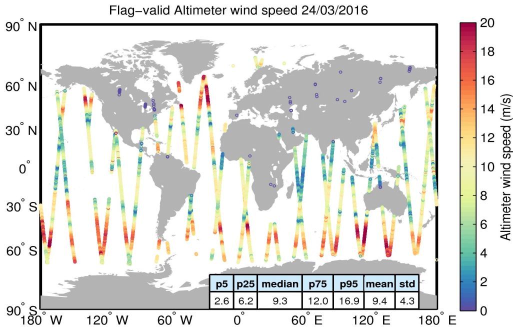
Figure 31. Geographical distribution of flag-valid wind data over oceans and lakes for 24/03/2016. The statistical values shown in the table refer to the wind in m/s and are calculated over all measurements shown in the figure.
