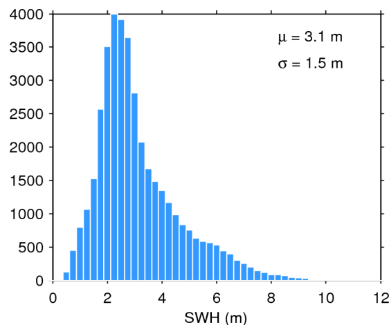
Figure 20. Histogram of science-valid SWH over oceans and lakes for 24/03/2016. The mean ( \mu ) and standard deviation ( \sigma ) are also shown. Note that values larger than 12 m are excluded from the histogram for the sake of readability but not from the computation of \mu and \sigma .
