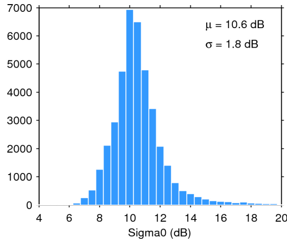
Figure 25. Histogram of flag-valid sigma0 over oceans and lakes for 24/03/2016. The mean ( \mu ) and standard deviation ( \sigma ) are also shown. Note that values outside [4 20] dB are excluded from the histogram for the sake of readability but not from the computation of \mu and \sigma .
