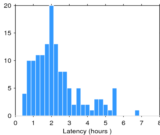
Figure 2. Histogram of the data latency for 24/03/2016. The y-axis denotes the number of files that are made available with a delay of x-hours with respect to the mean time of the records stored in the file.
