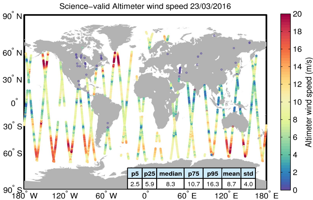
Figure 34. Geographical distribution of science-valid wind data over oceans and lakes for 23/03/2016. The statistical values shown in the table refer to the wind in m/s and are calculated over all measurements shown in the figure. Gray circles denote records that have been rejected based on the editing criteria described in Table 5.
