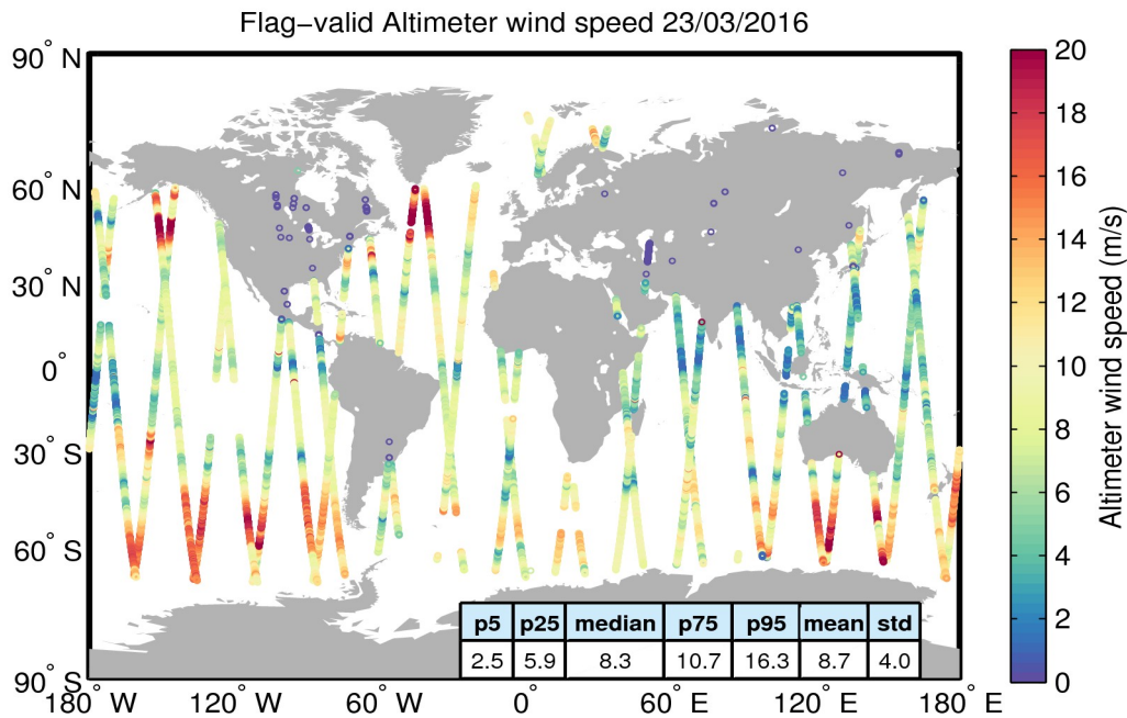
Figure 31. Geographical distribution of flag-valid wind data over oceans and lakes for 23/03/2016. The statistical values shown in the table refer to the wind in m/s and are calculated over all measurements shown in the figure.
