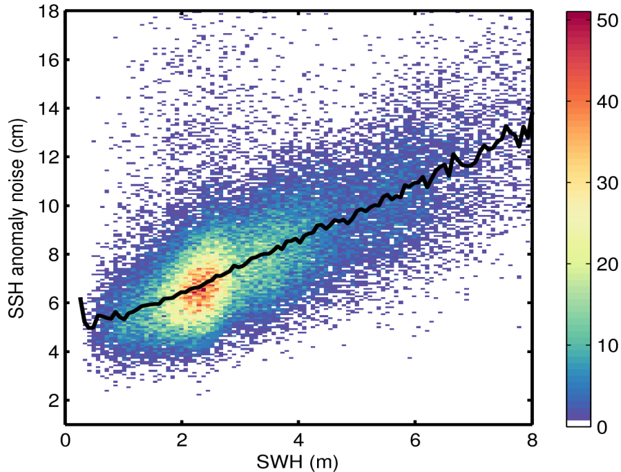
Figure 9. 2D histogram showing flag-valid SSH anomaly noise as a function of SWH for 23/03/2016. The black line denotes the median SSH anomaly noise as a function of SWH.
