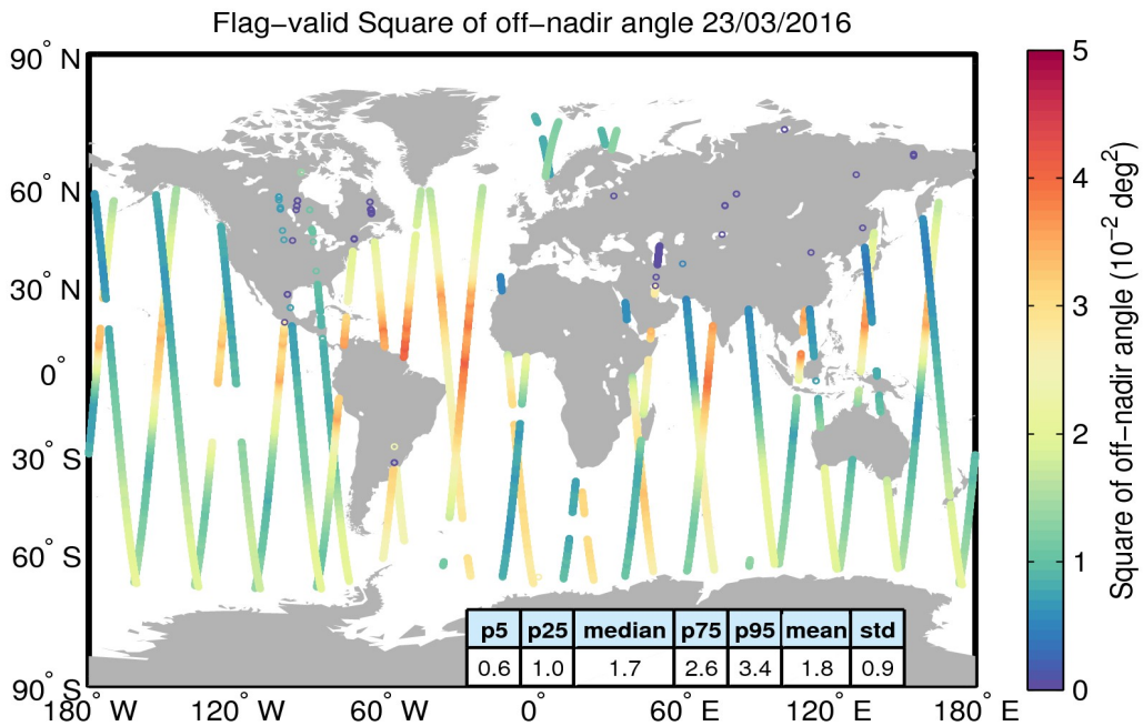
Figure 37. Geographical distribution of flag-valid mispointing data over oceans and lakes for 23/03/2016. The statistical values shown in the table refer to the mispointing in 10^{-2} deg 2 and are calculated over all measurements shown in the figure.
