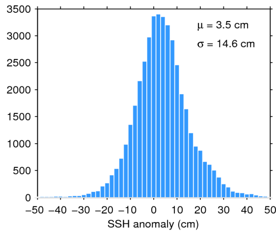
Figure 7. Histogram of flag-valid SSH anomaly over oceans and lakes for 23/03/2016. The mean ( \mu ) and standard deviation ( \sigma ) are also shown. Note that values outside [-50\ 50] cm are excluded from the histogram for the sake of readability but not from the computation of \mu and \sigma .
