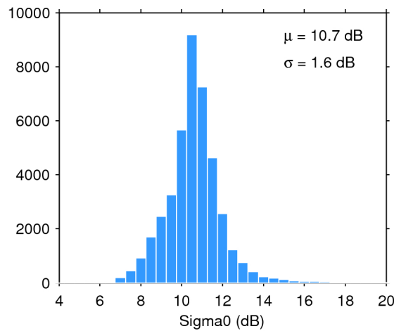
Figure 28. Histogram of science-valid sigma0 over oceans and lakes for 23/03/2016. The mean ( \mu ) and standard deviation ( \sigma ) are also shown. Note that values outside [4 20] dB are excluded from the histogram for the sake of readability but not from the computation of \mu and \sigma .
