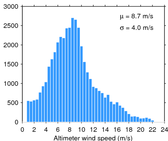
Figure 35. Histogram of science-valid wind over oceans and lakes for 23/03/2016. The mean ( \mu ) and standard deviation ( \sigma ) are also shown. Note that values larger than 24 m/s are excluded from the histogram for the sake of readability but not from the computation of \mu and \sigma .
