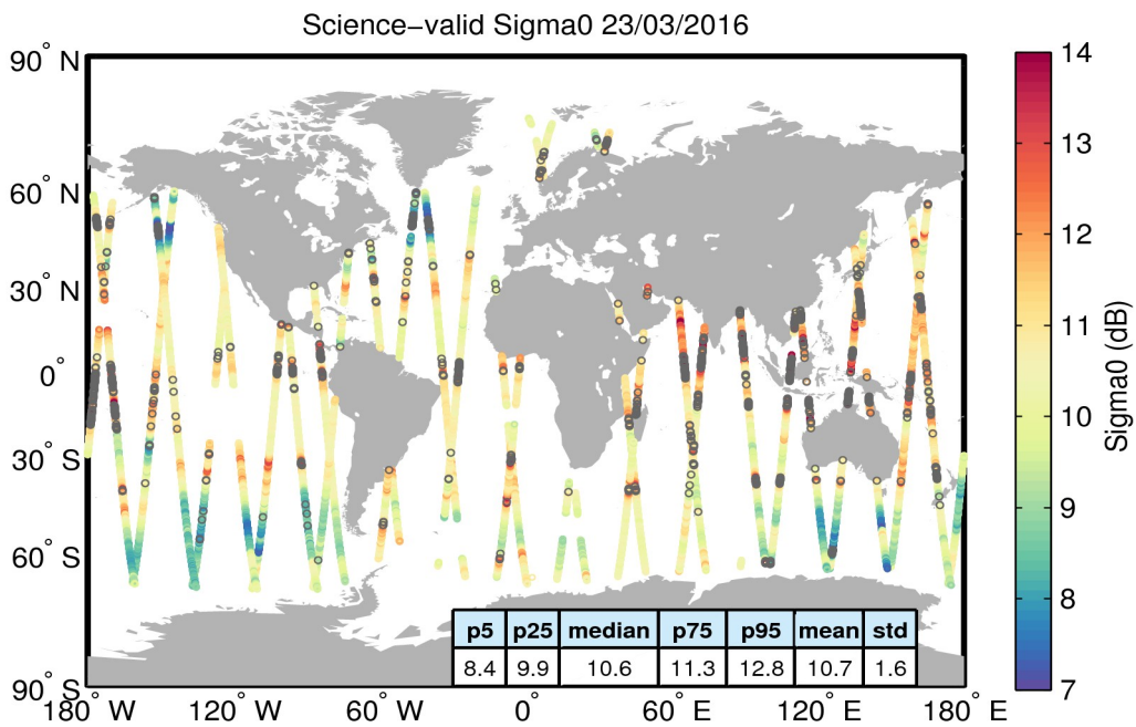
Figure 27. Geographical distribution of science-valid sigma0 data over oceans and lakes for 23/03/2016. The statistical values shown in the table refer to the sigma0 in dB and are calculated over all measurements shown in the figure. Gray circles denote records that have been rejected based on the editing criteria described in Table 4.
