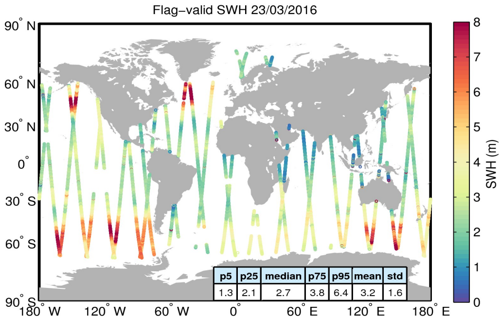
Figure 15. Geographical distribution of flag-valid SWH data over oceans and lakes for 23/03/2016. The statistical values shown in the table refer to the SWH in m and are calculated over all measurements shown in the figure.
