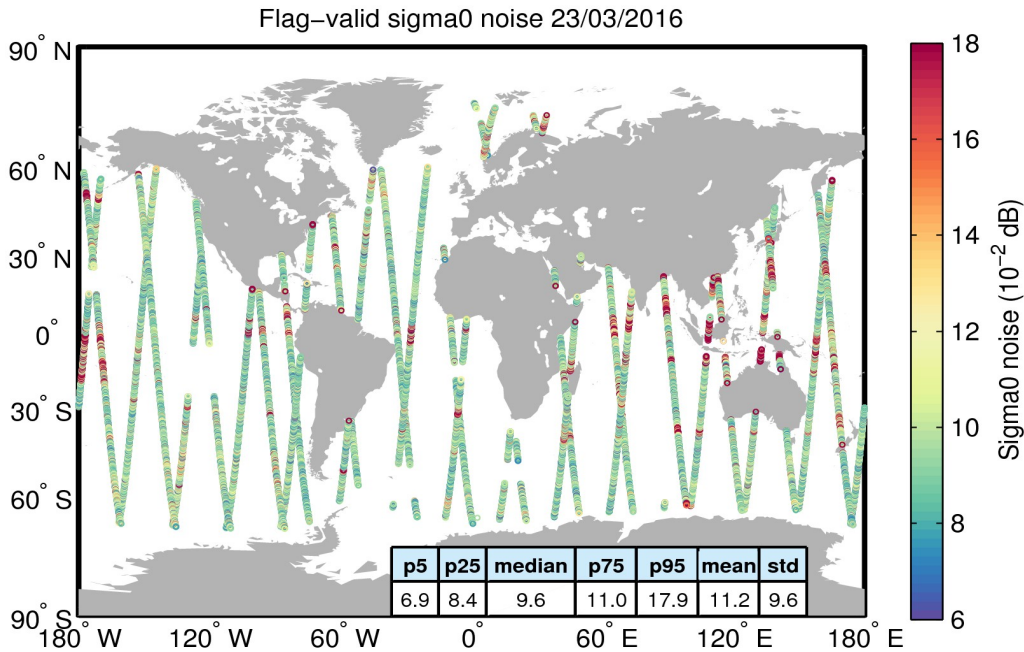
Figure 26. Geographical distribution of flag-valid 20-Hz sigma0 measurement noise over oceans and lakes for 23/03/2016. The statistical values shown in the table refer to the sigma0 noise and are calculated over all measurements shown in the figure.
