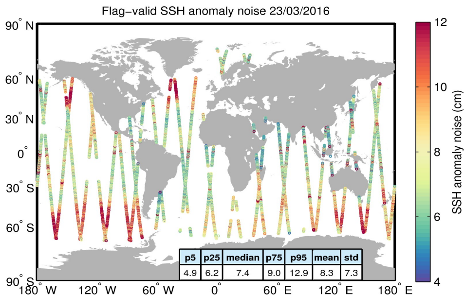
Figure 8. Geographical distribution of flag-valid 20-Hz SSH anomaly measurement noise over oceans and lakes for 23/03/2016. The statistical values shown in the table refer to the SSH anomaly noise and are calculated over all measurements shown in the figure.
