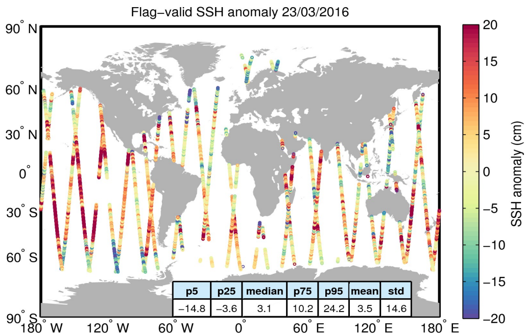
Figure 5. Geographical distribution of flag-valid 1-Hz SSH anomaly data over oceans and lakes for 23/03/2016. The statistical values shown in the table refer to the SSH anomaly in cm and are calculated over all measurements shown in the figure.
