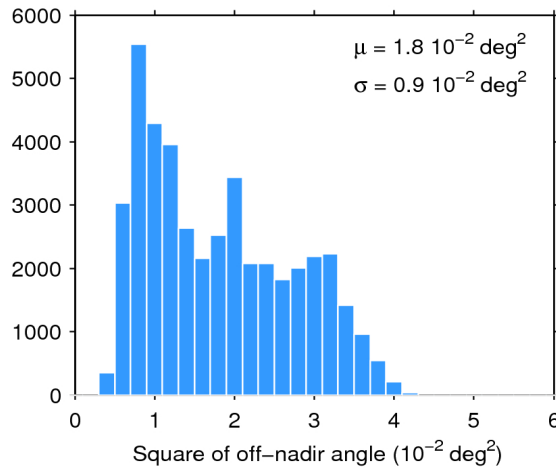
Figure 39. Histogram of flag-valid mispointing over oceans and lakes for 23/03/2016. The mean ( \mu ) and standard deviation ( \sigma ) are also shown. Note that values larger than 6 \cdot 10^{-2} \text{ deg}^2 are excluded from the histogram for the sake of readability but not from the computation of \mu and \sigma .
