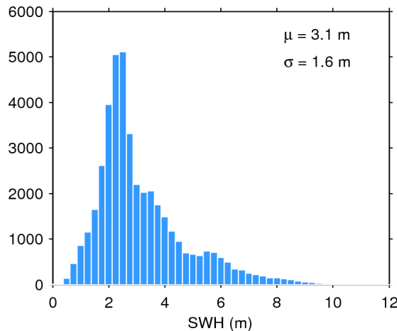
Figure 20. Histogram of science-valid SWH over oceans and lakes for 23/03/2016. The mean ( \mu ) and standard deviation ( \sigma ) are also shown. Note that values larger than 12 m are excluded from the histogram for the sake of readability but not from the computation of \mu and \sigma .
