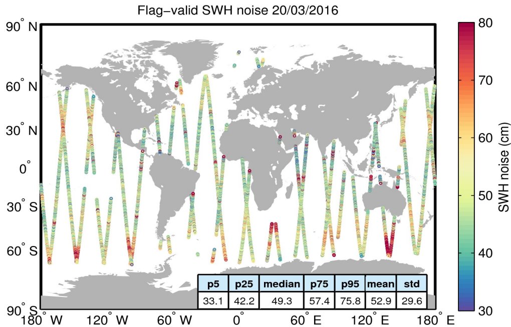
Figure 18. Geographical distribution of flag-valid 20-Hz SWH measurement noise over oceans and lakes for 20/03/2016. The statistical values shown in the table refer to the SWH noise and are calculated over all measurements shown in the figure.
