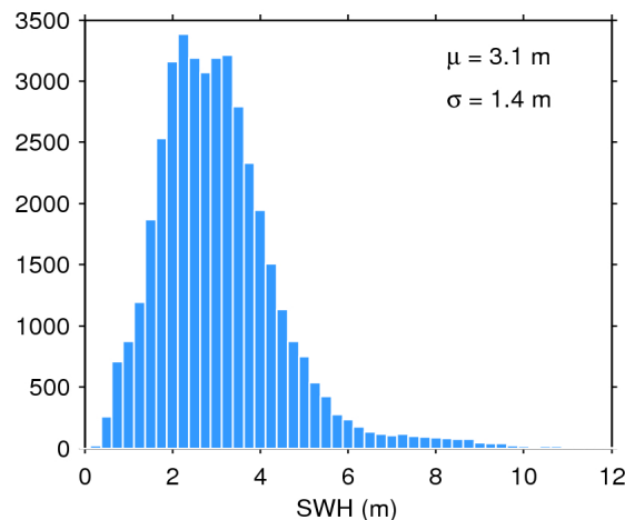
Figure 20. Histogram of science-valid SWH over oceans and lakes for 20/03/2016. The mean ( \mu ) and standard deviation ( \sigma ) are also shown. Note that values larger than 12 m are excluded from the histogram for the sake of readability but not from the computation of \mu and \sigma .
