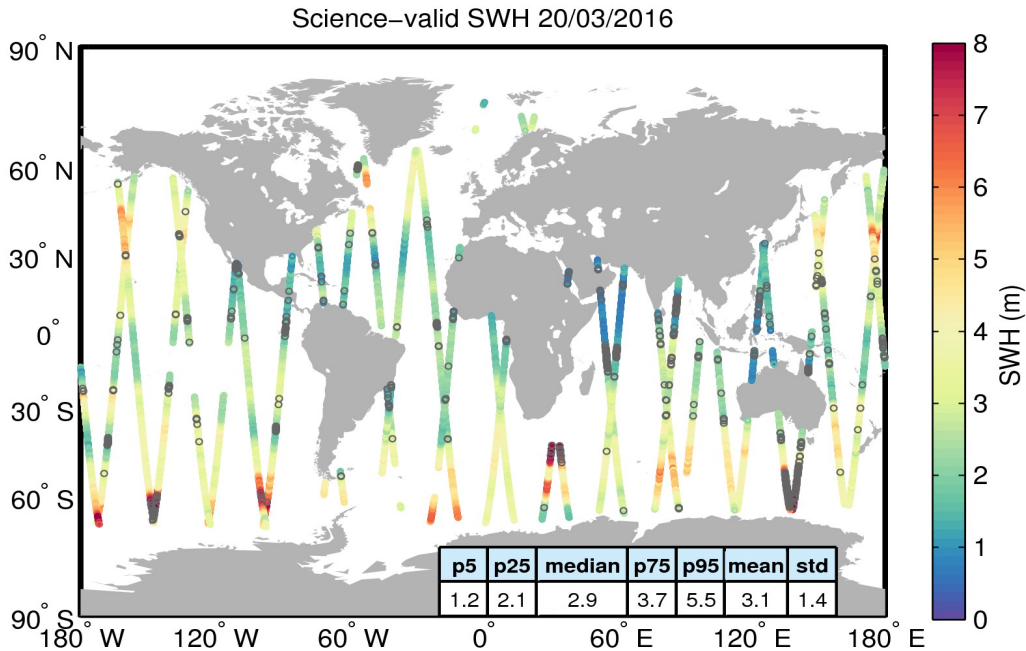
Figure 19. Geographical distribution of science-valid SWH data over oceans and lakes for 20/03/2016. The statistical values shown in the table refer to the SWH in m and are calculated over all measurements shown in the figure. Gray circles denote records that have been rejected based on the editing criteria described in Table 3.
