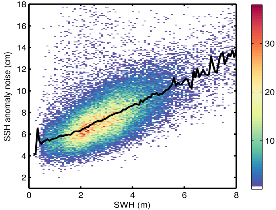
Figure 9. 2D histogram showing flag-valid SSH anomaly noise as a function of SWH for 20/03/2016. The black line denotes the median SSH anomaly noise as a function of SWH.
