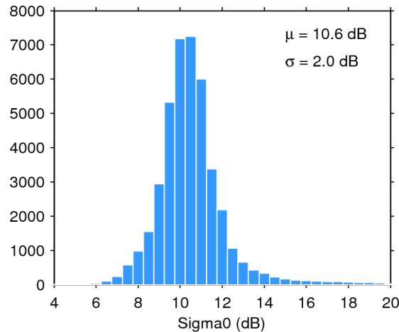
Figure 25. Histogram of flag-valid sigma0 over oceans and lakes for 20/03/2016. The mean ( \mu ) and standard deviation ( \sigma ) are also shown. Note that values outside [4 20] dB are excluded from the histogram for the sake of readability but not from the computation of \mu and \sigma .
