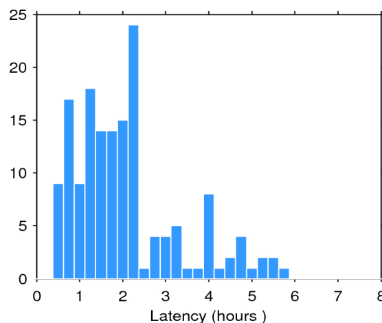
Figure 2. Histogram of the data latency for 20/03/2016. The y-axis denotes the number of files that are made available with a delay of x-hours with respect to the mean time of the records stored in the file.
