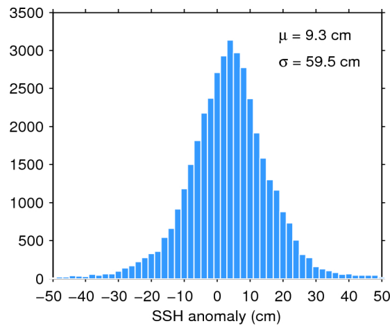
Figure 7. Histogram of flag-valid SSH anomaly over oceans and lakes for 20/03/2016. The mean ( \mu ) and standard deviation ( \sigma ) are also shown. Note that values outside [-50 50] cm are excluded from the histogram for the sake of readability but not from the computation of \mu and \sigma .
