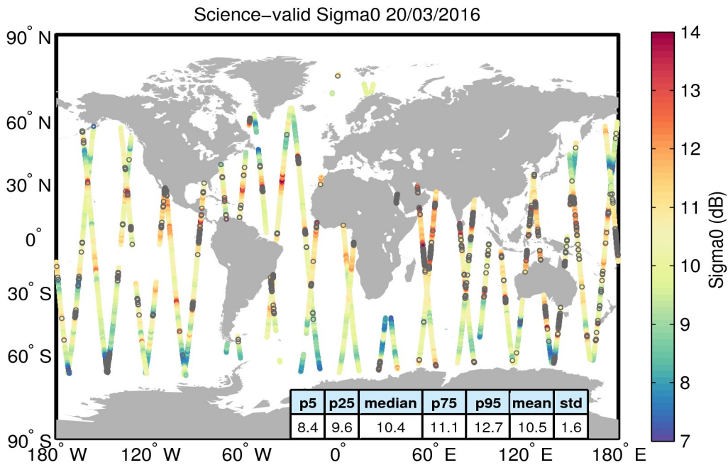
Figure 27. Geographical distribution of science-valid sigma0 data over oceans and lakes for 20/03/2016. The statistical values shown in the table refer to the sigma0 in dB and are calculated over all measurements shown in the figure. Gray circles denote records that have been rejected based on the editing criteria described in Table 4.
