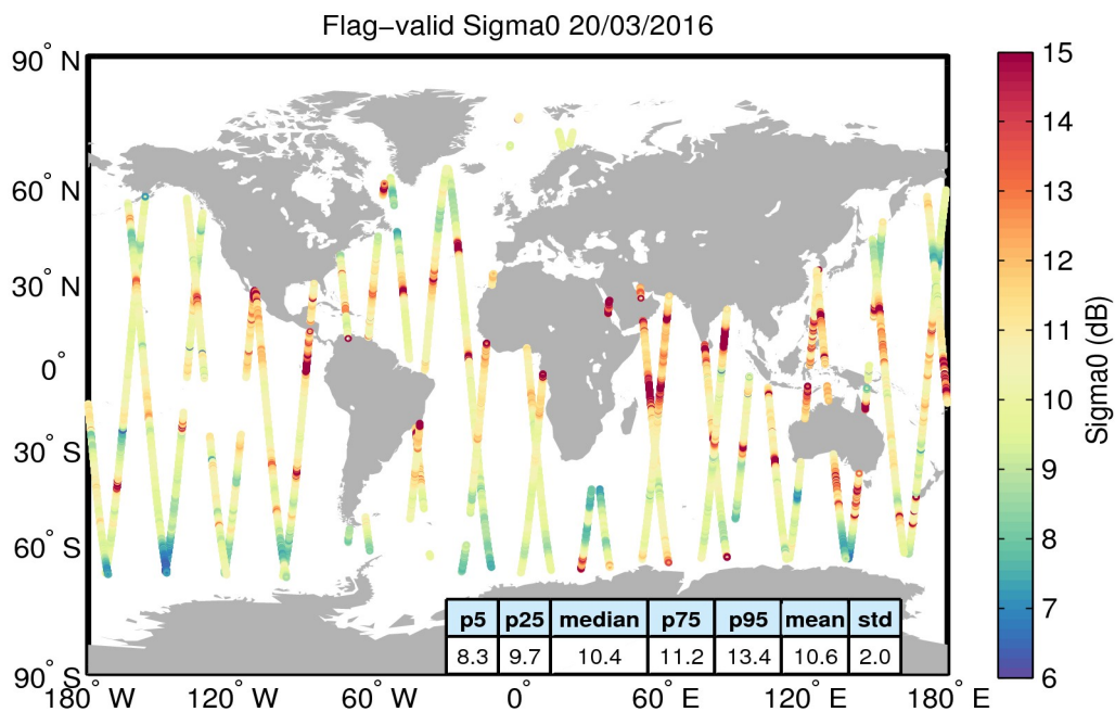
Figure 23. Geographical distribution of flag-valid sigma0 data over oceans and lakes for 20/03/2016. The statistical values shown in the table refer to the sigma0 in dB and are calculated over all measurements shown in the figure.
