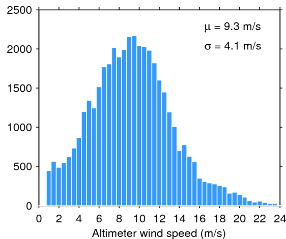
Figure 35. Histogram of science-valid wind over oceans and lakes for 20/03/2016. The mean ( \mu ) and standard deviation ( \sigma ) are also shown. Note that values larger than 24 m/s are excluded from the histogram for the sake of readability but not from the computation of \mu and \sigma .
