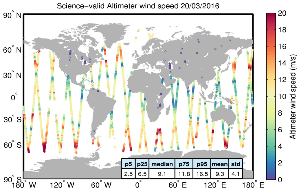
Figure 34. Geographical distribution of science-valid wind data over oceans and lakes for 20/03/2016. The statistical values shown in the table refer to the wind in m/s and are calculated over all measurements shown in the figure. Gray circles denote records that have been rejected based on the editing criteria described in Table 5.
