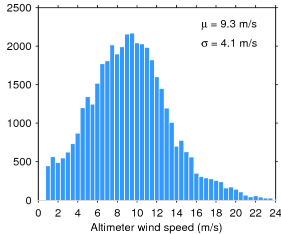
Figure 33. Histogram of flag-valid wind over oceans and lakes for 20/03/2016. The mean ( \mu ) and standard deviation ( \sigma ) are also shown. Note that values larger than 24 m/s are excluded from the histogram for the sake of readability but not from the computation of \mu and \sigma .
