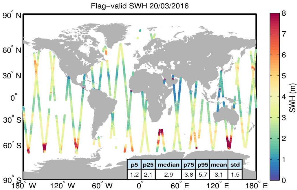
Figure 15. Geographical distribution of flag-valid SWH data over oceans and lakes for 20/03/2016. The statistical values shown in the table refer to the SWH in m and are calculated over all measurements shown in the figure.
