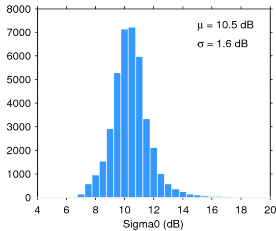
Figure 28. Histogram of science-valid sigma0 over oceans and lakes for 20/03/2016. The mean ( \mu ) and standard deviation ( \sigma ) are also shown. Note that values outside [4 20] dB are excluded from the histogram for the sake of readability but not from the computation of \mu and \sigma .
