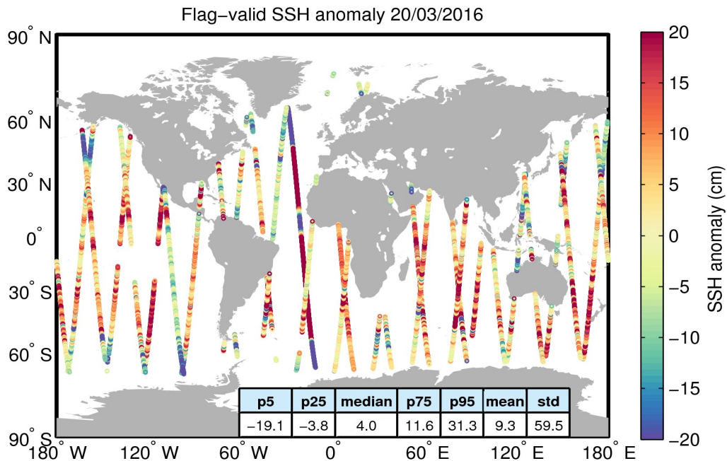
Figure 5. Geographical distribution of flag-valid 1-Hz SSH anomaly data over oceans and lakes for 20/03/2016. The statistical values shown in the table refer to the SSH anomaly in cm and are calculated over all measurements shown in the figure.
