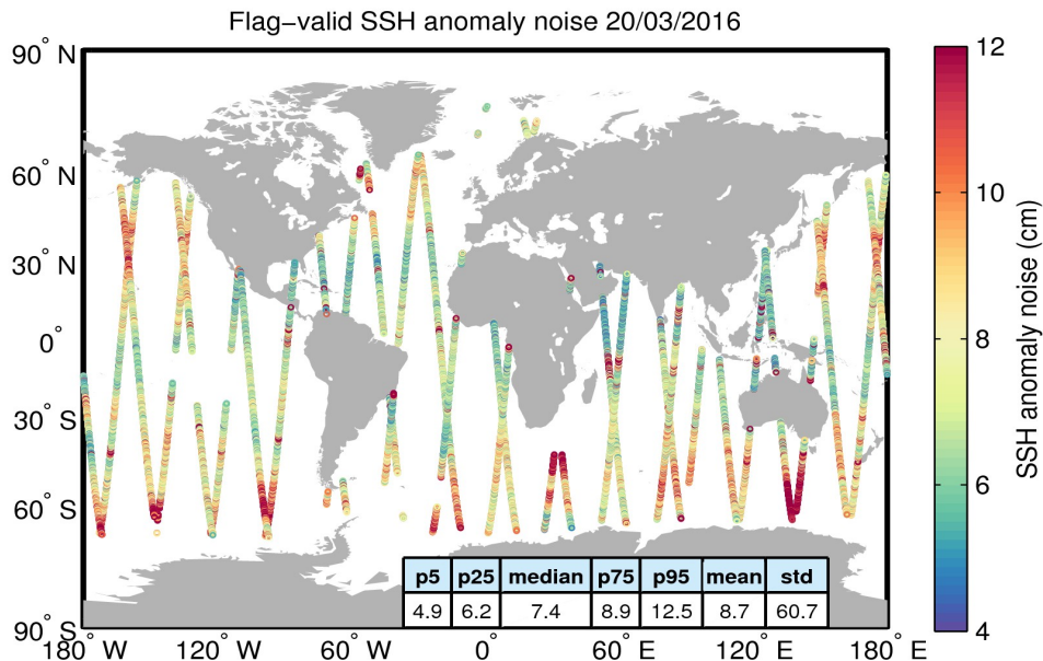
Figure 8. Geographical distribution of flag-valid 20-Hz SSH anomaly measurement noise over oceans and lakes for 20/03/2016. The statistical values shown in the table refer to the SSH anomaly noise and are calculated over all measurements shown in the figure.
