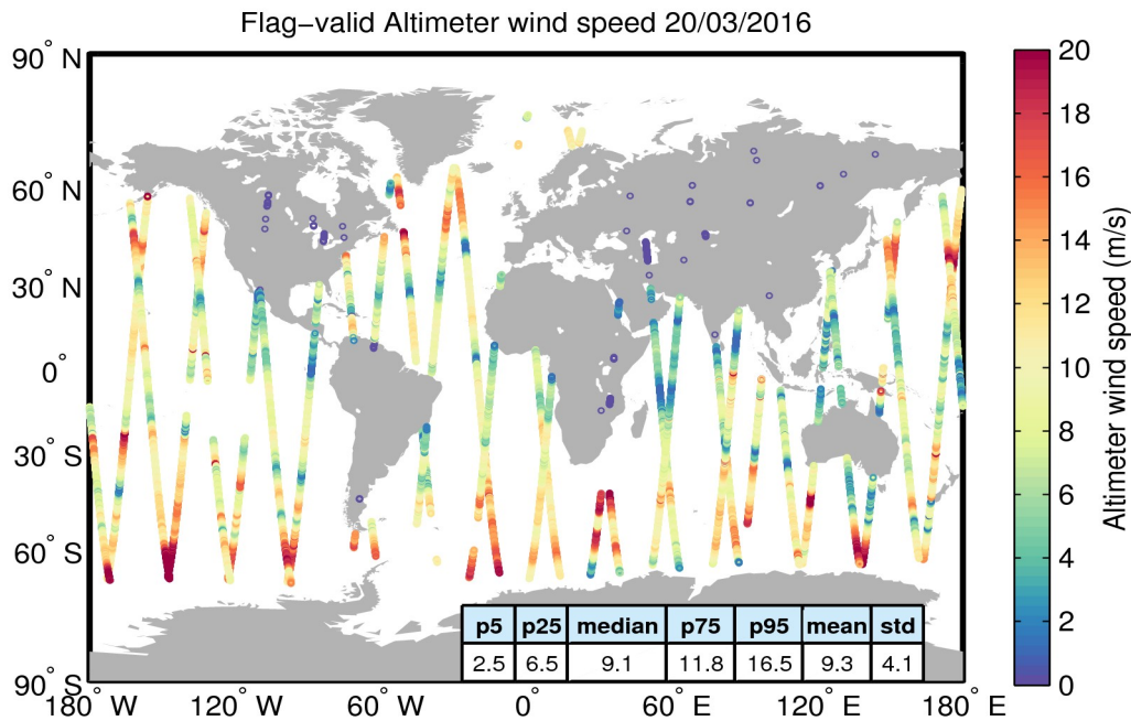
Figure 31. Geographical distribution of flag-valid wind data over oceans and lakes for 20/03/2016. The statistical values shown in the table refer to the wind in m/s and are calculated over all measurements shown in the figure.
