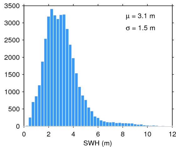
Figure 17. Histogram of flag-valid SWH over oceans and lakes for 20/03/2016. The mean ( \mu ) and standard deviation ( \sigma ) are also shown. Note that values larger than 12 m are excluded from the histogram for the sake of readability but not from the computation of \mu and \sigma .
