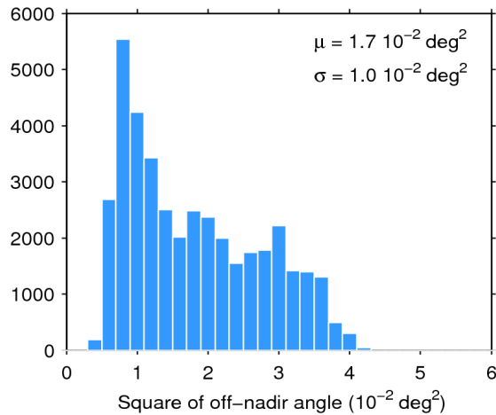
Figure 39. Histogram of flag-valid mispointing over oceans and lakes for 20/03/2016. The mean ( \mu ) and standard deviation ( \sigma ) are also shown. Note that values larger than 6 \cdot 10^{-2} \text{ deg}^2 are excluded from the histogram for the sake of readability but not from the computation of \mu and \sigma .
