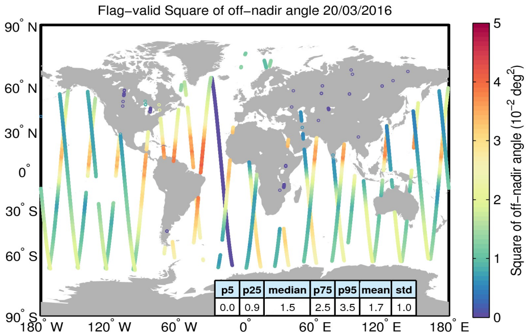
Figure 37. Geographical distribution of flag-valid mispointing data over oceans and lakes for 20/03/2016. The statistical values shown in the table refer to the mispointing in 10^{-2} deg 2 and are calculated over all measurements shown in the figure.
