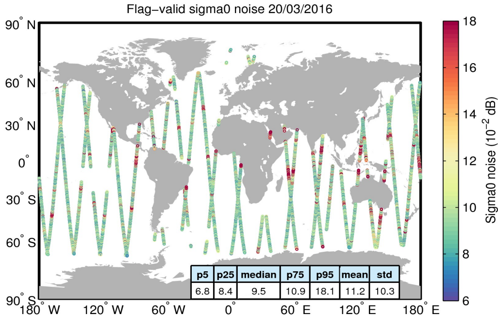
Figure 26. Geographical distribution of flag-valid 20-Hz sigma0 measurement noise over oceans and lakes for 20/03/2016. The statistical values shown in the table refer to the sigma0 noise and are calculated over all measurements shown in the figure.
