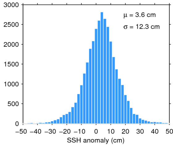
Figure 11. Histogram of science-valid SSH anomaly over oceans and lakes for 20/03/2016. The mean ( \mu ) and standard deviation ( \sigma ) are also shown. Note that values outside [-50 50] cm are excluded from the histogram for the sake of readability but not from the computation of \mu and \sigma .
