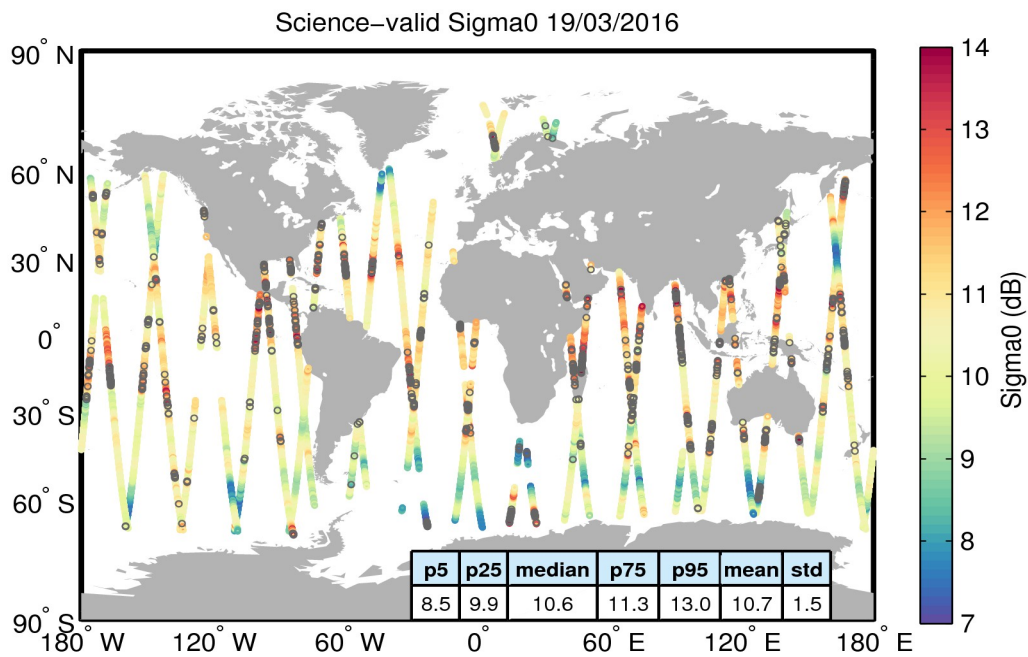
Figure 27. Geographical distribution of science-valid sigma0 data over oceans and lakes for 19/03/2016. The statistical values shown in the table refer to the sigma0 in dB and are calculated over all measurements shown in the figure. Gray circles denote records that have been rejected based on the editing criteria described in Table 4.
