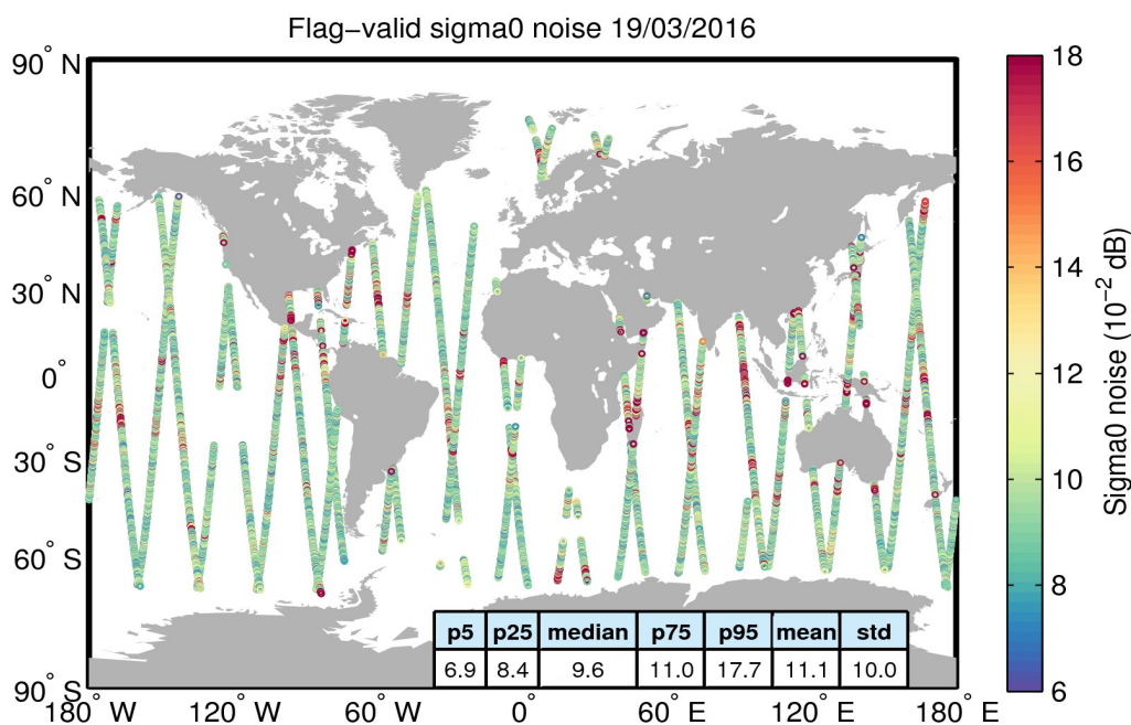
Figure 26. Geographical distribution of flag-valid 20-Hz sigma0 measurement noise over oceans and lakes for 19/03/2016. The statistical values shown in the table refer to the sigma0 noise and are calculated over all measurements shown in the figure.
