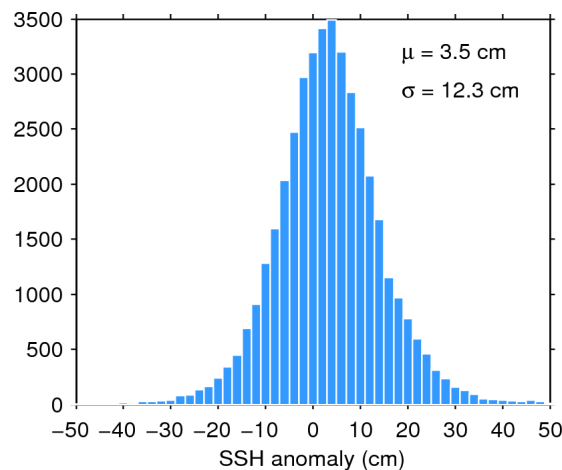
Figure 11. Histogram of science-valid SSH anomaly over oceans and lakes for 19/03/2016. The mean ( \mu ) and standard deviation ( \sigma ) are also shown. Note that values outside [-50 50] cm are excluded from the histogram for the sake of readability but not from the computation of \mu and \sigma .
