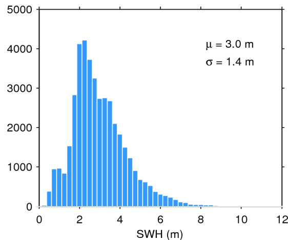
Figure 20. Histogram of science-valid SWH over oceans and lakes for 19/03/2016. The mean ( \mu ) and standard deviation ( \sigma ) are also shown. Note that values larger than 12 m are excluded from the histogram for the sake of readability but not from the computation of \mu and \sigma .
