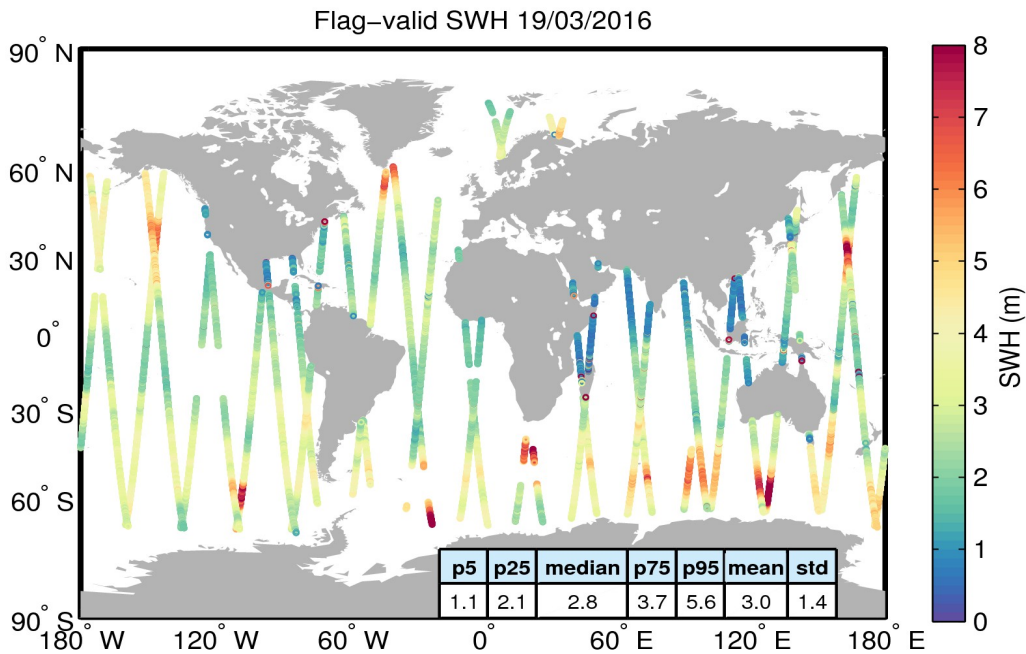
Figure 15. Geographical distribution of flag-valid SWH data over oceans and lakes for 19/03/2016. The statistical values shown in the table refer to the SWH in m and are calculated over all measurements shown in the figure.
