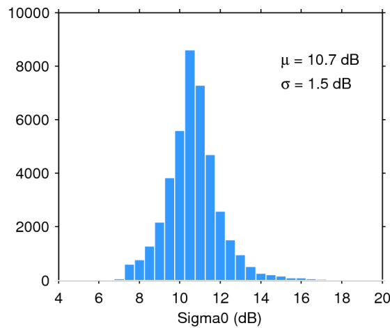
Figure 28. Histogram of science-valid sigma0 over oceans and lakes for 19/03/2016. The mean ( \mu ) and standard deviation ( \sigma ) are also shown. Note that values outside [4 20] dB are excluded from the histogram for the sake of readability but not from the computation of \mu and \sigma .
