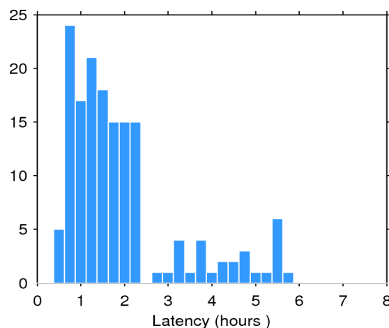
Figure 2. Histogram of the data latency for 19/03/2016. The y-axis denotes the number of files that are made available with a delay of x-hours with respect to the mean time of the records stored in the file.
