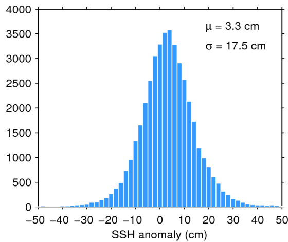
Figure 7. Histogram of flag-valid SSH anomaly over oceans and lakes for 19/03/2016. The mean ( \mu ) and standard deviation ( \sigma ) are also shown. Note that values outside [-50\ 50] cm are excluded from the histogram for the sake of readability but not from the computation of \mu and \sigma .
