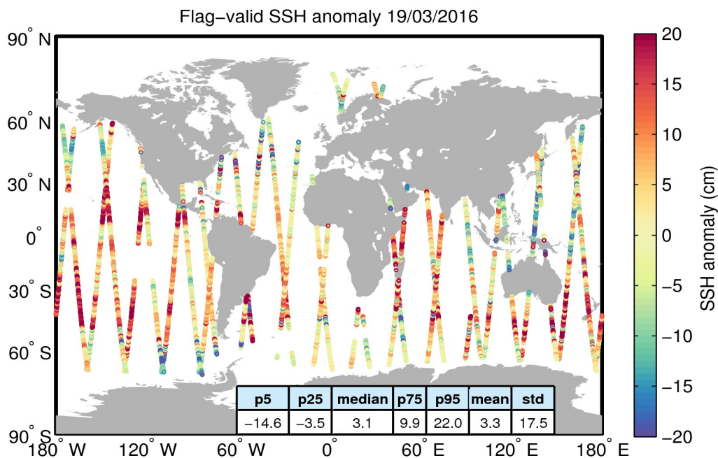
Figure 5. Geographical distribution of flag-valid 1-Hz SSH anomaly data over oceans and lakes for 19/03/2016. The statistical values shown in the table refer to the SSH anomaly in cm and are calculated over all measurements shown in the figure.
