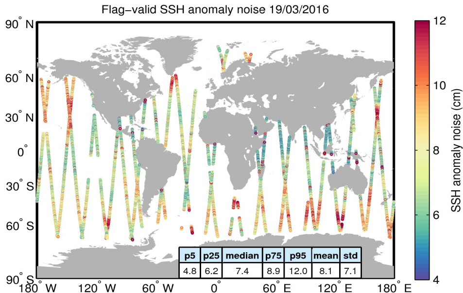
Figure 8. Geographical distribution of flag-valid 20-Hz SSH anomaly measurement noise over oceans and lakes for 19/03/2016. The statistical values shown in the table refer to the SSH anomaly noise and are calculated over all measurements shown in the figure.
