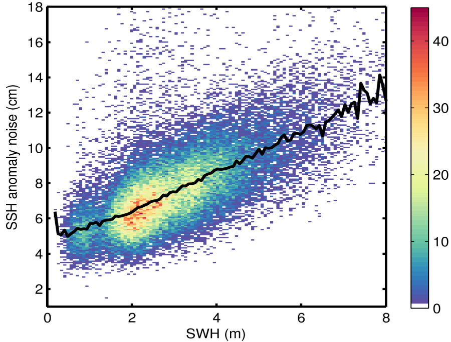
Figure 9. 2D histogram showing flag-valid SSH anomaly noise as a function of SWH for 19/03/2016. The black line denotes the median SSH anomaly noise as a function of SWH.
