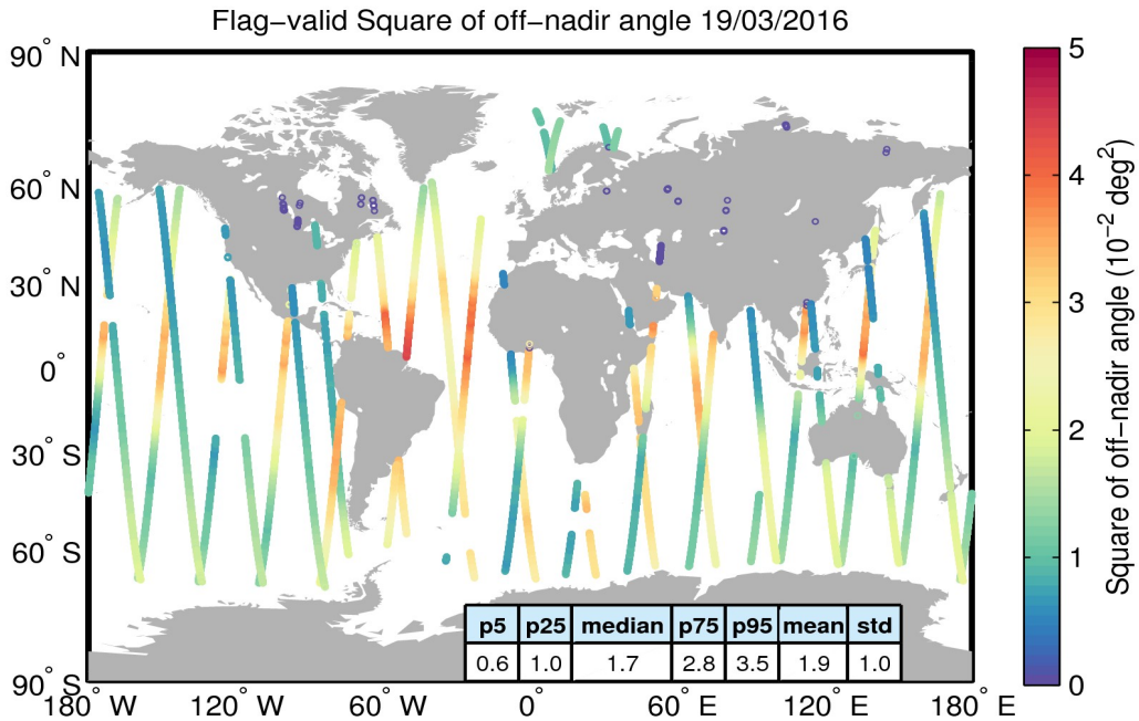
Figure 37. Geographical distribution of flag-valid mispointing data over oceans and lakes for 19/03/2016. The statistical values shown in the table refer to the mispointing in 10^{-2} deg 2 and are calculated over all measurements shown in the figure.
