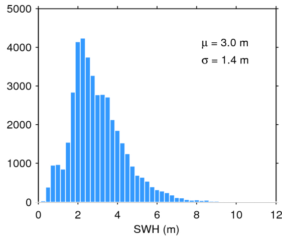
Figure 17. Histogram of flag-valid SWH over oceans and lakes for 19/03/2016. The mean ( \mu ) and standard deviation ( \sigma ) are also shown. Note that values larger than 12 m are excluded from the histogram for the sake of readability but not from the computation of \mu and \sigma .
