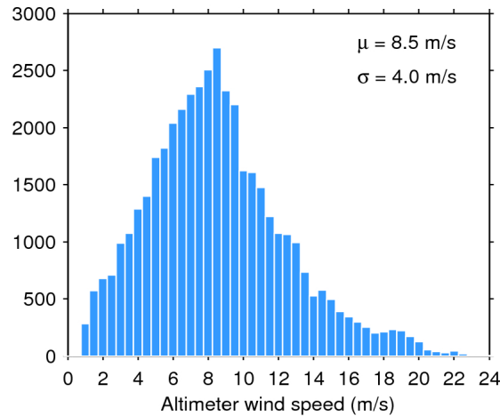
Figure 33. Histogram of flag-valid wind over oceans and lakes for 19/03/2016. The mean ( \mu ) and standard deviation ( \sigma ) are also shown. Note that values larger than 24 m/s are excluded from the histogram for the sake of readability but not from the computation of \mu and \sigma .
