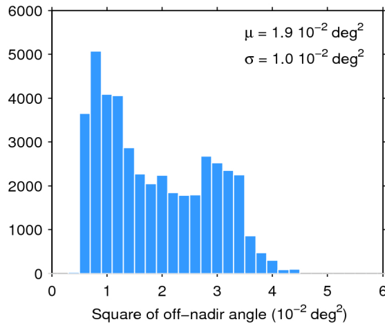
Figure 39. Histogram of flag-valid mispointing over oceans and lakes for 19/03/2016. The mean ( \mu ) and standard deviation ( \sigma ) are also shown. Note that values larger than 6 \cdot 10^{-2} \text{ deg}^2 are excluded from the histogram for the sake of readability but not from the computation of \mu and \sigma .
