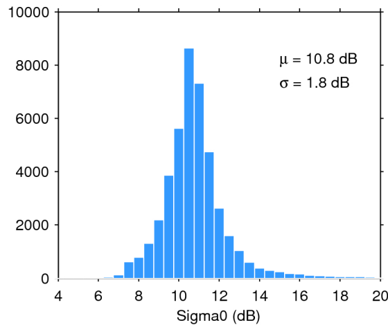
Figure 25. Histogram of flag-valid sigma0 over oceans and lakes for 19/03/2016. The mean ( \mu ) and standard deviation ( \sigma ) are also shown. Note that values outside [4 20] dB are excluded from the histogram for the sake of readability but not from the computation of \mu and \sigma .
