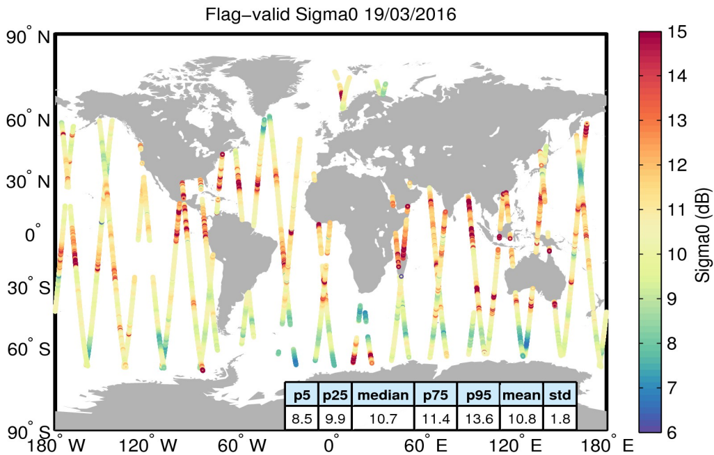
Figure 23. Geographical distribution of flag-valid sigma0 data over oceans and lakes for 19/03/2016. The statistical values shown in the table refer to the sigma0 in dB and are calculated over all measurements shown in the figure.
