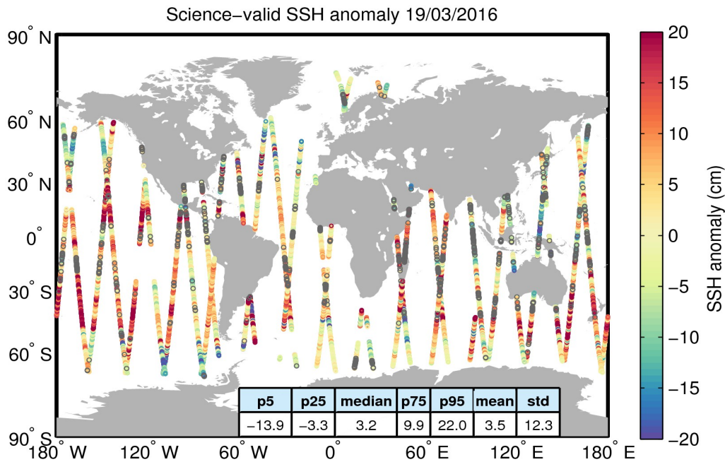
Figure 10. Geographical distribution of science-valid SSH anomaly data over oceans and lakes for 19/03/2016. The statistical values shown in the table refer to the SSH anomaly in cm and are calculated over all measurements shown in the figure. Gray circles denote records that have been rejected based on the editing criteria described in Table 2.
