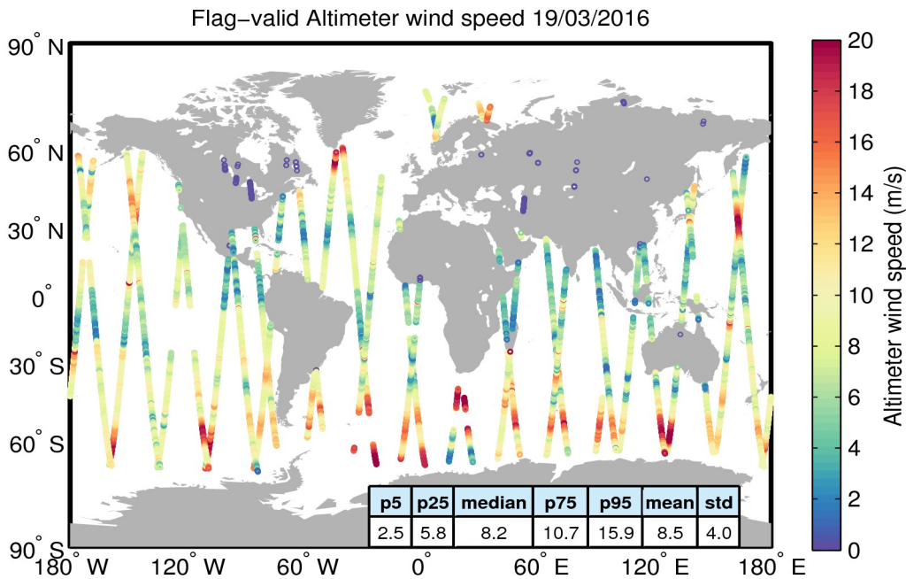
Figure 31. Geographical distribution of flag-valid wind data over oceans and lakes for 19/03/2016. The statistical values shown in the table refer to the wind in m/s and are calculated over all measurements shown in the figure.
