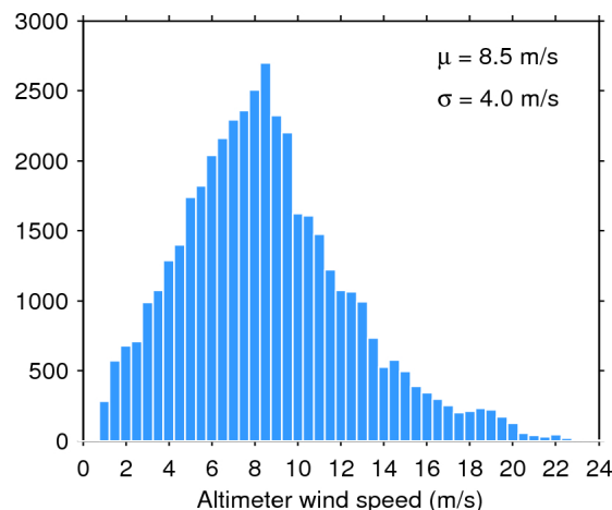
Figure 35. Histogram of science-valid wind over oceans and lakes for 19/03/2016. The mean ( \mu ) and standard deviation ( \sigma ) are also shown. Note that values larger than 24 m/s are excluded from the histogram for the sake of readability but not from the computation of \mu and \sigma .
