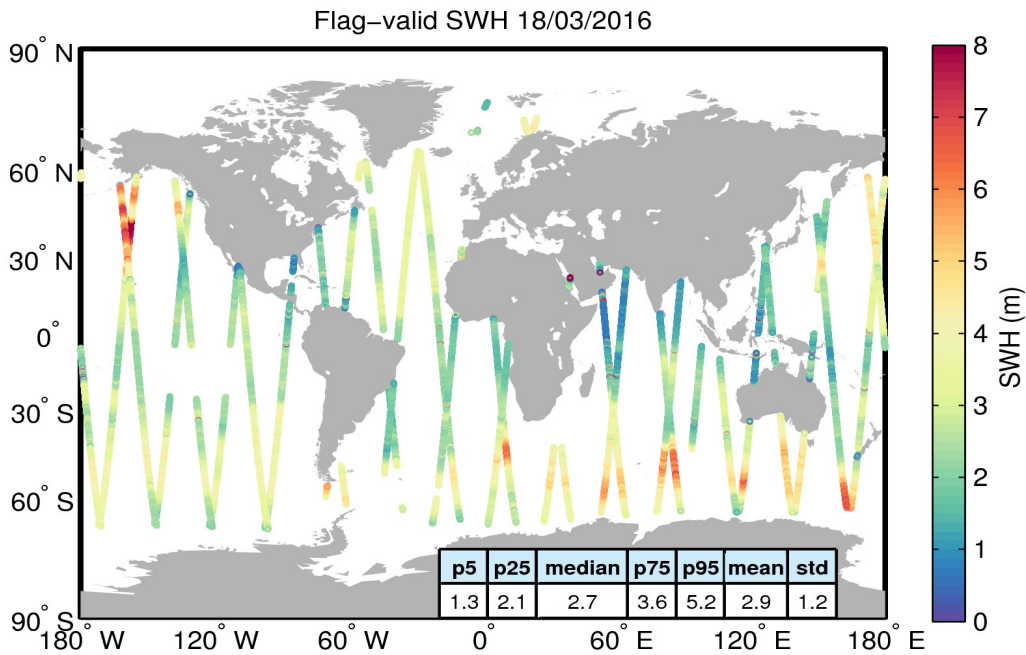
Figure 15. Geographical distribution of flag-valid SWH data over oceans and lakes for 18/03/2016. The statistical values shown in the table refer to the SWH in m and are calculated over all measurements shown in the figure.
