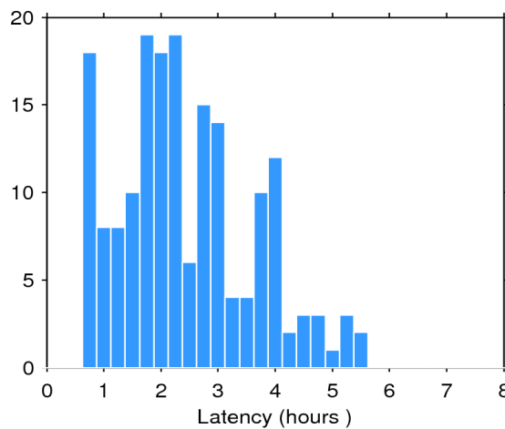
Figure 2. Histogram of the data latency for 18/03/2016. The y-axis denotes the number of files that are made available with a delay of x-hours with respect to the mean time of the records stored in the file.
