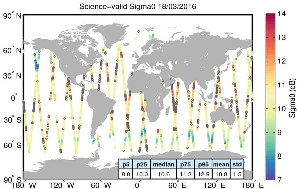
Figure 27. Geographical distribution of science-valid sigma0 data over oceans and lakes for 18/03/2016. The statistical values shown in the table refer to the sigma0 in dB and are calculated over all measurements shown in the figure. Gray circles denote records that have been rejected based on the editing criteria described in Table 4.
