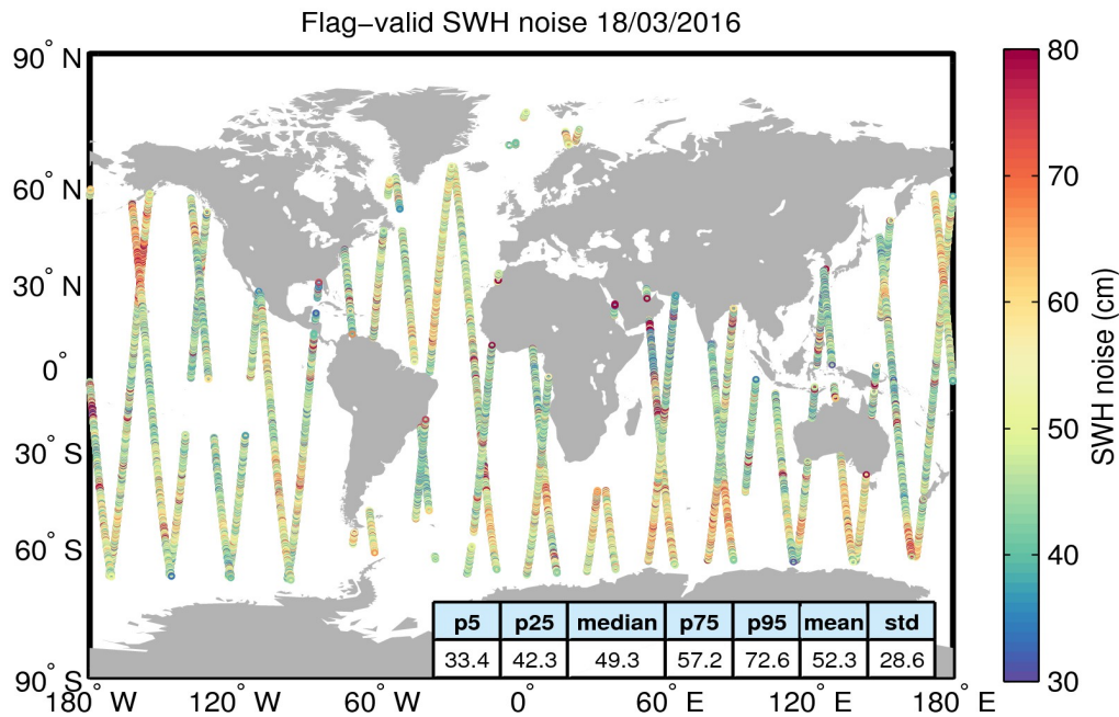
Figure 18. Geographical distribution of flag-valid 20-Hz SWH measurement noise over oceans and lakes for 18/03/2016. The statistical values shown in the table refer to the SWH noise and are calculated over all measurements shown in the figure.
