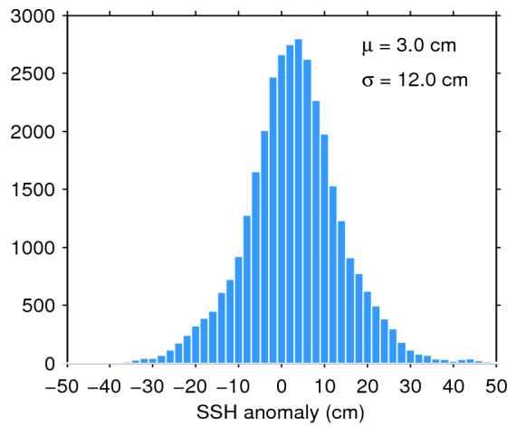
Figure 11. Histogram of science-valid SSH anomaly over oceans and lakes for 18/03/2016. The mean ( \mu ) and standard deviation ( \sigma ) are also shown. Note that values outside [-50 50] cm are excluded from the histogram for the sake of readability but not from the computation of \mu and \sigma .
