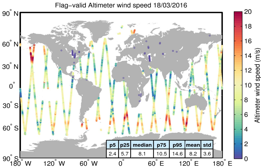
Figure 31. Geographical distribution of flag-valid wind data over oceans and lakes for 18/03/2016. The statistical values shown in the table refer to the wind in m/s and are calculated over all measurements shown in the figure.
