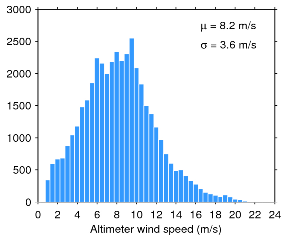
Figure 35. Histogram of science-valid wind over oceans and lakes for 18/03/2016. The mean ( \mu ) and standard deviation ( \sigma ) are also shown. Note that values larger than 24 m/s are excluded from the histogram for the sake of readability but not from the computation of \mu and \sigma .
