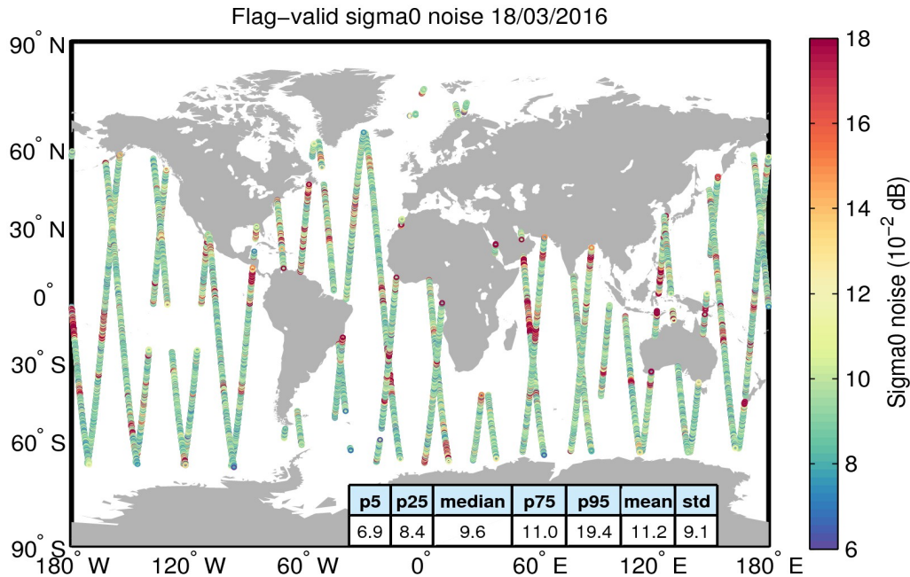
Figure 26. Geographical distribution of flag-valid 20-Hz sigma0 measurement noise over oceans and lakes for 18/03/2016. The statistical values shown in the table refer to the sigma0 noise and are calculated over all measurements shown in the figure.
