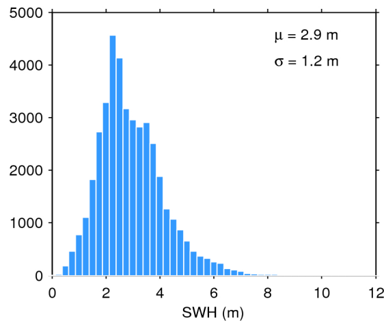
Figure 17. Histogram of flag-valid SWH over oceans and lakes for 18/03/2016. The mean ( \mu ) and standard deviation ( \sigma ) are also shown. Note that values larger than 12 m are excluded from the histogram for the sake of readability but not from the computation of \mu and \sigma .
