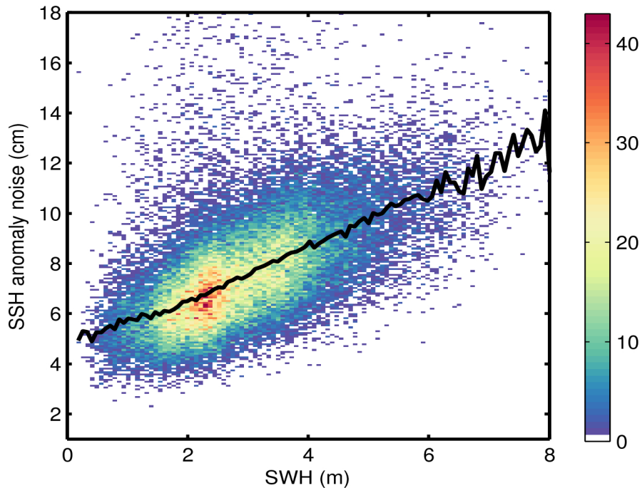
Figure 9. 2D histogram showing flag-valid SSH anomaly noise as a function of SWH for 18/03/2016. The black line denotes the median SSH anomaly noise as a function of SWH.
