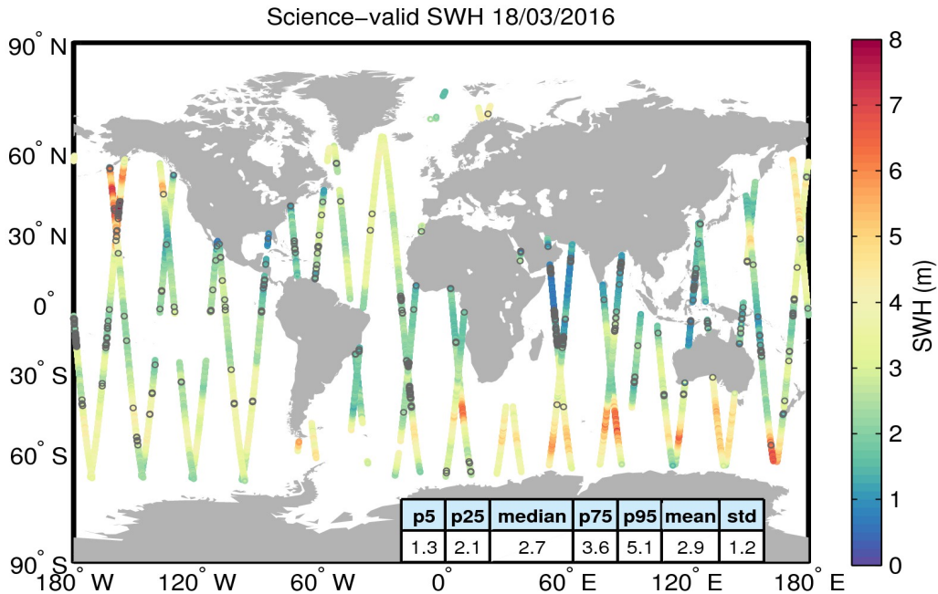
Figure 19. Geographical distribution of science-valid SWH data over oceans and lakes for 18/03/2016. The statistical values shown in the table refer to the SWH in m and are calculated over all measurements shown in the figure. Gray circles denote records that have been rejected based on the editing criteria described in Table 3.
