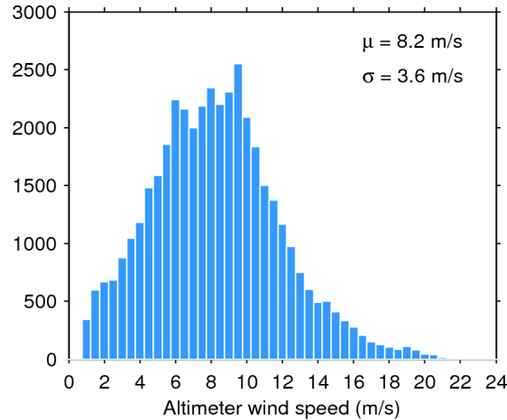
Figure 33. Histogram of flag-valid wind over oceans and lakes for 18/03/2016. The mean ( \mu ) and standard deviation ( \sigma ) are also shown. Note that values larger than 24 m/s are excluded from the histogram for the sake of readability but not from the computation of \mu and \sigma .
