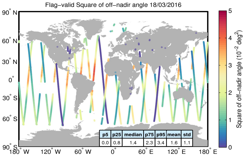
Figure 37. Geographical distribution of flag-valid mispointing data over oceans and lakes for 18/03/2016. The statistical values shown in the table refer to the mispointing in 10^{-2} \text{ deg}^2 and are calculated over all measurements shown in the figure.
