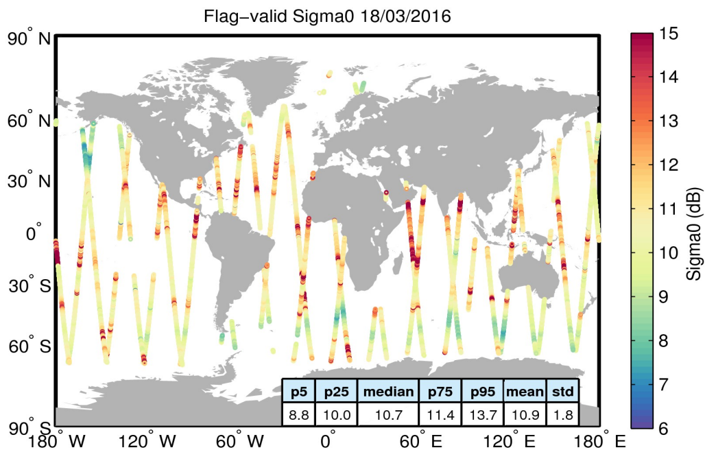
Figure 23. Geographical distribution of flag-valid sigma0 data over oceans and lakes for 18/03/2016. The statistical values shown in the table refer to the sigma0 in dB and are calculated over all measurements shown in the figure.
