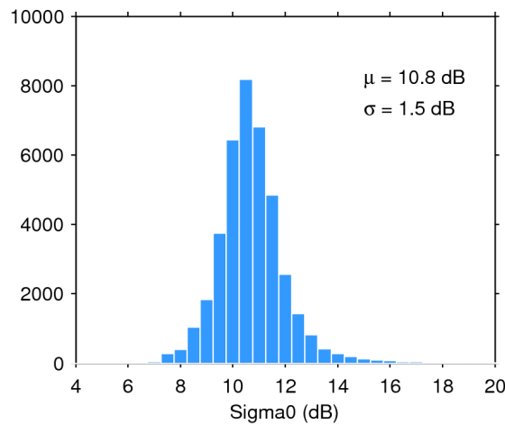
Figure 28. Histogram of science-valid sigma0 over oceans and lakes for 18/03/2016. The mean ( \mu ) and standard deviation ( \sigma ) are also shown. Note that values outside [4 20] dB are excluded from the histogram for the sake of readability but not from the computation of \mu and \sigma .
