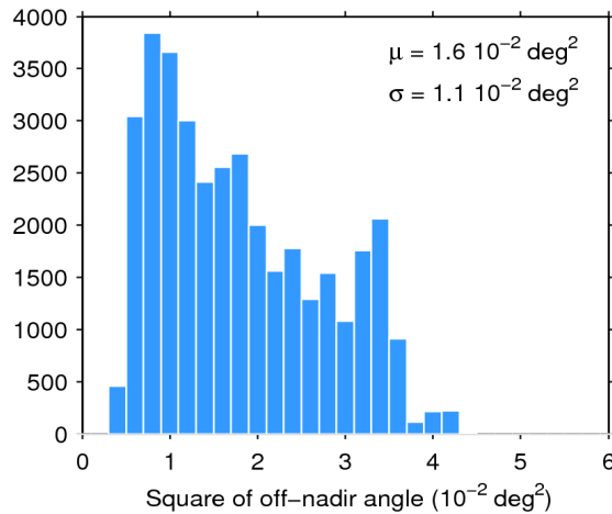
Figure 39. Histogram of flag-valid mispointing over oceans and lakes for 18/03/2016. The mean ( \mu ) and standard deviation ( \sigma ) are also shown. Note that values larger than 6 \cdot 10^{-2} \text{ deg}^2 are excluded from the histogram for the sake of readability but not from the computation of \mu and \sigma .
