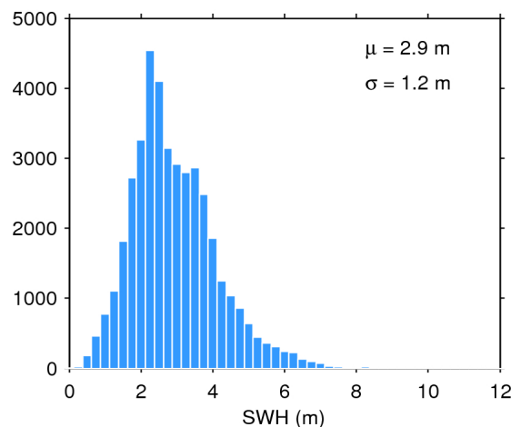
Figure 20. Histogram of science-valid SWH over oceans and lakes for 18/03/2016. The mean ( \mu ) and standard deviation ( \sigma ) are also shown. Note that values larger than 12 m are excluded from the histogram for the sake of readability but not from the computation of \mu and \sigma .
