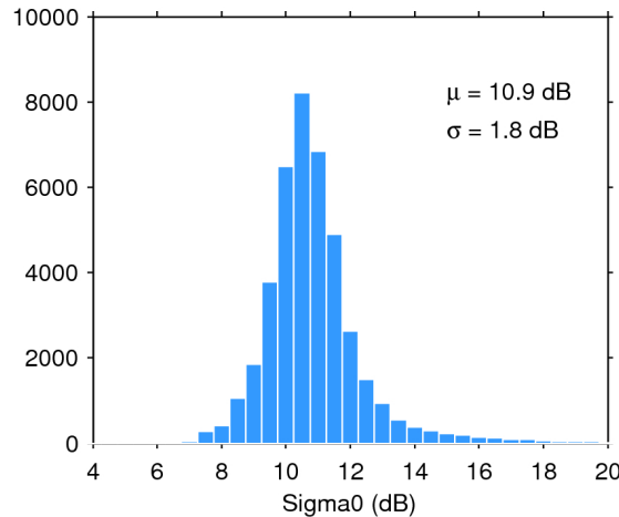
Figure 25. Histogram of flag-valid sigma0 over oceans and lakes for 18/03/2016. The mean ( \mu ) and standard deviation ( \sigma ) are also shown. Note that values outside [4 20] dB are excluded from the histogram for the sake of readability but not from the computation of \mu and \sigma .
