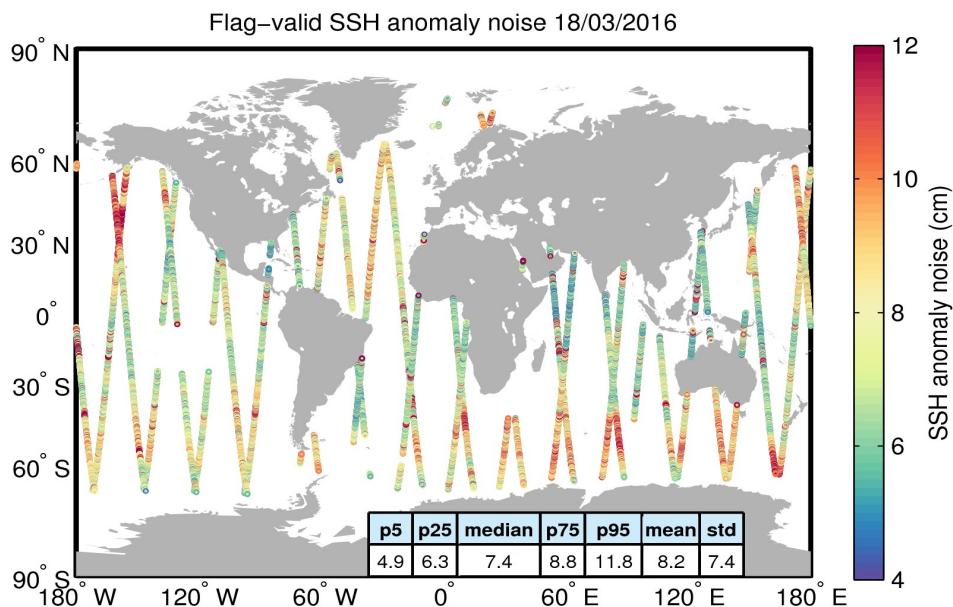
Figure 8. Geographical distribution of flag-valid 20-Hz SSH anomaly measurement noise over oceans and lakes for 18/03/2016. The statistical values shown in the table refer to the SSH anomaly noise and are calculated over all measurements shown in the figure.
