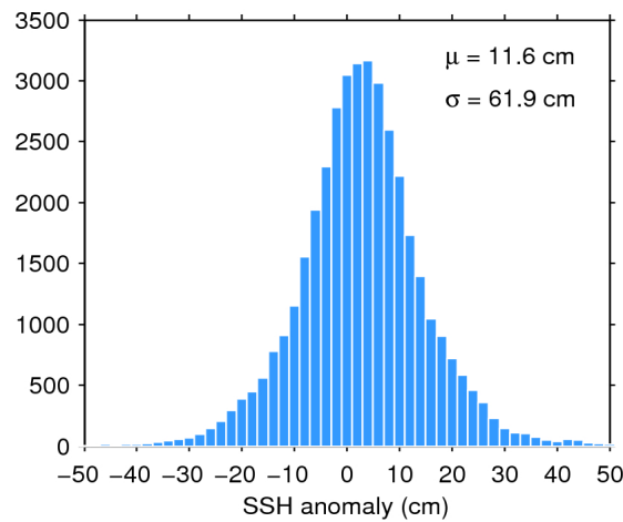
Figure 7. Histogram of flag-valid SSH anomaly over oceans and lakes for 18/03/2016. The mean ( \mu ) and standard deviation ( \sigma ) are also shown. Note that values outside [-50 50] cm are excluded from the histogram for the sake of readability but not from the computation of \mu and \sigma .
