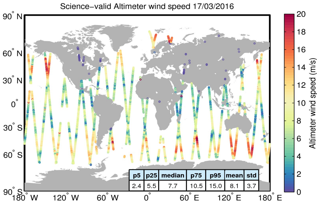
Figure 34. Geographical distribution of science-valid wind data over oceans and lakes for 17/03/2016. The statistical values shown in the table refer to the wind in m/s and are calculated over all measurements shown in the figure. Gray circles denote records that have been rejected based on the editing criteria described in Table 5.
