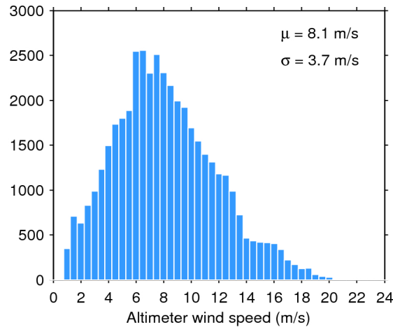
Figure 33. Histogram of flag-valid wind over oceans and lakes for 17/03/2016. The mean ( \mu ) and standard deviation ( \sigma ) are also shown. Note that values larger than 24 m/s are excluded from the histogram for the sake of readability but not from the computation of \mu and \sigma .
