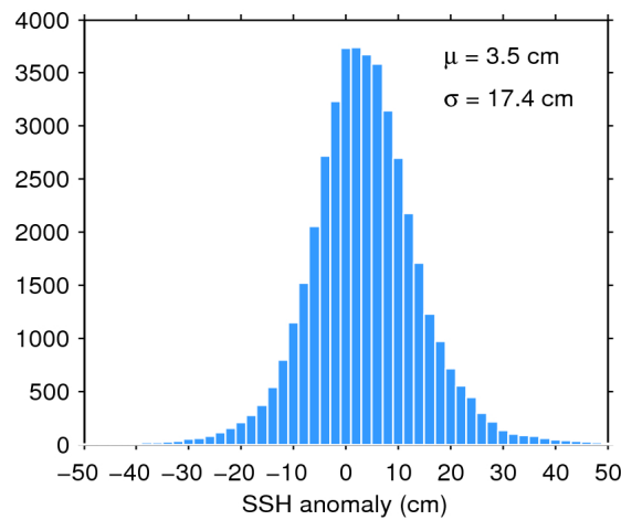
Figure 7. Histogram of flag-valid SSH anomaly over oceans and lakes for 17/03/2016. The mean ( \mu ) and standard deviation ( \sigma ) are also shown. Note that values outside [-50\ 50] cm are excluded from the histogram for the sake of readability but not from the computation of \mu and \sigma .
