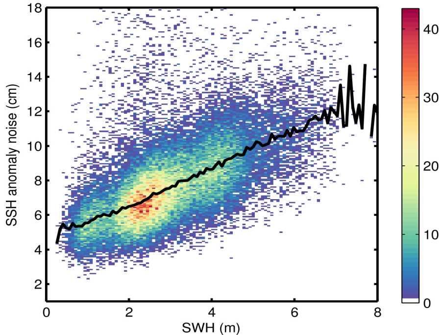
Figure 9. 2D histogram showing flag-valid SSH anomaly noise as a function of SWH for 17/03/2016. The black line denotes the median SSH anomaly noise as a function of SWH.
