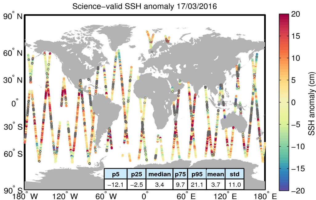
Figure 10. Geographical distribution of science-valid SSH anomaly data over oceans and lakes for 17/03/2016. The statistical values shown in the table refer to the SSH anomaly in cm and are calculated over all measurements shown in the figure. Gray circles denote records that have been rejected based on the editing criteria described in Table 2.
