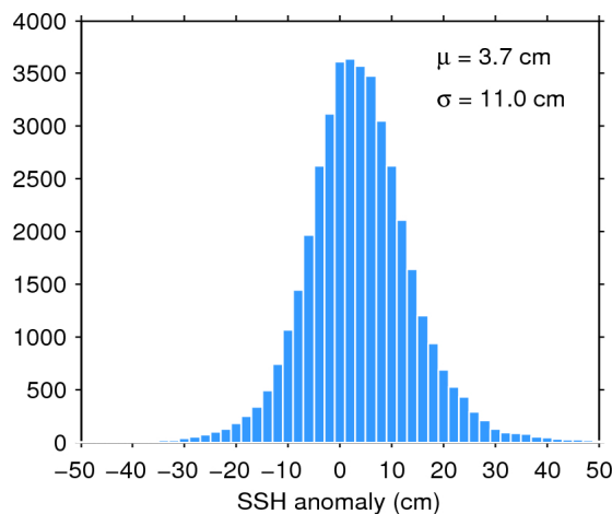
Figure 11. Histogram of science-valid SSH anomaly over oceans and lakes for 17/03/2016. The mean ( \mu ) and standard deviation ( \sigma ) are also shown. Note that values outside [-50 50] cm are excluded from the histogram for the sake of readability but not from the computation of \mu and \sigma .
