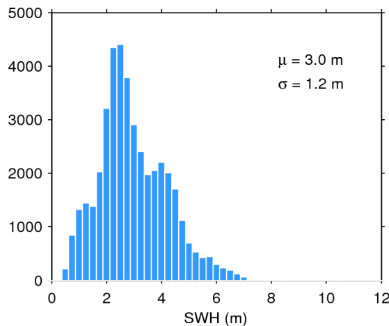
Figure 20. Histogram of science-valid SWH over oceans and lakes for 17/03/2016. The mean ( \mu ) and standard deviation ( \sigma ) are also shown. Note that values larger than 12 m are excluded from the histogram for the sake of readability but not from the computation of \mu and \sigma .
