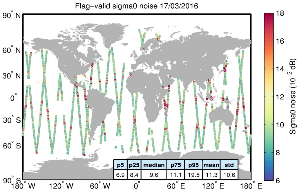
Figure 26. Geographical distribution of flag-valid 20-Hz sigma0 measurement noise over oceans and lakes for 17/03/2016. The statistical values shown in the table refer to the sigma0 noise and are calculated over all measurements shown in the figure.
