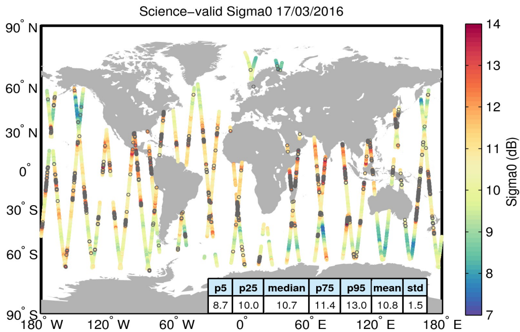
Figure 27. Geographical distribution of science-valid sigma0 data over oceans and lakes for 17/03/2016. The statistical values shown in the table refer to the sigma0 in dB and are calculated over all measurements shown in the figure. Gray circles denote records that have been rejected based on the editing criteria described in Table 4.
