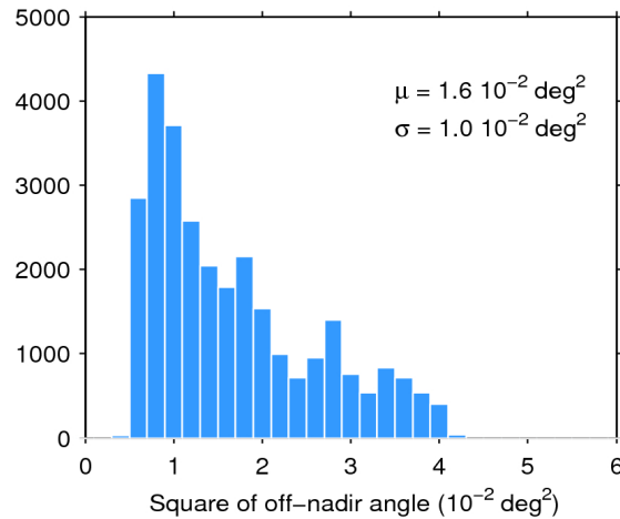
Figure 39. Histogram of flag-valid mispointing over oceans and lakes for 15/03/2016. The mean ( \mu ) and standard deviation ( \sigma ) are also shown. Note that values larger than 6 \cdot 10^{-2} \text{ deg}^2 are excluded from the histogram for the sake of readability but not from the computation of \mu and \sigma .
