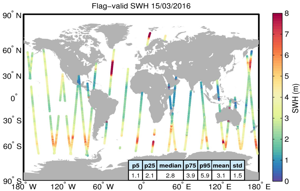
Figure 15. Geographical distribution of flag-valid SWH data over oceans and lakes for 15/03/2016. The statistical values shown in the table refer to the SWH in m and are calculated over all measurements shown in the figure.
