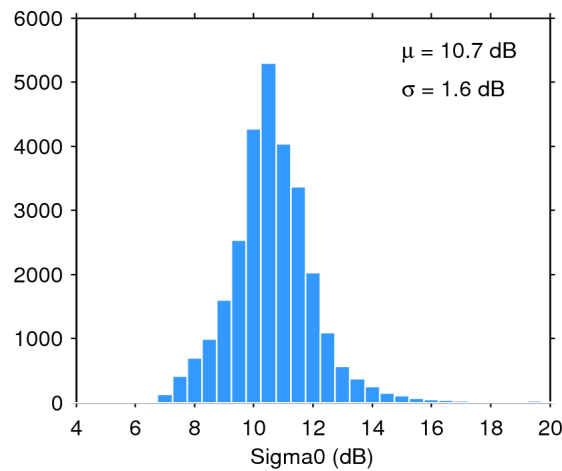
Figure 28. Histogram of science-valid sigma0 over oceans and lakes for 15/03/2016. The mean ( \mu ) and standard deviation ( \sigma ) are also shown. Note that values outside [4 20] dB are excluded from the histogram for the sake of readability but not from the computation of \mu and \sigma .
