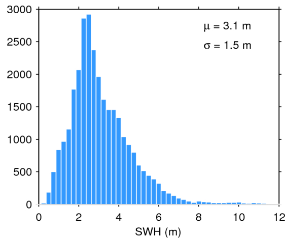
Figure 17. Histogram of flag-valid SWH over oceans and lakes for 15/03/2016. The mean ( \mu ) and standard deviation ( \sigma ) are also shown. Note that values larger than 12 m are excluded from the histogram for the sake of readability but not from the computation of \mu and \sigma .
