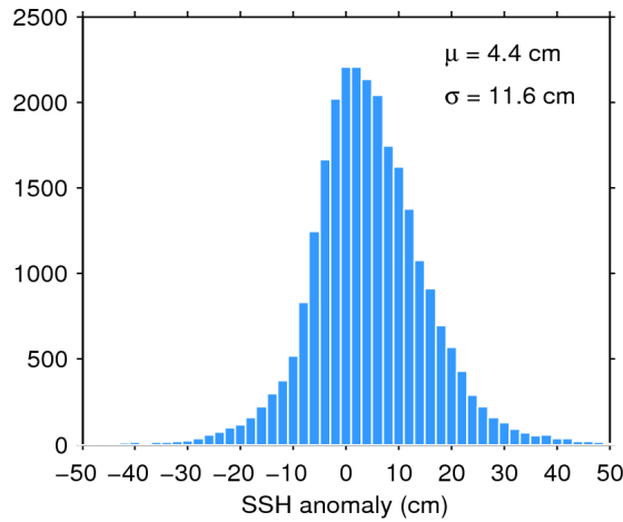
Figure 11. Histogram of science-valid SSH anomaly over oceans and lakes for 15/03/2016. The mean ( \mu ) and standard deviation ( \sigma ) are also shown. Note that values outside [-50 50] cm are excluded from the histogram for the sake of readability but not from the computation of \mu and \sigma .
