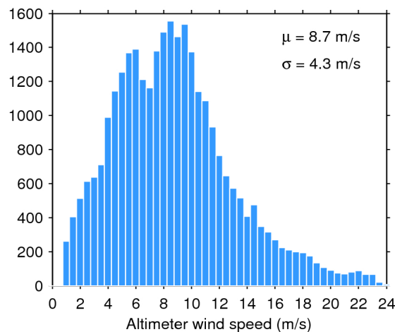
Figure 35. Histogram of science-valid wind over oceans and lakes for 15/03/2016. The mean ( \mu ) and standard deviation ( \sigma ) are also shown. Note that values larger than 24 m/s are excluded from the histogram for the sake of readability but not from the computation of \mu and \sigma .
