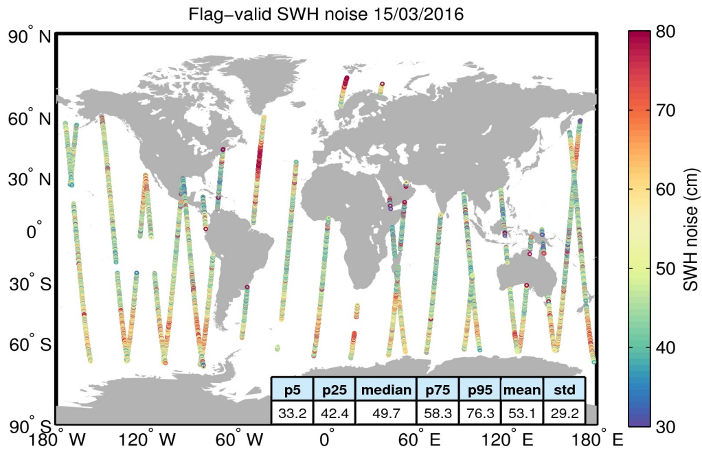
Figure 18. Geographical distribution of flag-valid 20-Hz SWH measurement noise over oceans and lakes for 15/03/2016. The statistical values shown in the figure refer to the SWH noise and are calculated over all measurements shown in the figure.
