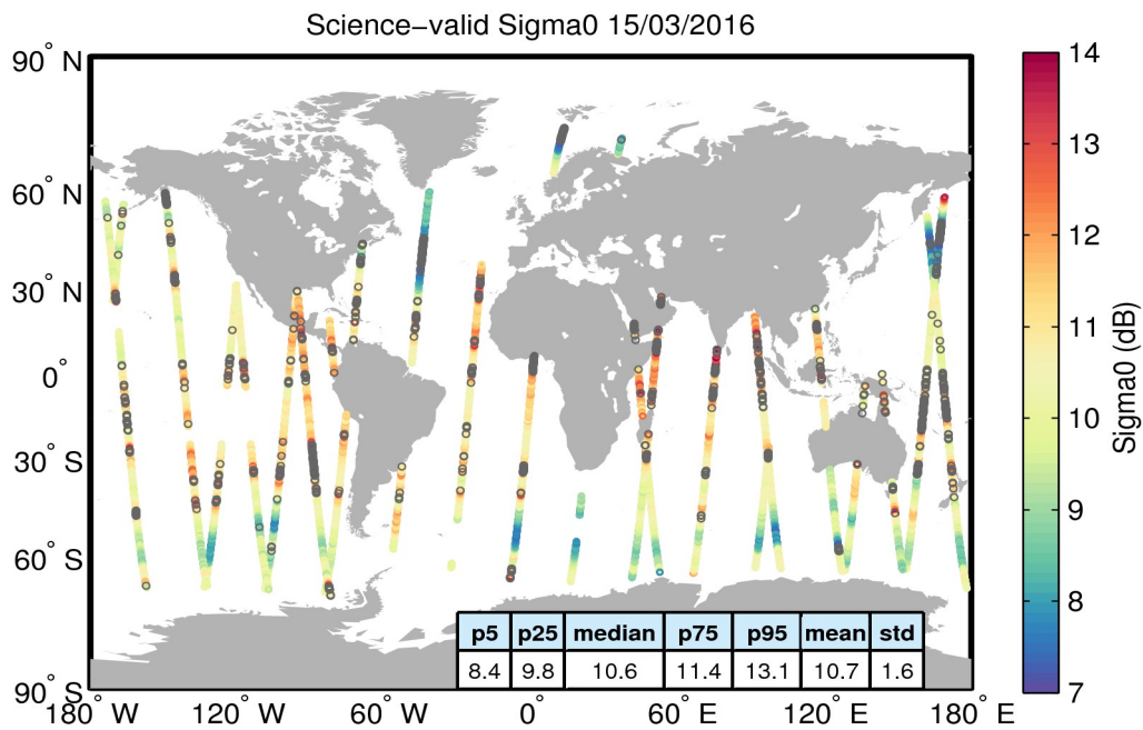
Figure 27. Geographical distribution of science-valid sigma0 data over oceans and lakes for 15/03/2016. The statistical values shown in the table refer to the sigma0 in dB and are calculated over all measurements shown in the figure. Gray circles denote records that have been rejected based on the editing criteria described in Table 4.
