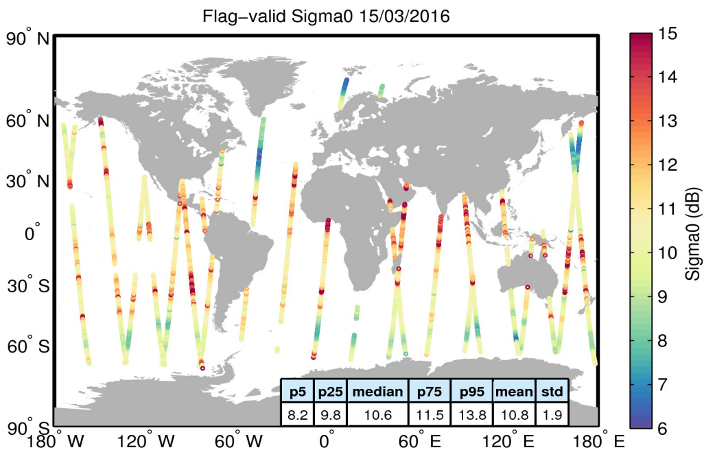
Figure 23. Geographical distribution of flag-valid sigma0 data over oceans and lakes for 15/03/2016. The statistical values shown in the table refer to the sigma0 in dB and are calculated over all measurements shown in the figure.
