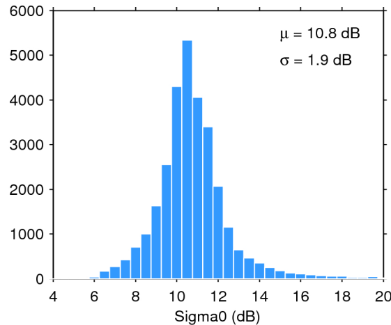
Figure 25. Histogram of flag-valid sigma0 over oceans and lakes for 15/03/2016. The mean ( \mu ) and standard deviation ( \sigma ) are also shown. Note that values outside [4 20] dB are excluded from the histogram for the sake of readability but not from the computation of \mu and \sigma .
