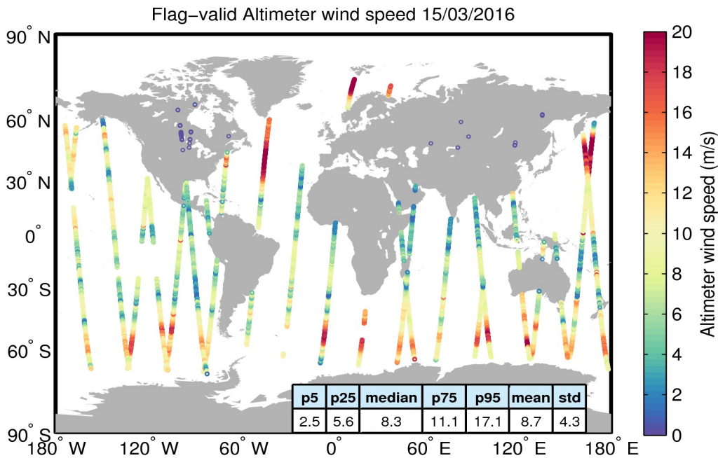
Figure 31. Geographical distribution of flag-valid wind data over oceans and lakes for 15/03/2016. The statistical values shown in the table refer to the wind in m/s and are calculated over all measurements shown in the figure.
