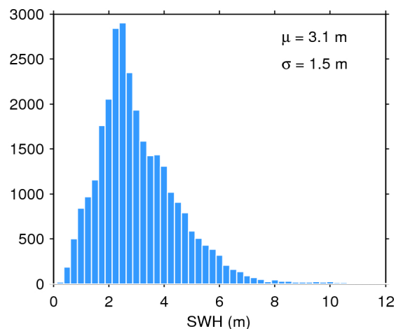
Figure 20. Histogram of science-valid SWH over oceans and lakes for 15/03/2016. The mean ( \mu ) and standard deviation ( \sigma ) are also shown. Note that values larger than 12 m are excluded from the histogram for the sake of readability but not from the computation of \mu and \sigma .
