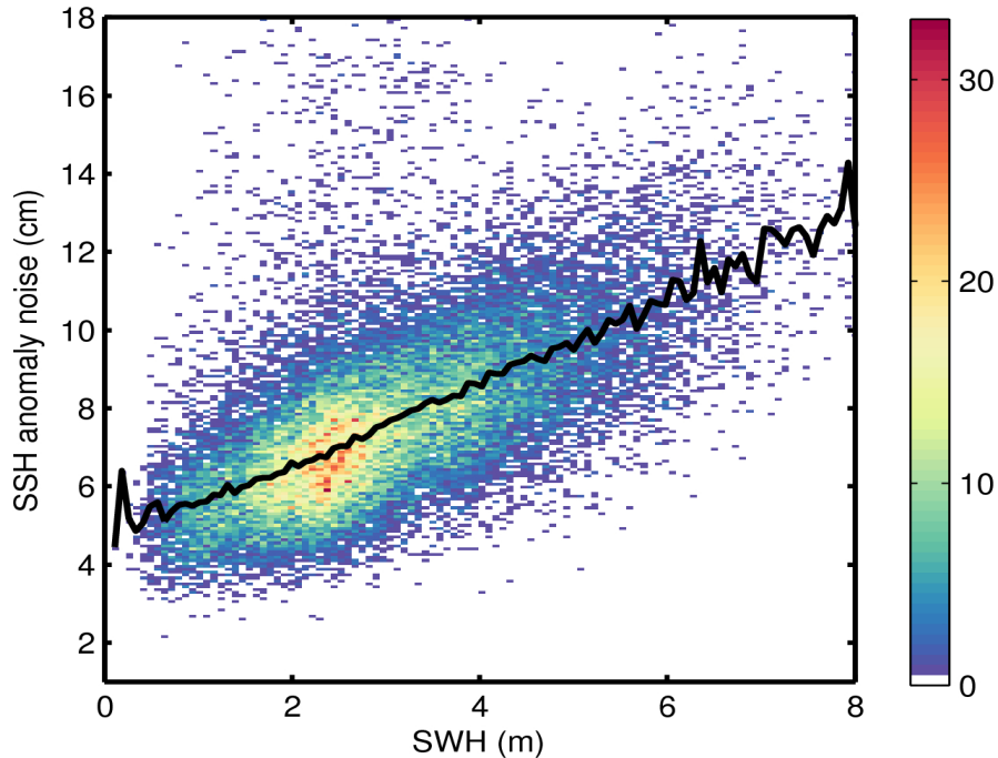
Figure 9. 2D histogram showing flag-valid SSH anomaly noise as a function of SWH for 15/03/2016. The black line denotes the median SSH anomaly noise as a function of SWH.
