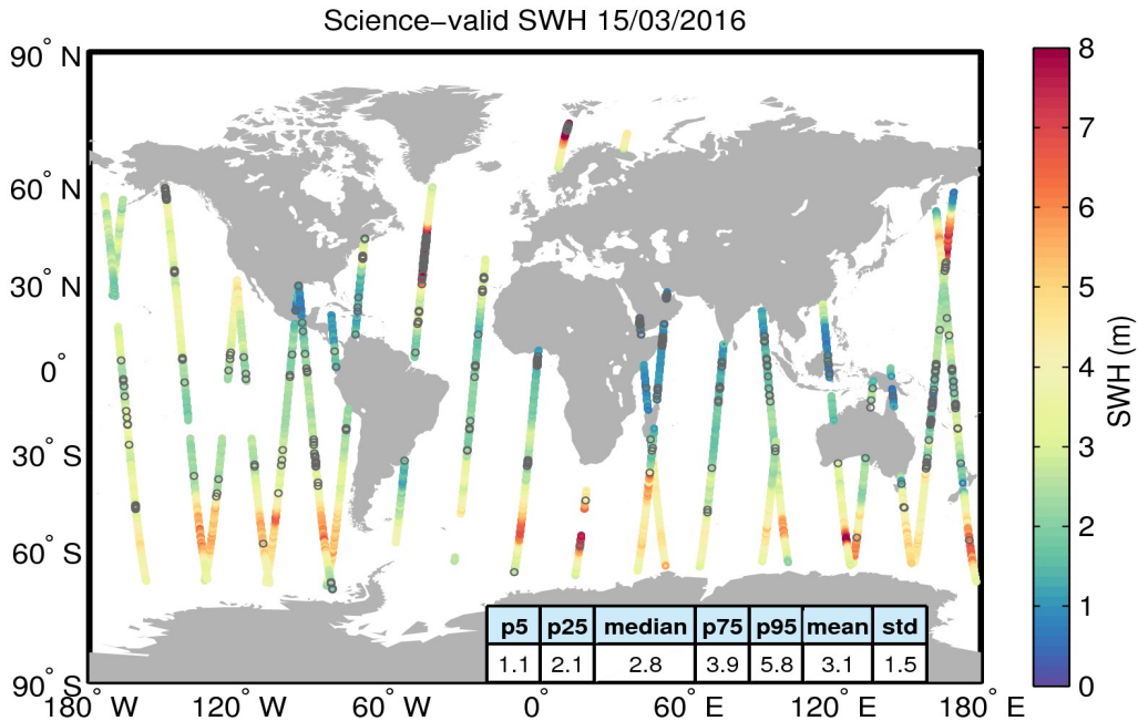
Figure 19. Geographical distribution of science-valid SWH data over oceans and lakes for 15/03/2016. The statistical values shown in the table refer to the SWH in m and are calculated over all measurements shown in the figure. Gray circles denote records that have been rejected based on the editing criteria described in Table 3.
