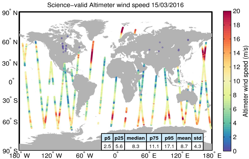
Figure 34. Geographical distribution of science-valid wind data over oceans and lakes for 15/03/2016. The statistical values shown in the table refer to the wind in m/s and are calculated over all measurements shown in the figure. Gray circles denote records that have been rejected based on the editing criteria described in Table 5.
