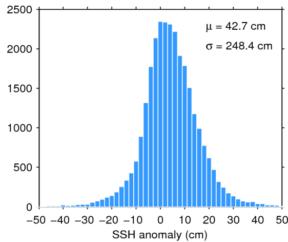
Figure 7. Histogram of flag-valid SSH anomaly over oceans and lakes for 15/03/2016. The mean ( \mu ) and standard deviation ( \sigma ) are also shown. Note that values outside [-50\ 50] cm are excluded from the histogram for the sake of readability but not from the computation of \mu and \sigma .
