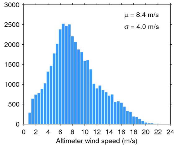
Figure 33. Histogram of flag-valid wind over oceans and lakes for 13/03/2016. The mean ( \mu ) and standard deviation ( \sigma ) are also shown. Note that values larger than 24 m/s are excluded from the histogram for the sake of readability but not from the computation of \mu and \sigma .
