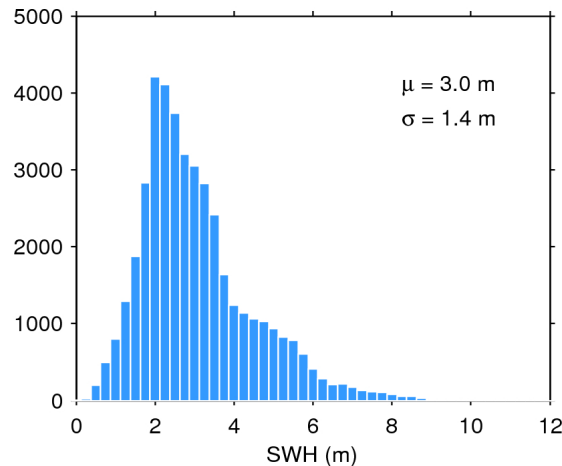
Figure 20. Histogram of science-valid SWH over oceans and lakes for 13/03/2016. The mean ( \mu ) and standard deviation ( \sigma ) are also shown. Note that values larger than 12 m are excluded from the histogram for the sake of readability but not from the computation of \mu and \sigma .
