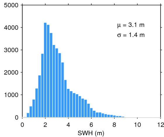
Figure 17. Histogram of flag-valid SWH over oceans and lakes for 13/03/2016. The mean ( \mu ) and standard deviation ( \sigma ) are also shown. Note that values larger than 12 m are excluded from the histogram for the sake of readability but not from the computation of \mu and \sigma .
