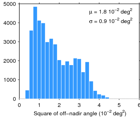
Figure 39. Histogram of flag-valid mispointing over oceans and lakes for 13/03/2016. The mean ( \mu ) and standard deviation ( \sigma ) are also shown. Note that values larger than 6 \cdot 10^{-2} \text{ deg}^2 are excluded from the histogram for the sake of readability but not from the computation of \mu and \sigma .
