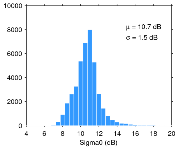
Figure 28. Histogram of science-valid sigma0 over oceans and lakes for 13/03/2016. The mean ( \mu ) and standard deviation ( \sigma ) are also shown. Note that values outside [4 20] dB are excluded from the histogram for the sake of readability but not from the computation of \mu and \sigma .
