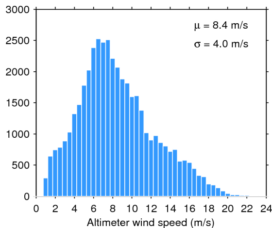
Figure 35. Histogram of science-valid wind over oceans and lakes for 13/03/2016. The mean ( \mu ) and standard deviation ( \sigma ) are also shown. Note that values larger than 24 m/s are excluded from the histogram for the sake of readability but not from the computation of \mu and \sigma .
