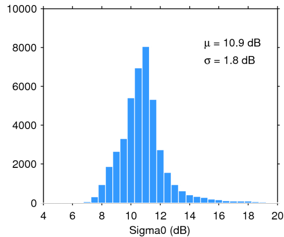
Figure 25. Histogram of flag-valid sigma0 over oceans and lakes for 13/03/2016. The mean ( \mu ) and standard deviation ( \sigma ) are also shown. Note that values outside [4 20] dB are excluded from the histogram for the sake of readability but not from the computation of \mu and \sigma .
