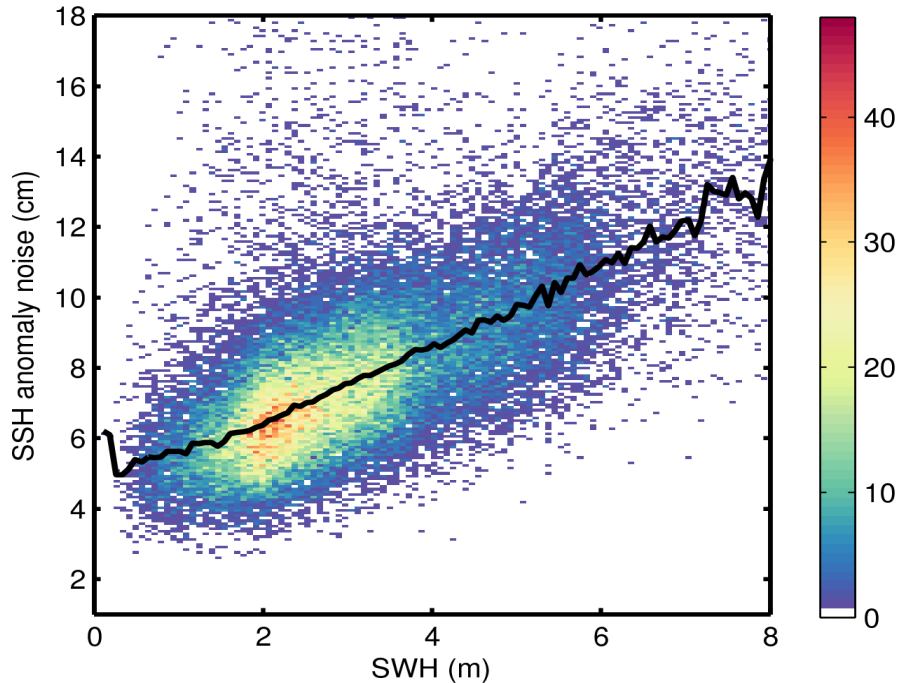
Figure 9. 2D histogram showing flag-valid SSH anomaly noise as a function of SWH for 13/03/2016. The black line denotes the median SSH anomaly noise as a function of SWH.
