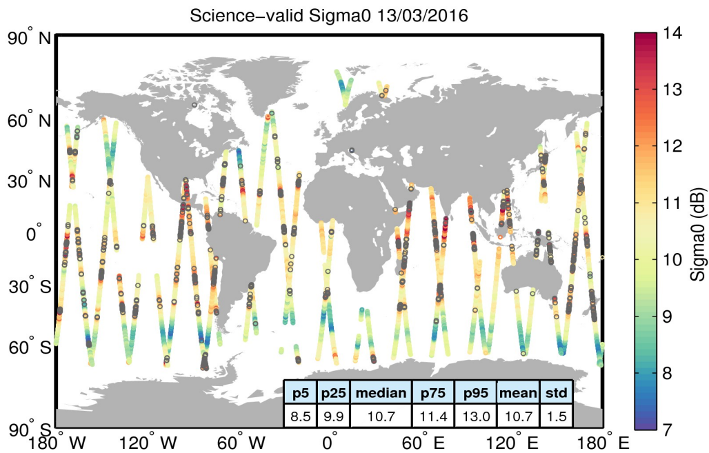
Figure 27. Geographical distribution of science-valid sigma0 data over oceans and lakes for 13/03/2016. The statistical values shown in the table refer to the sigma0 in dB and are calculated over all measurements shown in the figure. Gray circles denote records that have been rejected based on the editing criteria described in Table 4.
