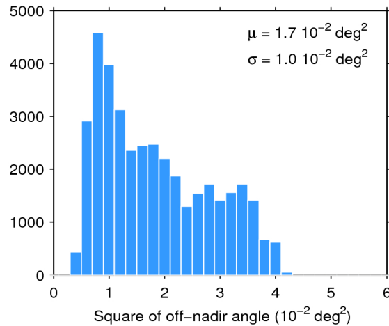
Figure 39. Histogram of flag-valid mispointing over oceans and lakes for 12/03/2016. The mean ( \mu ) and standard deviation ( \sigma ) are also shown. Note that values larger than 6 \cdot 10^{-2} \text{ deg}^2 are excluded from the histogram for the sake of readability but not from the computation of \mu and \sigma .
