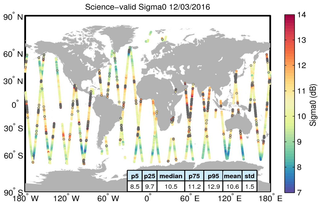
Figure 27. Geographical distribution of science-valid sigma0 data over oceans and lakes for 12/03/2016. The statistical values shown in the table refer to the sigma0 in dB and are calculated over all measurements shown in the figure. Gray circles denote records that have been rejected based on the editing criteria described in Table 4.
