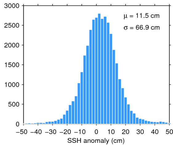
Figure 7. Histogram of flag-valid SSH anomaly over oceans and lakes for 12/03/2016. The mean ( \mu ) and standard deviation ( \sigma ) are also shown. Note that values outside [-50 50] cm are excluded from the histogram for the sake of readability but not from the computation of \mu and \sigma .
