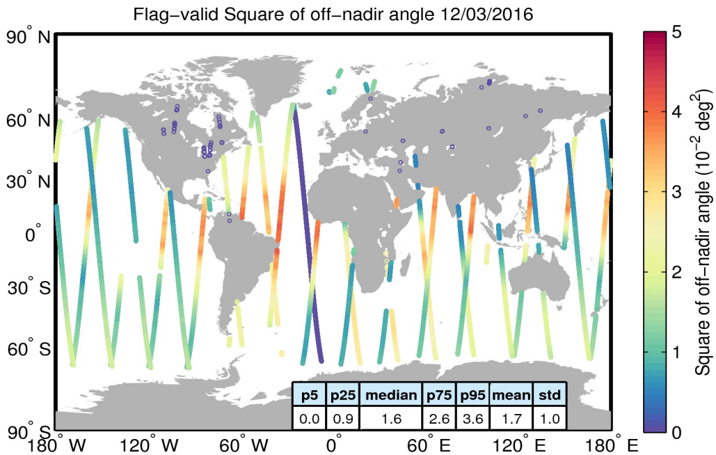
Figure 37. Geographical distribution of flag-valid mispointing data over oceans and lakes for 12/03/2016. The statistical values shown in the table refer to the mispointing in 10^{-2} deg 2 and are calculated over all measurements shown in the figure.
