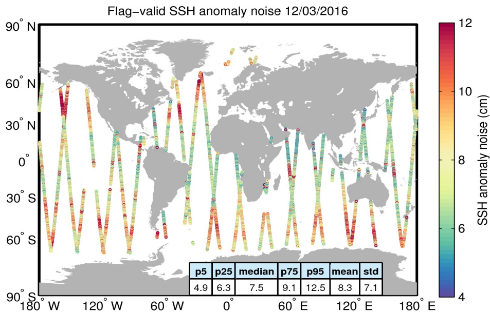
Figure 8. Geographical distribution of flag-valid 20-Hz SSH anomaly measurement noise over oceans and lakes for 12/03/2016. The statistical values shown in the table refer to the SSH anomaly noise and are calculated over all measurements shown in the figure.
