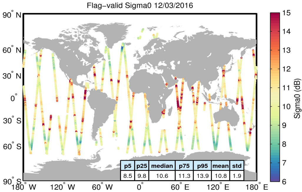
Figure 23. Geographical distribution of flag-valid sigma0 data over oceans and lakes for 12/03/2016. The statistical values shown in the table refer to the sigma0 in dB and are calculated over all measurements shown in the figure.
