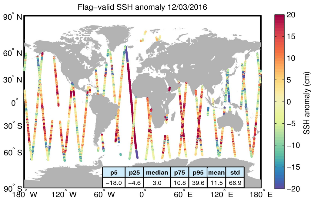
Figure 5. Geographical distribution of flag-valid 1-Hz SSH anomaly data over oceans and lakes for 12/03/2016. The statistical values shown in the table refer to the SSH anomaly in cm and are calculated over all measurements shown in the figure.
