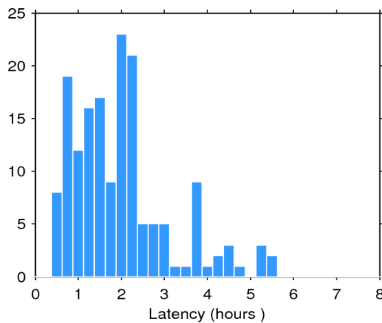
Figure 2. Histogram of the data latency for 12/03/2016. The y-axis denotes the number of files that are made available with a delay of x-hours with respect to the mean time of the records stored in the file.
