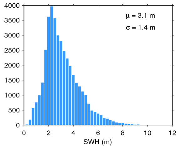
Figure 17. Histogram of flag-valid SWH over oceans and lakes for 12/03/2016. The mean ( \mu ) and standard deviation ( \sigma ) are also shown. Note that values larger than 12 m are excluded from the histogram for the sake of readability but not from the computation of \mu and \sigma .
