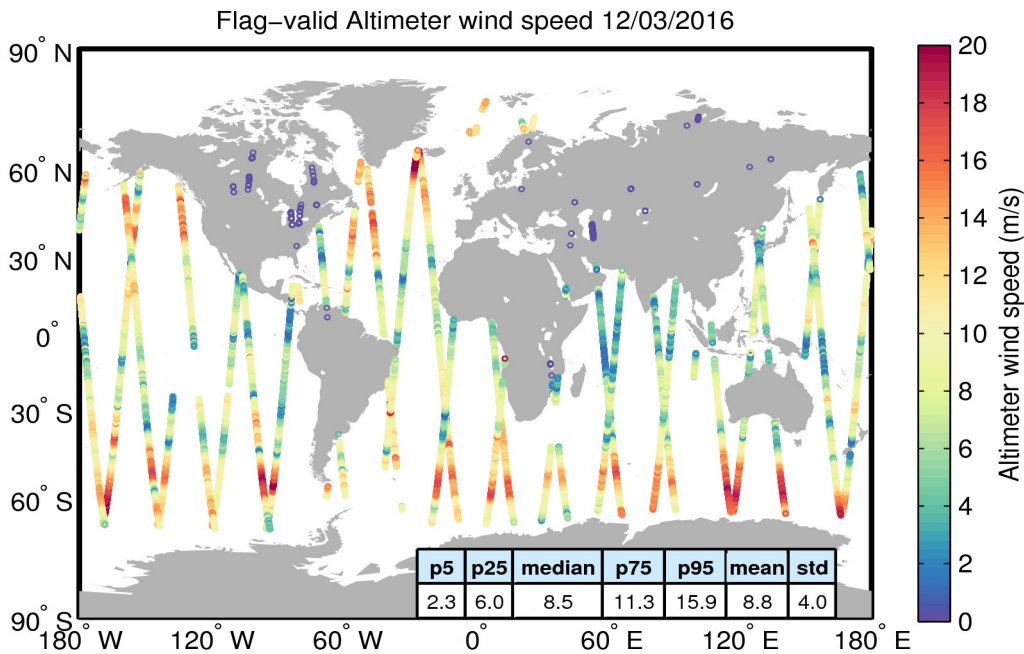
Figure 31. Geographical distribution of flag-valid wind data over oceans and lakes for 12/03/2016. The statistical values shown in the table refer to the wind in m/s and are calculated over all measurements shown in the figure.
