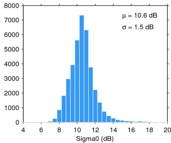
Figure 28. Histogram of science-valid sigma0 over oceans and lakes for 12/03/2016. The mean ( \mu ) and standard deviation ( \sigma ) are also shown. Note that values outside [4 20] dB are excluded from the histogram for the sake of readability but not from the computation of \mu and \sigma .
