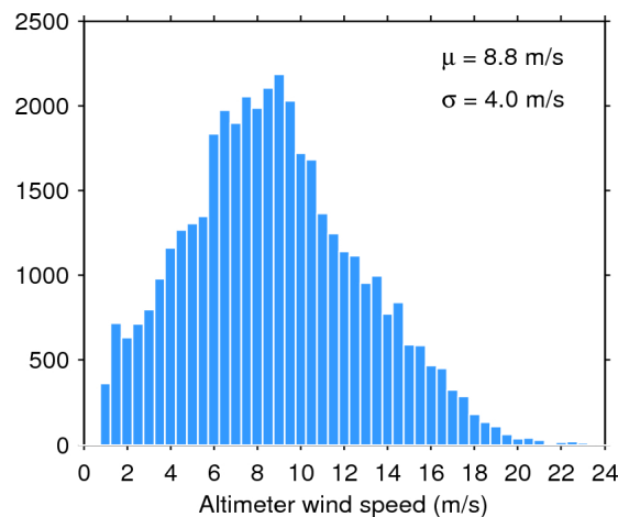
Figure 35. Histogram of science-valid wind over oceans and lakes for 12/03/2016. The mean ( \mu ) and standard deviation ( \sigma ) are also shown. Note that values larger than 24 m/s are excluded from the histogram for the sake of readability but not from the computation of \mu and \sigma .
