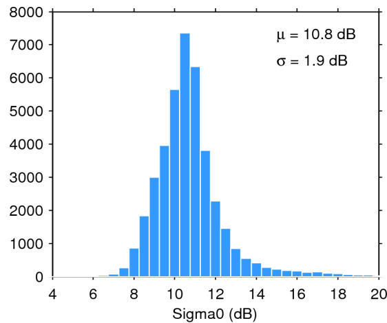
Figure 25. Histogram of flag-valid sigma0 over oceans and lakes for 12/03/2016. The mean ( \mu ) and standard deviation ( \sigma ) are also shown. Note that values outside [4 20] dB are excluded from the histogram for the sake of readability but not from the computation of \mu and \sigma .
