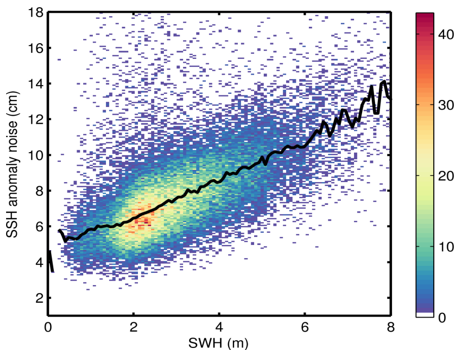
Figure 9. 2D histogram showing flag-valid SSH anomaly noise as a function of SWH for 12/03/2016. The black line denotes the median SSH anomaly noise as a function of SWH.
