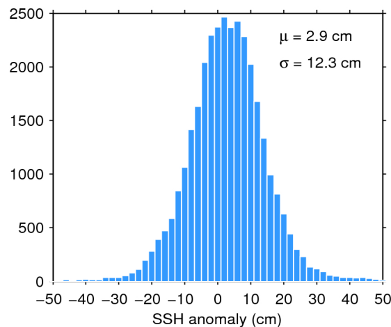
Figure 11. Histogram of science-valid SSH anomaly over oceans and lakes for 12/03/2016. The mean ( \mu ) and standard deviation ( \sigma ) are also shown. Note that values outside [-50 50] cm are excluded from the histogram for the sake of readability but not from the computation of \mu and \sigma .
