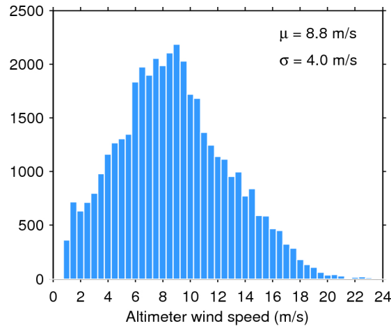
Figure 33. Histogram of flag-valid wind over oceans and lakes for 12/03/2016. The mean ( \mu ) and standard deviation ( \sigma ) are also shown. Note that values larger than 24 m/s are excluded from the histogram for the sake of readability but not from the computation of \mu and \sigma .
