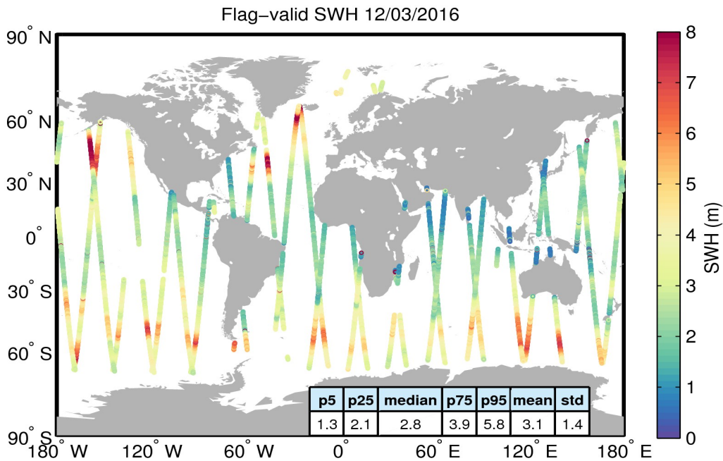
Figure 15. Geographical distribution of flag-valid SWH data over oceans and lakes for 12/03/2016. The statistical values shown in the table refer to the SWH in m and are calculated over all measurements shown in the figure.
