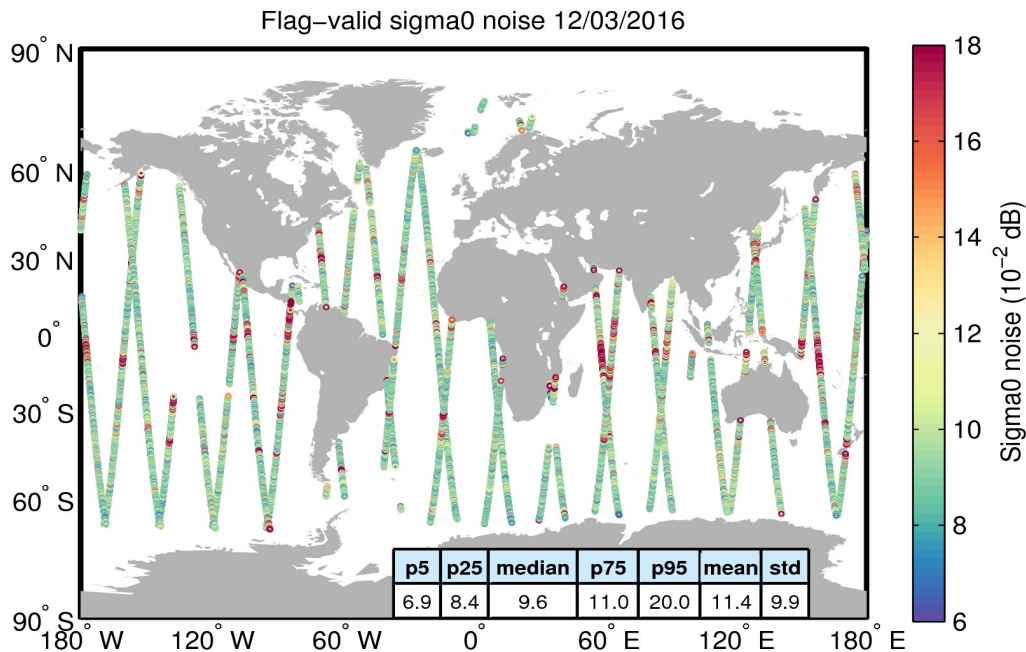
Figure 26. Geographical distribution of flag-valid 20-Hz sigma0 measurement noise over oceans and lakes for 12/03/2016. The statistical values shown in the table refer to the sigma0 noise and are calculated over all measurements shown in the figure.
