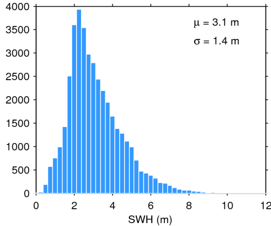
Figure 20. Histogram of science-valid SWH over oceans and lakes for 12/03/2016. The mean ( \mu ) and standard deviation ( \sigma ) are also shown. Note that values larger than 12 m are excluded from the histogram for the sake of readability but not from the computation of \mu and \sigma .
