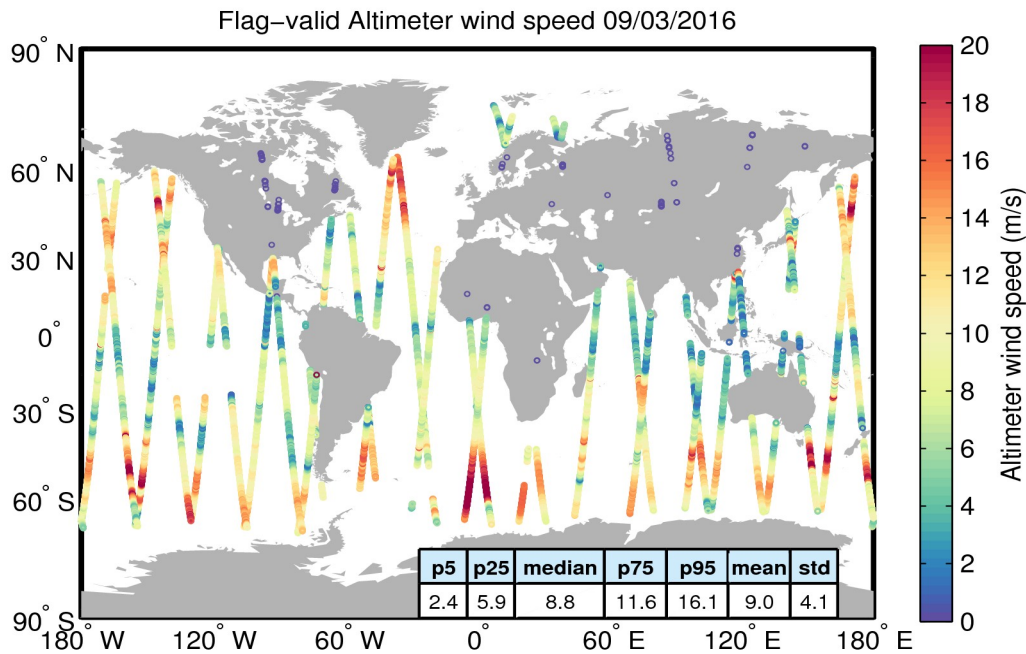
Figure 31. Geographical distribution of flag-valid wind data over oceans and lakes for 09/03/2016. The statistical values shown in the table refer to the wind in m/s and are calculated over all measurements shown in the figure.
