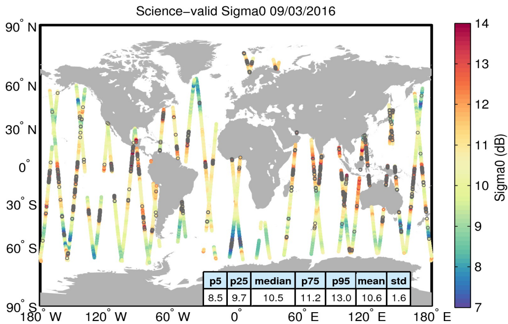
Figure 27. Geographical distribution of science-valid sigma0 data over oceans and lakes for 09/03/2016. The statistical values shown in the table refer to the sigma0 in dB and are calculated over all measurements shown in the figure. Gray circles denote records that have been rejected based on the editing criteria described in Table 4.
