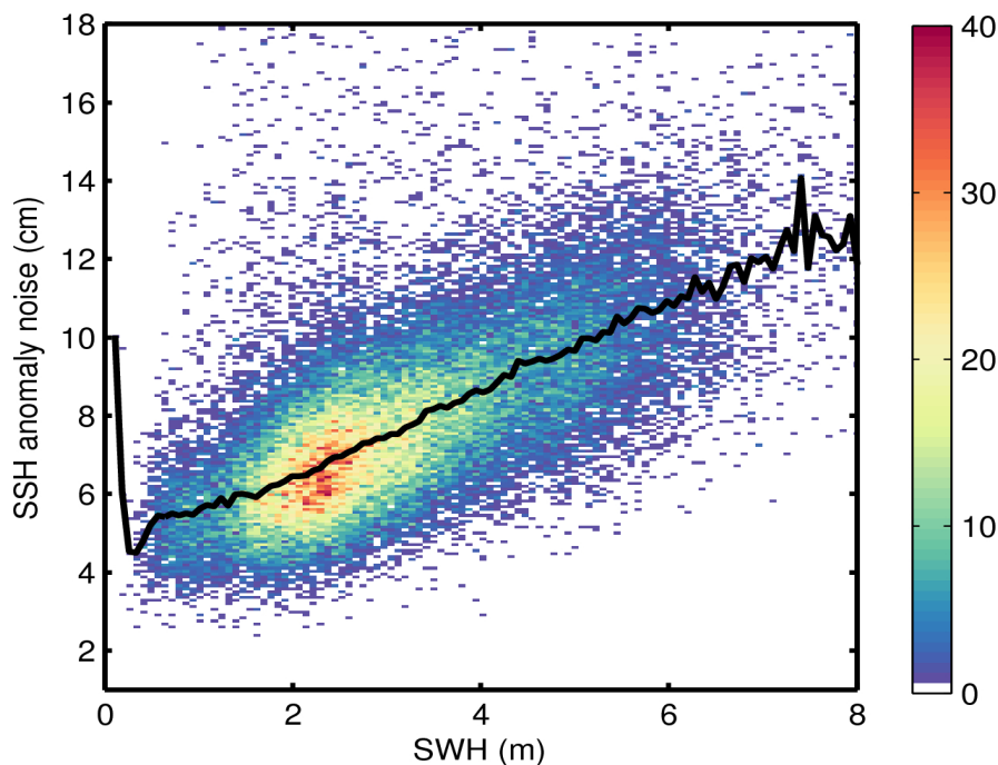
Figure 9. 2D histogram showing flag-valid SSH anomaly noise as a function of SWH for 09/03/2016. The black line denotes the median SSH anomaly noise as a function of SWH.
