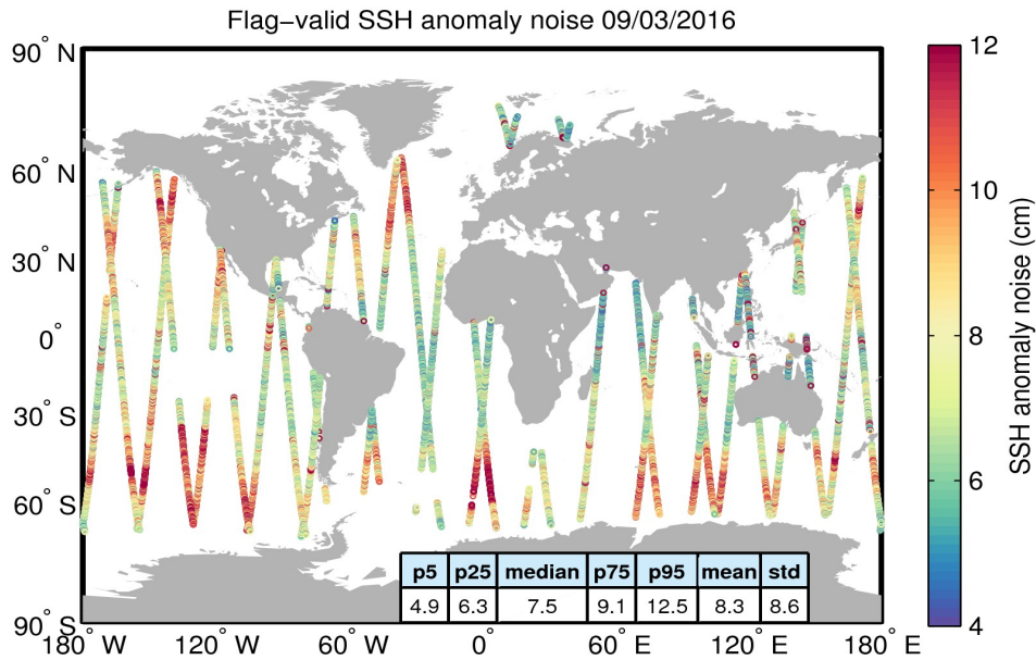
Figure 8. Geographical distribution of flag-valid 20-Hz SSH anomaly measurement noise over oceans and lakes for 09/03/2016. The statistical values shown in the table refer to the SSH anomaly noise and are calculated over all measurements shown in the figure.
