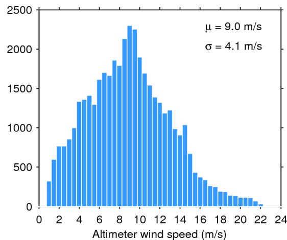
Figure 35. Histogram of science-valid wind over oceans and lakes for 09/03/2016. The mean ( \mu ) and standard deviation ( \sigma ) are also shown. Note that values larger than 24 m/s are excluded from the histogram for the sake of readability but not from the computation of \mu and \sigma .
