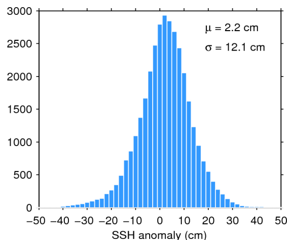
Figure 11. Histogram of science-valid SSH anomaly over oceans and lakes for 09/03/2016. The mean ( \mu ) and standard deviation ( \sigma ) are also shown. Note that values outside [-50 50] cm are excluded from the histogram for the sake of readability but not from the computation of \mu and \sigma .
