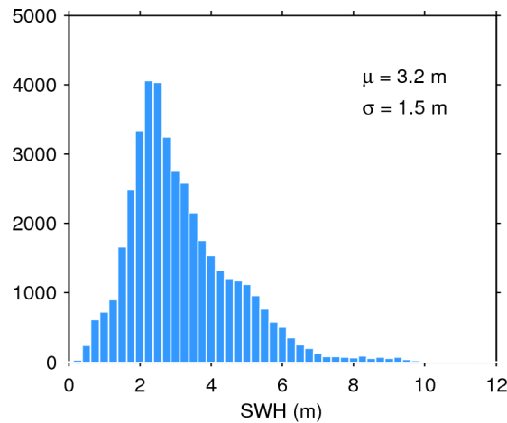
Figure 17. Histogram of flag-valid SWH over oceans and lakes for 09/03/2016. The mean ( \mu ) and standard deviation ( \sigma ) are also shown. Note that values larger than 12 m are excluded from the histogram for the sake of readability but not from the computation of \mu and \sigma .
