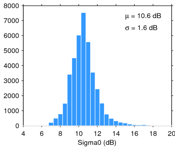
Figure 28. Histogram of science-valid sigma0 over oceans and lakes for 09/03/2016. The mean ( \mu ) and standard deviation ( \sigma ) are also shown. Note that values outside [4 20] dB are excluded from the histogram for the sake of readability but not from the computation of \mu and \sigma .
