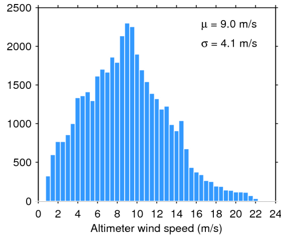
Figure 33. Histogram of flag-valid wind over oceans and lakes for 09/03/2016. The mean ( \mu ) and standard deviation ( \sigma ) are also shown. Note that values larger than 24 m/s are excluded from the histogram for the sake of readability but not from the computation of \mu and \sigma .
