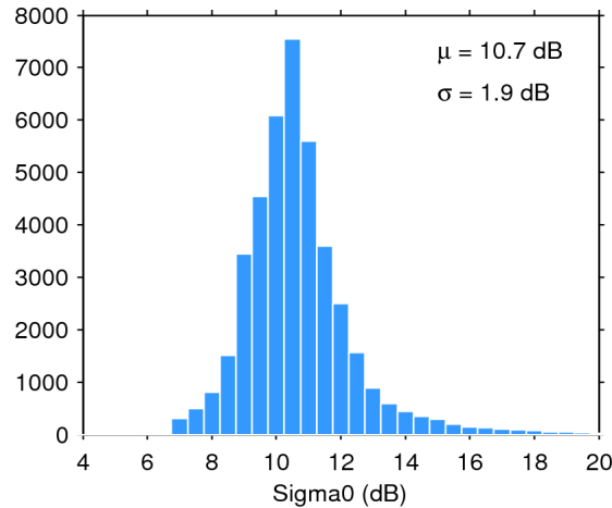
Figure 25. Histogram of flag-valid sigma0 over oceans and lakes for 09/03/2016. The mean ( \mu ) and standard deviation ( \sigma ) are also shown. Note that values outside [4 20] dB are excluded from the histogram for the sake of readability but not from the computation of \mu and \sigma .
