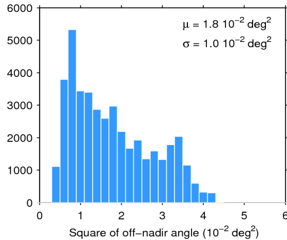
Figure 39. Histogram of flag-valid mispointing over oceans and lakes for 09/03/2016. The mean ( \mu ) and standard deviation ( \sigma ) are also shown. Note that values larger than 6 \cdot 10^{-2} \text{ deg}^2 are excluded from the histogram for the sake of readability but not from the computation of \mu and \sigma .
