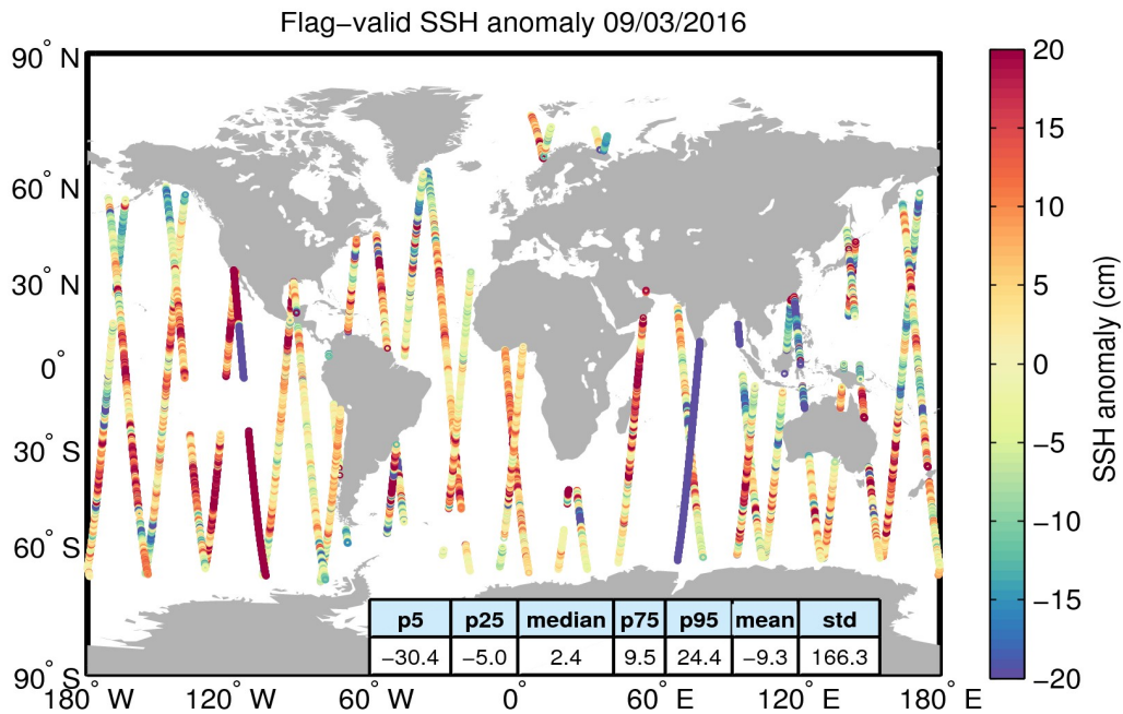
Figure 5. Geographical distribution of flag-valid 1-Hz SSH anomaly data over oceans and lakes for 09/03/2016. The statistical values shown in the table refer to the SSH anomaly in cm and are calculated over all measurements shown in the figure.
