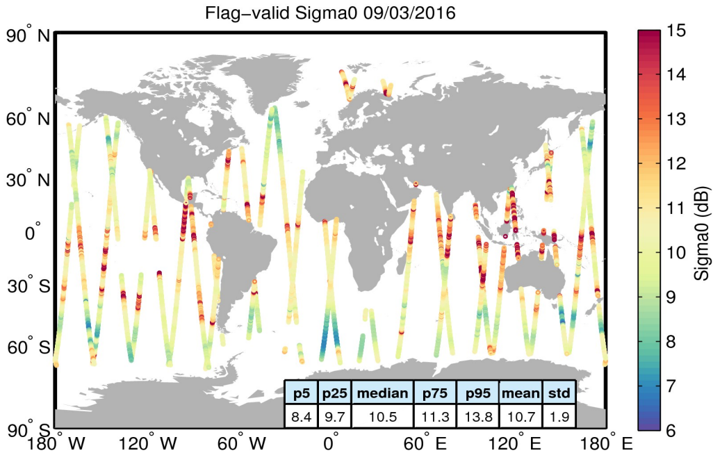
Figure 23. Geographical distribution of flag-valid sigma0 data over oceans and lakes for 09/03/2016. The statistical values shown in the table refer to the sigma0 in dB and are calculated over all measurements shown in the figure.
