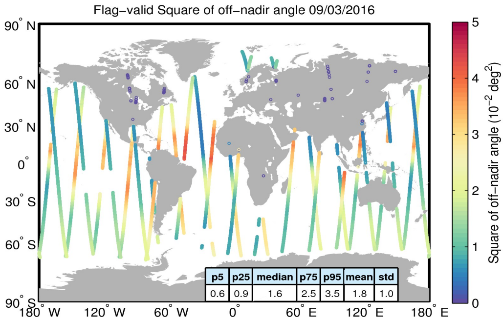
Figure 37. Geographical distribution of flag-valid mispointing data over oceans and lakes for 09/03/2016. The statistical values shown in the table refer to the mispointing in 10^{-2} deg 2 and are calculated over all measurements shown in the figure.
