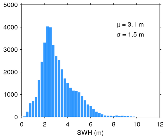
Figure 20. Histogram of science-valid SWH over oceans and lakes for 09/03/2016. The mean ( \mu ) and standard deviation ( \sigma ) are also shown. Note that values larger than 12 m are excluded from the histogram for the sake of readability but not from the computation of \mu and \sigma .
