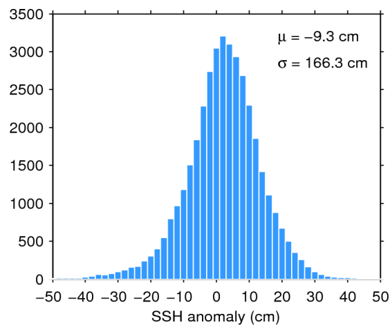
Figure 7. Histogram of flag-valid SSH anomaly over oceans and lakes for 09/03/2016. The mean ( \mu ) and standard deviation ( \sigma ) are also shown. Note that values outside [-50 50] cm are excluded from the histogram for the sake of readability but not from the computation of \mu and \sigma .
