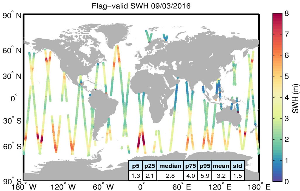
Figure 15. Geographical distribution of flag-valid SWH data over oceans and lakes for 09/03/2016. The statistical values shown in the table refer to the SWH in m and are calculated over all measurements shown in the figure.
