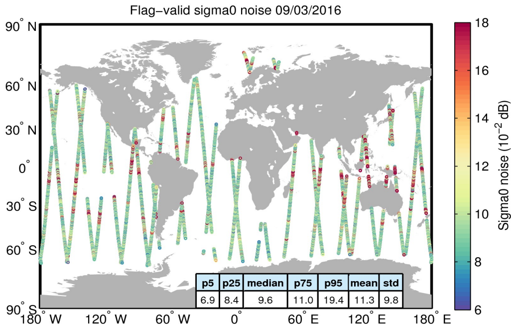
Figure 26. Geographical distribution of flag-valid 20-Hz sigma0 measurement noise over oceans and lakes for 09/03/2016. The statistical values shown in the table refer to the sigma0 noise and are calculated over all measurements shown in the figure.
