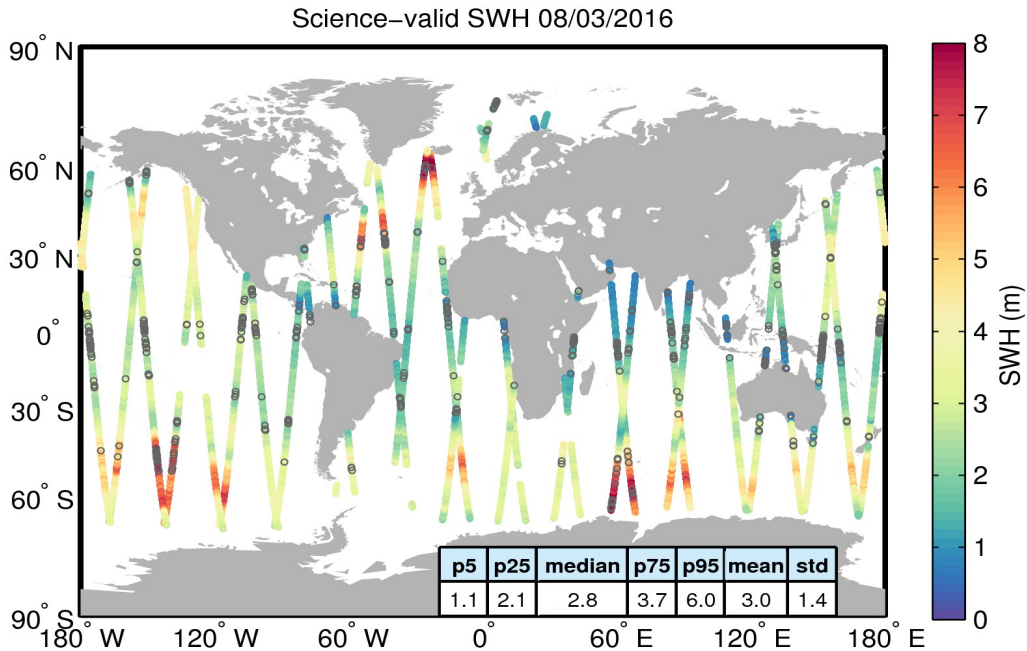
Figure 19. Geographical distribution of science-valid SWH data over oceans and lakes for 08/03/2016. The statistical values shown in the table refer to the SWH in m and are calculated over all measurements shown in the figure. Gray circles denote records that have been rejected based on the editing criteria described in Table 3.
