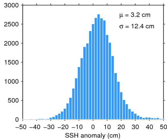
Figure 11. Histogram of science-valid SSH anomaly over oceans and lakes for 08/03/2016. The mean ( \mu ) and standard deviation ( \sigma ) are also shown. Note that values outside [-50 50] cm are excluded from the histogram for the sake of readability but not from the computation of \mu and \sigma .
