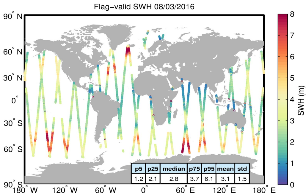
Figure 15. Geographical distribution of flag-valid SWH data over oceans and lakes for 08/03/2016. The statistical values shown in the table refer to the SWH in m and are calculated over all measurements shown in the figure.
