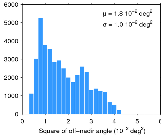
Figure 39. Histogram of flag-valid mispointing over oceans and lakes for 08/03/2016. The mean ( \mu ) and standard deviation ( \sigma ) are also shown. Note that values larger than 6 \cdot 10^{-2} \text{ deg}^2 are excluded from the histogram for the sake of readability but not from the computation of \mu and \sigma .
