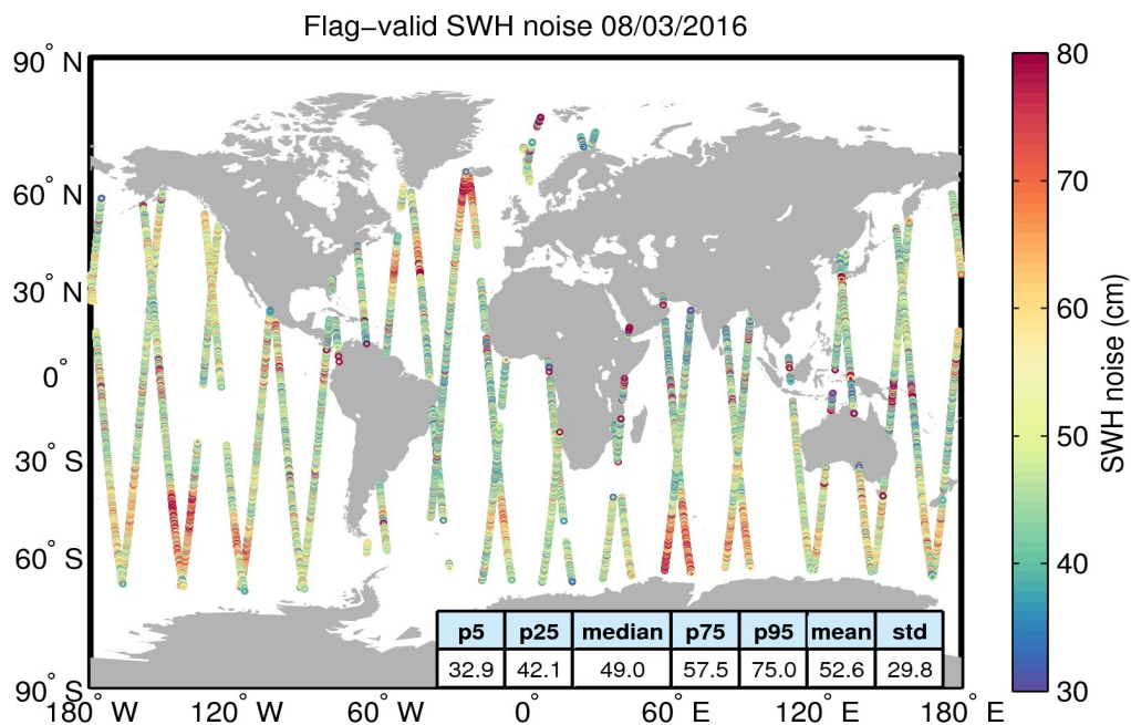
Figure 18. Geographical distribution of flag-valid 20-Hz SWH measurement noise over oceans and lakes for 08/03/2016. The statistical values shown in the table refer to the SWH noise and are calculated over all measurements shown in the figure.
