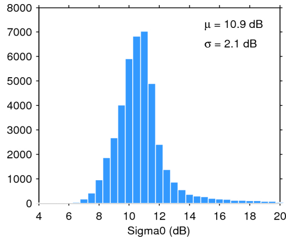
Figure 25. Histogram of flag-valid sigma0 over oceans and lakes for 08/03/2016. The mean ( \mu ) and standard deviation ( \sigma ) are also shown. Note that values outside [4 20] dB are excluded from the histogram for the sake of readability but not from the computation of \mu and \sigma .
