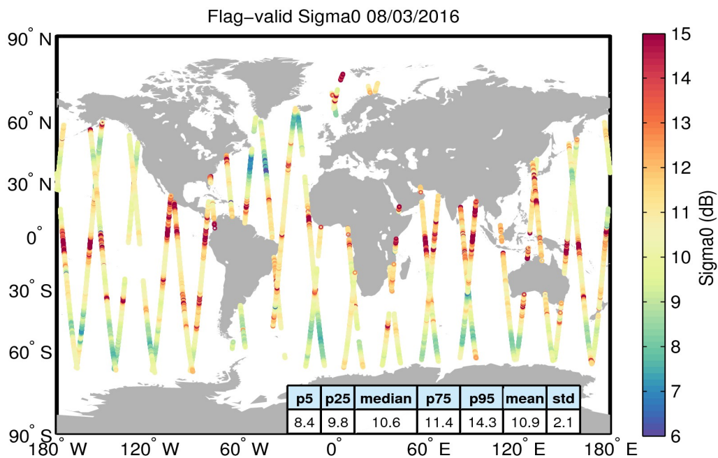
Figure 23. Geographical distribution of flag-valid sigma0 data over oceans and lakes for 08/03/2016. The statistical values shown in the table refer to the sigma0 in dB and are calculated over all measurements shown in the figure.
