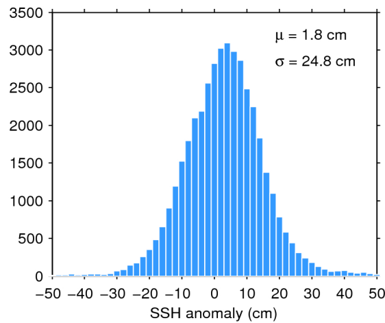
Figure 7. Histogram of flag-valid SSH anomaly over oceans and lakes for 08/03/2016. The mean ( \mu ) and standard deviation ( \sigma ) are also shown. Note that values outside [-50 50] cm are excluded from the histogram for the sake of readability but not from the computation of \mu and \sigma .
