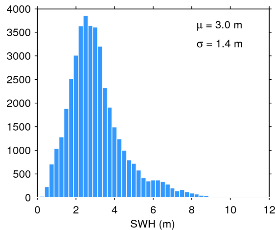
Figure 20. Histogram of science-valid SWH over oceans and lakes for 08/03/2016. The mean ( \mu ) and standard deviation ( \sigma ) are also shown. Note that values larger than 12 m are excluded from the histogram for the sake of readability but not from the computation of \mu and \sigma .
