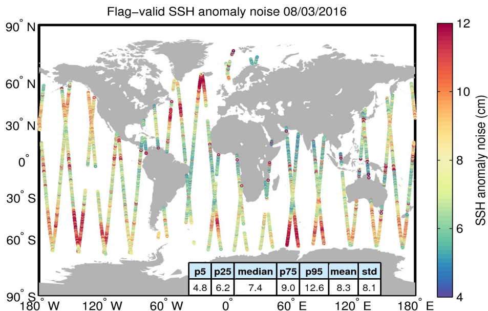
Figure 8. Geographical distribution of flag-valid 20-Hz SSH anomaly measurement noise over oceans and lakes for 08/03/2016. The statistical values shown in the table refer to the SSH anomaly noise and are calculated over all measurements shown in the figure.
