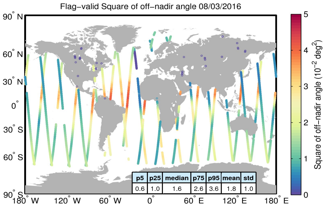
Figure 37. Geographical distribution of flag-valid mispointing data over oceans and lakes for 08/03/2016. The statistical values shown in the table refer to the mispointing in 10^{-2} deg 2 and are calculated over all measurements shown in the figure.
