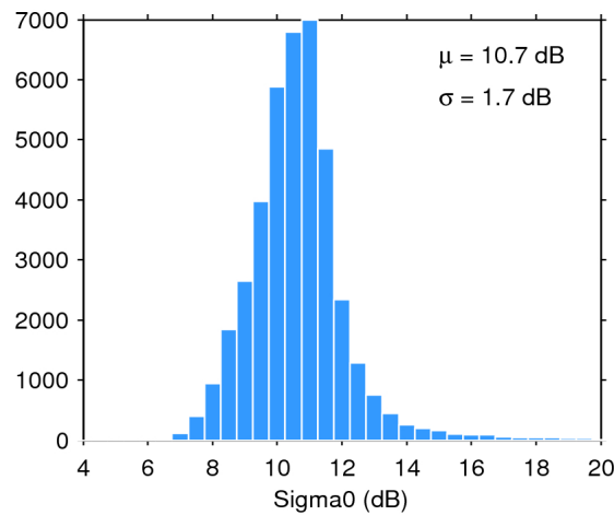
Figure 28. Histogram of science-valid sigma0 over oceans and lakes for 08/03/2016. The mean ( \mu ) and standard deviation ( \sigma ) are also shown. Note that values outside [4 20] dB are excluded from the histogram for the sake of readability but not from the computation of \mu and \sigma .
