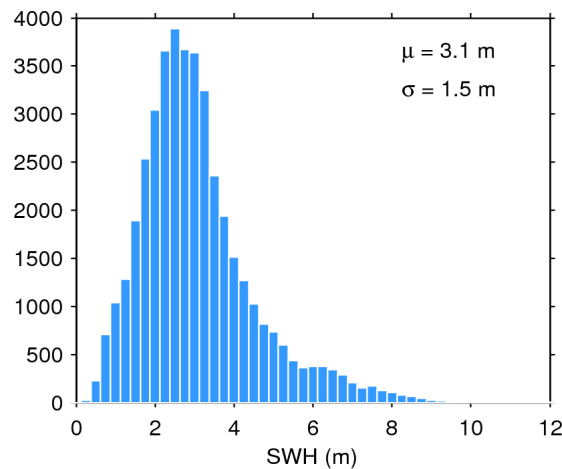
Figure 17. Histogram of flag-valid SWH over oceans and lakes for 08/03/2016. The mean ( \mu ) and standard deviation ( \sigma ) are also shown. Note that values larger than 12 m are excluded from the histogram for the sake of readability but not from the computation of \mu and \sigma .
