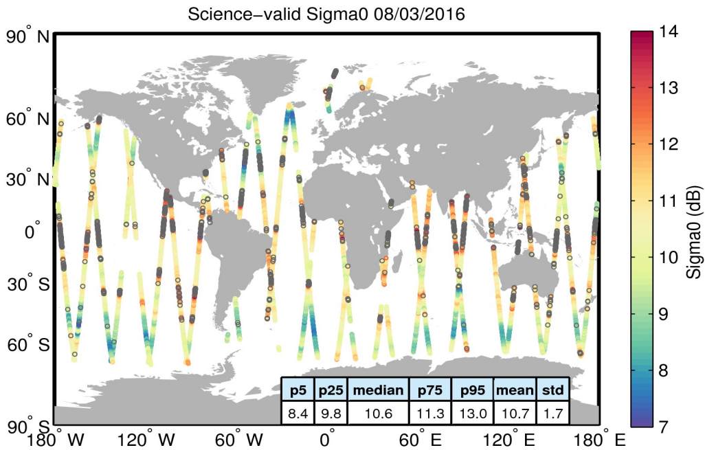
Figure 27. Geographical distribution of science-valid sigma0 data over oceans and lakes for 08/03/2016. The statistical values shown in the table refer to the sigma0 in dB and are calculated over all measurements shown in the figure. Gray circles denote records that have been rejected based on the editing criteria described in Table 4.
