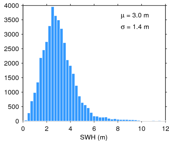
Figure 17. Histogram of flag-valid SWH over oceans and lakes for 06/03/2016. The mean ( \mu ) and standard deviation ( \sigma ) are also shown. Note that values larger than 12 m are excluded from the histogram for the sake of readability but not from the computation of \mu and \sigma .
