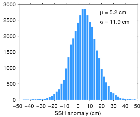
Figure 11. Histogram of science-valid SSH anomaly over oceans and lakes for 06/03/2016. The mean ( \mu ) and standard deviation ( \sigma ) are also shown. Note that values outside [-50 50] cm are excluded from the histogram for the sake of readability but not from the computation of \mu and \sigma .
