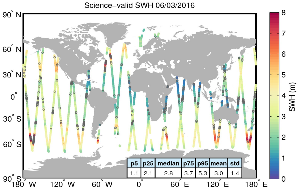
Figure 19. Geographical distribution of science-valid SWH data over oceans and lakes for 06/03/2016. The statistical values shown in the table refer to the SWH in m and are calculated over all measurements shown in the figure. Gray circles denote records that have been rejected based on the editing criteria described in Table 3.
