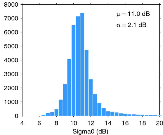
Figure 25. Histogram of flag-valid sigma0 over oceans and lakes for 06/03/2016. The mean ( \mu ) and standard deviation ( \sigma ) are also shown. Note that values outside [4 20] dB are excluded from the histogram for the sake of readability but not from the computation of \mu and \sigma .
