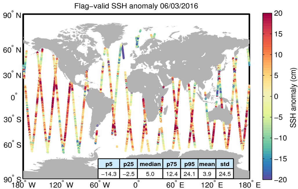
Figure 5. Geographical distribution of flag-valid 1-Hz SSH anomaly data over oceans and lakes for 06/03/2016. The statistical values shown in the table refer to the SSH anomaly in cm and are calculated over all measurements shown in the figure.
