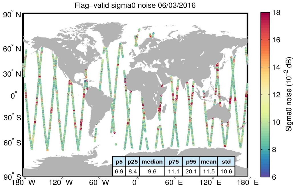
Figure 26. Geographical distribution of flag-valid 20-Hz sigma0 measurement noise over oceans and lakes for 06/03/2016. The statistical values shown in the table refer to the sigma0 noise and are calculated over all measurements shown in the figure.
