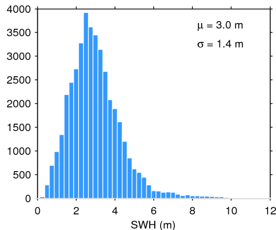
Figure 20. Histogram of science-valid SWH over oceans and lakes for 06/03/2016. The mean ( \mu ) and standard deviation ( \sigma ) are also shown. Note that values larger than 12 m are excluded from the histogram for the sake of readability but not from the computation of \mu and \sigma .
