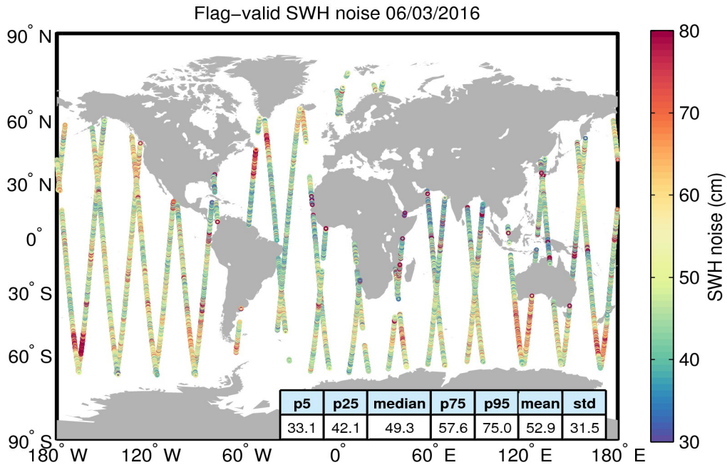
Figure 18. Geographical distribution of flag-valid 20-Hz SWH measurement noise over oceans and lakes for 06/03/2016. The statistical values shown in the figure refer to the SWH noise and are calculated over all measurements shown in the figure.
