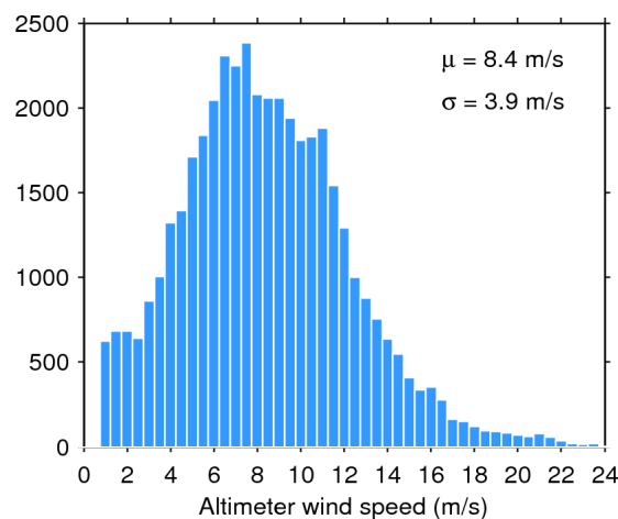
Figure 35. Histogram of science-valid wind over oceans and lakes for 06/03/2016. The mean ( \mu ) and standard deviation ( \sigma ) are also shown. Note that values larger than 24 m/s are excluded from the histogram for the sake of readability but not from the computation of \mu and \sigma .
