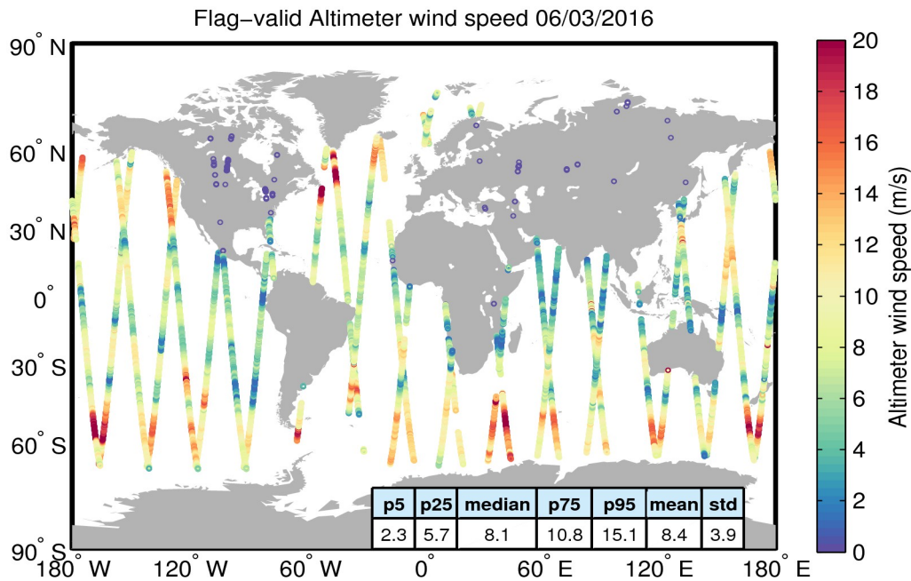
Figure 31. Geographical distribution of flag-valid wind data over oceans and lakes for 06/03/2016. The statistical values shown in the table refer to the wind in m/s and are calculated over all measurements shown in the figure.
