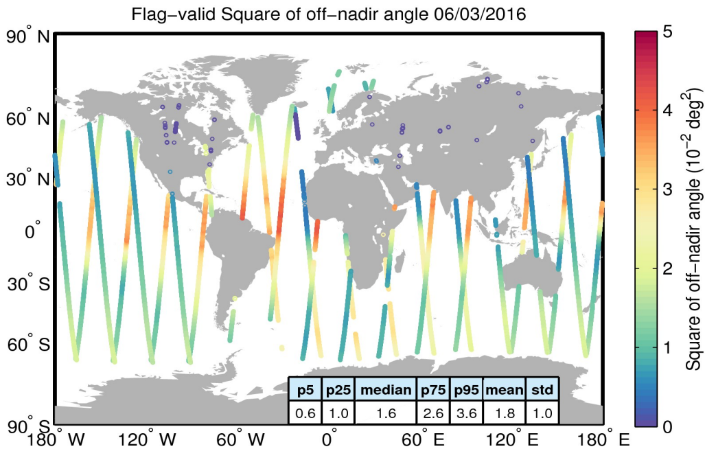
Figure 37. Geographical distribution of flag-valid mispointing data over oceans and lakes for 06/03/2016. The statistical values shown in the table refer to the mispointing in 10^{-2} deg 2 and are calculated over all measurements shown in the figure.
