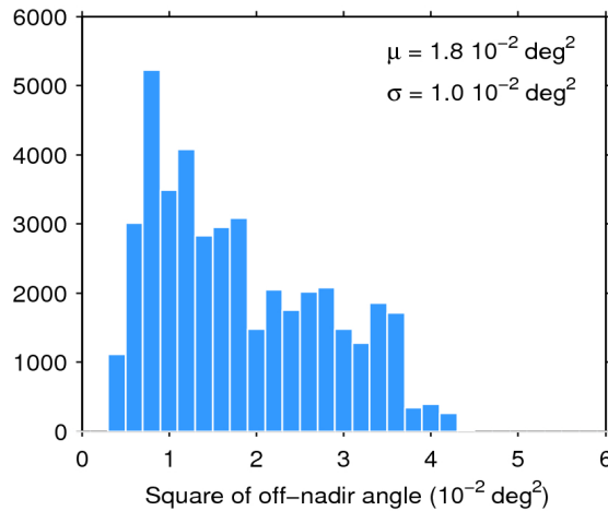
Figure 39. Histogram of flag-valid mispointing over oceans and lakes for 06/03/2016. The mean ( \mu ) and standard deviation ( \sigma ) are also shown. Note that values larger than 6 \cdot 10^{-2} \text{ deg}^2 are excluded from the histogram for the sake of readability but not from the computation of \mu and \sigma .
