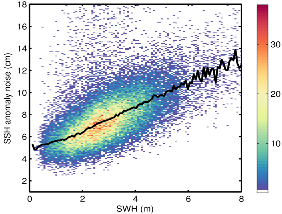
Figure 9. 2D histogram showing flag-valid SSH anomaly noise as a function of SWH for 06/03/2016. The black line denotes the median SSH anomaly noise as a function of SWH.
