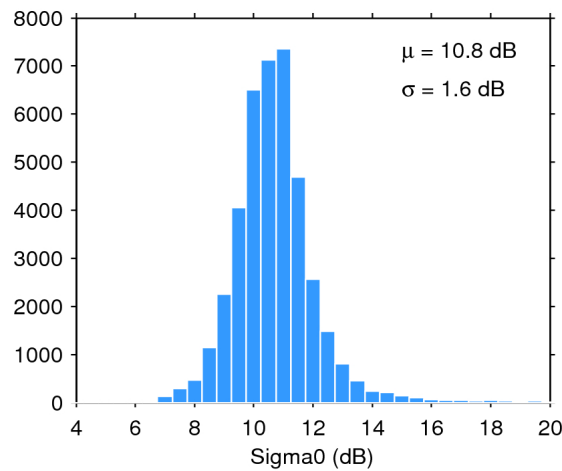
Figure 28. Histogram of science-valid sigma0 over oceans and lakes for 06/03/2016. The mean ( \mu ) and standard deviation ( \sigma ) are also shown. Note that values outside [4 20] dB are excluded from the histogram for the sake of readability but not from the computation of \mu and \sigma .
