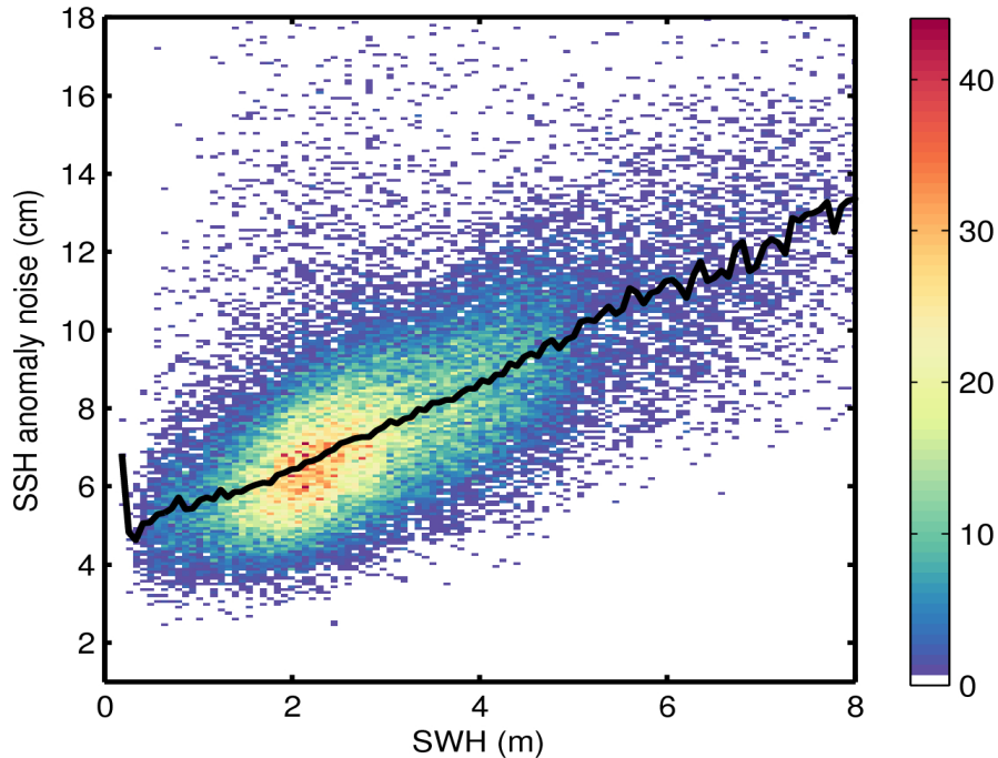
Figure 9. 2D histogram showing flag-valid SSH anomaly noise as a function of SWH for 03/03/2016. The black line denotes the median SSH anomaly noise as a function of SWH.
