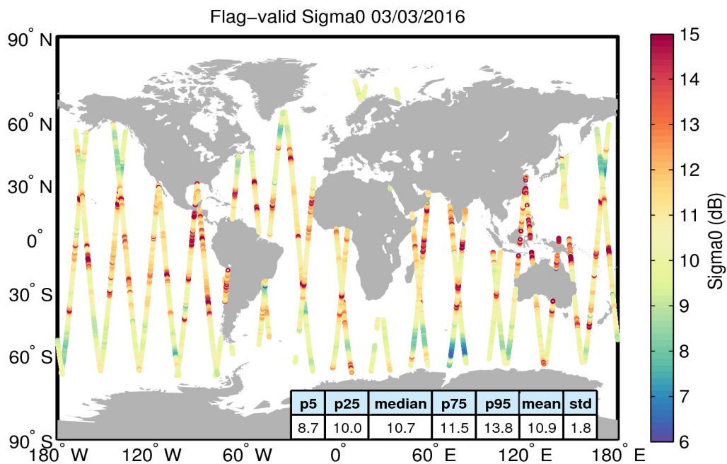
Figure 23. Geographical distribution of flag-valid sigma0 data over oceans and lakes for 03/03/2016. The statistical values shown in the table refer to the sigma0 in dB and are calculated over all measurements shown in the figure.
