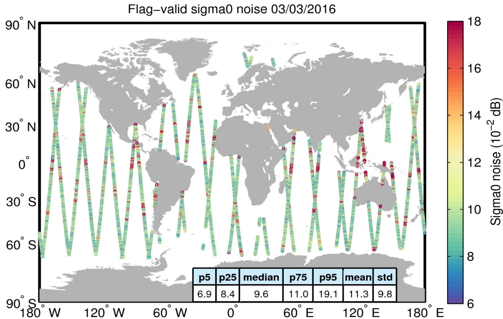
Figure 26. Geographical distribution of flag-valid 20-Hz sigma0 measurement noise over oceans and lakes for 03/03/2016. The statistical values shown in the table refer to the sigma0 noise and are calculated over all measurements shown in the figure.
