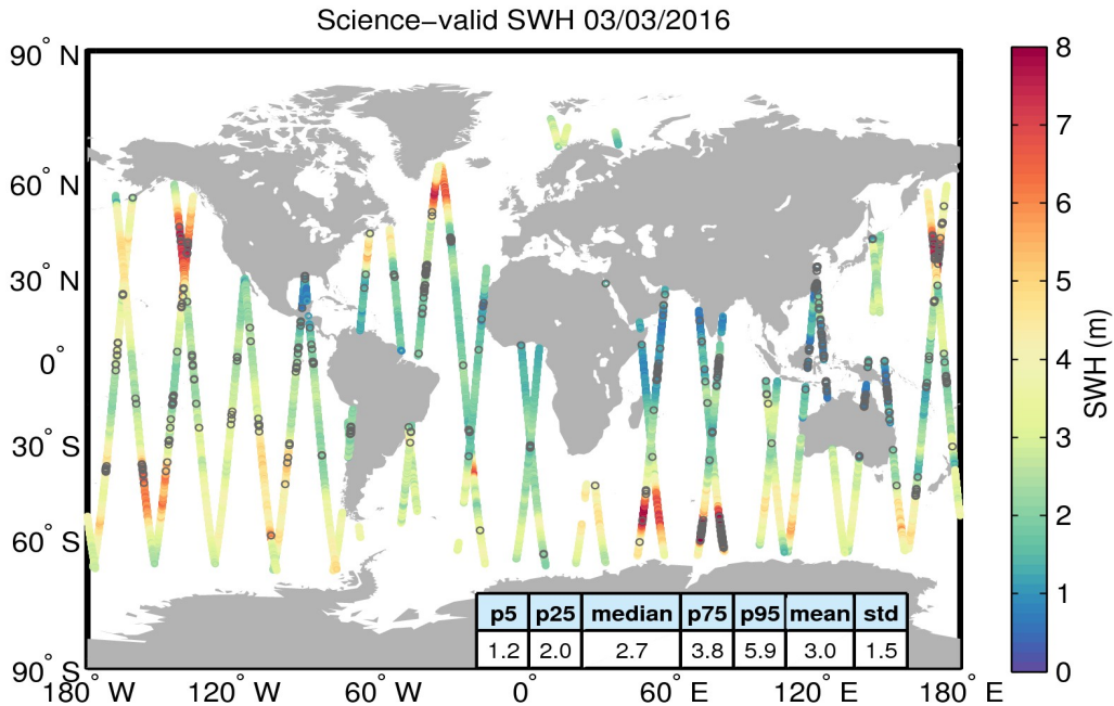
Figure 19. Geographical distribution of science-valid SWH data over oceans and lakes for 03/03/2016. The statistical values shown in the table refer to the SWH in m and are calculated over all measurements shown in the figure. Gray circles denote records that have been rejected based on the editing criteria described in Table 3.
