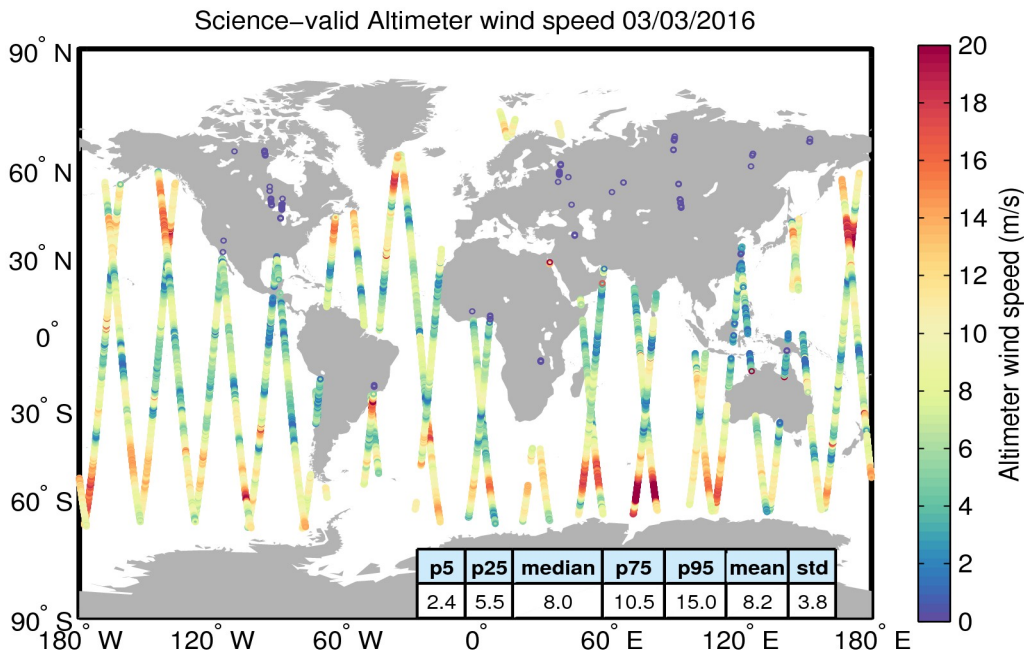
Figure 34. Geographical distribution of science-valid wind data over oceans and lakes for 03/03/2016. The statistical values shown in the table refer to the wind in m/s and are calculated over all measurements shown in the figure. Gray circles denote records that have been rejected based on the editing criteria described in Table 5.
