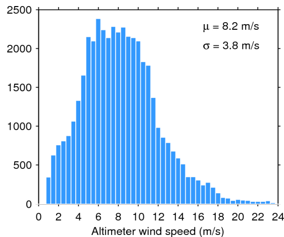
Figure 35. Histogram of science-valid wind over oceans and lakes for 03/03/2016. The mean ( \mu ) and standard deviation ( \sigma ) are also shown. Note that values larger than 24 m/s are excluded from the histogram for the sake of readability but not from the computation of \mu and \sigma .
