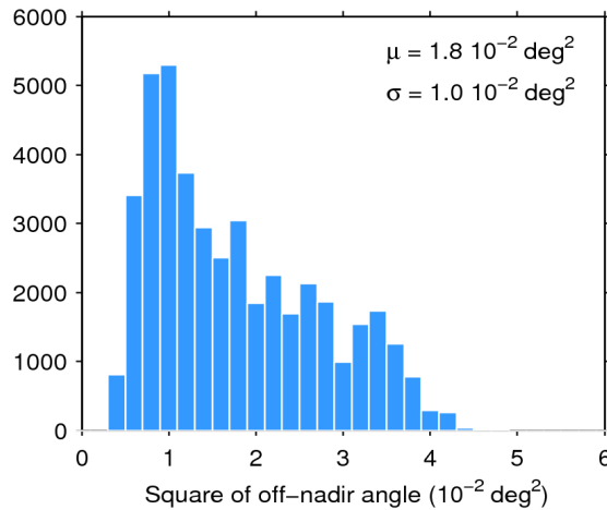
Figure 39. Histogram of flag-valid mispointing over oceans and lakes for 03/03/2016. The mean ( \mu ) and standard deviation ( \sigma ) are also shown. Note that values larger than 6 \cdot 10^{-2} \text{ deg}^2 are excluded from the histogram for the sake of readability but not from the computation of \mu and \sigma .
