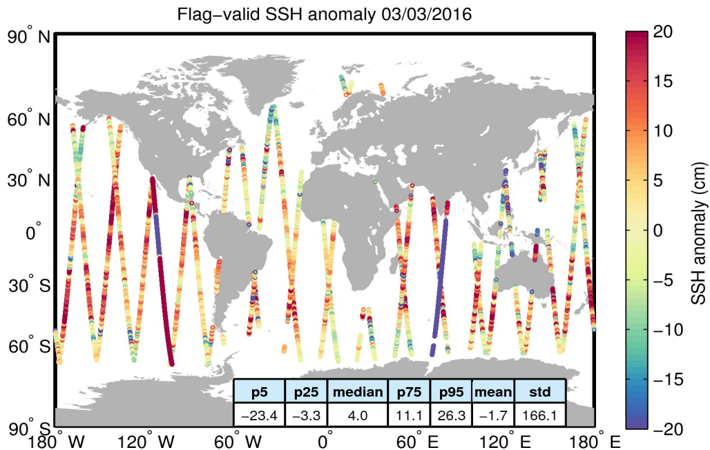
Figure 5. Geographical distribution of flag-valid 1-Hz SSH anomaly data over oceans and lakes for 03/03/2016. The statistical values shown in the table refer to the SSH anomaly in cm and are calculated over all measurements shown in the figure.
