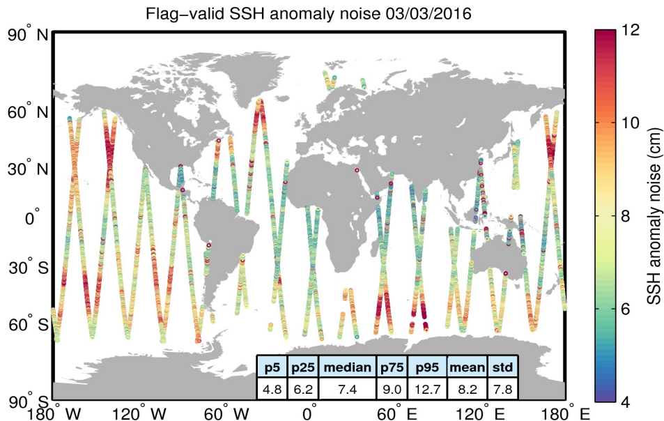
Figure 8. Geographical distribution of flag-valid 20-Hz SSH anomaly measurement noise over oceans and lakes for 03/03/2016. The statistical values shown in the table refer to the SSH anomaly noise and are calculated over all measurements shown in the figure.
