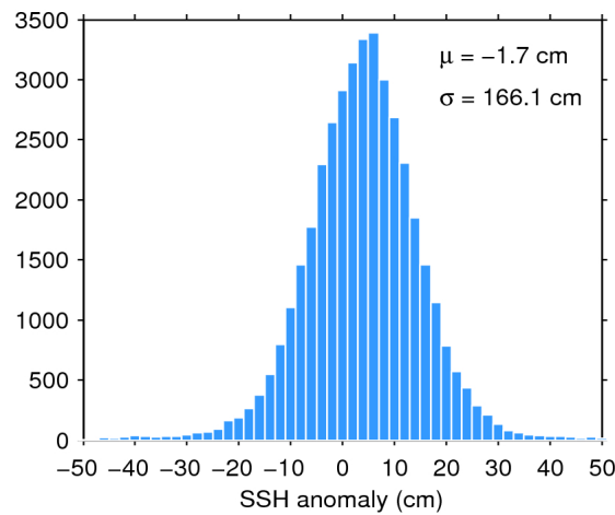
Figure 7. Histogram of flag-valid SSH anomaly over oceans and lakes for 03/03/2016. The mean ( \mu ) and standard deviation ( \sigma ) are also shown. Note that values outside [-50\ 50] cm are excluded from the histogram for the sake of readability but not from the computation of \mu and \sigma .
