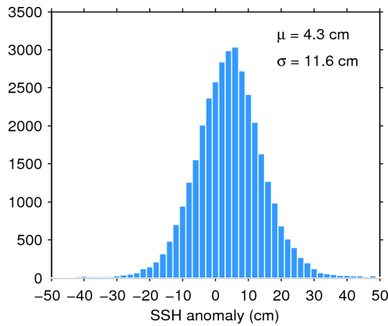
Figure 11. Histogram of science-valid SSH anomaly over oceans and lakes for 03/03/2016. The mean ( \mu ) and standard deviation ( \sigma ) are also shown. Note that values outside [-50 50] cm are excluded from the histogram for the sake of readability but not from the computation of \mu and \sigma .
