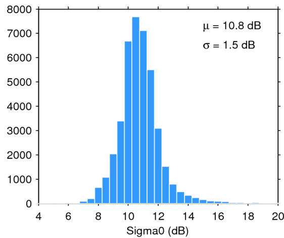
Figure 28. Histogram of science-valid sigma0 over oceans and lakes for 03/03/2016. The mean ( \mu ) and standard deviation ( \sigma ) are also shown. Note that values outside [4 20] dB are excluded from the histogram for the sake of readability but not from the computation of \mu and \sigma .
