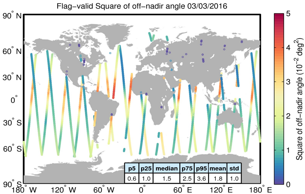
Figure 37. Geographical distribution of flag-valid mispointing data over oceans and lakes for 03/03/2016. The statistical values shown in the table refer to the mispointing in 10^{-2} \text{ deg}^2 and are calculated over all measurements shown in the figure.
