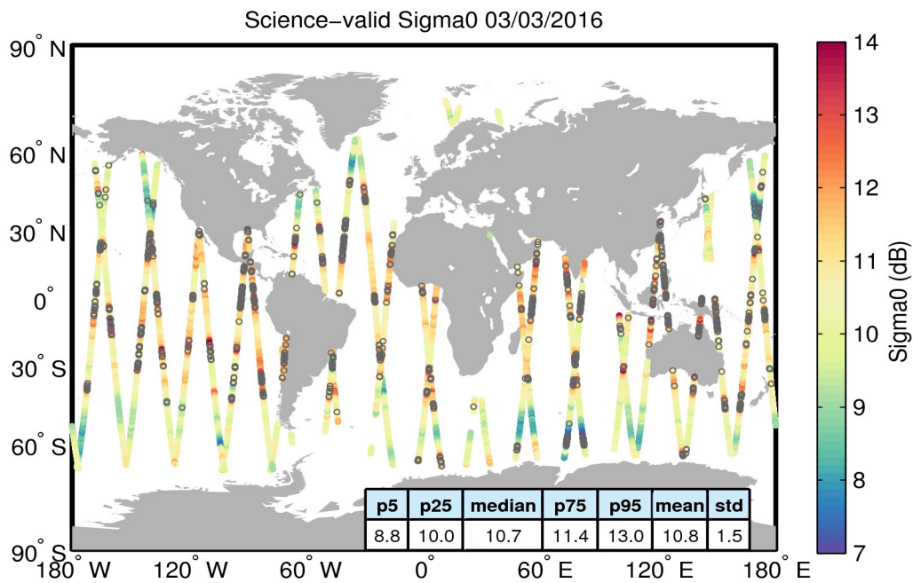
Figure 27. Geographical distribution of science-valid sigma0 data over oceans and lakes for 03/03/2016. The statistical values shown in the table refer to the sigma0 in dB and are calculated over all measurements shown in the figure. Gray circles denote records that have been rejected based on the editing criteria described in Table 4.
