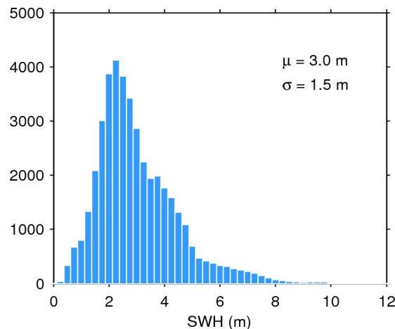
Figure 20. Histogram of science-valid SWH over oceans and lakes for 03/03/2016. The mean ( \mu ) and standard deviation ( \sigma ) are also shown. Note that values larger than 12 m are excluded from the histogram for the sake of readability but not from the computation of \mu and \sigma .
