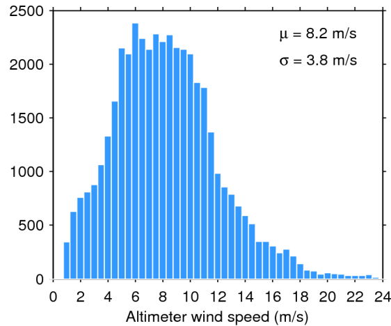
Figure 33. Histogram of flag-valid wind over oceans and lakes for 03/03/2016. The mean ( \mu ) and standard deviation ( \sigma ) are also shown. Note that values larger than 24 m/s are excluded from the histogram for the sake of readability but not from the computation of \mu and \sigma .
