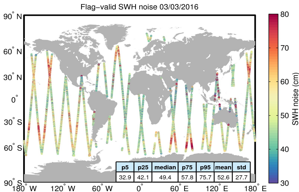
Figure 18. Geographical distribution of flag-valid 20-Hz SWH measurement noise over oceans and lakes for 03/03/2016. The statistical values shown in the table refer to the SWH noise and are calculated over all measurements shown in the figure.
