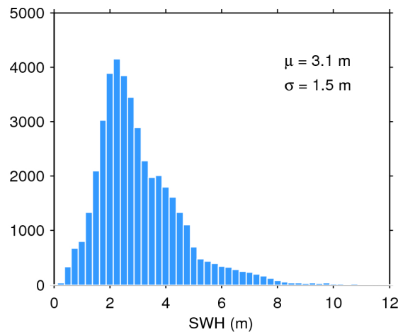
Figure 17. Histogram of flag-valid SWH over oceans and lakes for 03/03/2016. The mean ( \mu ) and standard deviation ( \sigma ) are also shown. Note that values larger than 12 m are excluded from the histogram for the sake of readability but not from the computation of \mu and \sigma .
