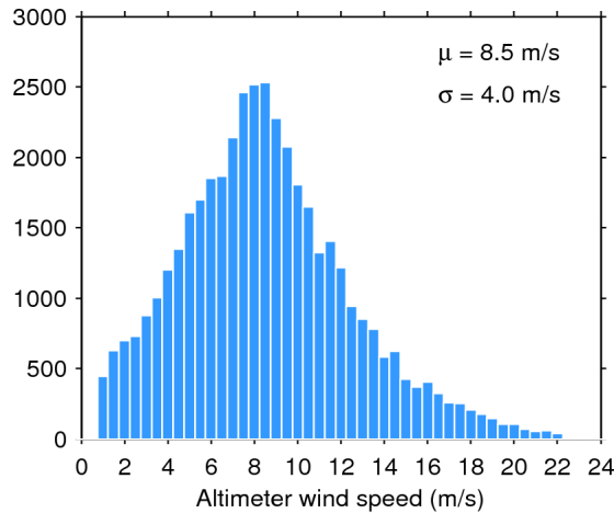
Figure 33. Histogram of flag-valid wind over oceans and lakes for 01/03/2016. The mean ( \mu ) and standard deviation ( \sigma ) are also shown. Note that values larger than 24 m/s are excluded from the histogram for the sake of readability but not from the computation of \mu and \sigma .
