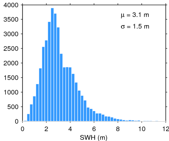
Figure 20. Histogram of science-valid SWH over oceans and lakes for 01/03/2016. The mean ( \mu ) and standard deviation ( \sigma ) are also shown. Note that values larger than 12 m are excluded from the histogram for the sake of readability but not from the computation of \mu and \sigma .
