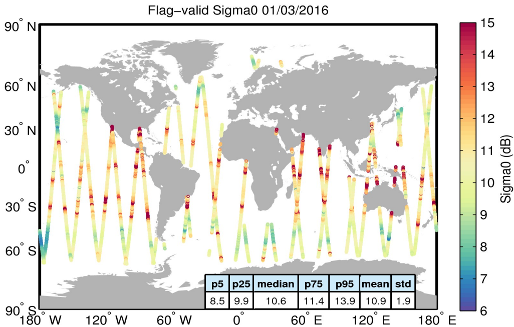
Figure 23. Geographical distribution of flag-valid sigma0 data over oceans and lakes for 01/03/2016. The statistical values shown in the table refer to the sigma0 in dB and are calculated over all measurements shown in the figure.
