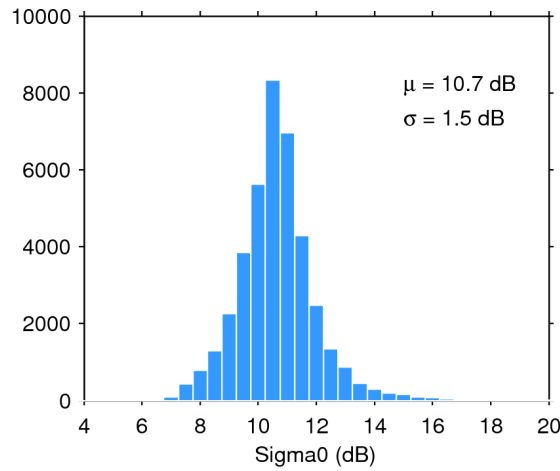
Figure 28. Histogram of science-valid sigma0 over oceans and lakes for 01/03/2016. The mean ( \mu ) and standard deviation ( \sigma ) are also shown. Note that values outside [4 20] dB are excluded from the histogram for the sake of readability but not from the computation of \mu and \sigma .
