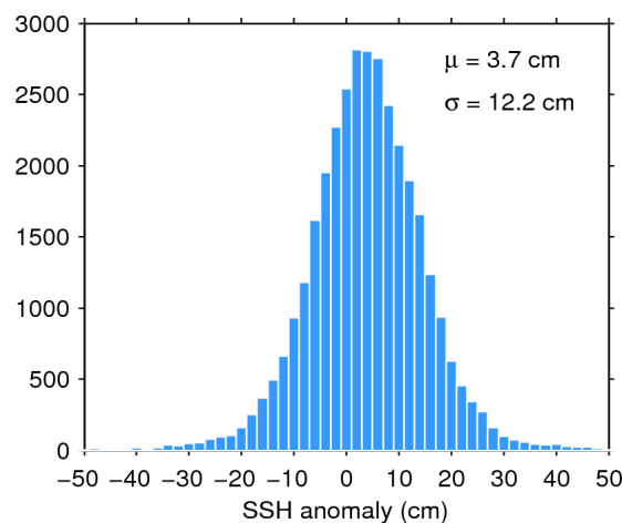
Figure 11. Histogram of science-valid SSH anomaly over oceans and lakes for 01/03/2016. The mean ( \mu ) and standard deviation ( \sigma ) are also shown. Note that values outside [-50 50] cm are excluded from the histogram for the sake of readability but not from the computation of \mu and \sigma .
