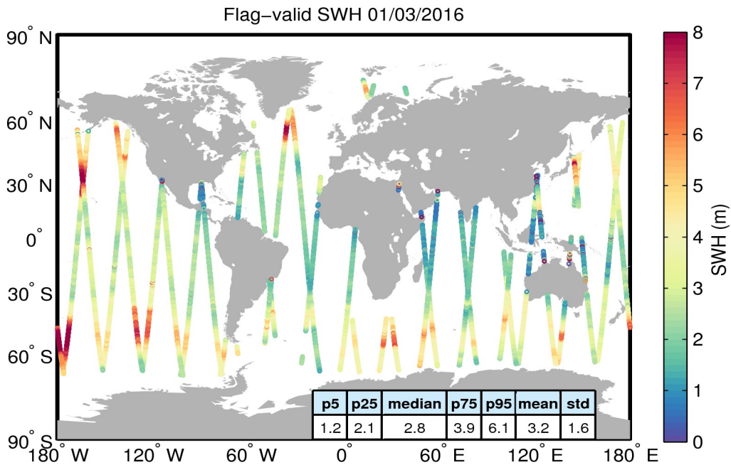
Figure 15. Geographical distribution of flag-valid SWH data over oceans and lakes for 01/03/2016. The statistical values shown in the table refer to the SWH in m and are calculated over all measurements shown in the figure.
