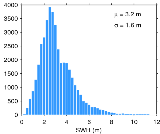
Figure 17. Histogram of flag-valid SWH over oceans and lakes for 01/03/2016. The mean ( \mu ) and standard deviation ( \sigma ) are also shown. Note that values larger than 12 m are excluded from the histogram for the sake of readability but not from the computation of \mu and \sigma .
