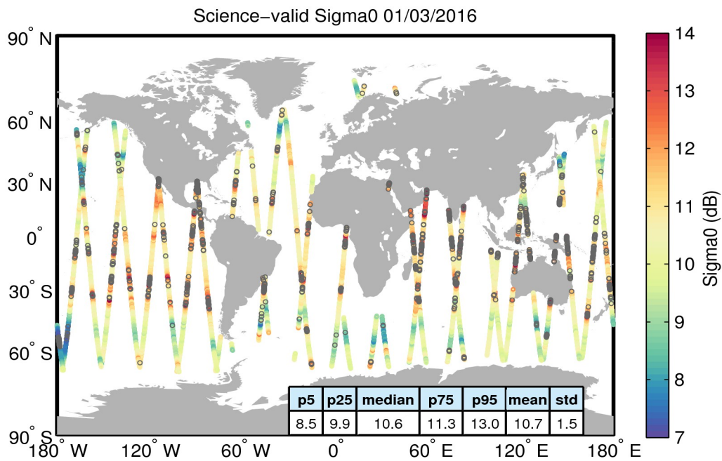
Figure 27. Geographical distribution of science-valid sigma0 data over oceans and lakes for 01/03/2016. The statistical values shown in the table refer to the sigma0 in dB and are calculated over all measurements shown in the figure. Gray circles denote records that have been rejected based on the editing criteria described in Table 4.
