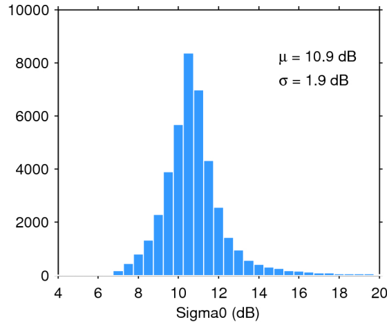
Figure 25. Histogram of flag-valid sigma0 over oceans and lakes for 01/03/2016. The mean ( \mu ) and standard deviation ( \sigma ) are also shown. Note that values outside [4 20] dB are excluded from the histogram for the sake of readability but not from the computation of \mu and \sigma .
