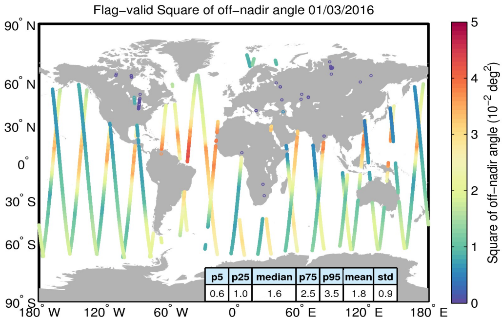
Figure 37. Geographical distribution of flag-valid mispointing data over oceans and lakes for 01/03/2016. The statistical values shown in the table refer to the mispointing in 10^{-2} \text{deg}^2 and are calculated over all measurements shown in the figure.
