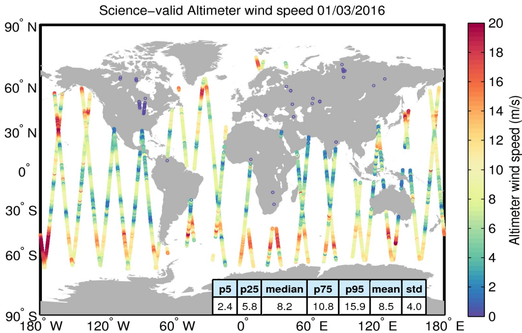
Figure 34. Geographical distribution of science-valid wind data over oceans and lakes for 01/03/2016. The statistical values shown in the table refer to the wind in m/s and are calculated over all measurements shown in the figure. Gray circles denote records that have been rejected based on the editing criteria described in Table 5.
