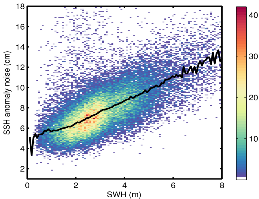
Figure 9. 2D histogram showing flag-valid SSH anomaly noise as a function of SWH for 01/03/2016. The black line denotes the median SSH anomaly noise as a function of SWH.
