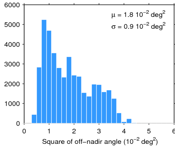
Figure 39. Histogram of flag-valid mispointing over oceans and lakes for 01/03/2016. The mean ( \mu ) and standard deviation ( \sigma ) are also shown. Note that values larger than 6 \cdot 10^{-2} \text{ deg}^2 are excluded from the histogram for the sake of readability but not from the computation of \mu and \sigma .
