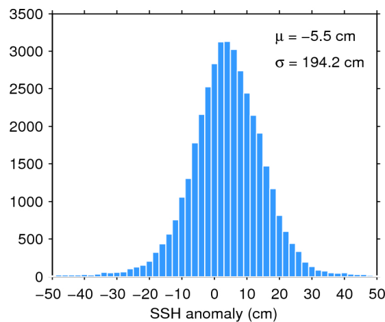
Figure 7. Histogram of flag-valid SSH anomaly over oceans and lakes for 01/03/2016. The mean ( \mu ) and standard deviation ( \sigma ) are also shown. Note that values outside [-50 50] cm are excluded from the histogram for the sake of readability but not from the computation of \mu and \sigma .
