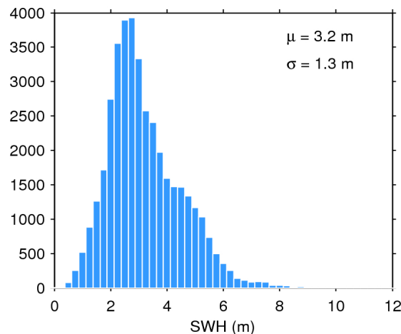
Figure 20. Histogram of science-valid SWH over oceans and lakes for 19/02/2016. The mean ( \mu ) and standard deviation ( \sigma ) are also shown. Note that values larger than 12 m are excluded from the histogram for the sake of readability but not from the computation of \mu and \sigma .
