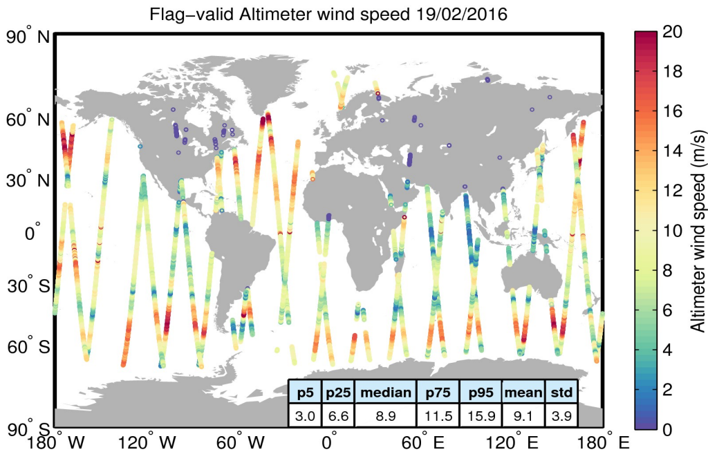
Figure 31. Geographical distribution of flag-valid wind data over oceans and lakes for 19/02/2016. The statistical values shown in the table refer to the wind in m/s and are calculated over all measurements shown in the figure.
