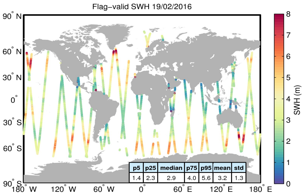
Figure 15. Geographical distribution of flag-valid SWH data over oceans and lakes for 19/02/2016. The statistical values shown in the table refer to the SWH in m and are calculated over all measurements shown in the figure.
