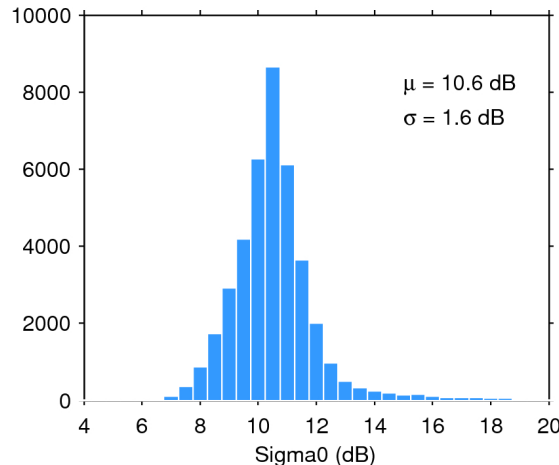
Figure 25. Histogram of flag-valid sigma0 over oceans and lakes for 19/02/2016. The mean ( \mu ) and standard deviation ( \sigma ) are also shown. Note that values outside [4 20] dB are excluded from the histogram for the sake of readability but not from the computation of \mu and \sigma .
