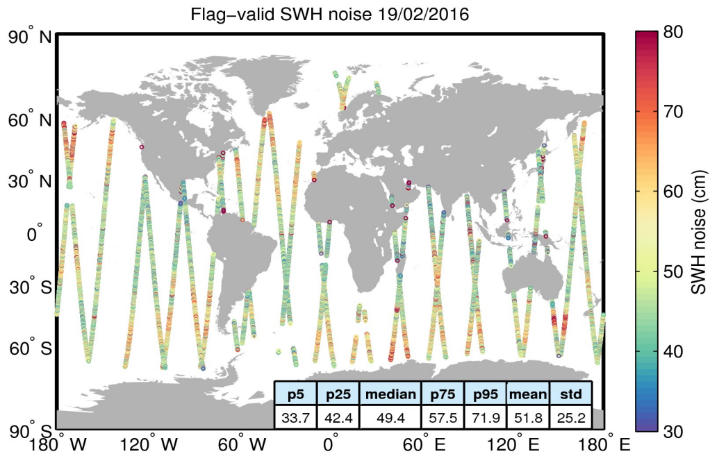
Figure 18. Geographical distribution of flag-valid 20-Hz SWH measurement noise over oceans and lakes for 19/02/2016. The statistical values shown in the figure refer to the SWH noise and are calculated over all measurements shown in the figure.
