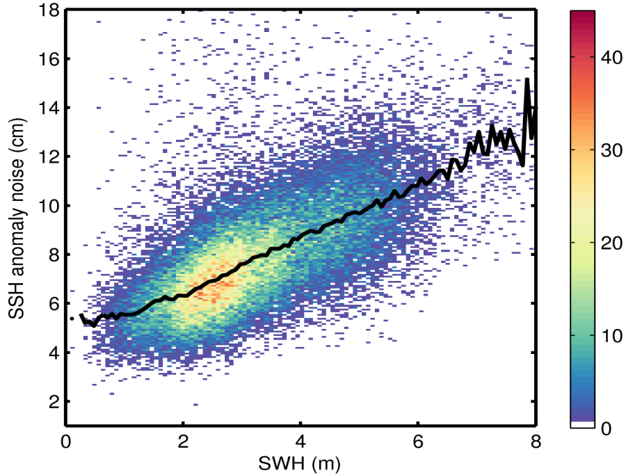
Figure 9. 2D histogram showing flag-valid SSH anomaly noise as a function of SWH for 19/02/2016. The black line denotes the median SSH anomaly noise as a function of SWH.
