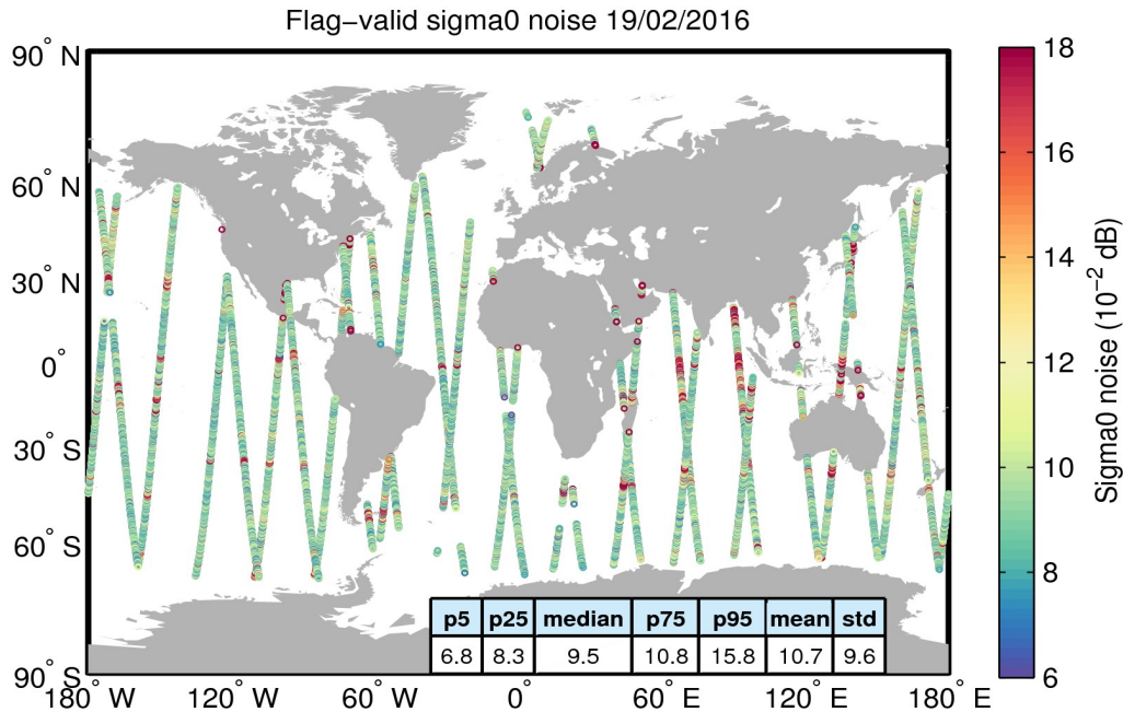
Figure 26. Geographical distribution of flag-valid 20-Hz sigma0 measurement noise over oceans and lakes for 19/02/2016. The statistical values shown in the table refer to the sigma0 noise and are calculated over all measurements shown in the figure.
