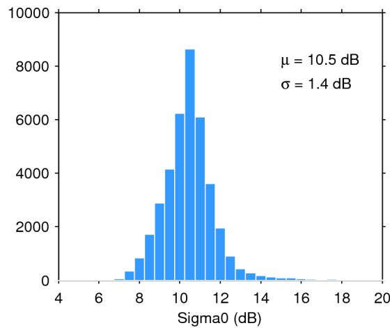
Figure 28. Histogram of science-valid sigma0 over oceans and lakes for 19/02/2016. The mean ( \mu ) and standard deviation ( \sigma ) are also shown. Note that values outside [4 20] dB are excluded from the histogram for the sake of readability but not from the computation of \mu and \sigma .
