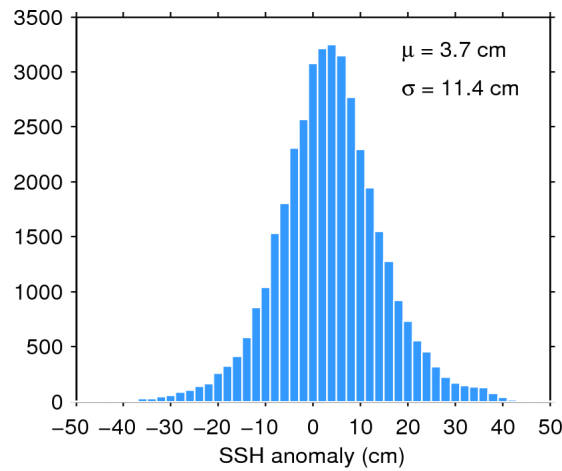
Figure 11. Histogram of science-valid SSH anomaly over oceans and lakes for 19/02/2016. The mean ( \mu ) and standard deviation ( \sigma ) are also shown. Note that values outside [-50 50] cm are excluded from the histogram for the sake of readability but not from the computation of \mu and \sigma .
