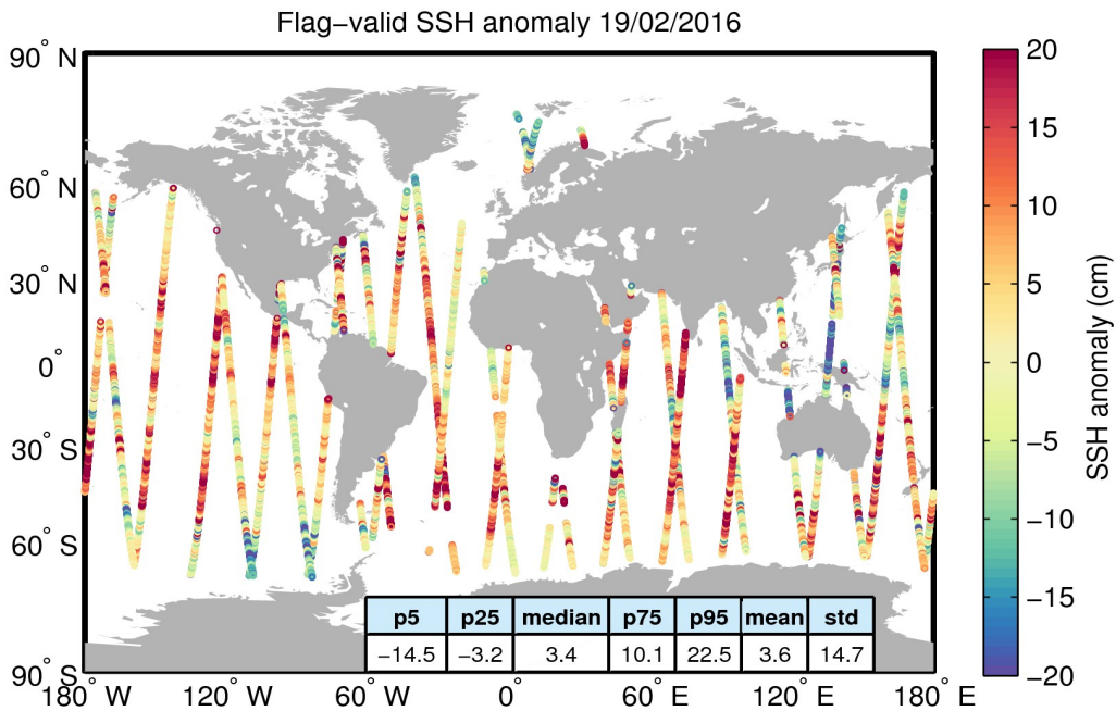
Figure 5. Geographical distribution of flag-valid 1-Hz SSH anomaly data over oceans and lakes for 19/02/2016. The statistical values shown in the table refer to the SSH anomaly in cm and are calculated over all measurements shown in the figure.
