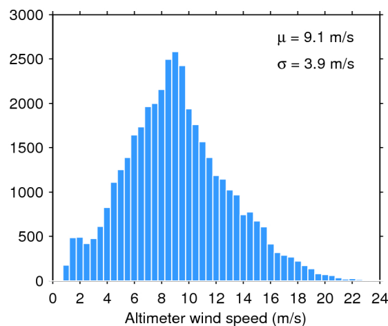
Figure 35. Histogram of science-valid wind over oceans and lakes for 19/02/2016. The mean ( \mu ) and standard deviation ( \sigma ) are also shown. Note that values larger than 24 m/s are excluded from the histogram for the sake of readability but not from the computation of \mu and \sigma .
