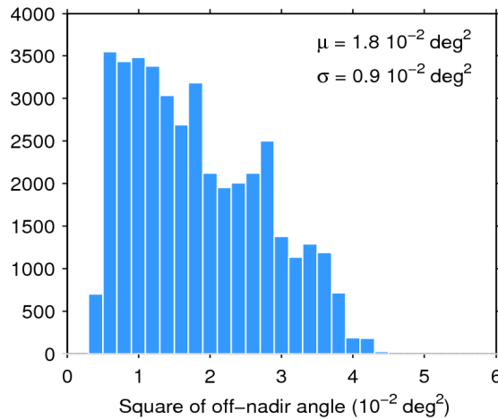
Figure 39. Histogram of flag-valid mispointing over oceans and lakes for 19/02/2016. The mean ( \mu ) and standard deviation ( \sigma ) are also shown. Note that values larger than 6 \cdot 10^{-2} \text{ deg}^2 are excluded from the histogram for the sake of readability but not from the computation of \mu and \sigma .
