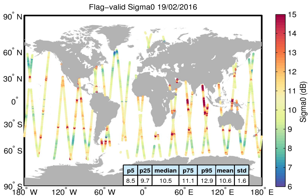
Figure 23. Geographical distribution of flag-valid sigma0 data over oceans and lakes for 19/02/2016. The statistical values shown in the table refer to the sigma0 in dB and are calculated over all measurements shown in the figure.
