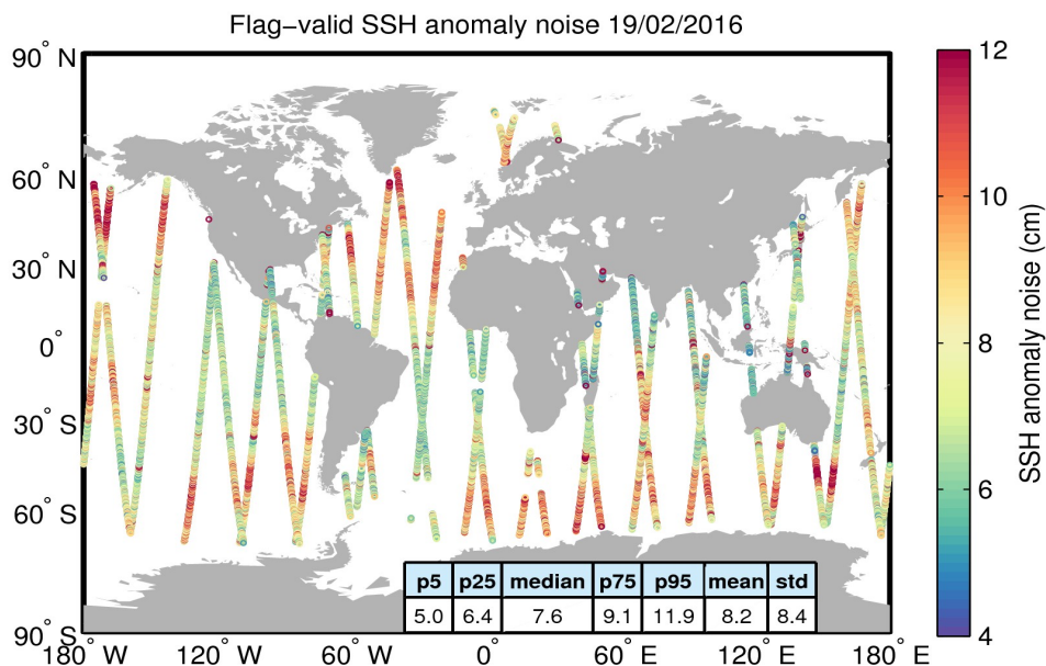
Figure 8. Geographical distribution of flag-valid 20-Hz SSH anomaly measurement noise over oceans and lakes for 19/02/2016. The statistical values shown in the table refer to the SSH anomaly noise and are calculated over all measurements shown in the figure.
