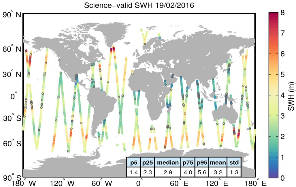
Figure 19. Geographical distribution of science-valid SWH data over oceans and lakes for 19/02/2016. The statistical values shown in the table refer to the SWH in m and are calculated over all measurements shown in the figure. Gray circles denote records that have been rejected based on the editing criteria described in Table 3.
