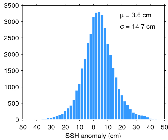
Figure 7. Histogram of flag-valid SSH anomaly over oceans and lakes for 19/02/2016. The mean ( \mu ) and standard deviation ( \sigma ) are also shown. Note that values outside [-50 50] cm are excluded from the histogram for the sake of readability but not from the computation of \mu and \sigma .
