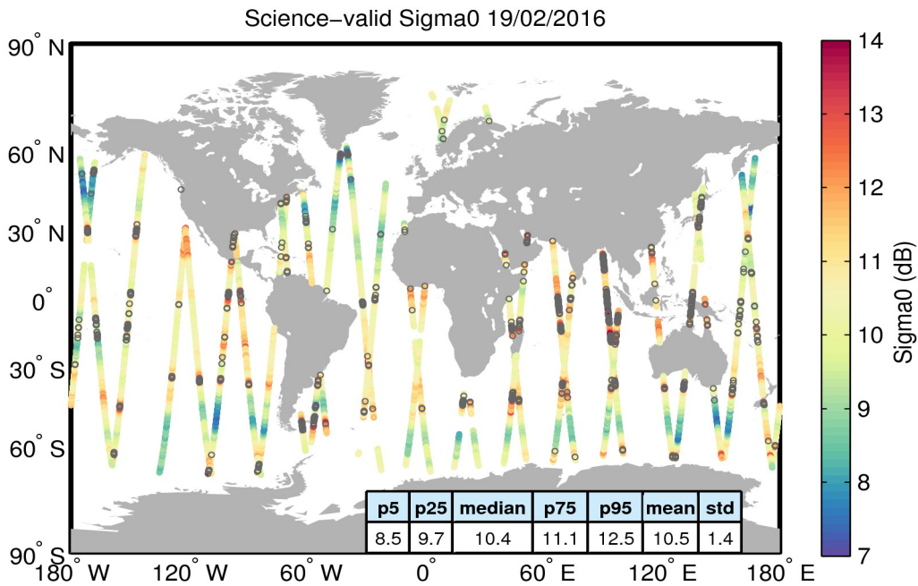
Figure 27. Geographical distribution of science-valid sigma0 data over oceans and lakes for 19/02/2016. The statistical values shown in the table refer to the sigma0 in dB and are calculated over all measurements shown in the figure. Gray circles denote records that have been rejected based on the editing criteria described in Table 4.
