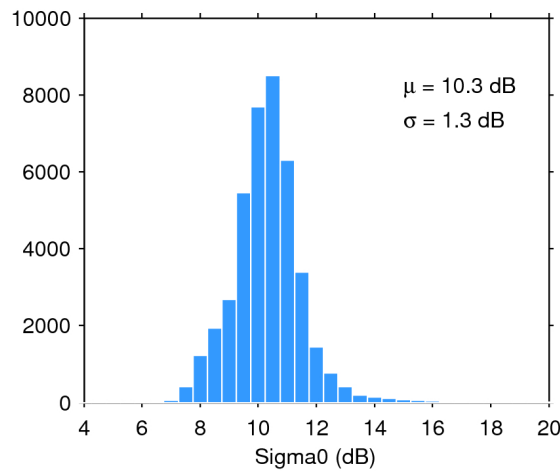
Figure 28. Histogram of science-valid sigma0 over oceans and lakes for 18/02/2016. The mean ( \mu ) and standard deviation ( \sigma ) are also shown. Note that values outside [4 20] dB are excluded from the histogram for the sake of readability but not from the computation of \mu and \sigma .
