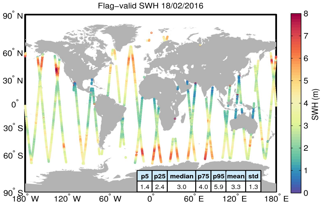
Figure 15. Geographical distribution of flag-valid SWH data over oceans and lakes for 18/02/2016. The statistical values shown in the table refer to the SWH in m and are calculated over all measurements shown in the figure.
