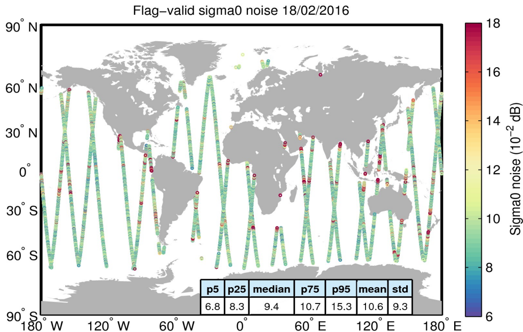
Figure 26. Geographical distribution of flag-valid 20-Hz sigma0 measurement noise over oceans and lakes for 18/02/2016. The statistical values shown in the table refer to the sigma0 noise and are calculated over all measurements shown in the figure.
