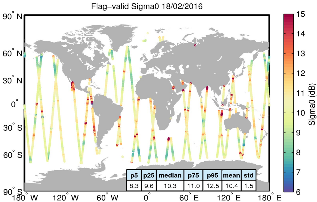
Figure 23. Geographical distribution of flag-valid sigma0 data over oceans and lakes for 18/02/2016. The statistical values shown in the table refer to the sigma0 in dB and are calculated over all measurements shown in the figure.
