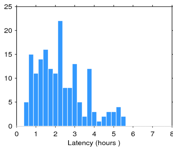
Figure 2. Histogram of the data latency for 18/02/2016. The y-axis denotes the number of files that are made available with a delay of x-hours with respect to the mean time of the records stored in the file.
