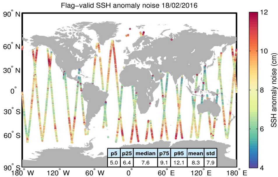
Figure 8. Geographical distribution of flag-valid 20-Hz SSH anomaly measurement noise over oceans and lakes for 18/02/2016. The statistical values shown in the table refer to the SSH anomaly noise and are calculated over all measurements shown in the figure.
