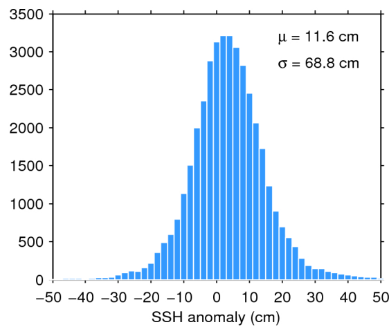
Figure 7. Histogram of flag-valid SSH anomaly over oceans and lakes for 18/02/2016. The mean ( \mu ) and standard deviation ( \sigma ) are also shown. Note that values outside [-50 50] cm are excluded from the histogram for the sake of readability but not from the computation of \mu and \sigma .
