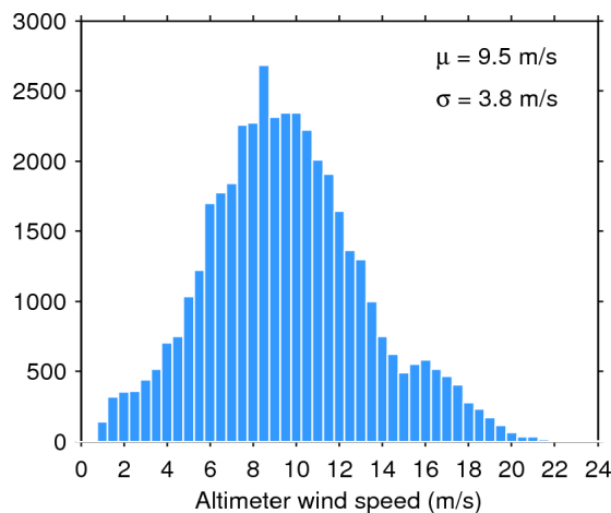
Figure 35. Histogram of science-valid wind over oceans and lakes for 18/02/2016. The mean ( \mu ) and standard deviation ( \sigma ) are also shown. Note that values larger than 24 m/s are excluded from the histogram for the sake of readability but not from the computation of \mu and \sigma .
