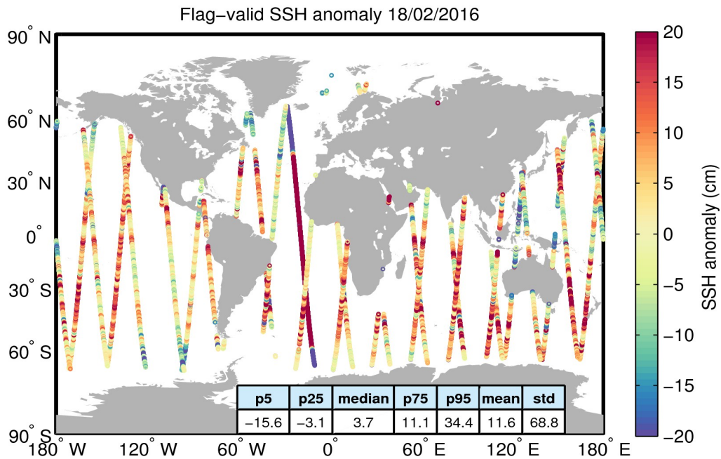
Figure 5. Geographical distribution of flag-valid 1-Hz SSH anomaly data over oceans and lakes for 18/02/2016. The statistical values shown in the table refer to the SSH anomaly in cm and are calculated over all measurements shown in the figure.
