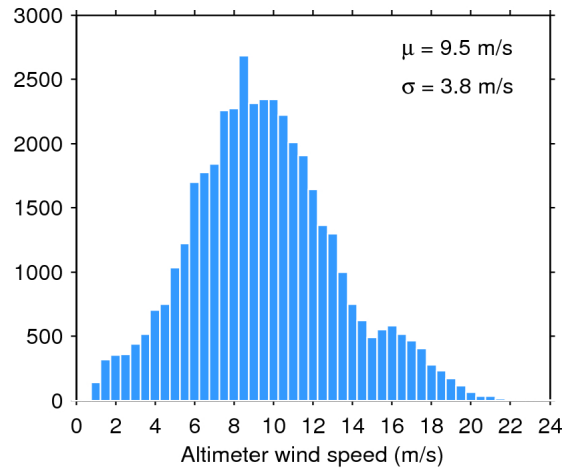
Figure 33. Histogram of flag-valid wind over oceans and lakes for 18/02/2016. The mean ( \mu ) and standard deviation ( \sigma ) are also shown. Note that values larger than 24 m/s are excluded from the histogram for the sake of readability but not from the computation of \mu and \sigma .
