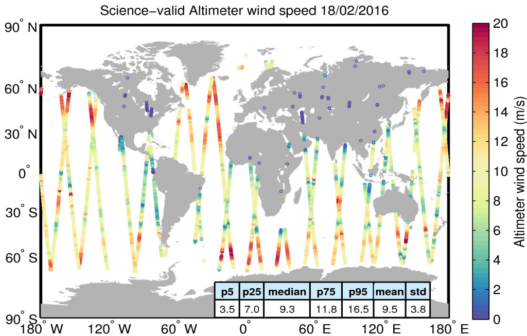
Figure 34. Geographical distribution of science-valid wind data over oceans and lakes for 18/02/2016. The statistical values shown in the table refer to the wind in m/s and are calculated over all measurements shown in the figure. Gray circles denote records that have been rejected based on the editing criteria described in Table 5.
