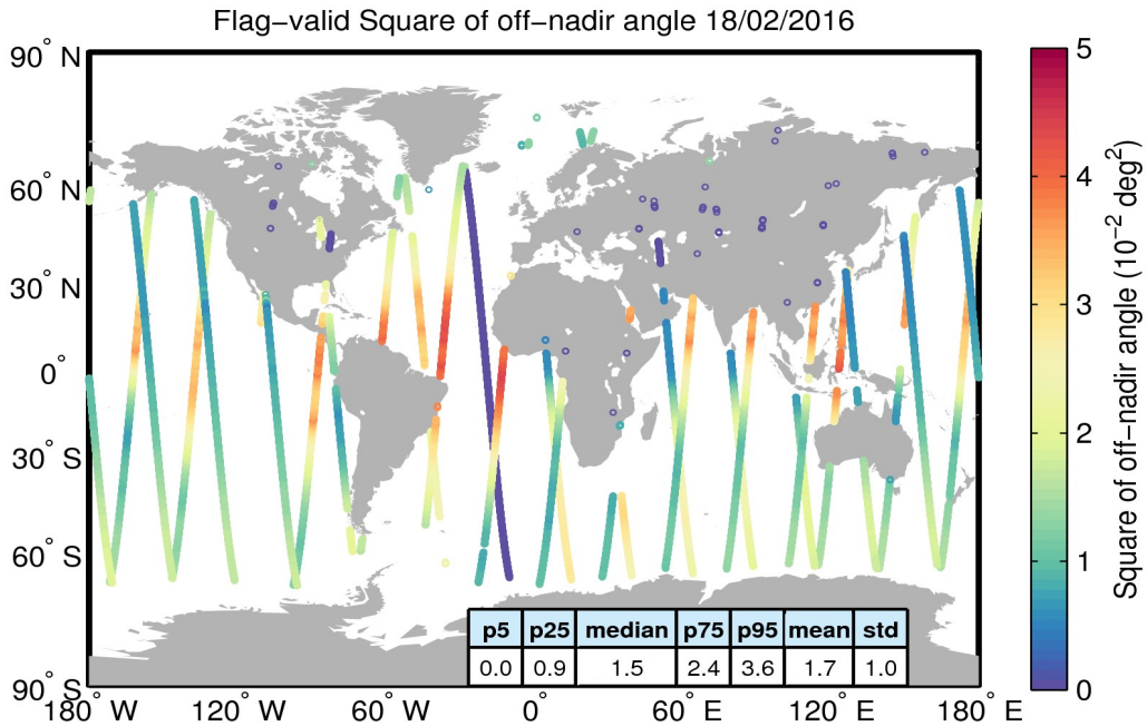
Figure 37. Geographical distribution of flag-valid mispointing data over oceans and lakes for 18/02/2016. The statistical values shown in the table refer to the mispointing in 10^{-2} deg 2 and are calculated over all measurements shown in the figure.
