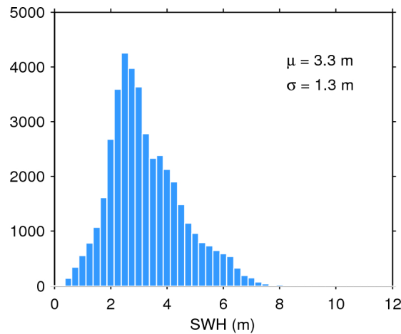
Figure 17. Histogram of flag-valid SWH over oceans and lakes for 18/02/2016. The mean ( \mu ) and standard deviation ( \sigma ) are also shown. Note that values larger than 12 m are excluded from the histogram for the sake of readability but not from the computation of \mu and \sigma .
