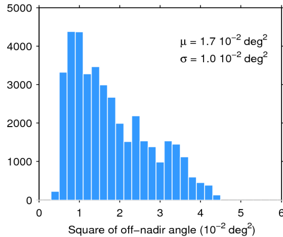
Figure 39. Histogram of flag-valid mispointing over oceans and lakes for 18/02/2016. The mean ( \mu ) and standard deviation ( \sigma ) are also shown. Note that values larger than 6 \cdot 10^{-2} \text{ deg}^2 are excluded from the histogram for the sake of readability but not from the computation of \mu and \sigma .
