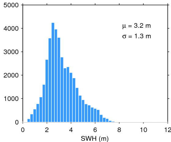
Figure 20. Histogram of science-valid SWH over oceans and lakes for 18/02/2016. The mean ( \mu ) and standard deviation ( \sigma ) are also shown. Note that values larger than 12 m are excluded from the histogram for the sake of readability but not from the computation of \mu and \sigma .
