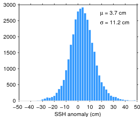
Figure 11. Histogram of science-valid SSH anomaly over oceans and lakes for 18/02/2016. The mean ( \mu ) and standard deviation ( \sigma ) are also shown. Note that values outside [-50 50] cm are excluded from the histogram for the sake of readability but not from the computation of \mu and \sigma .
