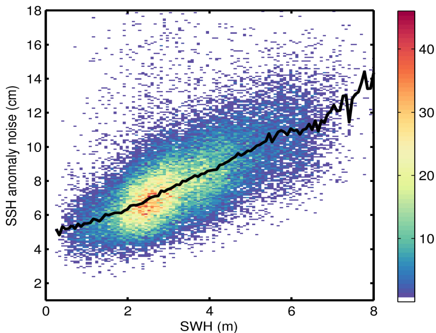
Figure 9. 2D histogram showing flag-valid SSH anomaly noise as a function of SWH for 18/02/2016. The black line denotes the median SSH anomaly noise as a function of SWH.
