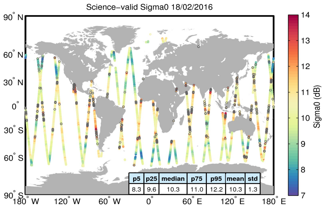
Figure 27. Geographical distribution of science-valid sigma0 data over oceans and lakes for 18/02/2016. The statistical values shown in the table refer to the sigma0 in dB and are calculated over all measurements shown in the figure. Gray circles denote records that have been rejected based on the editing criteria described in Table 4.
