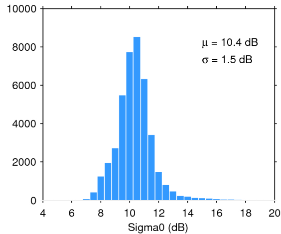
Figure 25. Histogram of flag-valid sigma0 over oceans and lakes for 18/02/2016. The mean ( \mu ) and standard deviation ( \sigma ) are also shown. Note that values outside [4 20] dB are excluded from the histogram for the sake of readability but not from the computation of \mu and \sigma .
