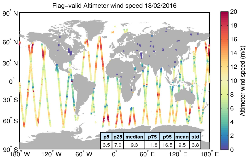
Figure 31. Geographical distribution of flag-valid wind data over oceans and lakes for 18/02/2016. The statistical values shown in the table refer to the wind in m/s and are calculated over all measurements shown in the figure.
