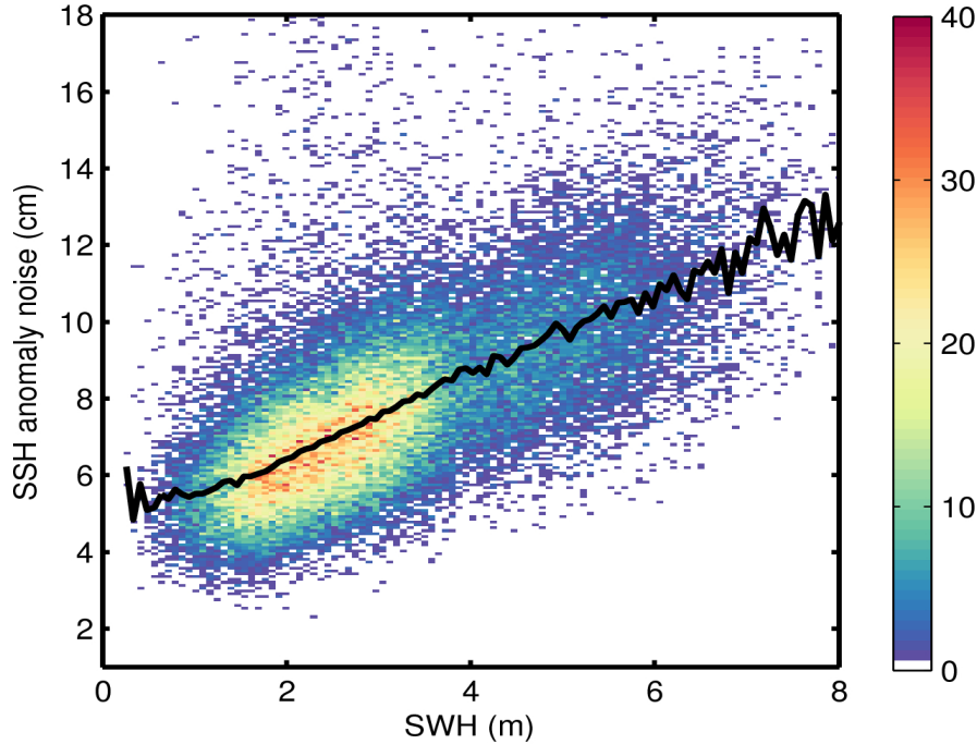
Figure 9. 2D histogram showing flag-valid SSH anomaly noise as a function of SWH for 31/01/2016. The black line denotes the median SSH anomaly noise as a function of SWH.
