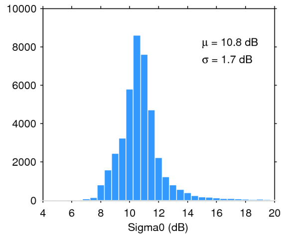
Figure 25. Histogram of flag-valid sigma0 over oceans and lakes for 31/01/2016. The mean ( \mu ) and standard deviation ( \sigma ) are also shown. Note that values outside [4 20] dB are excluded from the histogram for the sake of readability but not from the computation of \mu and \sigma .
