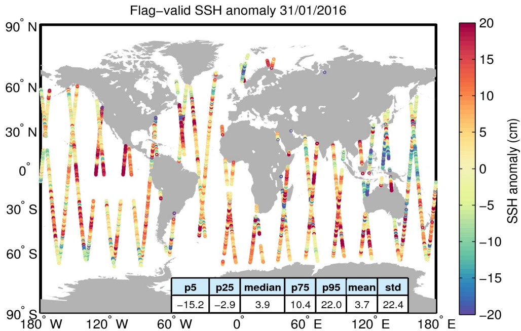
Figure 5. Geographical distribution of flag-valid 1-Hz SSH anomaly data over oceans and lakes for 31/01/2016. The statistical values shown in the table refer to the SSH anomaly in cm and are calculated over all measurements shown in the figure.
