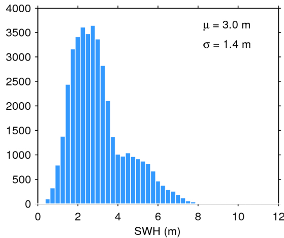
Figure 20. Histogram of science-valid SWH over oceans and lakes for 31/01/2016. The mean ( \mu ) and standard deviation ( \sigma ) are also shown. Note that values larger than 12 m are excluded from the histogram for the sake of readability but not from the computation of \mu and \sigma .
