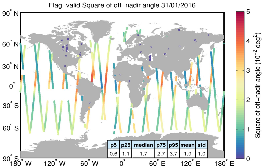
Figure 37. Geographical distribution of flag-valid mispointing data over oceans and lakes for 31/01/2016. The statistical values shown in the table refer to the mispointing in 10^{-2} deg 2 and are calculated over all measurements shown in the figure.
