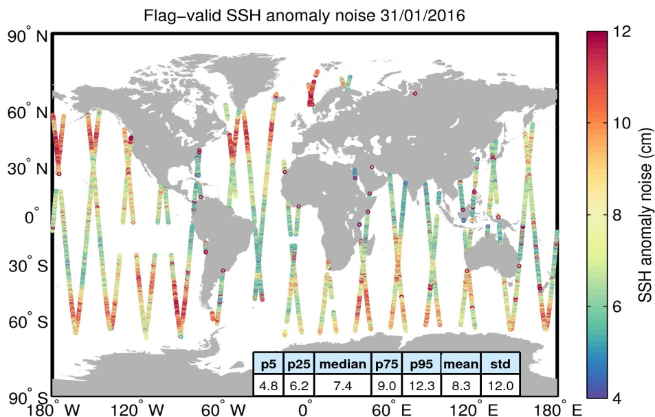
Figure 8. Geographical distribution of flag-valid 20-Hz SSH anomaly measurement noise over oceans and lakes for 31/01/2016. The statistical values shown in the table refer to the SSH anomaly noise and are calculated over all measurements shown in the figure.
