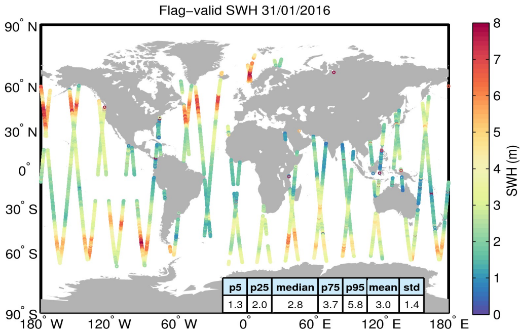
Figure 15. Geographical distribution of flag-valid SWH data over oceans and lakes for 31/01/2016. The statistical values shown in the table refer to the SWH in m and are calculated over all measurements shown in the figure.
