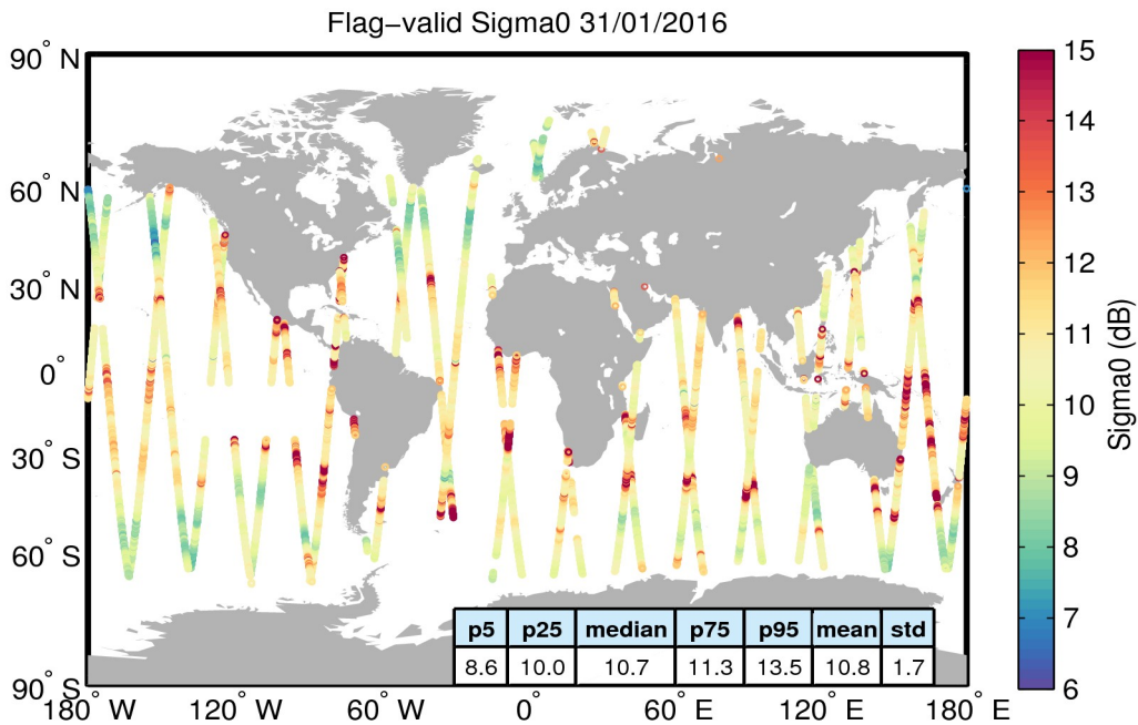
Figure 23. Geographical distribution of flag-valid sigma0 data over oceans and lakes for 31/01/2016. The statistical values shown in the table refer to the sigma0 in dB and are calculated over all measurements shown in the figure.
