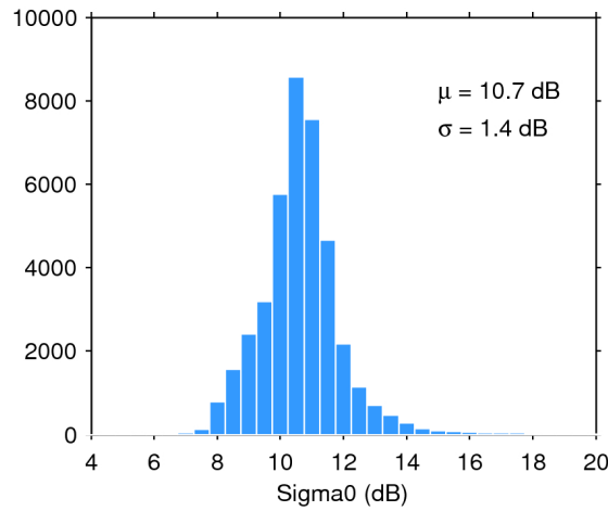
Figure 28. Histogram of science-valid sigma0 over oceans and lakes for 31/01/2016. The mean ( \mu ) and standard deviation ( \sigma ) are also shown. Note that values outside [4 20] dB are excluded from the histogram for the sake of readability but not from the computation of \mu and \sigma .
