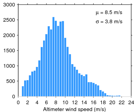
Figure 35. Histogram of science-valid wind over oceans and lakes for 31/01/2016. The mean ( \mu ) and standard deviation ( \sigma ) are also shown. Note that values larger than 24 m/s are excluded from the histogram for the sake of readability but not from the computation of \mu and \sigma .
