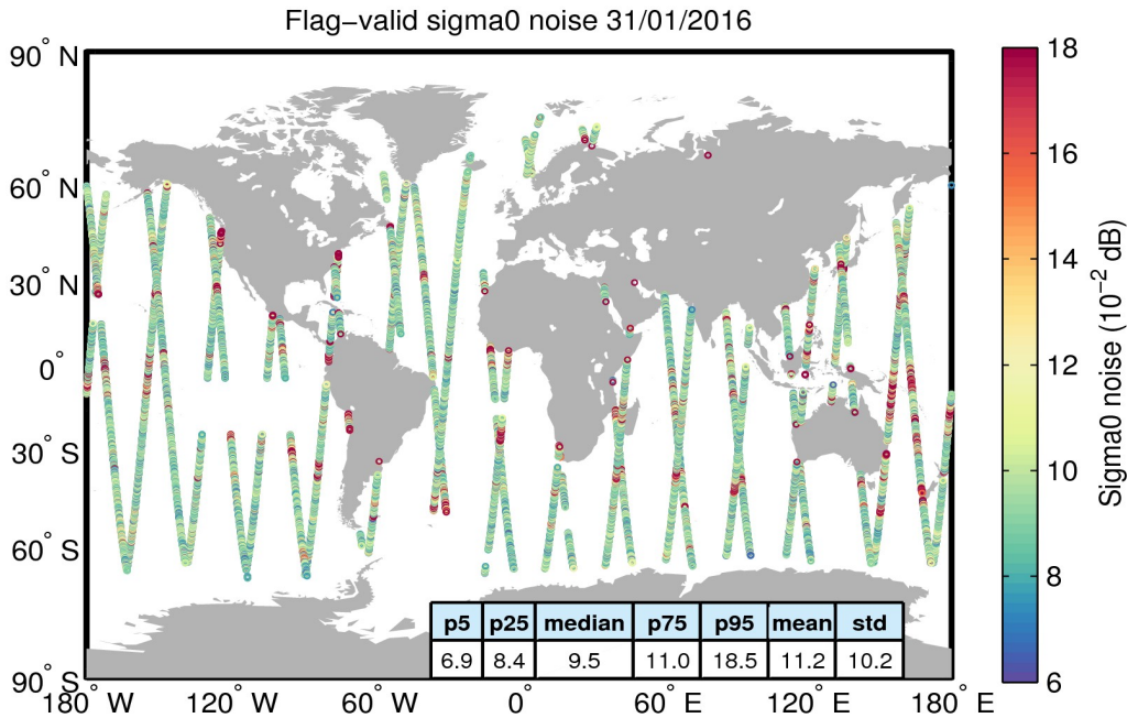
Figure 26. Geographical distribution of flag-valid 20-Hz sigma0 measurement noise over oceans and lakes for 31/01/2016. The statistical values shown in the table refer to the sigma0 noise and are calculated over all measurements shown in the figure.
