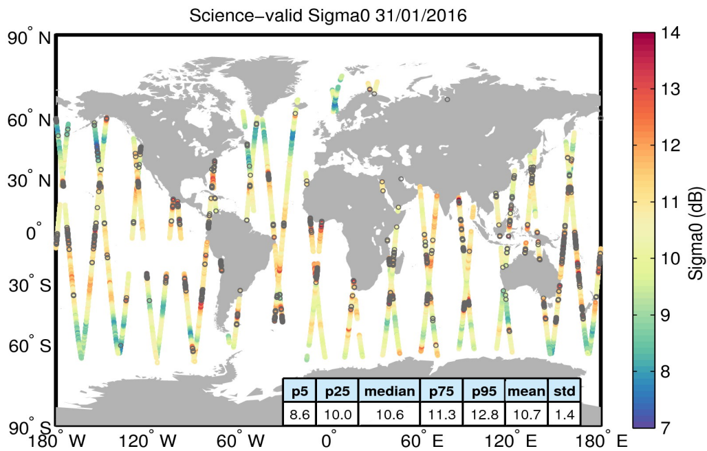
Figure 27. Geographical distribution of science-valid sigma0 data over oceans and lakes for 31/01/2016. The statistical values shown in the table refer to the sigma0 in dB and are calculated over all measurements shown in the figure. Gray circles denote records that have been rejected based on the editing criteria described in Table 4.
