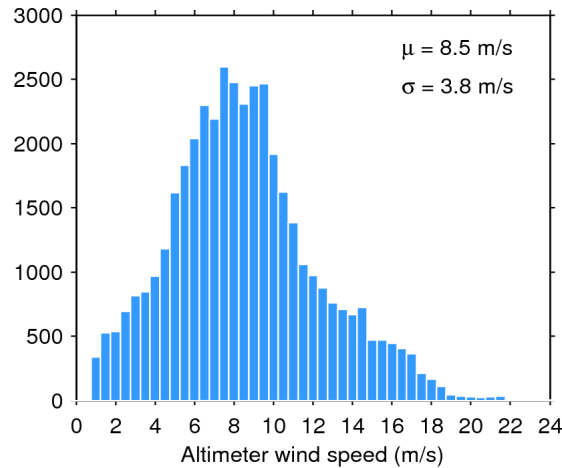
Figure 33. Histogram of flag-valid wind over oceans and lakes for 31/01/2016. The mean ( \mu ) and standard deviation ( \sigma ) are also shown. Note that values larger than 24 m/s are excluded from the histogram for the sake of readability but not from the computation of \mu and \sigma .
