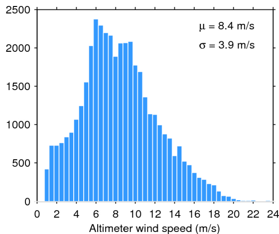
Figure 35. Histogram of science-valid wind over oceans and lakes for 30/01/2016. The mean ( \mu ) and standard deviation ( \sigma ) are also shown. Note that values larger than 24 m/s are excluded from the histogram for the sake of readability but not from the computation of \mu and \sigma .
