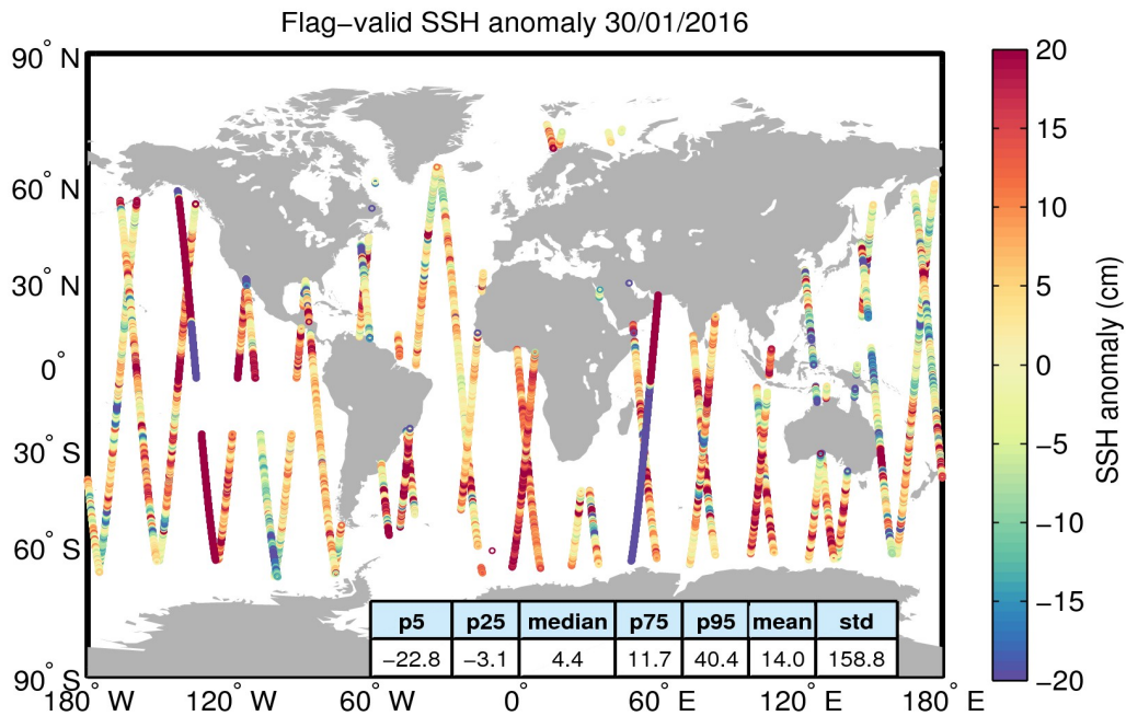
Figure 5. Geographical distribution of flag-valid 1-Hz SSH anomaly data over oceans and lakes for 30/01/2016. The statistical values shown in the table refer to the SSH anomaly in cm and are calculated over all measurements shown in the figure.
