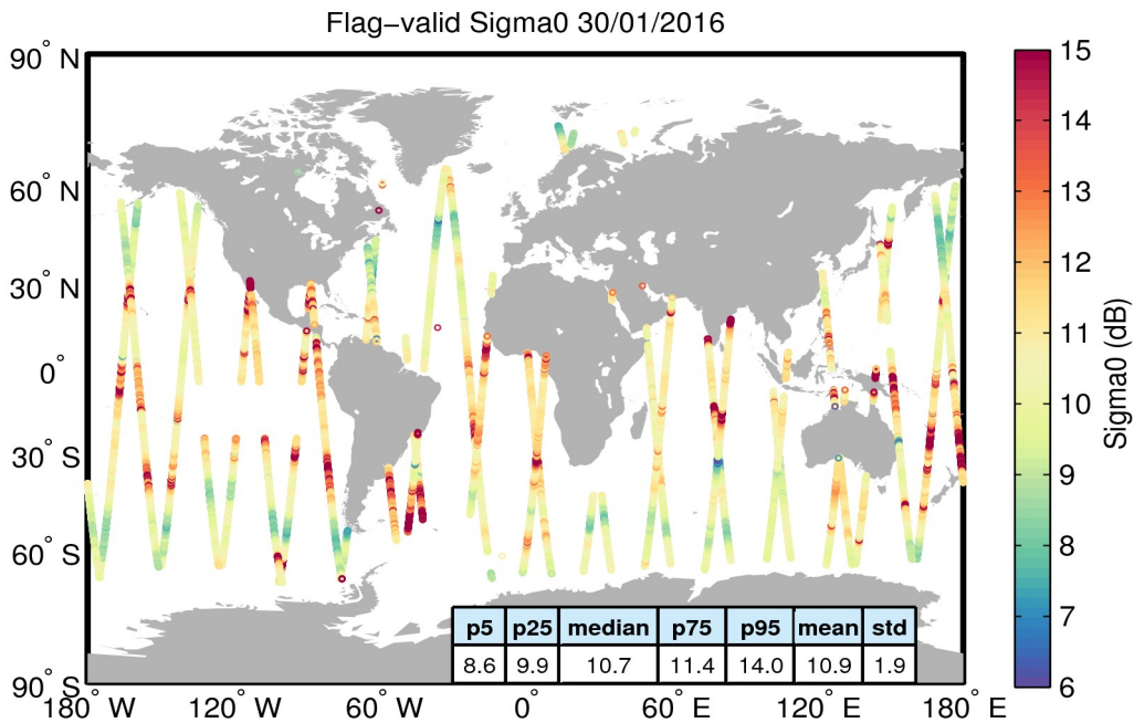
Figure 23. Geographical distribution of flag-valid sigma0 data over oceans and lakes for 30/01/2016. The statistical values shown in the table refer to the sigma0 in dB and are calculated over all measurements shown in the figure.
