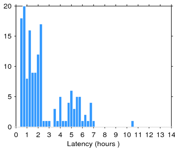
Figure 2. Histogram of the data latency for 30/01/2016. The y-axis denotes the number of files that are made available with a delay of x-hours with respect to the mean time of the records stored in the file.
