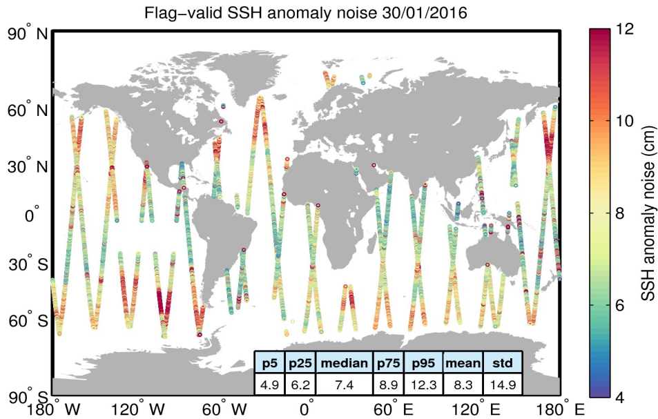
Figure 8. Geographical distribution of flag-valid 20-Hz SSH anomaly measurement noise over oceans and lakes for 30/01/2016. The statistical values shown in the table refer to the SSH anomaly noise and are calculated over all measurements shown in the figure.
