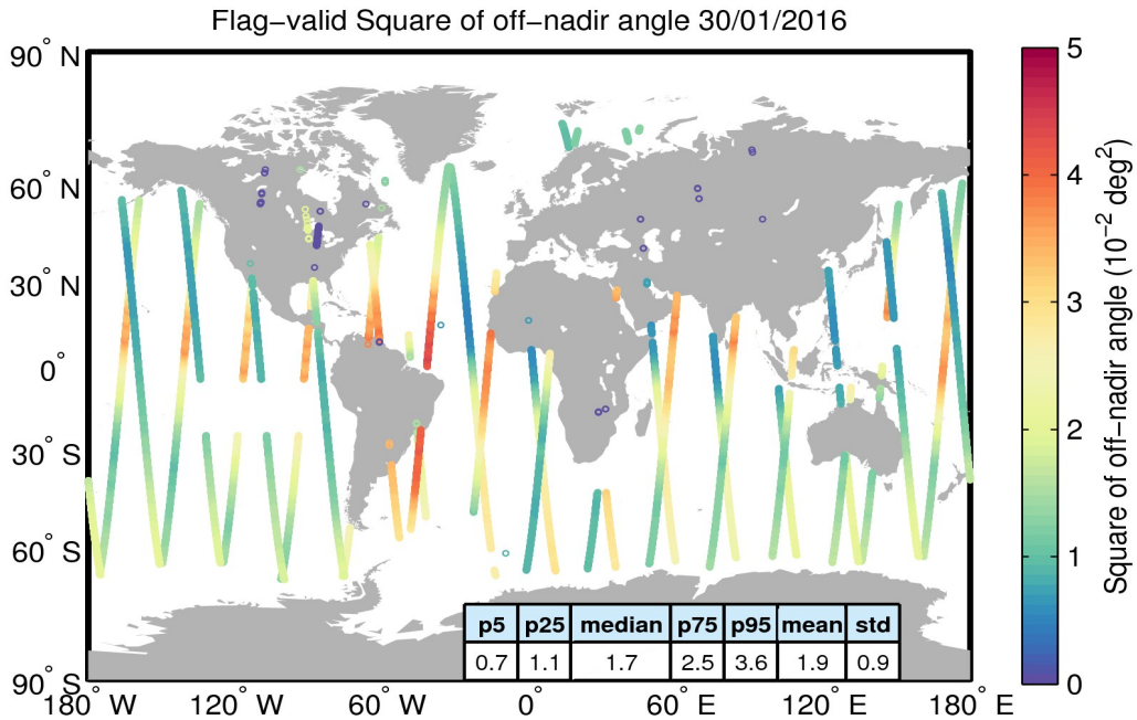
Figure 37. Geographical distribution of flag-valid mispointing data over oceans and lakes for 30/01/2016. The statistical values shown in the table refer to the mispointing in 10^{-2} deg 2 and are calculated over all measurements shown in the figure.
