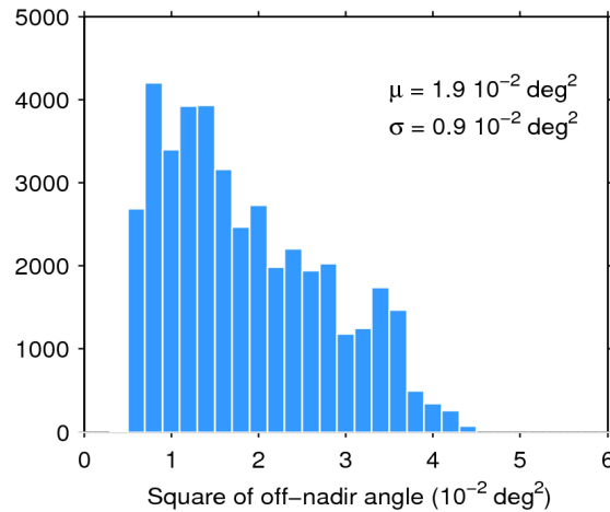
Figure 39. Histogram of flag-valid mispointing over oceans and lakes for 30/01/2016. The mean ( \mu ) and standard deviation ( \sigma ) are also shown. Note that values larger than 6 \cdot 10^{-2} \text{ deg}^2 are excluded from the histogram for the sake of readability but not from the computation of \mu and \sigma .
