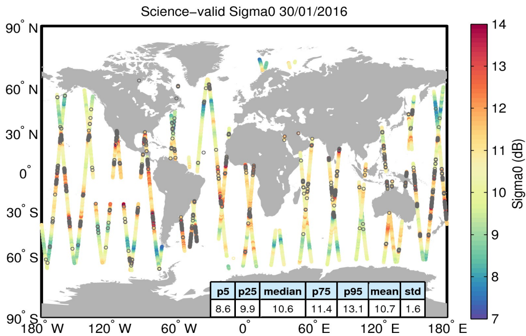
Figure 27. Geographical distribution of science-valid sigma0 data over oceans and lakes for 30/01/2016. The statistical values shown in the table refer to the sigma0 in dB and are calculated over all measurements shown in the figure. Gray circles denote records that have been rejected based on the editing criteria described in Table 4.
