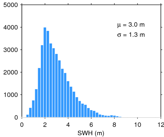
Figure 20. Histogram of science-valid SWH over oceans and lakes for 30/01/2016. The mean ( \mu ) and standard deviation ( \sigma ) are also shown. Note that values larger than 12 m are excluded from the histogram for the sake of readability but not from the computation of \mu and \sigma .
