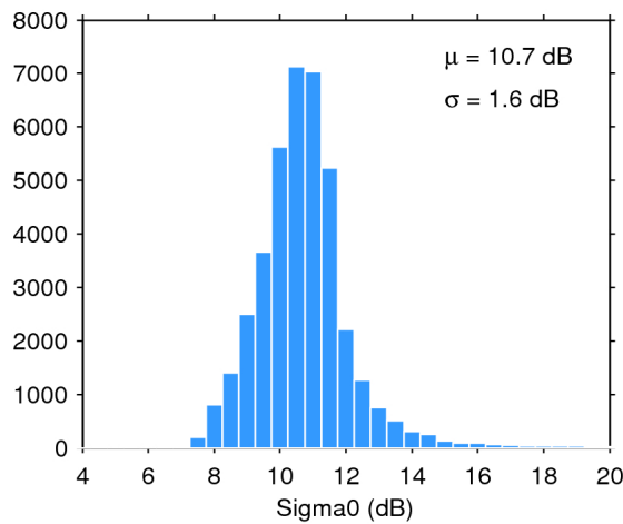
Figure 28. Histogram of science-valid sigma0 over oceans and lakes for 30/01/2016. The mean ( \mu ) and standard deviation ( \sigma ) are also shown. Note that values outside [4 20] dB are excluded from the histogram for the sake of readability but not from the computation of \mu and \sigma .
