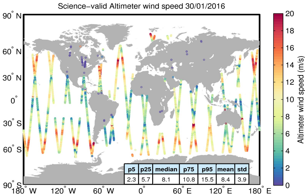
Figure 34. Geographical distribution of science-valid wind data over oceans and lakes for 30/01/2016. The statistical values shown in the table refer to the wind in m/s and are calculated over all measurements shown in the figure. Gray circles denote records that have been rejected based on the editing criteria described in Table 5.
