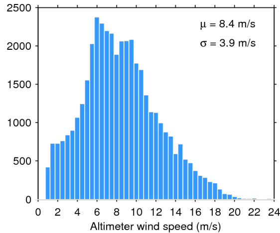
Figure 33. Histogram of flag-valid wind over oceans and lakes for 30/01/2016. The mean ( \mu ) and standard deviation ( \sigma ) are also shown. Note that values larger than 24 m/s are excluded from the histogram for the sake of readability but not from the computation of \mu and \sigma .
