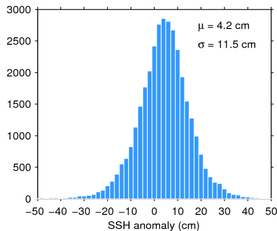
Figure 11. Histogram of science-valid SSH anomaly over oceans and lakes for 30/01/2016. The mean ( \mu ) and standard deviation ( \sigma ) are also shown. Note that values outside [-50 50] cm are excluded from the histogram for the sake of readability but not from the computation of \mu and \sigma .
