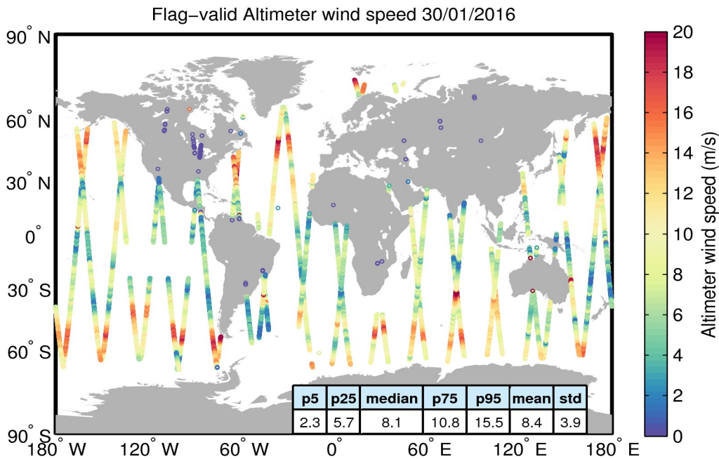
Figure 31. Geographical distribution of flag-valid wind data over oceans and lakes for 30/01/2016. The statistical values shown in the table refer to the wind in m/s and are calculated over all measurements shown in the figure.
