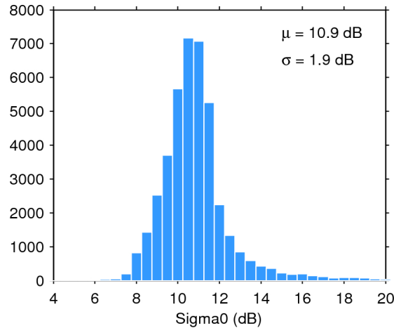
Figure 25. Histogram of flag-valid sigma0 over oceans and lakes for 30/01/2016. The mean ( \mu ) and standard deviation ( \sigma ) are also shown. Note that values outside [4 20] dB are excluded from the histogram for the sake of readability but not from the computation of \mu and \sigma .
