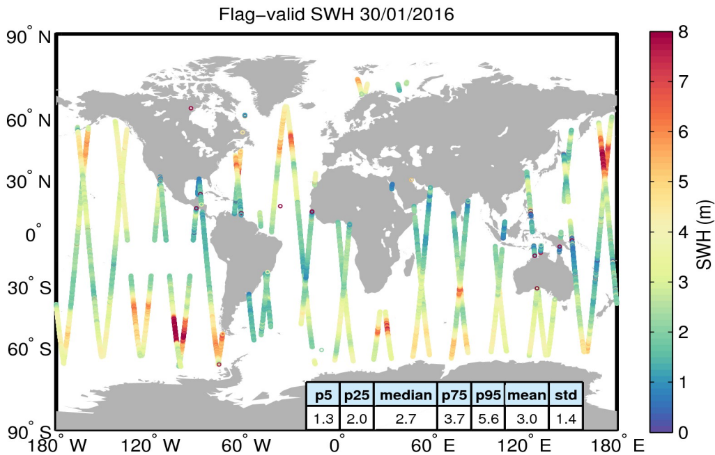
Figure 15. Geographical distribution of flag-valid SWH data over oceans and lakes for 30/01/2016. The statistical values shown in the table refer to the SWH in m and are calculated over all measurements shown in the figure.
