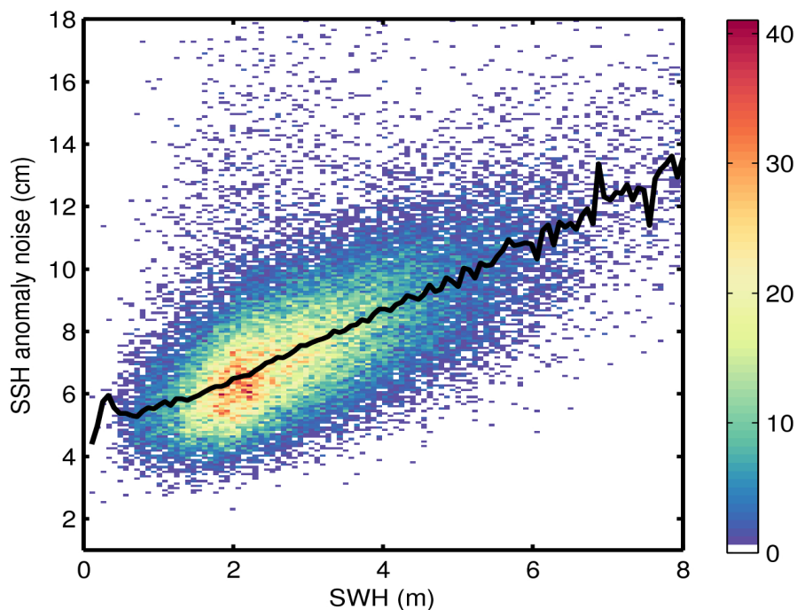
Figure 9. 2D histogram showing flag-valid SSH anomaly noise as a function of SWH for 30/01/2016. The black line denotes the median SSH anomaly noise as a function of SWH.
