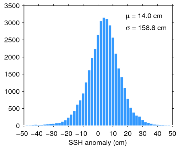
Figure 7. Histogram of flag-valid SSH anomaly over oceans and lakes for 30/01/2016. The mean ( \mu ) and standard deviation ( \sigma ) are also shown. Note that values outside [-50 50] cm are excluded from the histogram for the sake of readability but not from the computation of \mu and \sigma .
