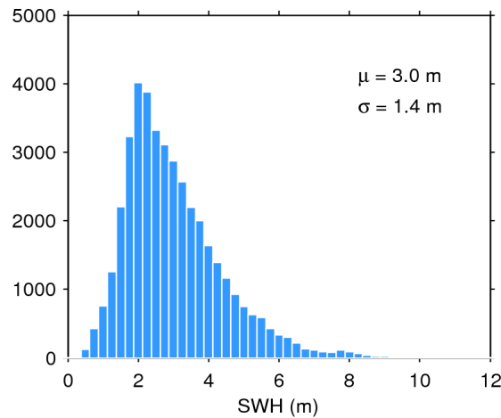
Figure 17. Histogram of flag-valid SWH over oceans and lakes for 30/01/2016. The mean ( \mu ) and standard deviation ( \sigma ) are also shown. Note that values larger than 12 m are excluded from the histogram for the sake of readability but not from the computation of \mu and \sigma .
