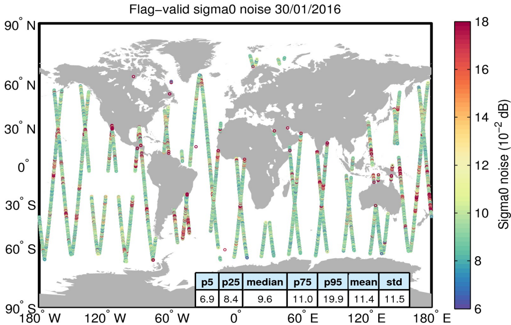
Figure 26. Geographical distribution of flag-valid 20-Hz sigma0 measurement noise over oceans and lakes for 30/01/2016. The statistical values shown in the table refer to the sigma0 noise and are calculated over all measurements shown in the figure.
