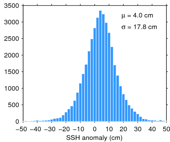
Figure 7. Histogram of flag-valid SSH anomaly over oceans and lakes for 29/01/2016. The mean ( \mu ) and standard deviation ( \sigma ) are also shown. Note that values outside [-50\ 50] cm are excluded from the histogram for the sake of readability but not from the computation of \mu and \sigma .
