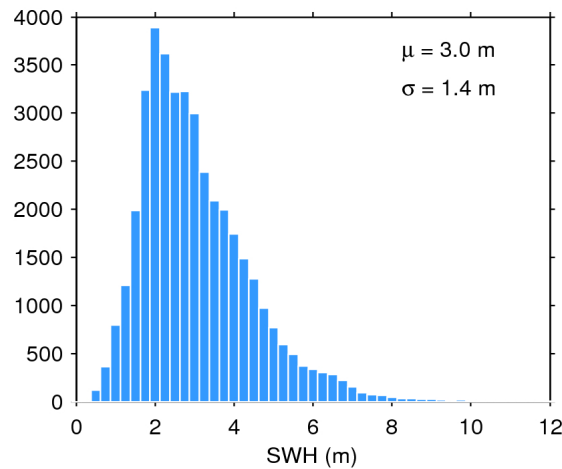
Figure 17. Histogram of flag-valid SWH over oceans and lakes for 29/01/2016. The mean ( \mu ) and standard deviation ( \sigma ) are also shown. Note that values larger than 12 m are excluded from the histogram for the sake of readability but not from the computation of \mu and \sigma .
