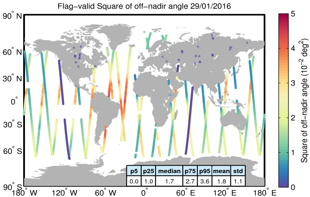
Figure 37. Geographical distribution of flag-valid mispointing data over oceans and lakes for 29/01/2016. The statistical values shown in the table refer to the mispointing in 10^{-2} deg 2 and are calculated over all measurements shown in the figure.
