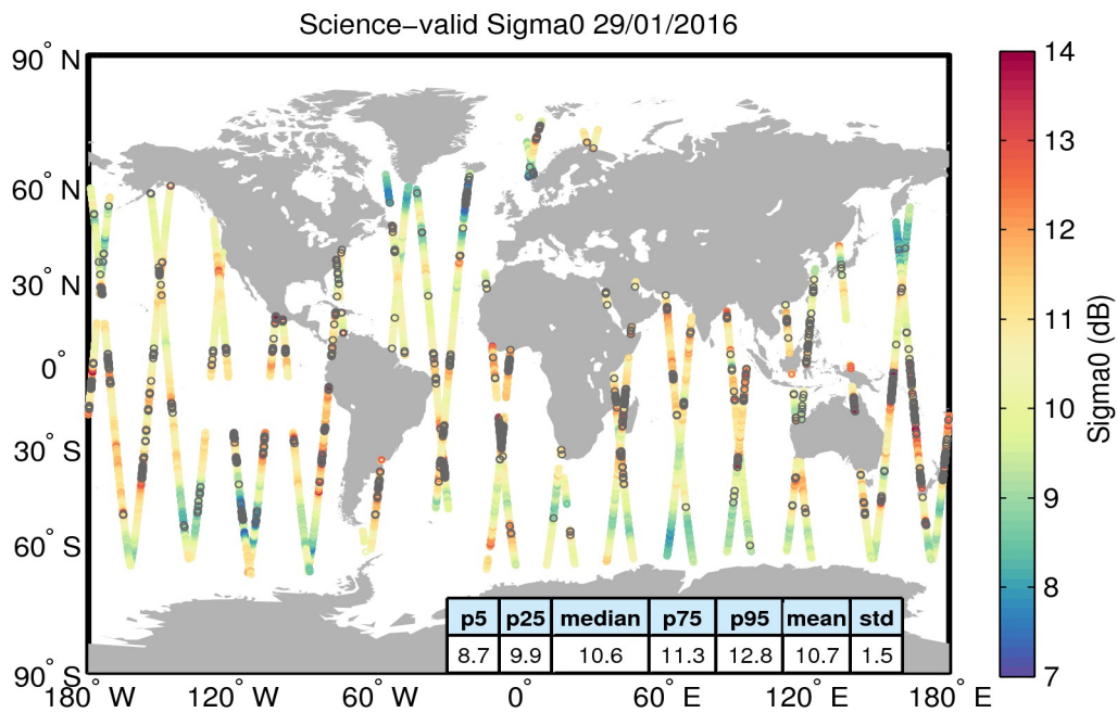
Figure 27. Geographical distribution of science-valid sigma0 data over oceans and lakes for 29/01/2016. The statistical values shown in the table refer to the sigma0 in dB and are calculated over all measurements shown in the figure. Gray circles denote records that have been rejected based on the editing criteria described in Table 4.
