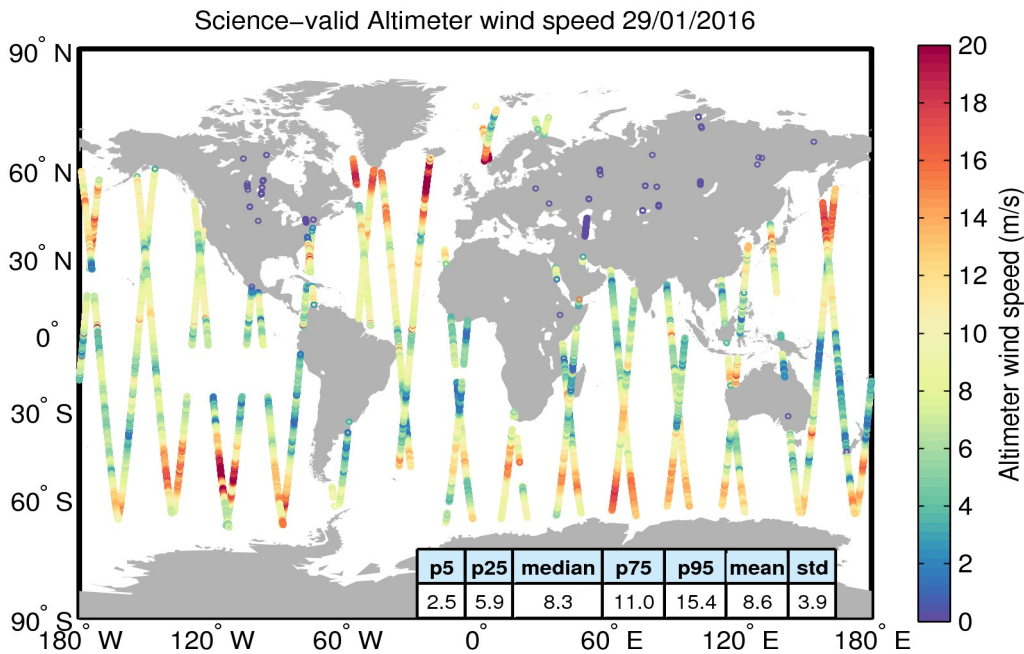
Figure 34. Geographical distribution of science-valid wind data over oceans and lakes for 29/01/2016. The statistical values shown in the table refer to the wind in m/s and are calculated over all measurements shown in the figure. Gray circles denote records that have been rejected based on the editing criteria described in Table 5.
