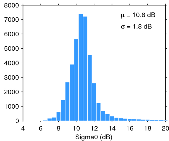
Figure 25. Histogram of flag-valid sigma0 over oceans and lakes for 29/01/2016. The mean ( \mu ) and standard deviation ( \sigma ) are also shown. Note that values outside [4 20] dB are excluded from the histogram for the sake of readability but not from the computation of \mu and \sigma .
