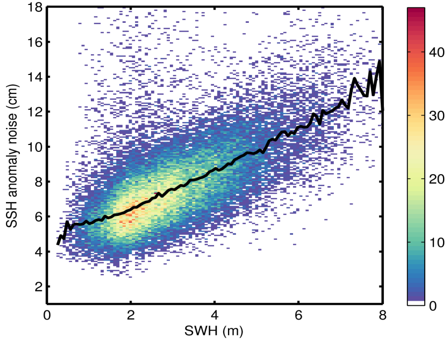
Figure 9. 2D histogram showing flag-valid SSH anomaly noise as a function of SWH for 29/01/2016. The black line denotes the median SSH anomaly noise as a function of SWH.
