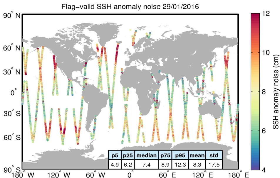
Figure 8. Geographical distribution of flag-valid 20-Hz SSH anomaly measurement noise over oceans and lakes for 29/01/2016. The statistical values shown in the table refer to the SSH anomaly noise and are calculated over all measurements shown in the figure.
