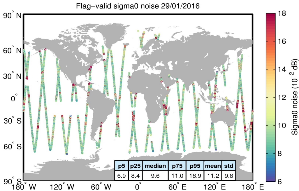
Figure 26. Geographical distribution of flag-valid 20-Hz sigma0 measurement noise over oceans and lakes for 29/01/2016. The statistical values shown in the table refer to the sigma0 noise and are calculated over all measurements shown in the figure.
