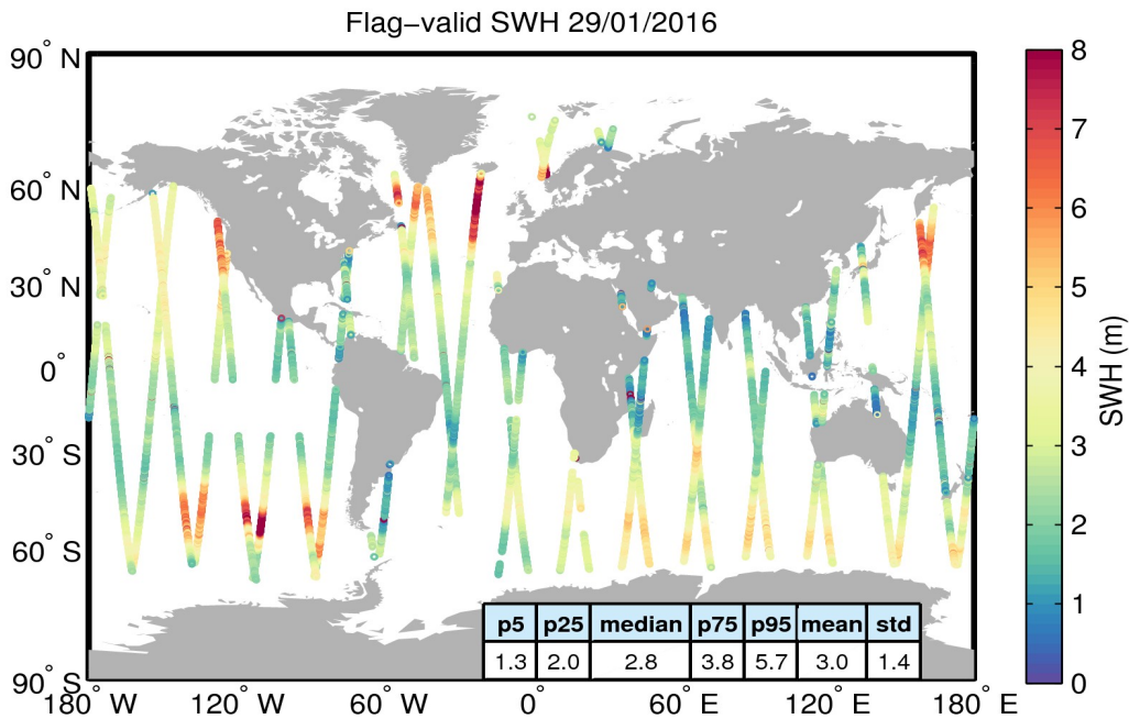
Figure 15. Geographical distribution of flag-valid SWH data over oceans and lakes for 29/01/2016. The statistical values shown in the table refer to the SWH in m and are calculated over all measurements shown in the figure.
