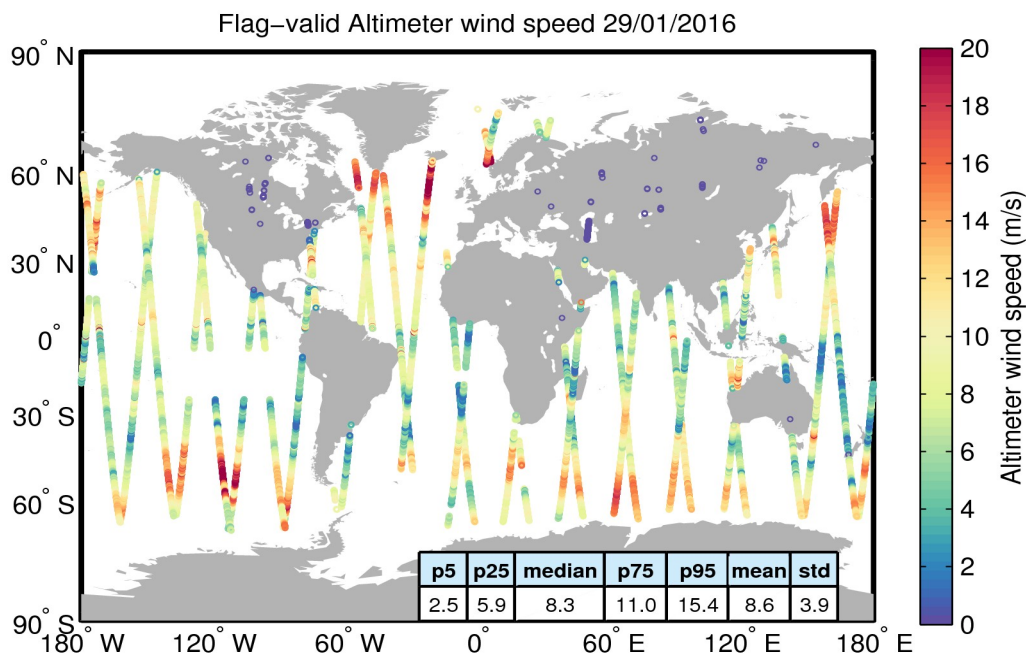
Figure 31. Geographical distribution of flag-valid wind data over oceans and lakes for 29/01/2016. The statistical values shown in the table refer to the wind in m/s and are calculated over all measurements shown in the figure.
