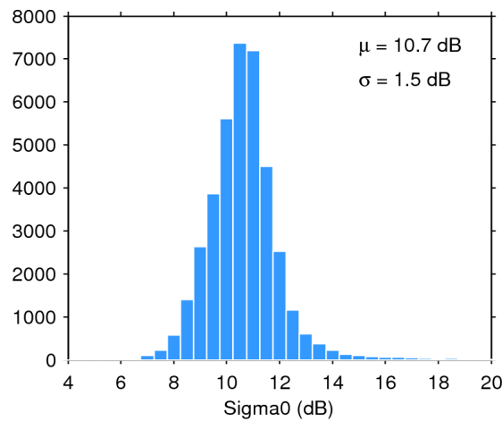
Figure 28. Histogram of science-valid sigma0 over oceans and lakes for 29/01/2016. The mean ( \mu ) and standard deviation ( \sigma ) are also shown. Note that values outside [4 20] dB are excluded from the histogram for the sake of readability but not from the computation of \mu and \sigma .
