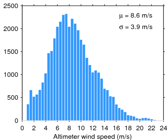
Figure 35. Histogram of science-valid wind over oceans and lakes for 29/01/2016. The mean ( \mu ) and standard deviation ( \sigma ) are also shown. Note that values larger than 24 m/s are excluded from the histogram for the sake of readability but not from the computation of \mu and \sigma .
