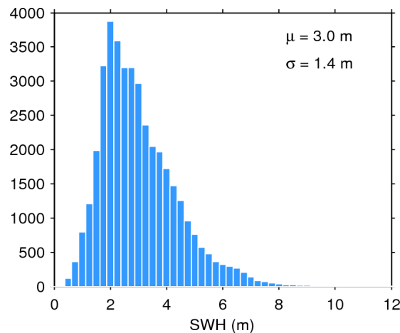
Figure 20. Histogram of science-valid SWH over oceans and lakes for 29/01/2016. The mean ( \mu ) and standard deviation ( \sigma ) are also shown. Note that values larger than 12 m are excluded from the histogram for the sake of readability but not from the computation of \mu and \sigma .
