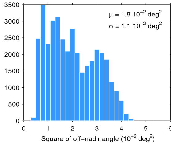
Figure 39. Histogram of flag-valid mispointing over oceans and lakes for 29/01/2016. The mean ( \mu ) and standard deviation ( \sigma ) are also shown. Note that values larger than 6 \cdot 10^{-2} \text{ deg}^2 are excluded from the histogram for the sake of readability but not from the computation of \mu and \sigma .
