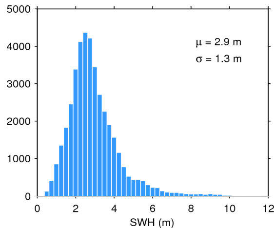
Figure 20. Histogram of science-valid SWH over oceans and lakes for 27/01/2016. The mean ( \mu ) and standard deviation ( \sigma ) are also shown. Note that values larger than 12 m are excluded from the histogram for the sake of readability but not from the computation of \mu and \sigma .
