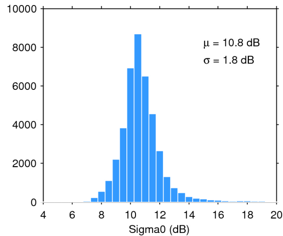
Figure 25. Histogram of flag-valid sigma0 over oceans and lakes for 27/01/2016. The mean ( \mu ) and standard deviation ( \sigma ) are also shown. Note that values outside [4 20] dB are excluded from the histogram for the sake of readability but not from the computation of \mu and \sigma .
