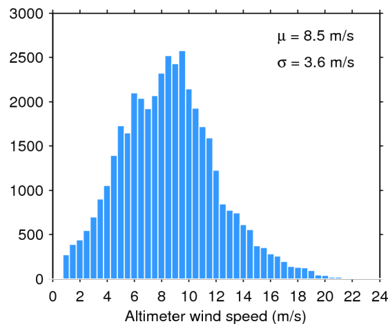
Figure 35. Histogram of science-valid wind over oceans and lakes for 27/01/2016. The mean ( \mu ) and standard deviation ( \sigma ) are also shown. Note that values larger than 24 m/s are excluded from the histogram for the sake of readability but not from the computation of \mu and \sigma .
