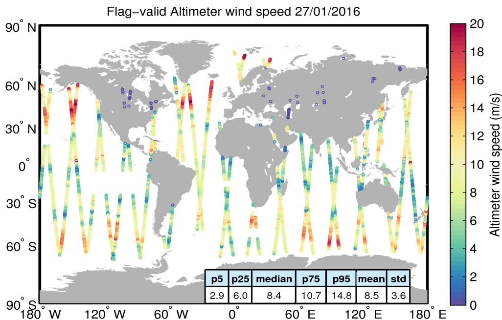
Figure 31. Geographical distribution of flag-valid wind data over oceans and lakes for 27/01/2016. The statistical values shown in the table refer to the wind in m/s and are calculated over all measurements shown in the figure.
