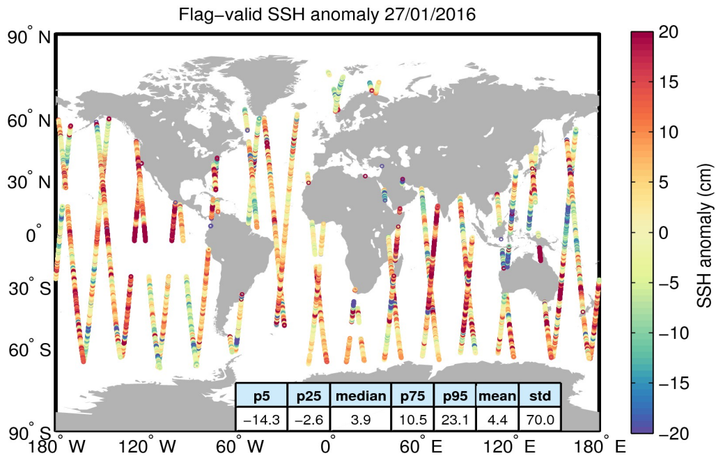
Figure 5. Geographical distribution of flag-valid 1-Hz SSH anomaly data over oceans and lakes for 27/01/2016. The statistical values shown in the table refer to the SSH anomaly in cm and are calculated over all measurements shown in the figure.
