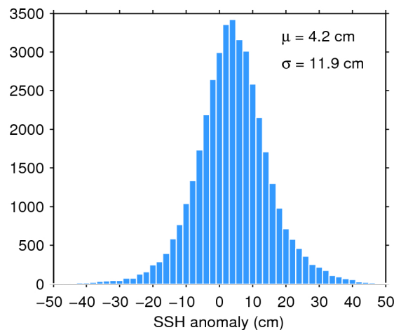
Figure 11. Histogram of science-valid SSH anomaly over oceans and lakes for 27/01/2016. The mean ( \mu ) and standard deviation ( \sigma ) are also shown. Note that values outside [-50 50] cm are excluded from the histogram for the sake of readability but not from the computation of \mu and \sigma .
