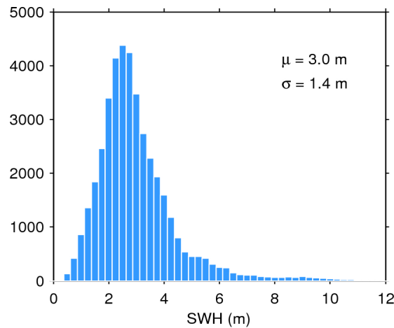
Figure 17. Histogram of flag-valid SWH over oceans and lakes for 27/01/2016. The mean ( \mu ) and standard deviation ( \sigma ) are also shown. Note that values larger than 12 m are excluded from the histogram for the sake of readability but not from the computation of \mu and \sigma .
