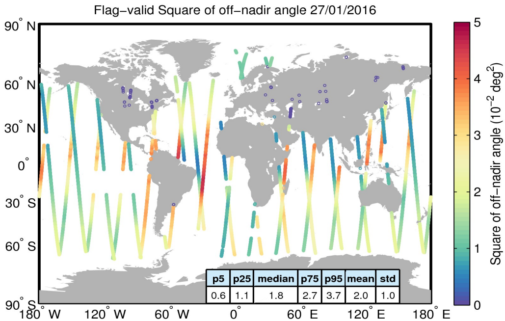
Figure 37. Geographical distribution of flag-valid mispointing data over oceans and lakes for 27/01/2016. The statistical values shown in the table refer to the mispointing in 10^{-2} deg 2 and are calculated over all measurements shown in the figure.
