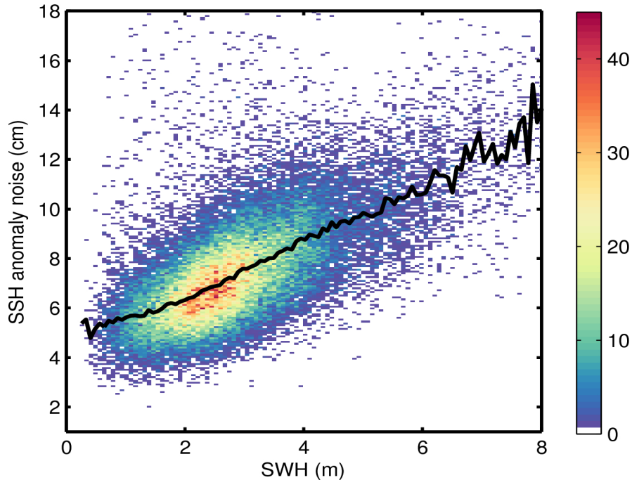
Figure 9. 2D histogram showing flag-valid SSH anomaly noise as a function of SWH for 27/01/2016. The black line denotes the median SSH anomaly noise as a function of SWH.
