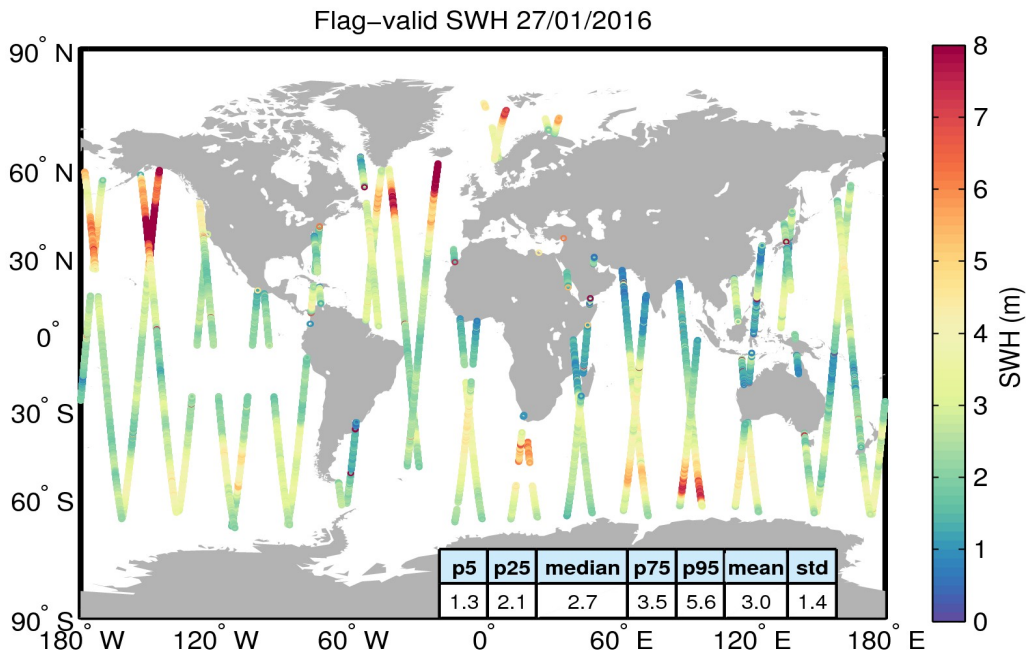
Figure 15. Geographical distribution of flag-valid SWH data over oceans and lakes for 27/01/2016. The statistical values shown in the table refer to the SWH in m and are calculated over all measurements shown in the figure.
