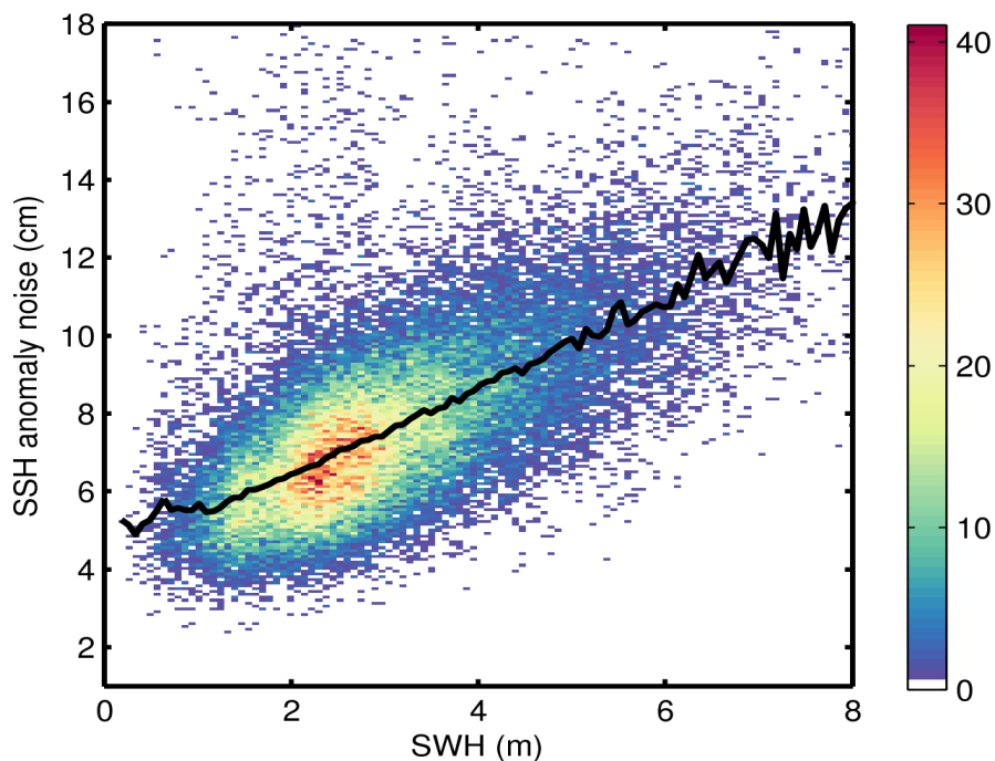
Figure 9. 2D histogram showing flag-valid SSH anomaly noise as a function of SWH for 25/01/2016. The black line denotes the median SSH anomaly noise as a function of SWH.
