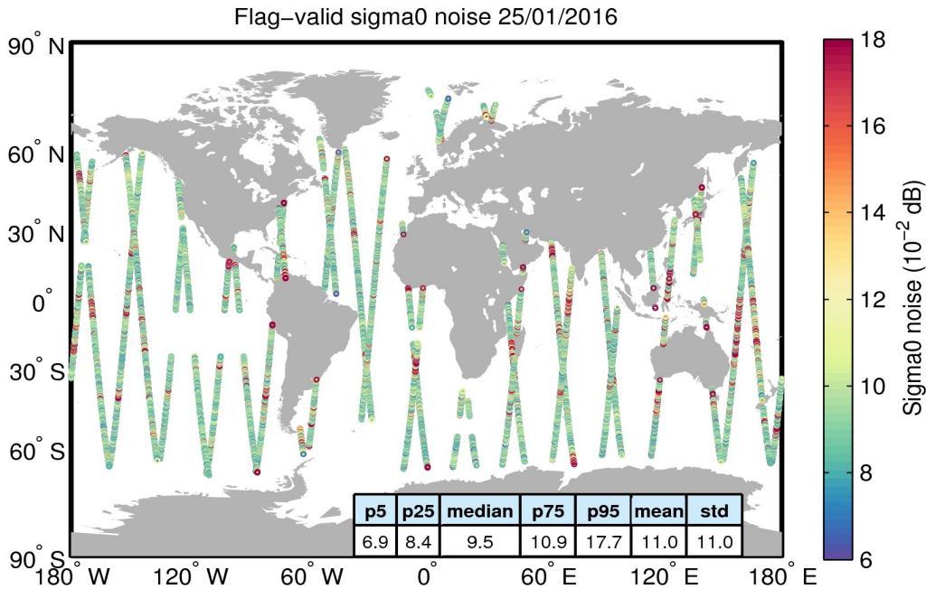
Figure 26. Geographical distribution of flag-valid 20-Hz sigma0 measurement noise over oceans and lakes for 25/01/2016. The statistical values shown in the table refer to the sigma0 noise and are calculated over all measurements shown in the figure.
