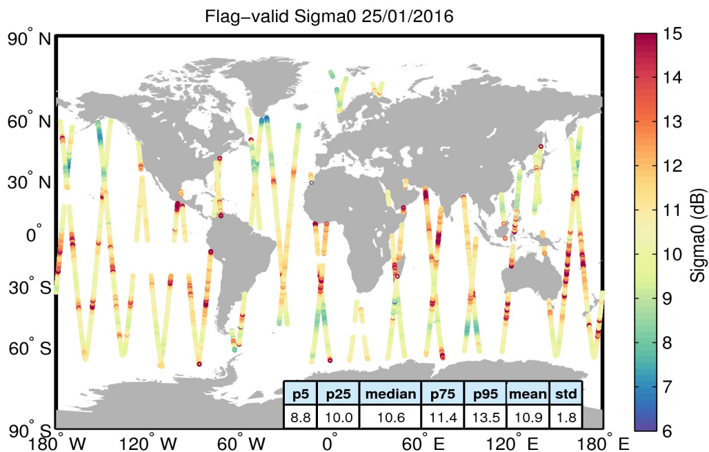
Figure 23. Geographical distribution of flag-valid sigma0 data over oceans and lakes for 25/01/2016. The statistical values shown in the table refer to the sigma0 in dB and are calculated over all measurements shown in the figure.
