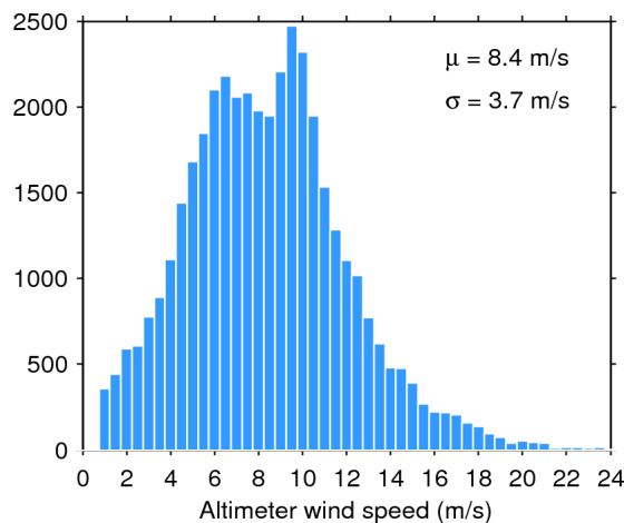
Figure 35. Histogram of science-valid wind over oceans and lakes for 25/01/2016. The mean ( \mu ) and standard deviation ( \sigma ) are also shown. Note that values larger than 24 m/s are excluded from the histogram for the sake of readability but not from the computation of \mu and \sigma .
