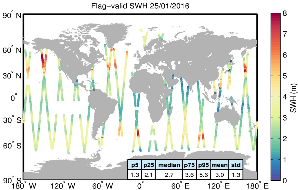
Figure 15. Geographical distribution of flag-valid SWH data over oceans and lakes for 25/01/2016. The statistical values shown in the table refer to the SWH in m and are calculated over all measurements shown in the figure.
