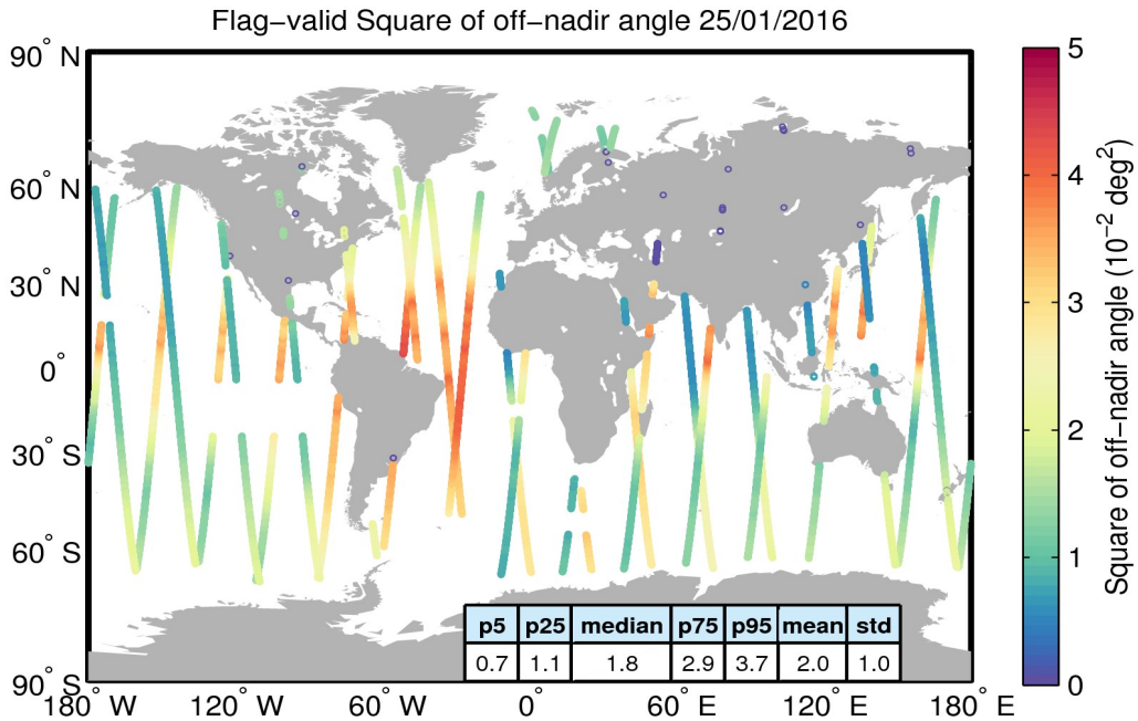
Figure 37. Geographical distribution of flag-valid mispointing data over oceans and lakes for 25/01/2016. The statistical values shown in the table refer to the mispointing in 10^{-2} \text{ deg}^2 and are calculated over all measurements shown in the figure.
