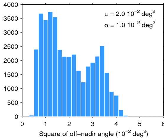
Figure 39. Histogram of flag-valid mispointing over oceans and lakes for 25/01/2016. The mean ( \mu ) and standard deviation ( \sigma ) are also shown. Note that values larger than 6 \cdot 10^{-2} \text{ deg}^2 are excluded from the histogram for the sake of readability but not from the computation of \mu and \sigma .
