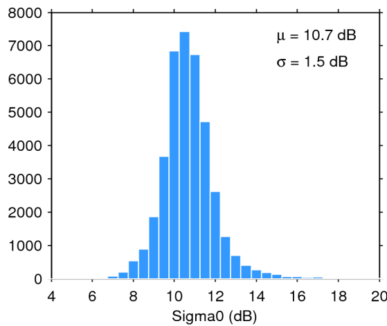
Figure 28. Histogram of science-valid sigma0 over oceans and lakes for 25/01/2016. The mean ( \mu ) and standard deviation ( \sigma ) are also shown. Note that values outside [4 20] dB are excluded from the histogram for the sake of readability but not from the computation of \mu and \sigma .
