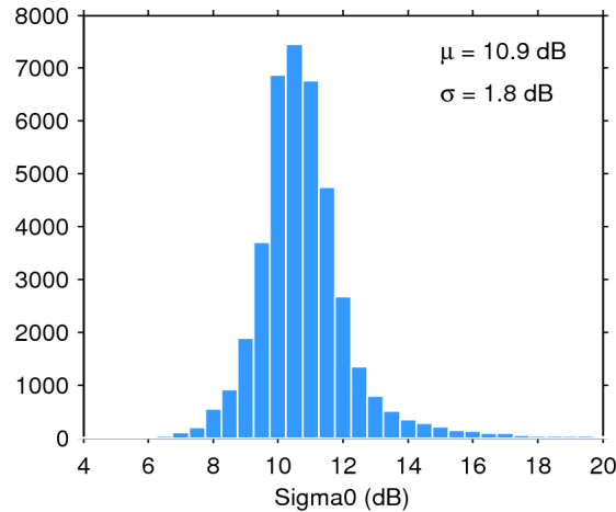
Figure 25. Histogram of flag-valid sigma0 over oceans and lakes for 25/01/2016. The mean ( \mu ) and standard deviation ( \sigma ) are also shown. Note that values outside [4 20] dB are excluded from the histogram for the sake of readability but not from the computation of \mu and \sigma .
