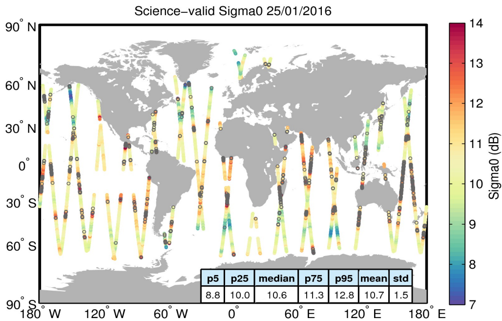
Figure 27. Geographical distribution of science-valid sigma0 data over oceans and lakes for 25/01/2016. The statistical values shown in the table refer to the sigma0 in dB and are calculated over all measurements shown in the figure. Gray circles denote records that have been rejected based on the editing criteria described in Table 4.
