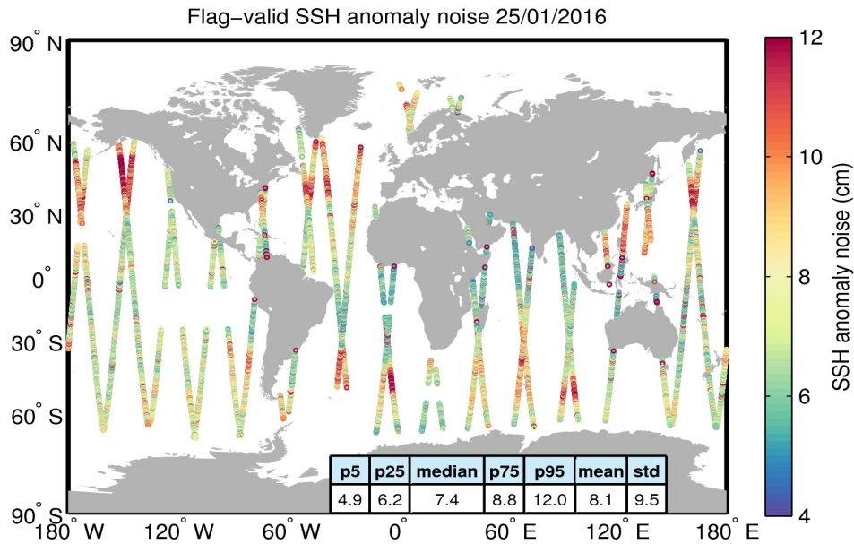
Figure 8. Geographical distribution of flag-valid 20-Hz SSH anomaly measurement noise over oceans and lakes for 25/01/2016. The statistical values shown in the table refer to the SSH anomaly noise and are calculated over all measurements shown in the figure.
