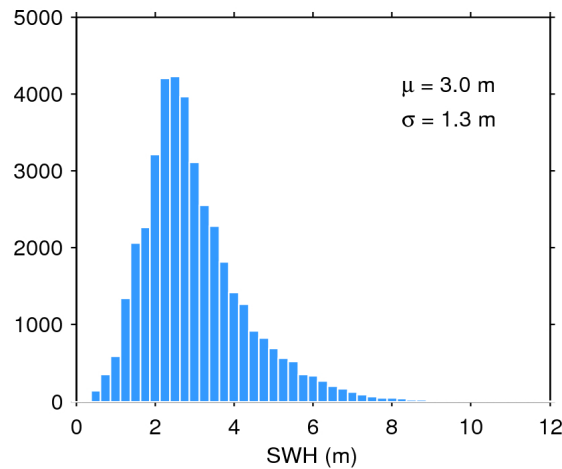
Figure 17. Histogram of flag-valid SWH over oceans and lakes for 25/01/2016. The mean ( \mu ) and standard deviation ( \sigma ) are also shown. Note that values larger than 12 m are excluded from the histogram for the sake of readability but not from the computation of \mu and \sigma .
