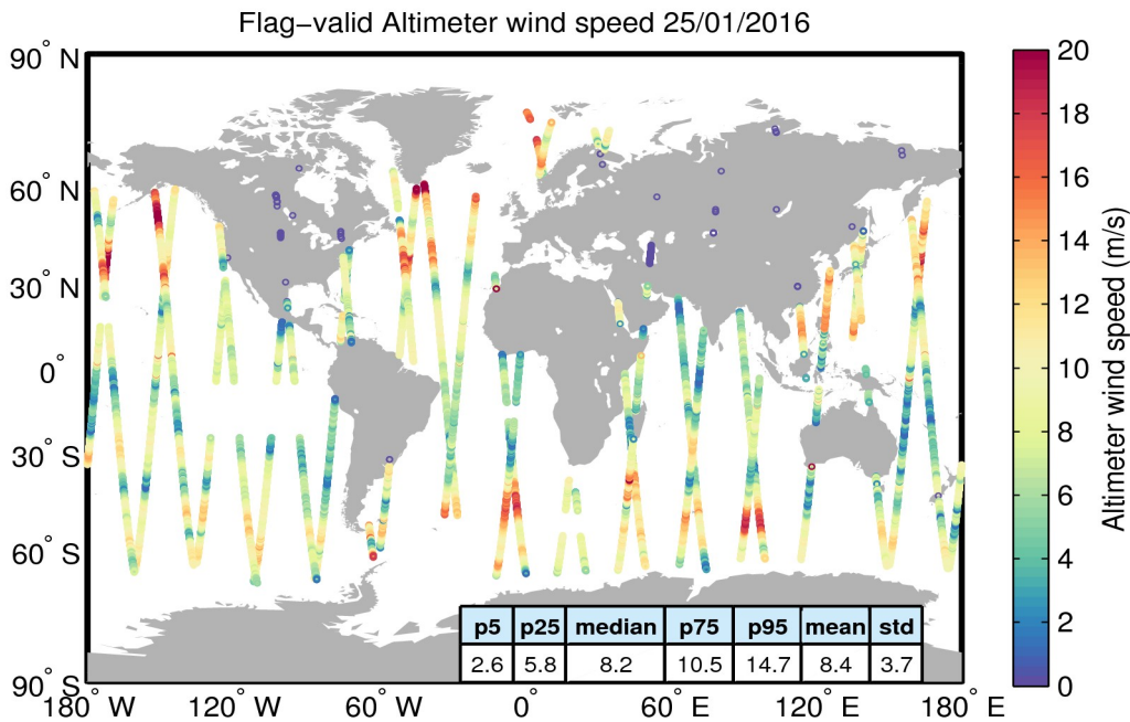
Figure 31. Geographical distribution of flag-valid wind data over oceans and lakes for 25/01/2016. The statistical values shown in the table refer to the wind in m/s and are calculated over all measurements shown in the figure.
