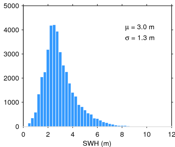
Figure 20. Histogram of science-valid SWH over oceans and lakes for 25/01/2016. The mean ( \mu ) and standard deviation ( \sigma ) are also shown. Note that values larger than 12 m are excluded from the histogram for the sake of readability but not from the computation of \mu and \sigma .
