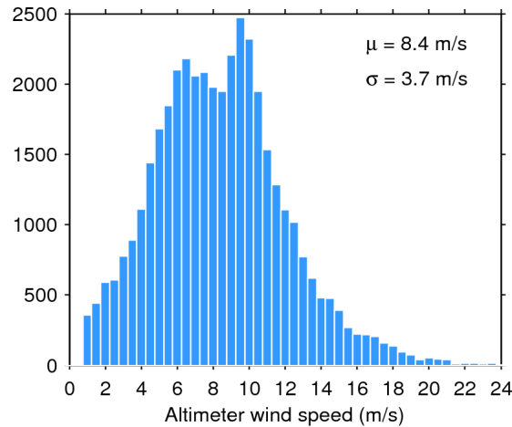
Figure 33. Histogram of flag-valid wind over oceans and lakes for 25/01/2016. The mean ( \mu ) and standard deviation ( \sigma ) are also shown. Note that values larger than 24 m/s are excluded from the histogram for the sake of readability but not from the computation of \mu and \sigma .
