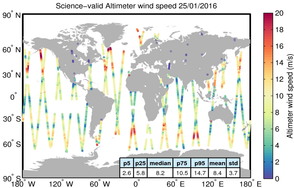
Figure 34. Geographical distribution of science-valid wind data over oceans and lakes for 25/01/2016. The statistical values shown in the table refer to the wind in m/s and are calculated over all measurements shown in the figure. Gray circles denote records that have been rejected based on the editing criteria described in Table 5.
