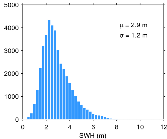
Figure 20. Histogram of science-valid SWH over oceans and lakes for 24/01/2016. The mean ( \mu ) and standard deviation ( \sigma ) are also shown. Note that values larger than 12 m are excluded from the histogram for the sake of readability but not from the computation of \mu and \sigma .
