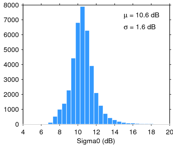
Figure 28. Histogram of science-valid sigma0 over oceans and lakes for 24/01/2016. The mean ( \mu ) and standard deviation ( \sigma ) are also shown. Note that values outside [4 20] dB are excluded from the histogram for the sake of readability but not from the computation of \mu and \sigma .
