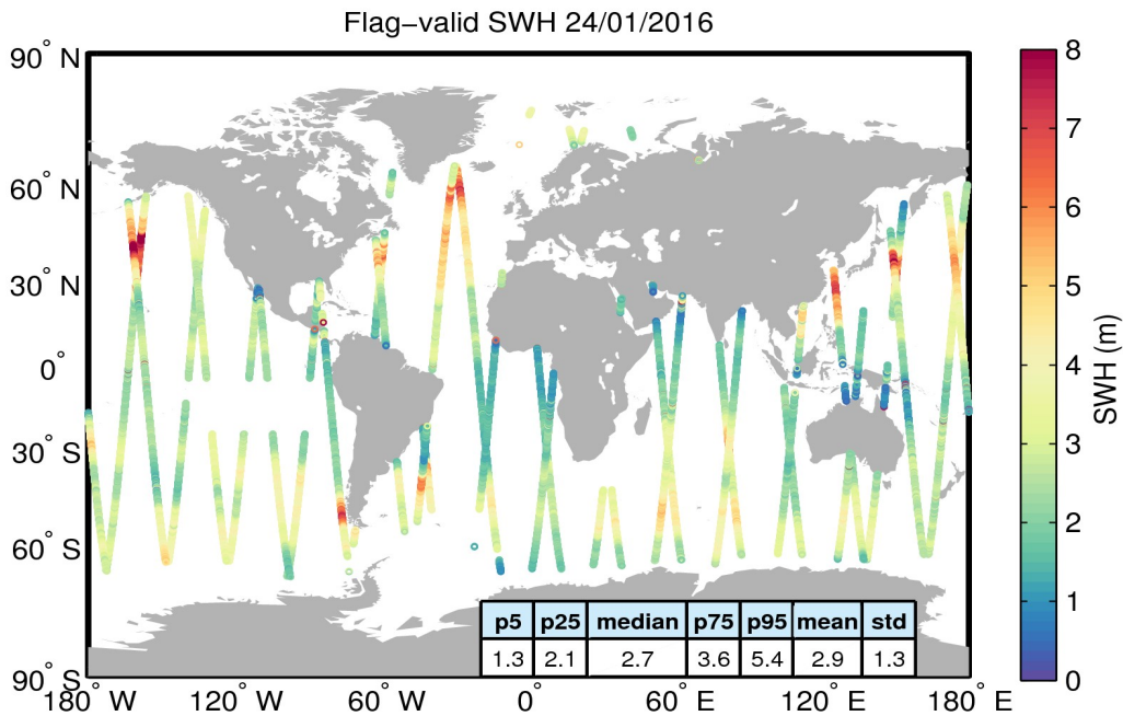
Figure 15. Geographical distribution of flag-valid SWH data over oceans and lakes for 24/01/2016. The statistical values shown in the table refer to the SWH in m and are calculated over all measurements shown in the figure.
