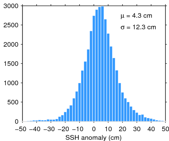
Figure 11. Histogram of science-valid SSH anomaly over oceans and lakes for 24/01/2016. The mean ( \mu ) and standard deviation ( \sigma ) are also shown. Note that values outside [-50 50] cm are excluded from the histogram for the sake of readability but not from the computation of \mu and \sigma .
