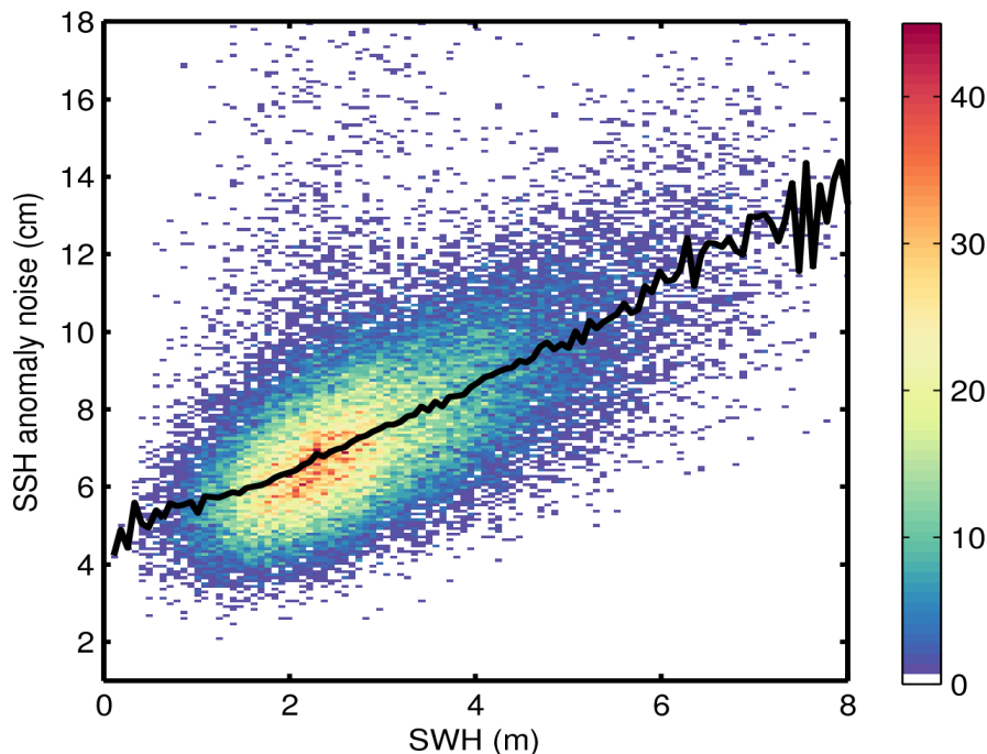
Figure 9. 2D histogram showing flag-valid SSH anomaly noise as a function of SWH for 24/01/2016. The black line denotes the median SSH anomaly noise as a function of SWH.
