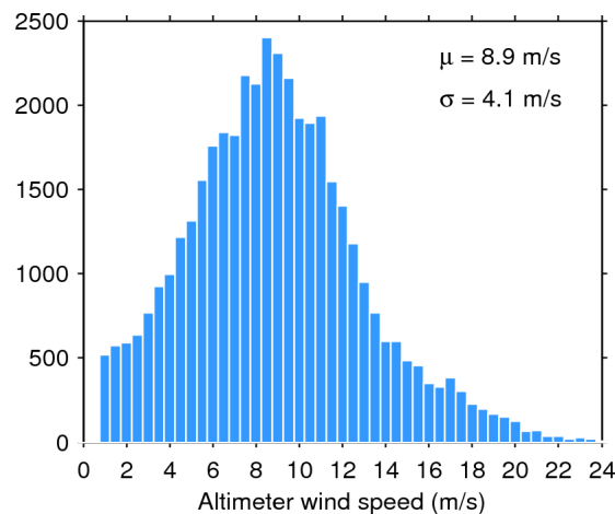
Figure 35. Histogram of science-valid wind over oceans and lakes for 24/01/2016. The mean ( \mu ) and standard deviation ( \sigma ) are also shown. Note that values larger than 24 m/s are excluded from the histogram for the sake of readability but not from the computation of \mu and \sigma .
