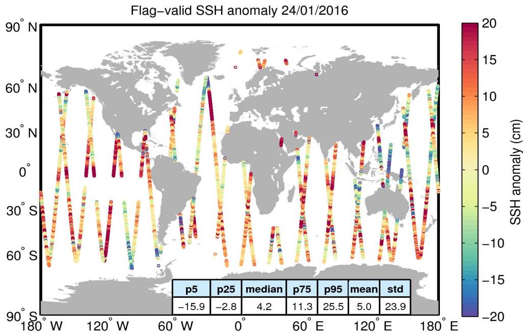
Figure 5. Geographical distribution of flag-valid 1-Hz SSH anomaly data over oceans and lakes for 24/01/2016. The statistical values shown in the table refer to the SSH anomaly in cm and are calculated over all measurements shown in the figure.
