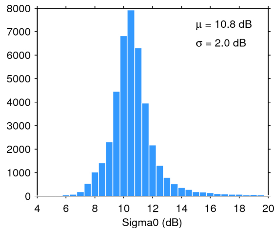
Figure 25. Histogram of flag-valid sigma0 over oceans and lakes for 24/01/2016. The mean ( \mu ) and standard deviation ( \sigma ) are also shown. Note that values outside [4 20] dB are excluded from the histogram for the sake of readability but not from the computation of \mu and \sigma .
