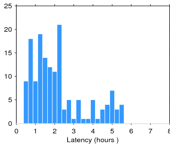
Figure 2. Histogram of the data latency for 24/01/2016. The y-axis denotes the number of files that are made available with a delay of x-hours with respect to the mean time of the records stored in the file.
