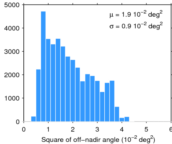
Figure 39. Histogram of flag-valid mispointing over oceans and lakes for 24/01/2016. The mean ( \mu ) and standard deviation ( \sigma ) are also shown. Note that values larger than 6 \cdot 10^{-2} \text{ deg}^2 are excluded from the histogram for the sake of readability but not from the computation of \mu and \sigma .
