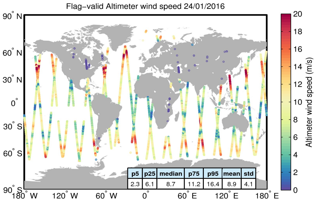
Figure 31. Geographical distribution of flag-valid wind data over oceans and lakes for 24/01/2016. The statistical values shown in the table refer to the wind in m/s and are calculated over all measurements shown in the figure.
