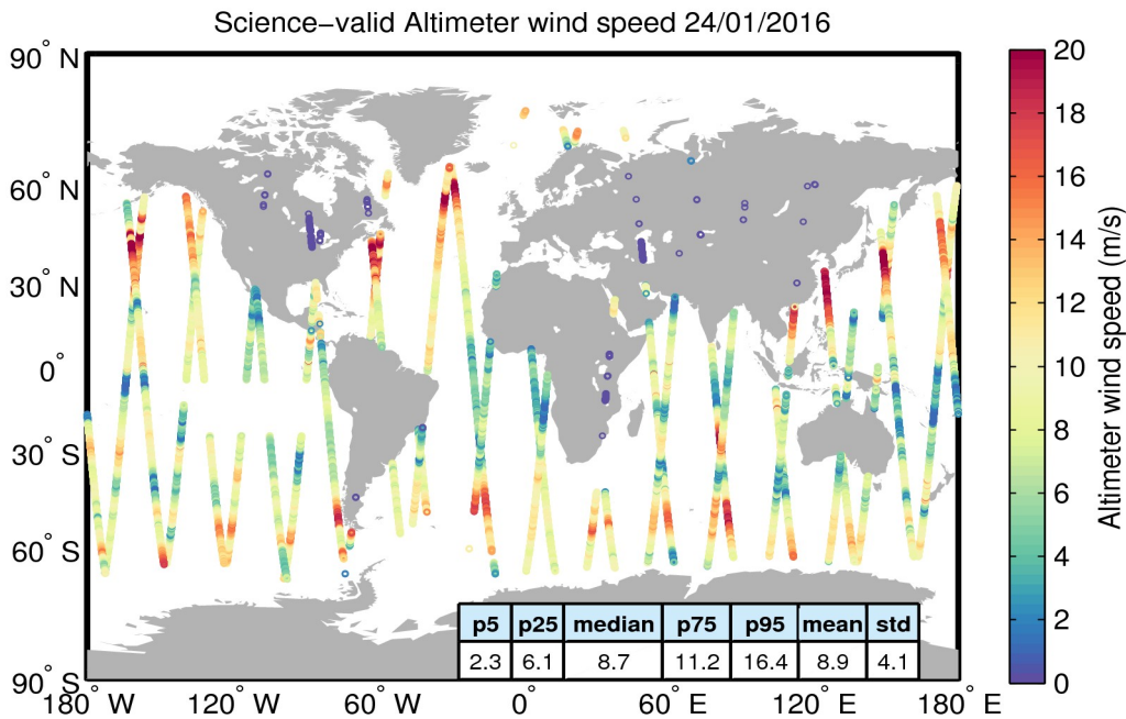
Figure 34. Geographical distribution of science-valid wind data over oceans and lakes for 24/01/2016. The statistical values shown in the table refer to the wind in m/s and are calculated over all measurements shown in the figure. Gray circles denote records that have been rejected based on the editing criteria described in Table 5.
