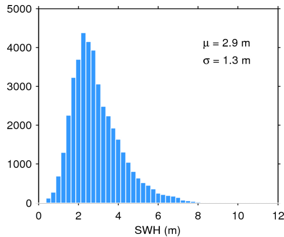
Figure 17. Histogram of flag-valid SWH over oceans and lakes for 24/01/2016. The mean ( \mu ) and standard deviation ( \sigma ) are also shown. Note that values larger than 12 m are excluded from the histogram for the sake of readability but not from the computation of \mu and \sigma .
