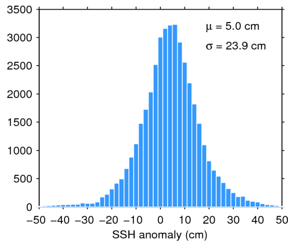
Figure 7. Histogram of flag-valid SSH anomaly over oceans and lakes for 24/01/2016. The mean ( \mu ) and standard deviation ( \sigma ) are also shown. Note that values outside [-50\ 50] cm are excluded from the histogram for the sake of readability but not from the computation of \mu and \sigma .
