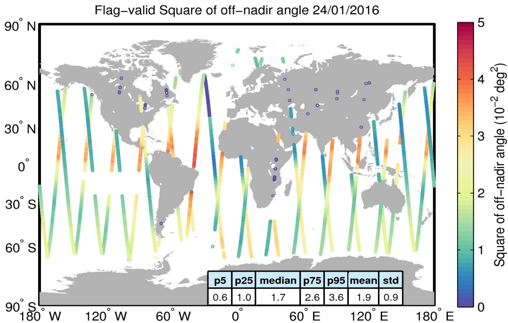
Figure 37. Geographical distribution of flag-valid mispointing data over oceans and lakes for 24/01/2016. The statistical values shown in the table refer to the mispointing in 10^{-2} deg 2 and are calculated over all measurements shown in the figure.
