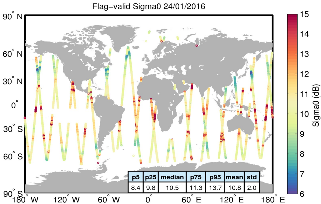
Figure 23. Geographical distribution of flag-valid sigma0 data over oceans and lakes for 24/01/2016. The statistical values shown in the table refer to the sigma0 in dB and are calculated over all measurements shown in the figure.
