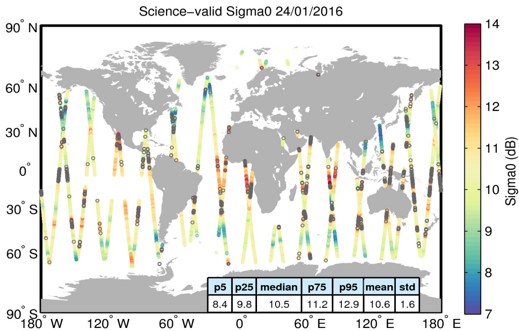
Figure 27. Geographical distribution of science-valid sigma0 data over oceans and lakes for 24/01/2016. The statistical values shown in the table refer to the sigma0 in dB and are calculated over all measurements shown in the figure. Gray circles denote records that have been rejected based on the editing criteria described in Table 4.
