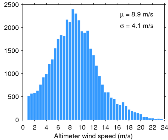
Figure 33. Histogram of flag-valid wind over oceans and lakes for 24/01/2016. The mean ( \mu ) and standard deviation ( \sigma ) are also shown. Note that values larger than 24 m/s are excluded from the histogram for the sake of readability but not from the computation of \mu and \sigma .
