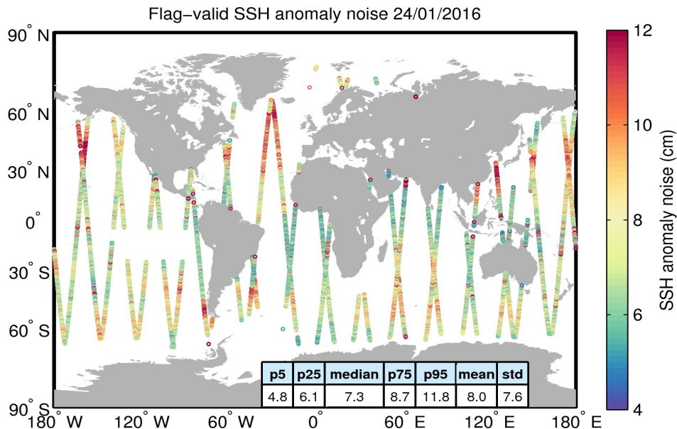
Figure 8. Geographical distribution of flag-valid 20-Hz SSH anomaly measurement noise over oceans and lakes for 24/01/2016. The statistical values shown in the table refer to the SSH anomaly noise and are calculated over all measurements shown in the figure.
