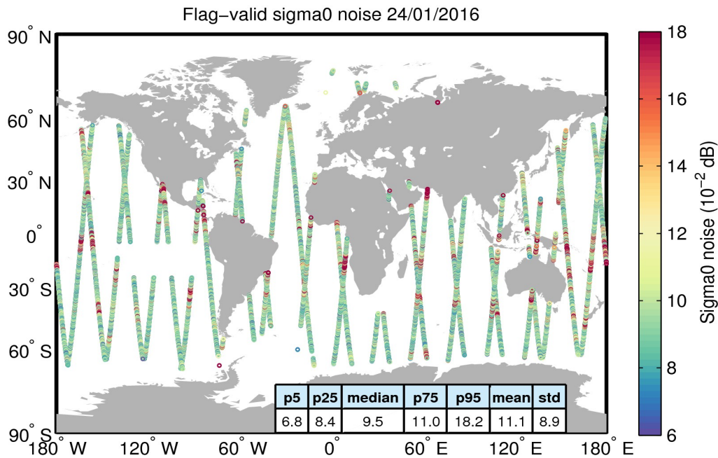
Figure 26. Geographical distribution of flag-valid 20-Hz sigma0 measurement noise over oceans and lakes for 24/01/2016. The statistical values shown in the table refer to the sigma0 noise and are calculated over all measurements shown in the figure.
