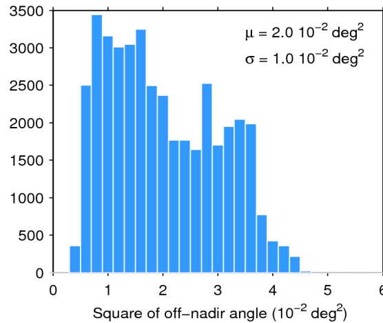
Figure 39. Histogram of flag-valid mispointing over oceans and lakes for 23/01/2016. The mean ( \mu ) and standard deviation ( \sigma ) are also shown. Note that values larger than 6 \cdot 10^{-2} \text{ deg}^2 are excluded from the histogram for the sake of readability but not from the computation of \mu and \sigma .
