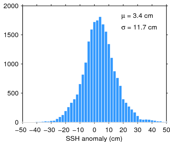
Figure 11. Histogram of science-valid SSH anomaly over oceans and lakes for 23/01/2016. The mean ( \mu ) and standard deviation ( \sigma ) are also shown. Note that values outside [-50 50] cm are excluded from the histogram for the sake of readability but not from the computation of \mu and \sigma .
