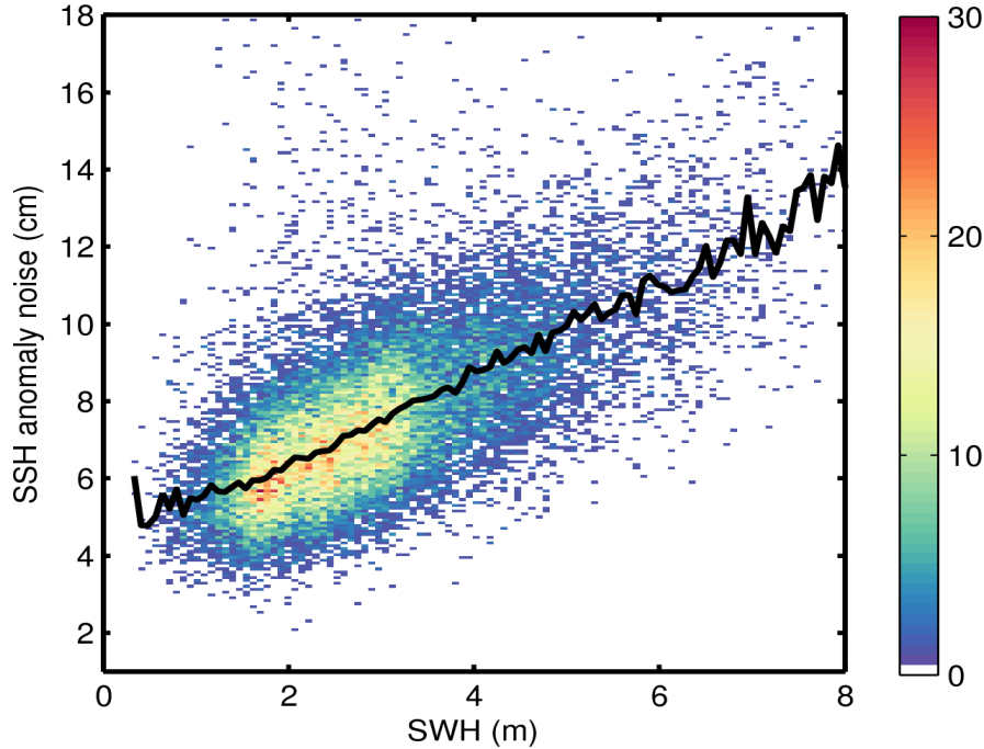
Figure 9. 2D histogram showing flag-valid SSH anomaly noise as a function of SWH for 23/01/2016. The black line denotes the median SSH anomaly noise as a function of SWH.
