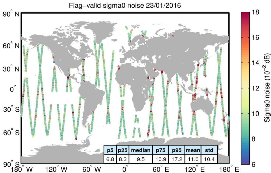
Figure 26. Geographical distribution of flag-valid 20-Hz sigma0 measurement noise over oceans and lakes for 23/01/2016. The statistical values shown in the table refer to the sigma0 noise and are calculated over all measurements shown in the figure.
