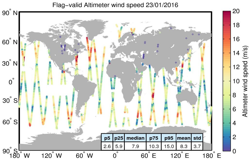
Figure 31. Geographical distribution of flag-valid wind data over oceans and lakes for 23/01/2016. The statistical values shown in the table refer to the wind in m/s and are calculated over all measurements shown in the figure.
