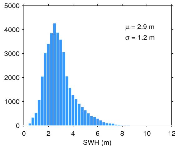
Figure 20. Histogram of science-valid SWH over oceans and lakes for 23/01/2016. The mean ( \mu ) and standard deviation ( \sigma ) are also shown. Note that values larger than 12 m are excluded from the histogram for the sake of readability but not from the computation of \mu and \sigma .
