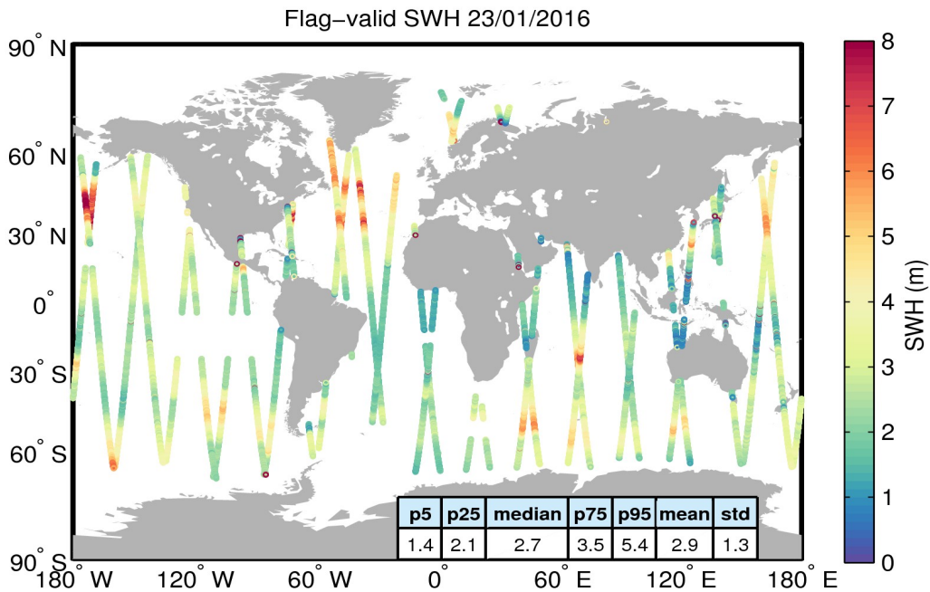
Figure 15. Geographical distribution of flag-valid SWH data over oceans and lakes for 23/01/2016. The statistical values shown in the table refer to the SWH in m and are calculated over all measurements shown in the figure.
