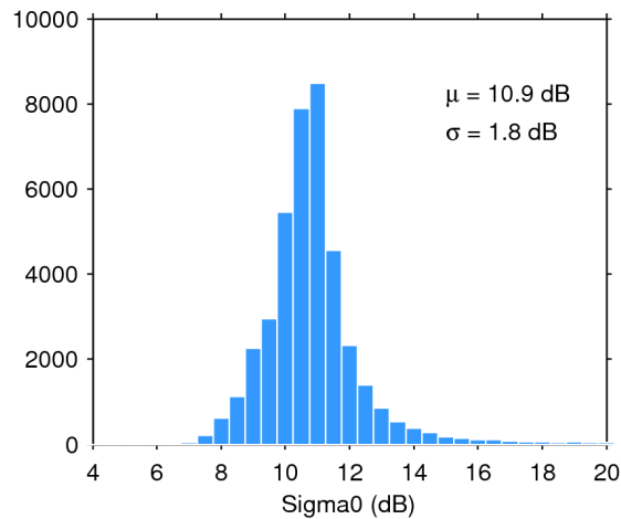
Figure 25. Histogram of flag-valid sigma0 over oceans and lakes for 23/01/2016. The mean ( \mu ) and standard deviation ( \sigma ) are also shown. Note that values outside [4 20] dB are excluded from the histogram for the sake of readability but not from the computation of \mu and \sigma .
