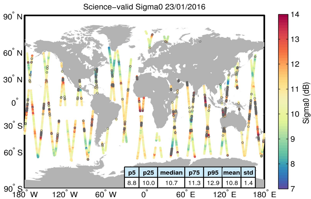
Figure 27. Geographical distribution of science-valid sigma0 data over oceans and lakes for 23/01/2016. The statistical values shown in the table refer to the sigma0 in dB and are calculated over all measurements shown in the figure. Gray circles denote records that have been rejected based on the editing criteria described in Table 4.
