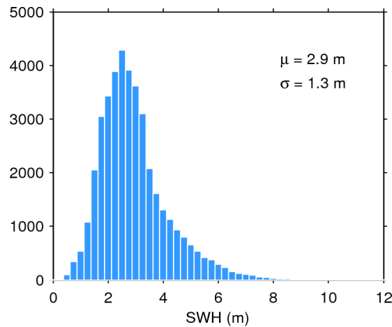
Figure 17. Histogram of flag-valid SWH over oceans and lakes for 23/01/2016. The mean ( \mu ) and standard deviation ( \sigma ) are also shown. Note that values larger than 12 m are excluded from the histogram for the sake of readability but not from the computation of \mu and \sigma .
