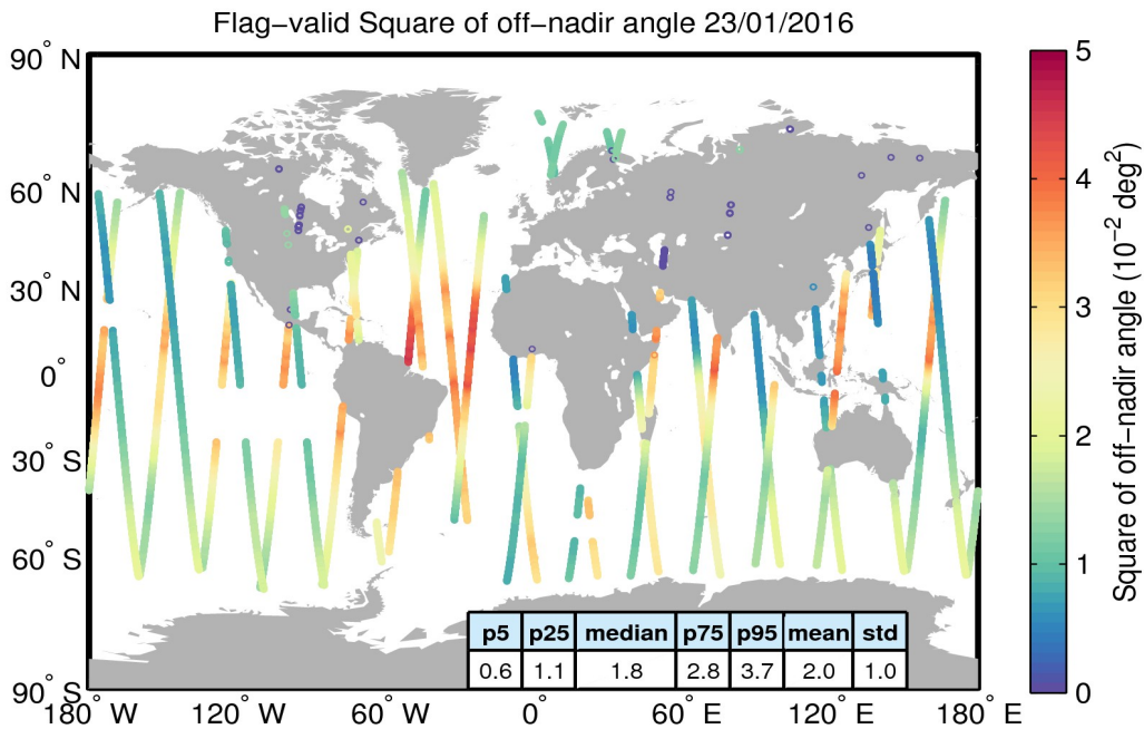
Figure 37. Geographical distribution of flag-valid mispointing data over oceans and lakes for 23/01/2016. The statistical values shown in the table refer to the mispointing in 10^{-2} \text{deg}^2 and are calculated over all measurements shown in the figure.
