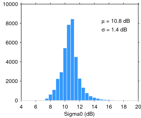
Figure 28. Histogram of science-valid sigma0 over oceans and lakes for 23/01/2016. The mean ( \mu ) and standard deviation ( \sigma ) are also shown. Note that values outside [4 20] dB are excluded from the histogram for the sake of readability but not from the computation of \mu and \sigma .
