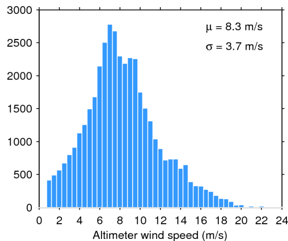
Figure 35. Histogram of science-valid wind over oceans and lakes for 23/01/2016. The mean ( \mu ) and standard deviation ( \sigma ) are also shown. Note that values larger than 24 m/s are excluded from the histogram for the sake of readability but not from the computation of \mu and \sigma .
