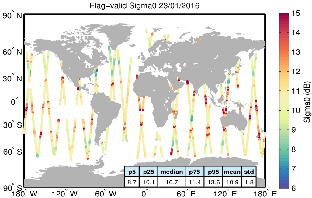
Figure 23. Geographical distribution of flag-valid sigma0 data over oceans and lakes for 23/01/2016. The statistical values shown in the table refer to the sigma0 in dB and are calculated over all measurements shown in the figure.
