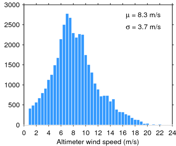
Figure 33. Histogram of flag-valid wind over oceans and lakes for 23/01/2016. The mean ( \mu ) and standard deviation ( \sigma ) are also shown. Note that values larger than 24 m/s are excluded from the histogram for the sake of readability but not from the computation of \mu and \sigma .
