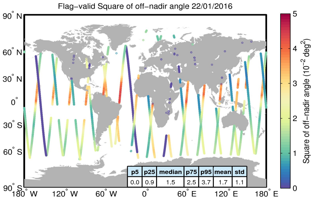
Figure 37. Geographical distribution of flag-valid mispointing data over oceans and lakes for 22/01/2016. The statistical values shown in the table refer to the mispointing in 10^{-2} \text{ deg}^2 and are calculated over all measurements shown in the figure.
