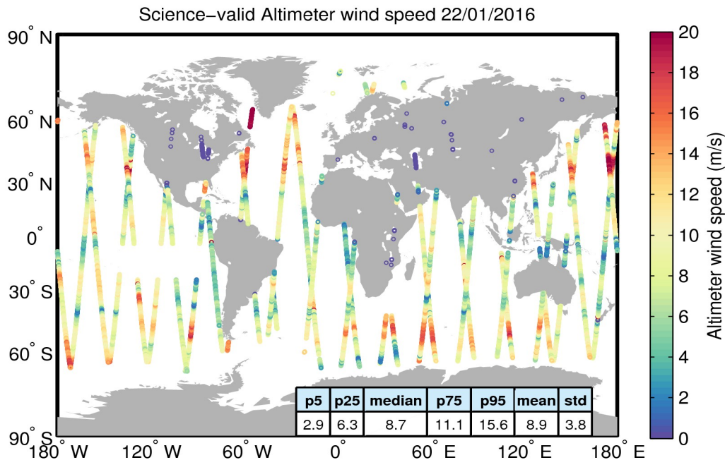
Figure 34. Geographical distribution of science-valid wind data over oceans and lakes for 22/01/2016. The statistical values shown in the table refer to the wind in m/s and are calculated over all measurements shown in the figure. Gray circles denote records that have been rejected based on the editing criteria described in Table 5.
