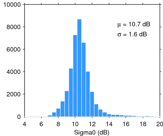
Figure 25. Histogram of flag-valid sigma0 over oceans and lakes for 22/01/2016. The mean ( \mu ) and standard deviation ( \sigma ) are also shown. Note that values outside [4 20] dB are excluded from the histogram for the sake of readability but not from the computation of \mu and \sigma .
