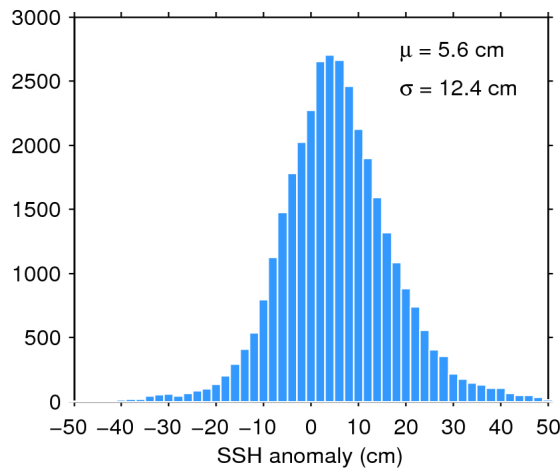
Figure 11. Histogram of science-valid SSH anomaly over oceans and lakes for 22/01/2016. The mean ( \mu ) and standard deviation ( \sigma ) are also shown. Note that values outside [-50 50] cm are excluded from the histogram for the sake of readability but not from the computation of \mu and \sigma .
