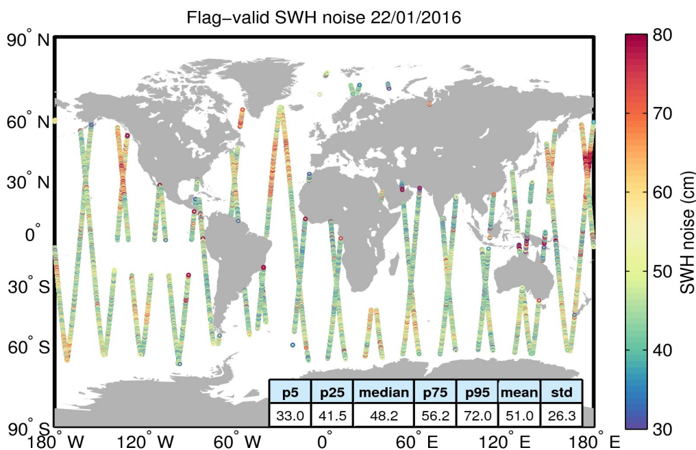
Figure 18. Geographical distribution of flag-valid 20-Hz SWH measurement noise over oceans and lakes for 22/01/2016. The statistical values shown in the figure refer to the SWH noise and are calculated over all measurements shown in the figure.
