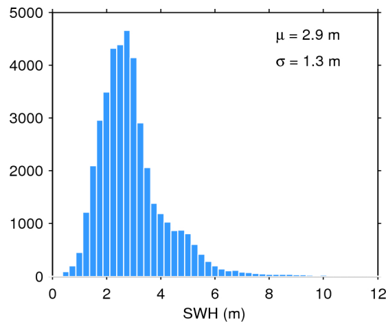
Figure 17. Histogram of flag-valid SWH over oceans and lakes for 22/01/2016. The mean ( \mu ) and standard deviation ( \sigma ) are also shown. Note that values larger than 12 m are excluded from the histogram for the sake of readability but not from the computation of \mu and \sigma .
