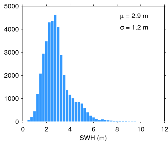
Figure 20. Histogram of science-valid SWH over oceans and lakes for 22/01/2016. The mean ( \mu ) and standard deviation ( \sigma ) are also shown. Note that values larger than 12 m are excluded from the histogram for the sake of readability but not from the computation of \mu and \sigma .
