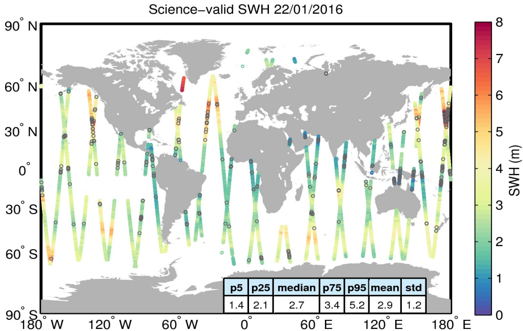
Figure 19. Geographical distribution of science-valid SWH data over oceans and lakes for 22/01/2016. The statistical values shown in the table refer to the SWH in m and are calculated over all measurements shown in the figure. Gray circles denote records that have been rejected based on the editing criteria described in Table 3.
