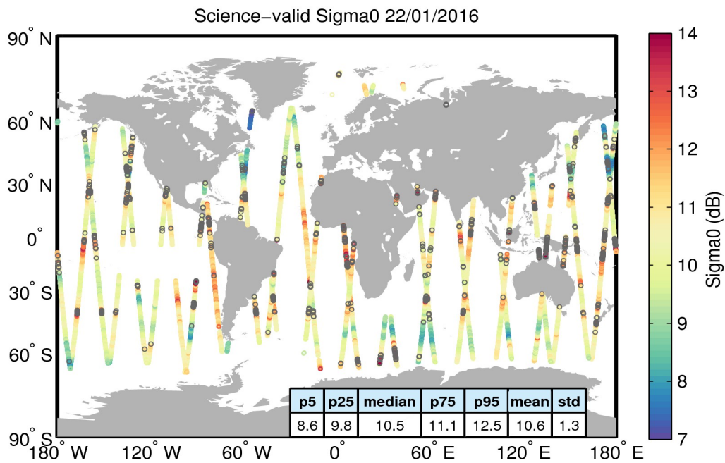
Figure 27. Geographical distribution of science-valid sigma0 data over oceans and lakes for 22/01/2016. The statistical values shown in the table refer to the sigma0 in dB and are calculated over all measurements shown in the figure. Gray circles denote records that have been rejected based on the editing criteria described in Table 4.
