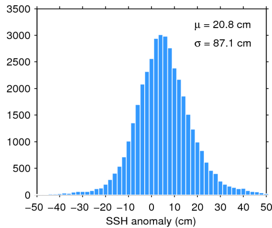
Figure 7. Histogram of flag-valid SSH anomaly over oceans and lakes for 22/01/2016. The mean ( \mu ) and standard deviation ( \sigma ) are also shown. Note that values outside [-50 50] cm are excluded from the histogram for the sake of readability but not from the computation of \mu and \sigma .
