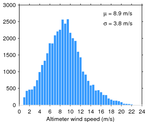
Figure 35. Histogram of science-valid wind over oceans and lakes for 22/01/2016. The mean ( \mu ) and standard deviation ( \sigma ) are also shown. Note that values larger than 24 m/s are excluded from the histogram for the sake of readability but not from the computation of \mu and \sigma .
