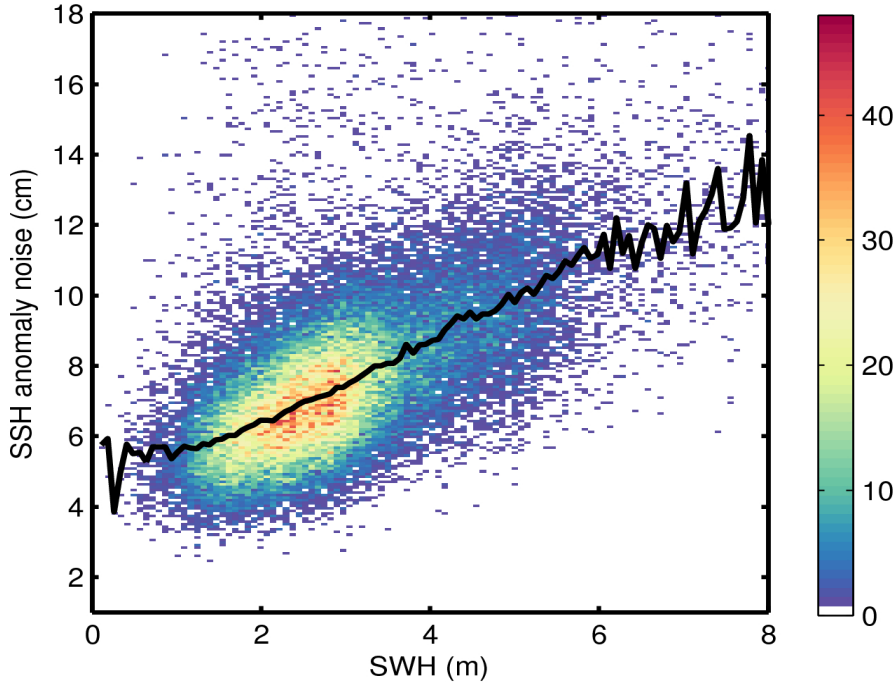
Figure 9. 2D histogram showing flag-valid SSH anomaly noise as a function of SWH for 22/01/2016. The black line denotes the median SSH anomaly noise as a function of SWH.
