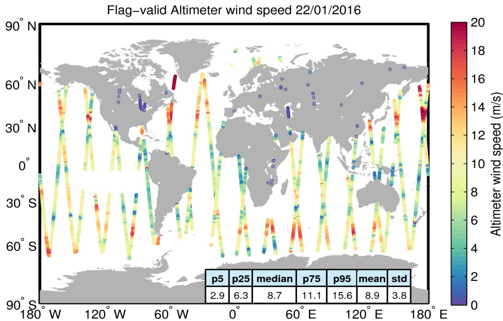
Figure 31. Geographical distribution of flag-valid wind data over oceans and lakes for 22/01/2016. The statistical values shown in the figure refer to the wind in m/s and are calculated over all measurements shown in the figure.
