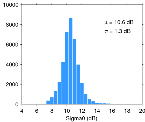
Figure 28. Histogram of science-valid sigma0 over oceans and lakes for 22/01/2016. The mean ( \mu ) and standard deviation ( \sigma ) are also shown. Note that values outside [4 20] dB are excluded from the histogram for the sake of readability but not from the computation of \mu and \sigma .
