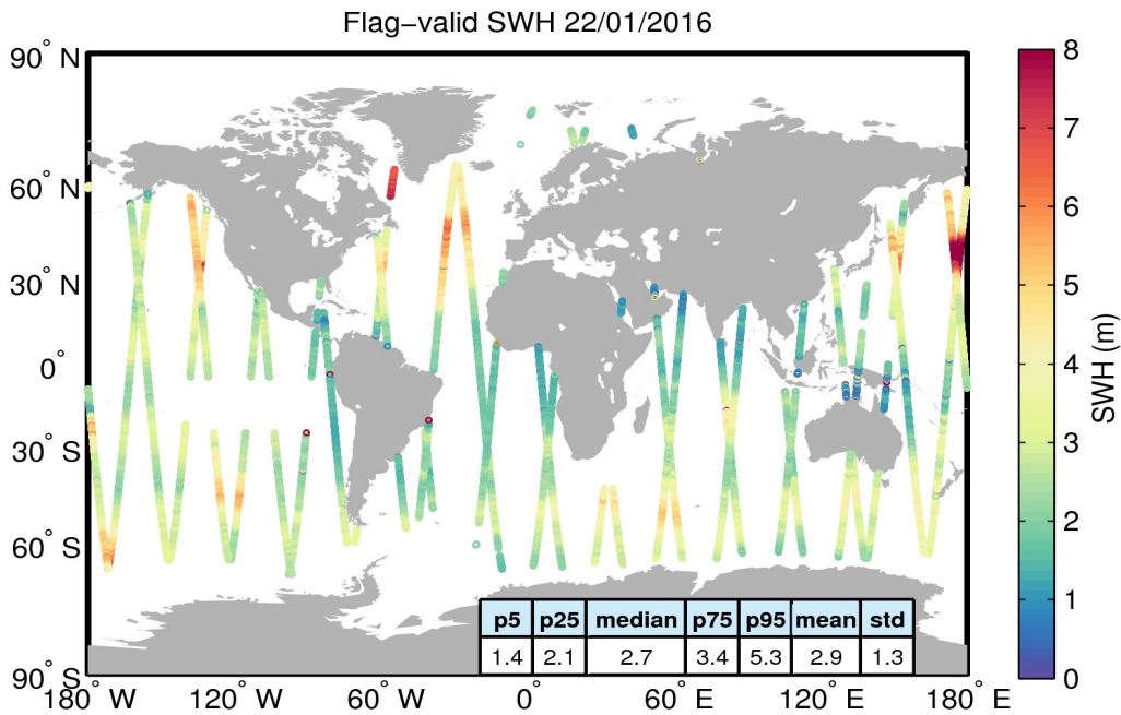
Figure 15. Geographical distribution of flag-valid SWH data over oceans and lakes for 22/01/2016. The statistical values shown in the table refer to the SWH in m and are calculated over all measurements shown in the figure.
