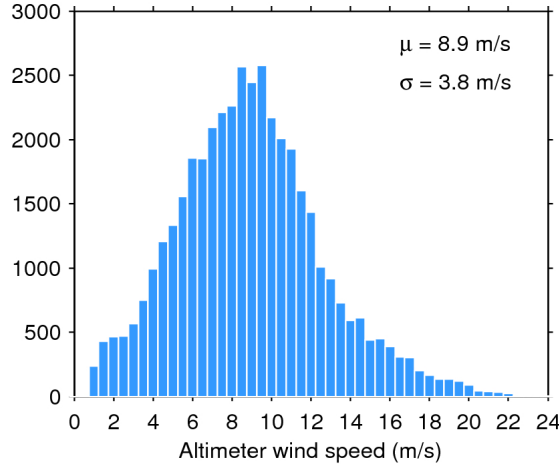
Figure 33. Histogram of flag-valid wind over oceans and lakes for 22/01/2016. The mean ( \mu ) and standard deviation ( \sigma ) are also shown. Note that values larger than 24 m/s are excluded from the histogram for the sake of readability but not from the computation of \mu and \sigma .
