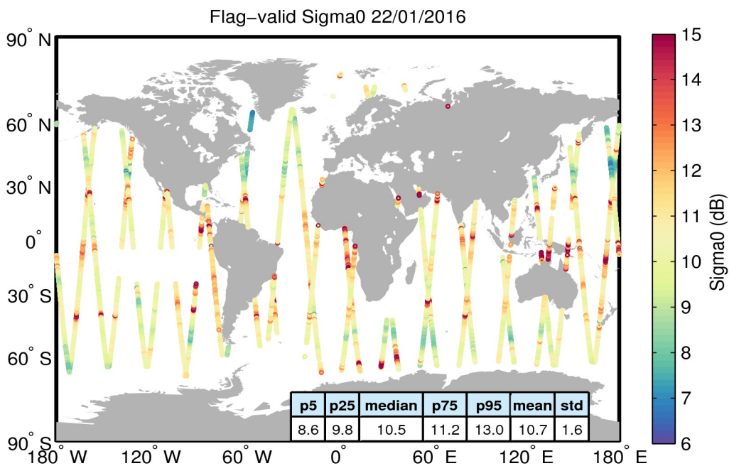
Figure 23. Geographical distribution of flag-valid sigma0 data over oceans and lakes for 22/01/2016. The statistical values shown in the table refer to the sigma0 in dB and are calculated over all measurements shown in the figure.
