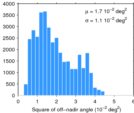
Figure 39. Histogram of flag-valid mispointing over oceans and lakes for 22/01/2016. The mean ( \mu ) and standard deviation ( \sigma ) are also shown. Note that values larger than 6 \cdot 10^{-2} \text{ deg}^2 are excluded from the histogram for the sake of readability but not from the computation of \mu and \sigma .
