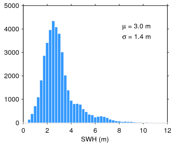
Figure 17. Histogram of flag-valid SWH over oceans and lakes for 21/01/2016. The mean ( \mu ) and standard deviation ( \sigma ) are also shown. Note that values larger than 12 m are excluded from the histogram for the sake of readability but not from the computation of \mu and \sigma .
