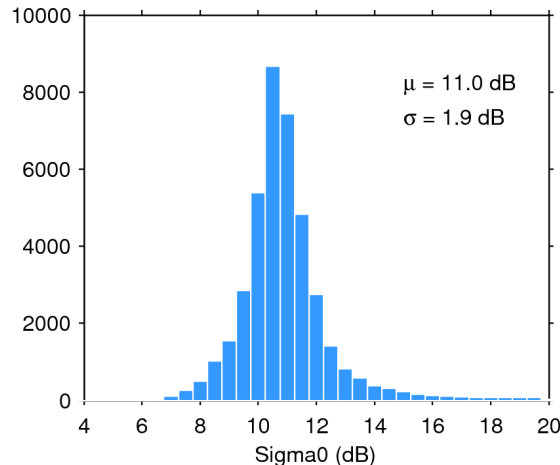
Figure 25. Histogram of flag-valid sigma0 over oceans and lakes for 21/01/2016. The mean ( \mu ) and standard deviation ( \sigma ) are also shown. Note that values outside [4 20] dB are excluded from the histogram for the sake of readability but not from the computation of \mu and \sigma .
