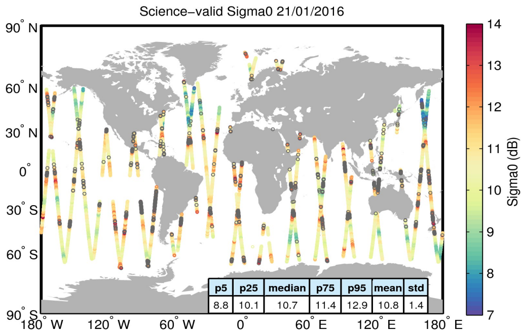
Figure 27. Geographical distribution of science-valid sigma0 data over oceans and lakes for 21/01/2016. The statistical values shown in the table refer to the sigma0 in dB and are calculated over all measurements shown in the figure. Gray circles denote records that have been rejected based on the editing criteria described in Table 4.
