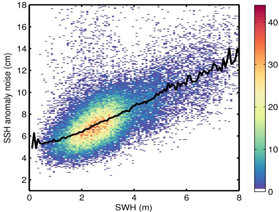
Figure 9. 2D histogram showing flag-valid SSH anomaly noise as a function of SWH for 21/01/2016. The black line denotes the median SSH anomaly noise as a function of SWH.
