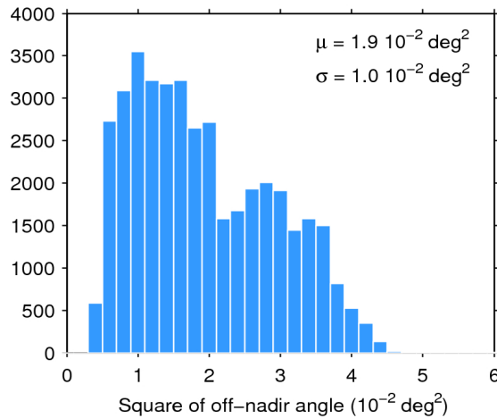
Figure 39. Histogram of flag-valid mispointing over oceans and lakes for 21/01/2016. The mean ( \mu ) and standard deviation ( \sigma ) are also shown. Note that values larger than 6 \cdot 10^{-2} \text{ deg}^2 are excluded from the histogram for the sake of readability but not from the computation of \mu and \sigma .
