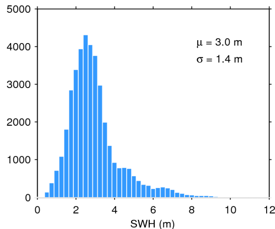
Figure 20. Histogram of science-valid SWH over oceans and lakes for 21/01/2016. The mean ( \mu ) and standard deviation ( \sigma ) are also shown. Note that values larger than 12 m are excluded from the histogram for the sake of readability but not from the computation of \mu and \sigma .
