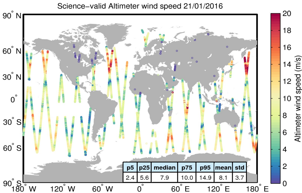
Figure 34. Geographical distribution of science-valid wind data over oceans and lakes for 21/01/2016. The statistical values shown in the table refer to the wind in m/s and are calculated over all measurements shown in the figure. Gray circles denote records that have been rejected based on the editing criteria described in Table 5.
