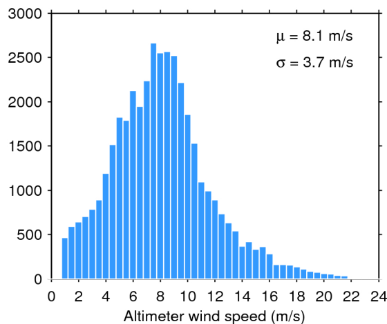
Figure 35. Histogram of science-valid wind over oceans and lakes for 21/01/2016. The mean ( \mu ) and standard deviation ( \sigma ) are also shown. Note that values larger than 24 m/s are excluded from the histogram for the sake of readability but not from the computation of \mu and \sigma .
