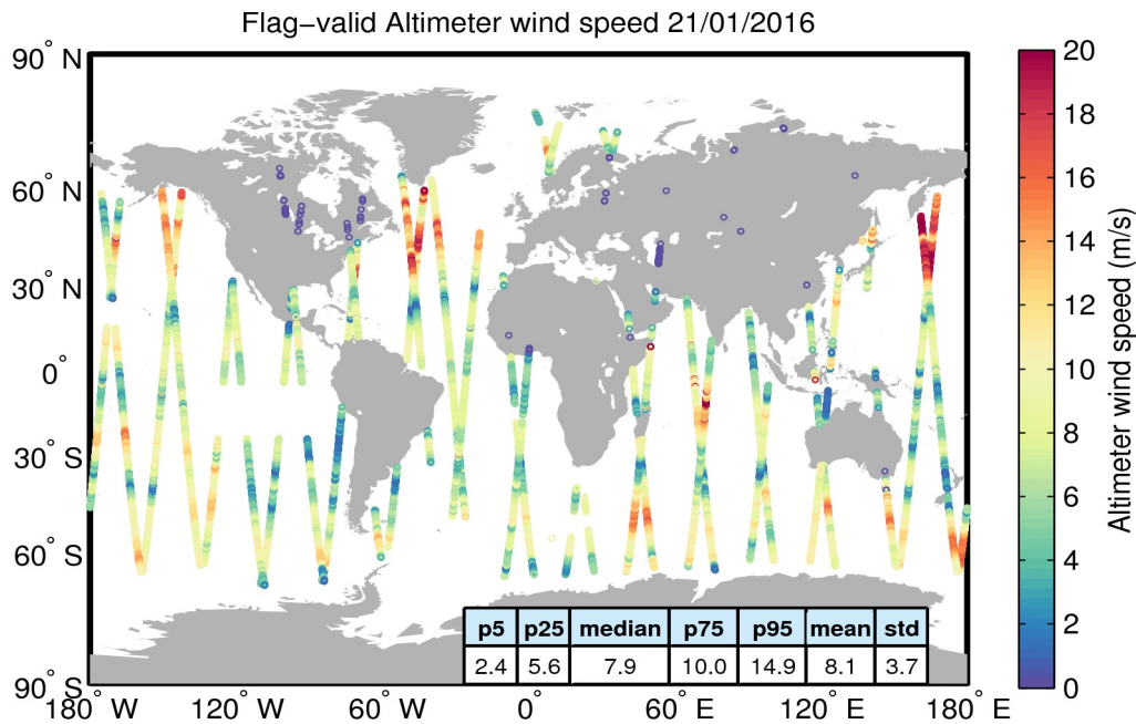
Figure 31. Geographical distribution of flag-valid wind data over oceans and lakes for 21/01/2016. The statistical values shown in the table refer to the wind in m/s and are calculated over all measurements shown in the figure.
