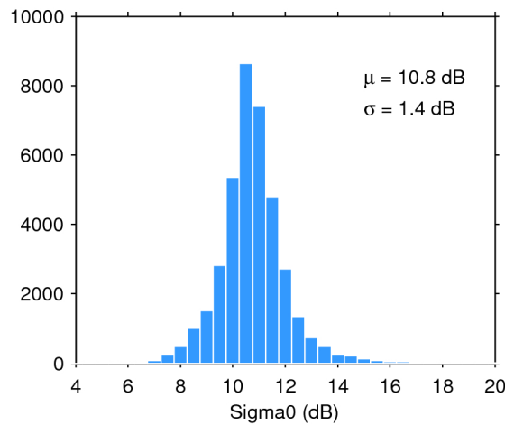
Figure 28. Histogram of science-valid sigma0 over oceans and lakes for 21/01/2016. The mean ( \mu ) and standard deviation ( \sigma ) are also shown. Note that values outside [4 20] dB are excluded from the histogram for the sake of readability but not from the computation of \mu and \sigma .
