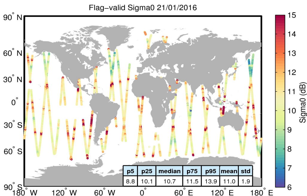
Figure 23. Geographical distribution of flag-valid sigma0 data over oceans and lakes for 21/01/2016. The statistical values shown in the table refer to the sigma0 in dB and are calculated over all measurements shown in the figure.
