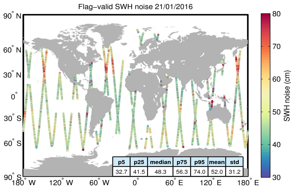
Figure 18. Geographical distribution of flag-valid 20-Hz SWH measurement noise over oceans and lakes for 21/01/2016. The statistical values shown in the figure refer to the SWH noise and are calculated over all measurements shown in the figure.
