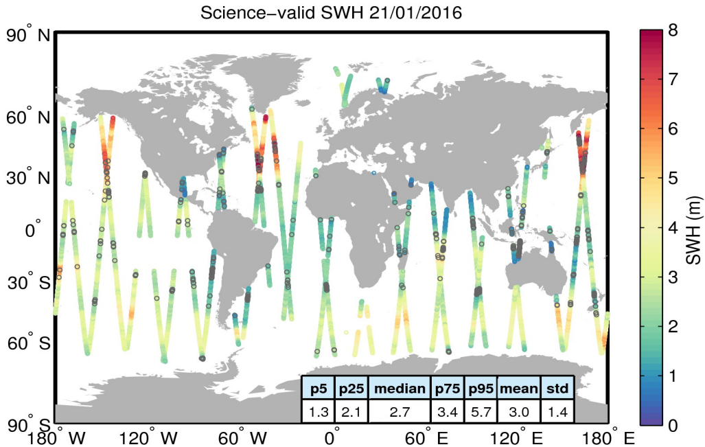
Figure 19. Geographical distribution of science-valid SWH data over oceans and lakes for 21/01/2016. The statistical values shown in the table refer to the SWH in m and are calculated over all measurements shown in the figure. Gray circles denote records that have been rejected based on the editing criteria described in Table 3.
