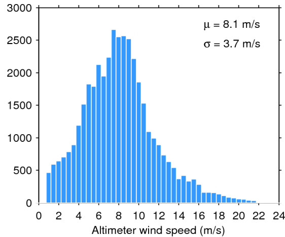
Figure 33. Histogram of flag-valid wind over oceans and lakes for 21/01/2016. The mean ( \mu ) and standard deviation ( \sigma ) are also shown. Note that values larger than 24 m/s are excluded from the histogram for the sake of readability but not from the computation of \mu and \sigma .
