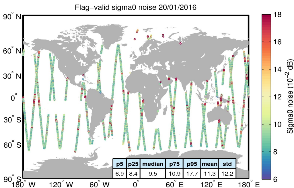
Figure 26. Geographical distribution of flag-valid 20-Hz sigma0 measurement noise over oceans and lakes for 20/01/2016. The statistical values shown in the table refer to the sigma0 noise and are calculated over all measurements shown in the figure.
