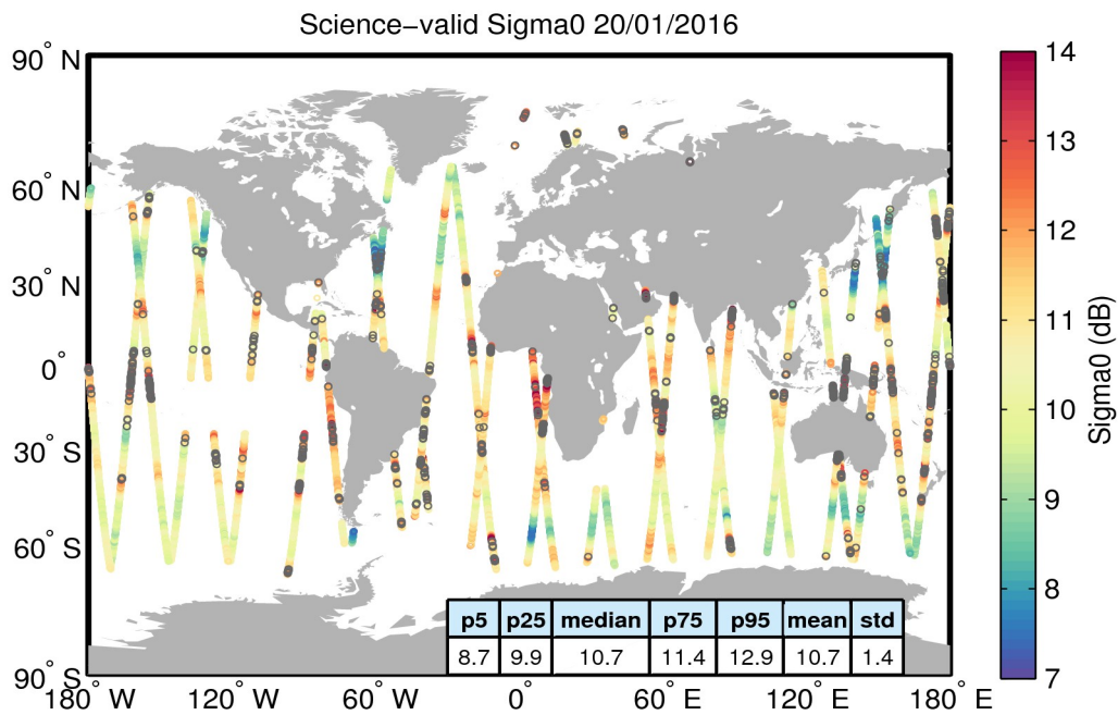
Figure 27. Geographical distribution of science-valid sigma0 data over oceans and lakes for 20/01/2016. The statistical values shown in the table refer to the sigma0 in dB and are calculated over all measurements shown in the figure. Gray circles denote records that have been rejected based on the editing criteria described in Table 4.
