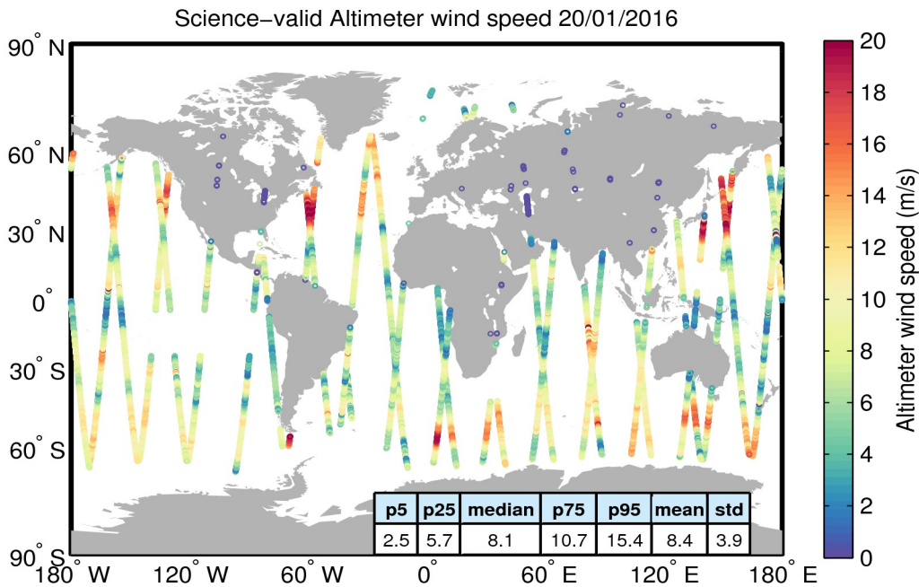
Figure 34. Geographical distribution of science-valid wind data over oceans and lakes for 20/01/2016. The statistical values shown in the table refer to the wind in m/s and are calculated over all measurements shown in the figure. Gray circles denote records that have been rejected based on the editing criteria described in Table 5.
