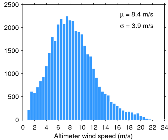
Figure 33. Histogram of flag-valid wind over oceans and lakes for 20/01/2016. The mean ( \mu ) and standard deviation ( \sigma ) are also shown. Note that values larger than 24 m/s are excluded from the histogram for the sake of readability but not from the computation of \mu and \sigma .
