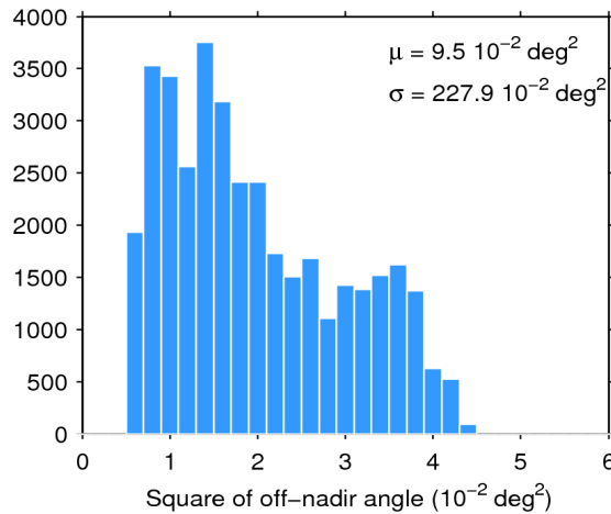
Figure 39. Histogram of flag-valid mispointing over oceans and lakes for 20/01/2016. The mean ( \mu ) and standard deviation ( \sigma ) are also shown. Note that values larger than 6 \cdot 10^{-2} \text{ deg}^2 are excluded from the histogram for the sake of readability but not from the computation of \mu and \sigma .
