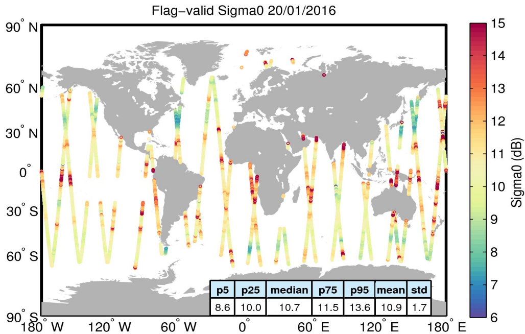
Figure 23. Geographical distribution of flag-valid sigma0 data over oceans and lakes for 20/01/2016. The statistical values shown in the table refer to the sigma0 in dB and are calculated over all measurements shown in the figure.
