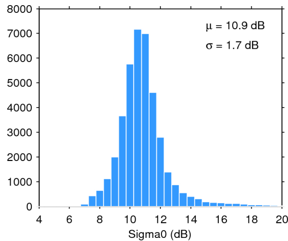
Figure 25. Histogram of flag-valid sigma0 over oceans and lakes for 20/01/2016. The mean ( \mu ) and standard deviation ( \sigma ) are also shown. Note that values outside [4 20] dB are excluded from the histogram for the sake of readability but not from the computation of \mu and \sigma .
