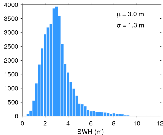
Figure 20. Histogram of science-valid SWH over oceans and lakes for 20/01/2016. The mean ( \mu ) and standard deviation ( \sigma ) are also shown. Note that values larger than 12 m are excluded from the histogram for the sake of readability but not from the computation of \mu and \sigma .
