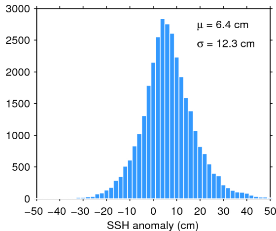
Figure 11. Histogram of science-valid SSH anomaly over oceans and lakes for 20/01/2016. The mean ( \mu ) and standard deviation ( \sigma ) are also shown. Note that values outside [-50 50] cm are excluded from the histogram for the sake of readability but not from the computation of \mu and \sigma .
