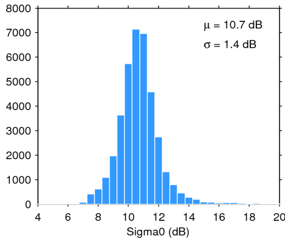
Figure 28. Histogram of science-valid sigma0 over oceans and lakes for 20/01/2016. The mean ( \mu ) and standard deviation ( \sigma ) are also shown. Note that values outside [4 20] dB are excluded from the histogram for the sake of readability but not from the computation of \mu and \sigma .
