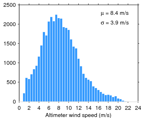
Figure 35. Histogram of science-valid wind over oceans and lakes for 20/01/2016. The mean ( \mu ) and standard deviation ( \sigma ) are also shown. Note that values larger than 24 m/s are excluded from the histogram for the sake of readability but not from the computation of \mu and \sigma .
