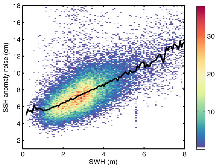
Figure 9. 2D histogram showing flag-valid SSH anomaly noise as a function of SWH for 20/01/2016. The black line denotes the median SSH anomaly noise as a function of SWH.
