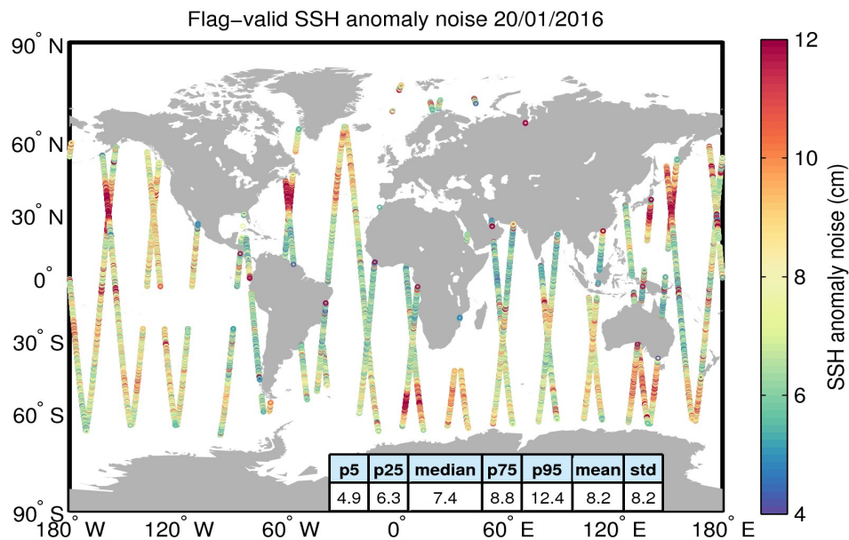
Figure 8. Geographical distribution of flag-valid 20-Hz SSH anomaly measurement noise over oceans and lakes for 20/01/2016. The statistical values shown in the table refer to the SSH anomaly noise and are calculated over all measurements shown in the figure.
