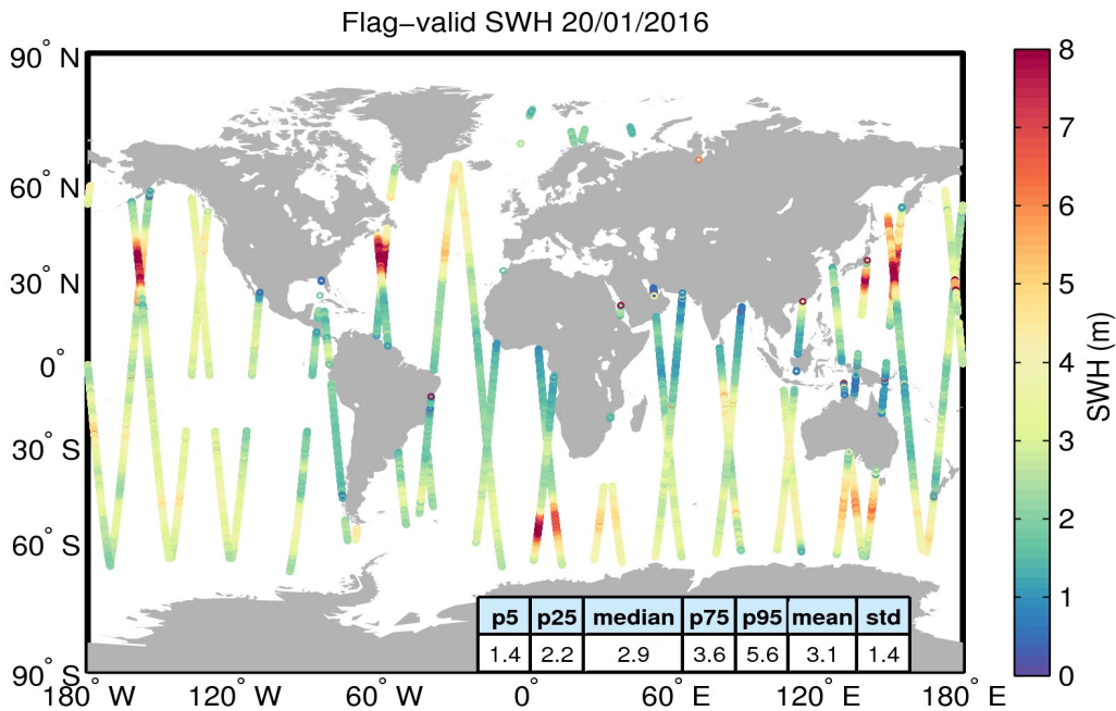
Figure 15. Geographical distribution of flag-valid SWH data over oceans and lakes for 20/01/2016. The statistical values shown in the table refer to the SWH in m and are calculated over all measurements shown in the figure.
