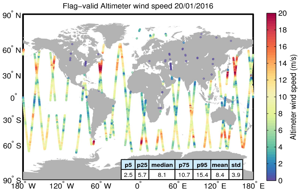
Figure 31. Geographical distribution of flag-valid wind data over oceans and lakes for 20/01/2016. The statistical values shown in the table refer to the wind in m/s and are calculated over all measurements shown in the figure.
