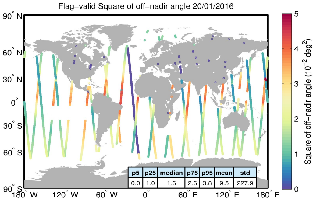
Figure 37. Geographical distribution of flag-valid mispointing data over oceans and lakes for 20/01/2016. The statistical values shown in the table refer to the mispointing in 10^{-2} deg 2 and are calculated over all measurements shown in the figure.
