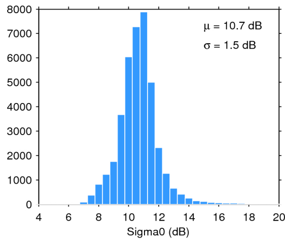
Figure 28. Histogram of science-valid sigma0 over oceans and lakes for 18/01/2016. The mean ( \mu ) and standard deviation ( \sigma ) are also shown. Note that values outside [4 20] dB are excluded from the histogram for the sake of readability but not from the computation of \mu and \sigma .
