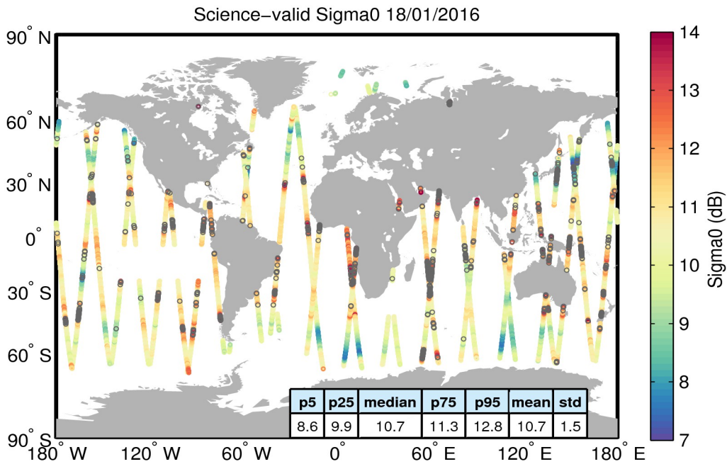
Figure 27. Geographical distribution of science-valid sigma0 data over oceans and lakes for 18/01/2016. The statistical values shown in the table refer to the sigma0 in dB and are calculated over all measurements shown in the figure. Gray circles denote records that have been rejected based on the editing criteria described in Table 4.
