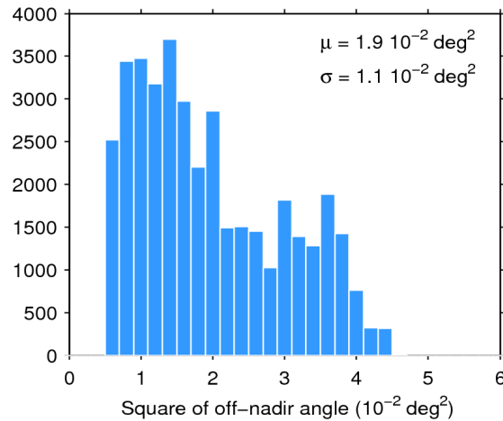
Figure 39. Histogram of flag-valid mispointing over oceans and lakes for 18/01/2016. The mean ( \mu ) and standard deviation ( \sigma ) are also shown. Note that values larger than 6 \cdot 10^{-2} \text{ deg}^2 are excluded from the histogram for the sake of readability but not from the computation of \mu and \sigma .
