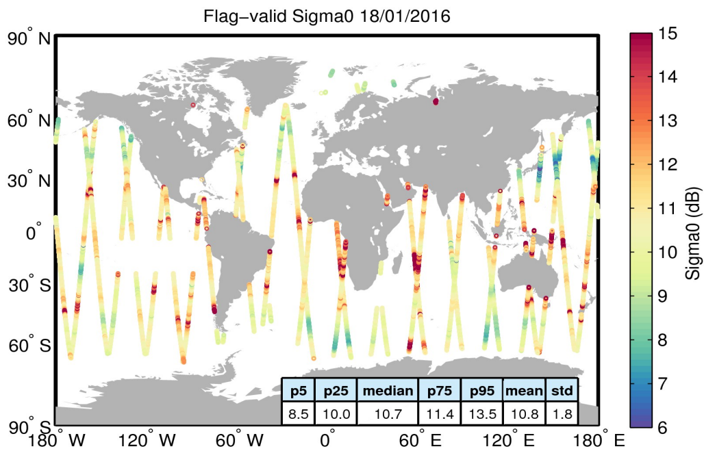
Figure 23. Geographical distribution of flag-valid sigma0 data over oceans and lakes for 18/01/2016. The statistical values shown in the table refer to the sigma0 in dB and are calculated over all measurements shown in the figure.
