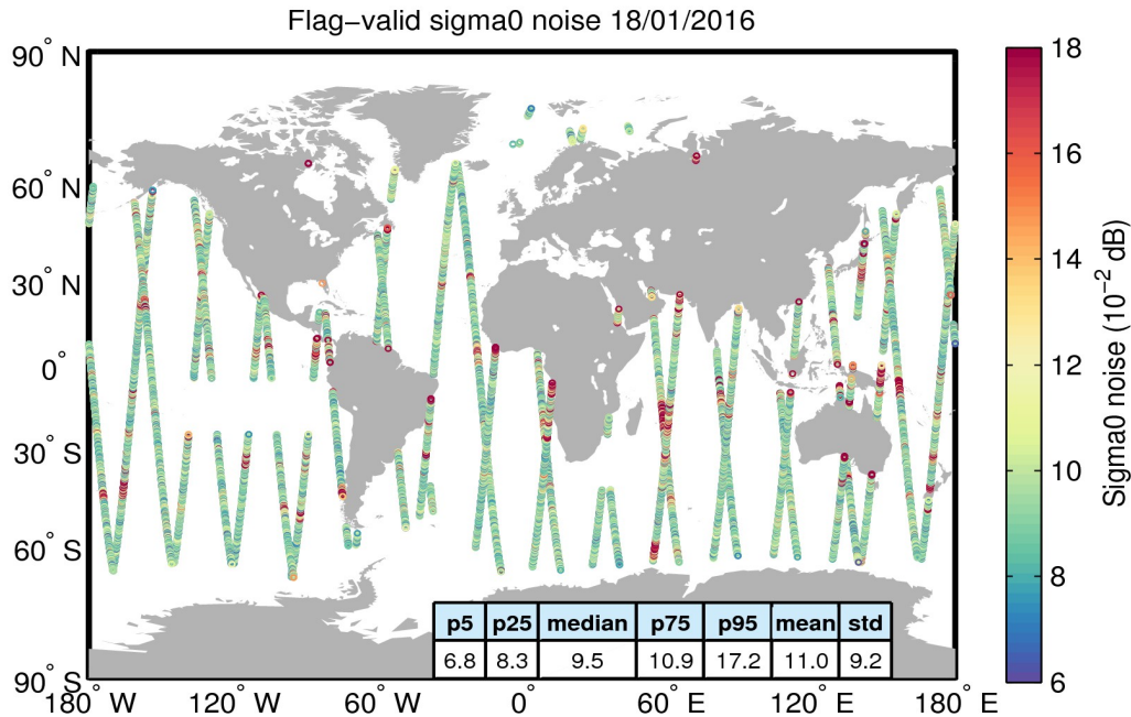
Figure 26. Geographical distribution of flag-valid 20-Hz sigma0 measurement noise over oceans and lakes for 18/01/2016. The statistical values shown in the table refer to the sigma0 noise and are calculated over all measurements shown in the figure.
