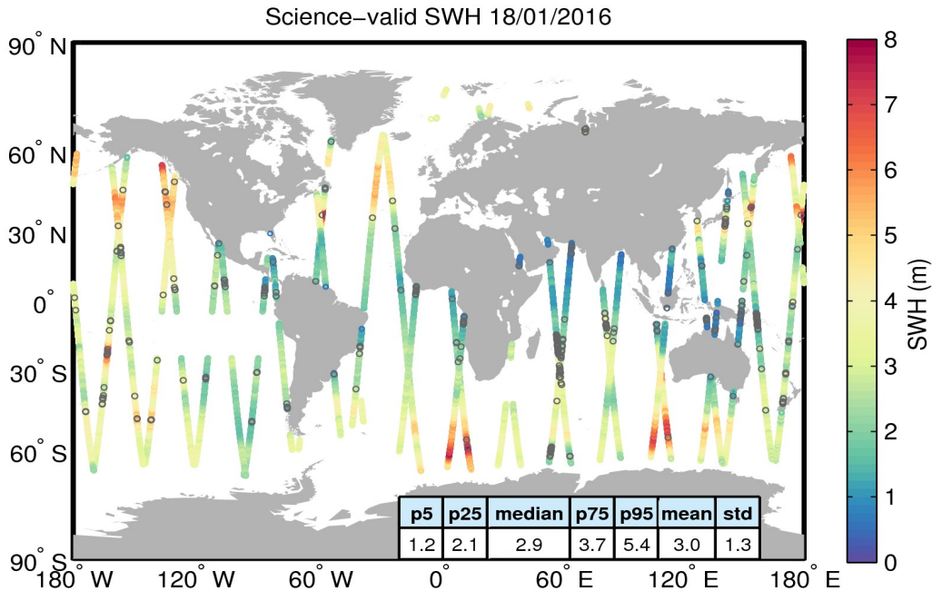
Figure 19. Geographical distribution of science-valid SWH data over oceans and lakes for 18/01/2016. The statistical values shown in the table refer to the SWH in m and are calculated over all measurements shown in the figure. Gray circles denote records that have been rejected based on the editing criteria described in Table 3.
