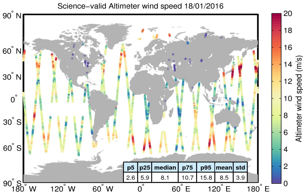
Figure 34. Geographical distribution of science-valid wind data over oceans and lakes for 18/01/2016. The statistical values shown in the table refer to the wind in m/s and are calculated over all measurements shown in the figure. Gray circles denote records that have been rejected based on the editing criteria described in Table 5.
