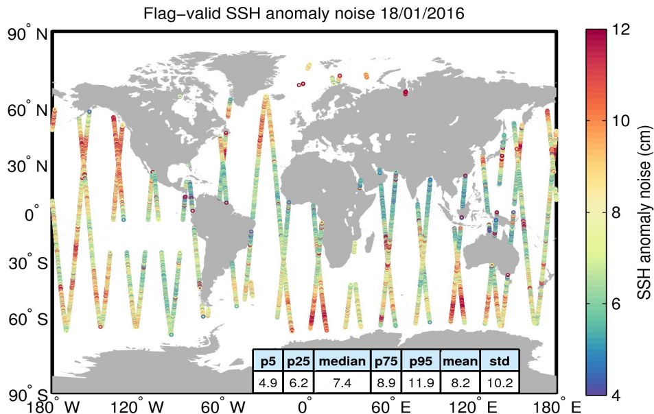
Figure 8. Geographical distribution of flag-valid 20-Hz SSH anomaly measurement noise over oceans and lakes for 18/01/2016. The statistical values shown in the table refer to the SSH anomaly noise and are calculated over all measurements shown in the figure.
