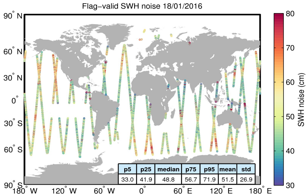
Figure 18. Geographical distribution of flag-valid 20-Hz SWH measurement noise over oceans and lakes for 18/01/2016. The statistical values shown in the table refer to the SWH noise and are calculated over all measurements shown in the figure.
