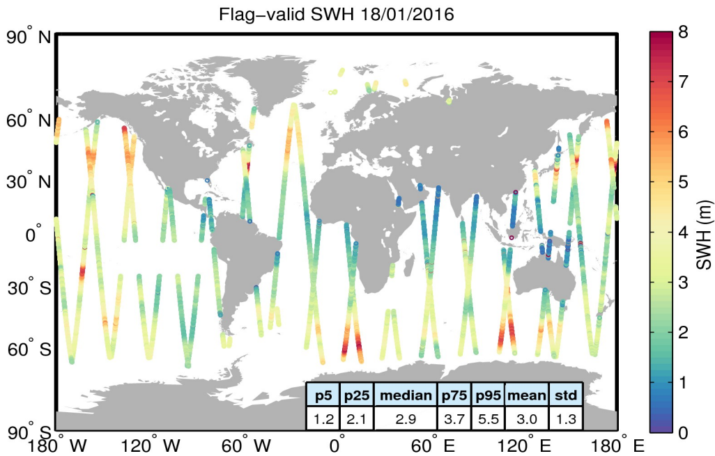
Figure 15. Geographical distribution of flag-valid SWH data over oceans and lakes for 18/01/2016. The statistical values shown in the table refer to the SWH in m and are calculated over all measurements shown in the figure.
