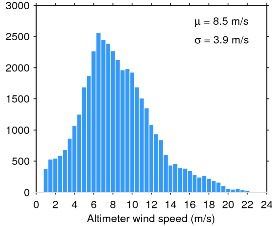
Figure 33. Histogram of flag-valid wind over oceans and lakes for 18/01/2016. The mean ( \mu ) and standard deviation ( \sigma ) are also shown. Note that values larger than 24 m/s are excluded from the histogram for the sake of readability but not from the computation of \mu and \sigma .
