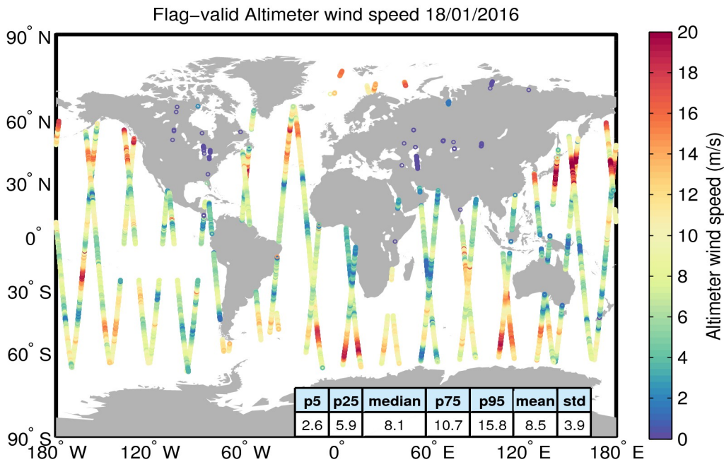
Figure 31. Geographical distribution of flag-valid wind data over oceans and lakes for 18/01/2016. The statistical values shown in the table refer to the wind in m/s and are calculated over all measurements shown in the figure.
