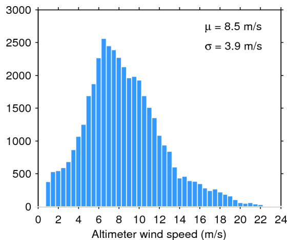
Figure 35. Histogram of science-valid wind over oceans and lakes for 18/01/2016. The mean ( \mu ) and standard deviation ( \sigma ) are also shown. Note that values larger than 24 m/s are excluded from the histogram for the sake of readability but not from the computation of \mu and \sigma .
