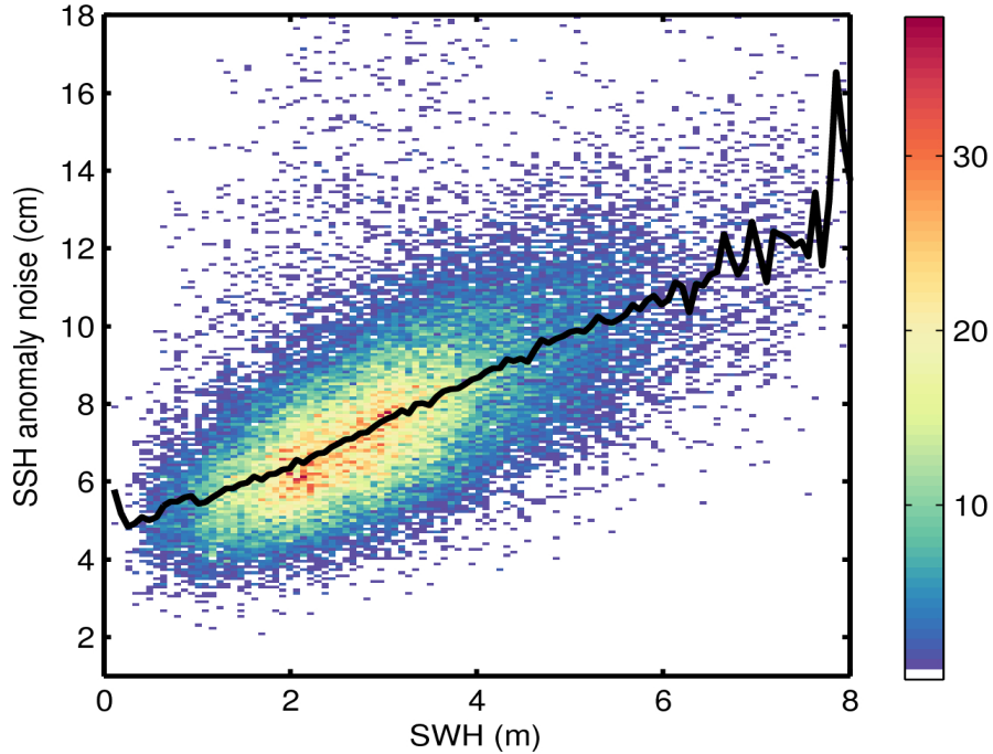
Figure 9. 2D histogram showing flag-valid SSH anomaly noise as a function of SWH for 18/01/2016. The black line denotes the median SSH anomaly noise as a function of SWH.
