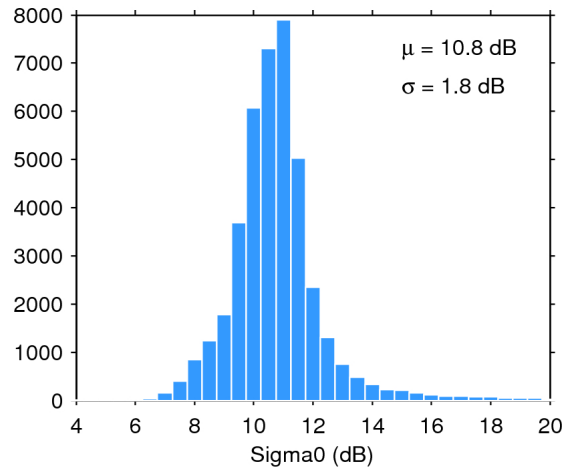
Figure 25. Histogram of flag-valid sigma0 over oceans and lakes for 18/01/2016. The mean ( \mu ) and standard deviation ( \sigma ) are also shown. Note that values outside [4 20] dB are excluded from the histogram for the sake of readability but not from the computation of \mu and \sigma .
