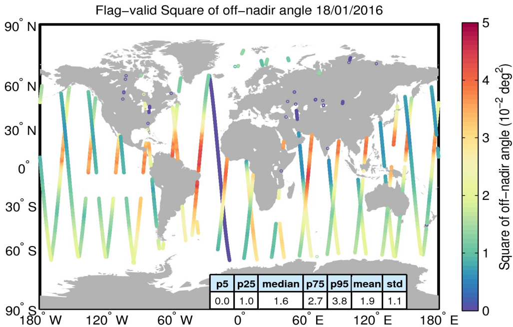
Figure 37. Geographical distribution of flag-valid mispointing data over oceans and lakes for 18/01/2016. The statistical values shown in the table refer to the mispointing in 10^{-2} \text{ deg}^2 and are calculated over all measurements shown in the figure.
