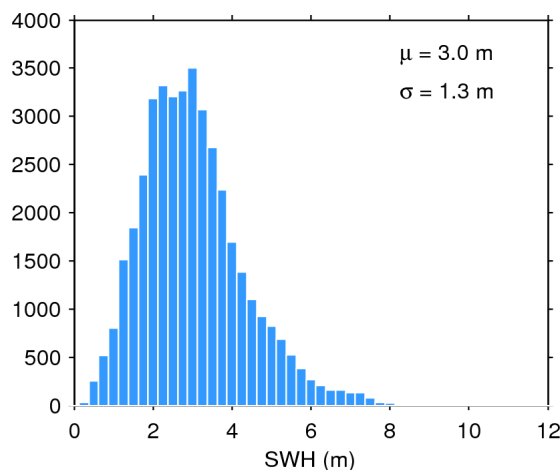
Figure 20. Histogram of science-valid SWH over oceans and lakes for 18/01/2016. The mean ( \mu ) and standard deviation ( \sigma ) are also shown. Note that values larger than 12 m are excluded from the histogram for the sake of readability but not from the computation of \mu and \sigma .
