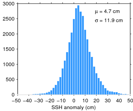
Figure 11. Histogram of science-valid SSH anomaly over oceans and lakes for 18/01/2016. The mean ( \mu ) and standard deviation ( \sigma ) are also shown. Note that values outside [-50 50] cm are excluded from the histogram for the sake of readability but not from the computation of \mu and \sigma .
