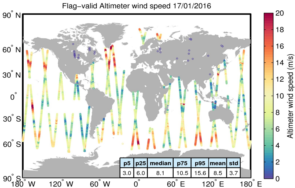
Figure 31. Geographical distribution of flag-valid wind data over oceans and lakes for 17/01/2016. The statistical values shown in the table refer to the wind in m/s and are calculated over all measurements shown in the figure.
