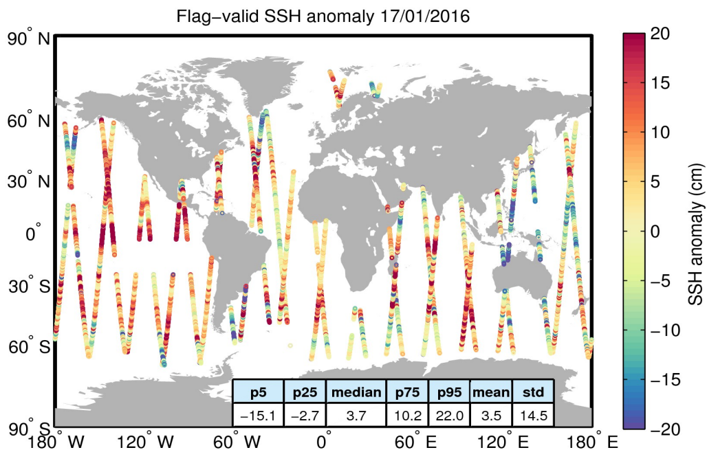
Figure 5. Geographical distribution of flag-valid 1-Hz SSH anomaly data over oceans and lakes for 17/01/2016. The statistical values shown in the table refer to the SSH anomaly in cm and are calculated over all measurements shown in the figure.
