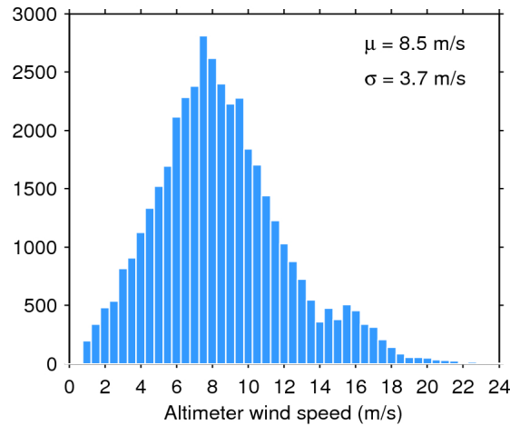
Figure 33. Histogram of flag-valid wind over oceans and lakes for 17/01/2016. The mean ( \mu ) and standard deviation ( \sigma ) are also shown. Note that values larger than 24 m/s are excluded from the histogram for the sake of readability but not from the computation of \mu and \sigma .
