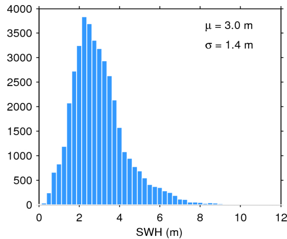
Figure 17. Histogram of flag-valid SWH over oceans and lakes for 17/01/2016. The mean ( \mu ) and standard deviation ( \sigma ) are also shown. Note that values larger than 12 m are excluded from the histogram for the sake of readability but not from the computation of \mu and \sigma .
