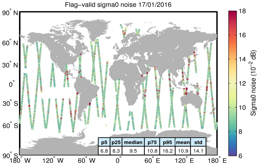
Figure 26. Geographical distribution of flag-valid 20-Hz sigma0 measurement noise over oceans and lakes for 17/01/2016. The statistical values shown in the table refer to the sigma0 noise and are calculated over all measurements shown in the figure.
