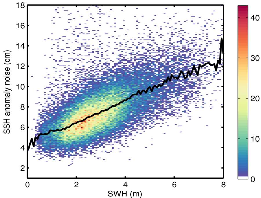
Figure 9. 2D histogram showing flag-valid SSH anomaly noise as a function of SWH for 17/01/2016. The black line denotes the median SSH anomaly noise as a function of SWH.
