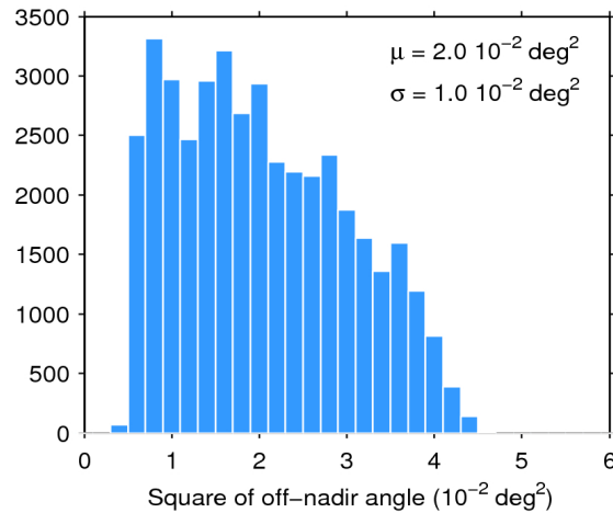
Figure 39. Histogram of flag-valid mispointing over oceans and lakes for 17/01/2016. The mean ( \mu ) and standard deviation ( \sigma ) are also shown. Note that values larger than 6 \cdot 10^{-2} \text{ deg}^2 are excluded from the histogram for the sake of readability but not from the computation of \mu and \sigma .
