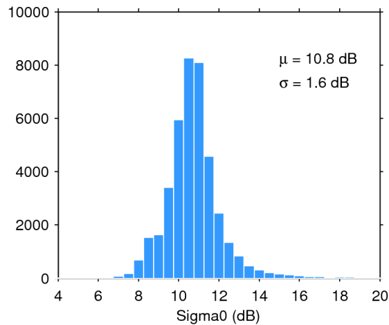
Figure 25. Histogram of flag-valid sigma0 over oceans and lakes for 17/01/2016. The mean ( \mu ) and standard deviation ( \sigma ) are also shown. Note that values outside [4 20] dB are excluded from the histogram for the sake of readability but not from the computation of \mu and \sigma .
