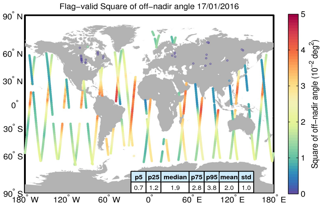
Figure 37. Geographical distribution of flag-valid mispointing data over oceans and lakes for 17/01/2016. The statistical values shown in the table refer to the mispointing in 10^{-2} deg 2 and are calculated over all measurements shown in the figure.
