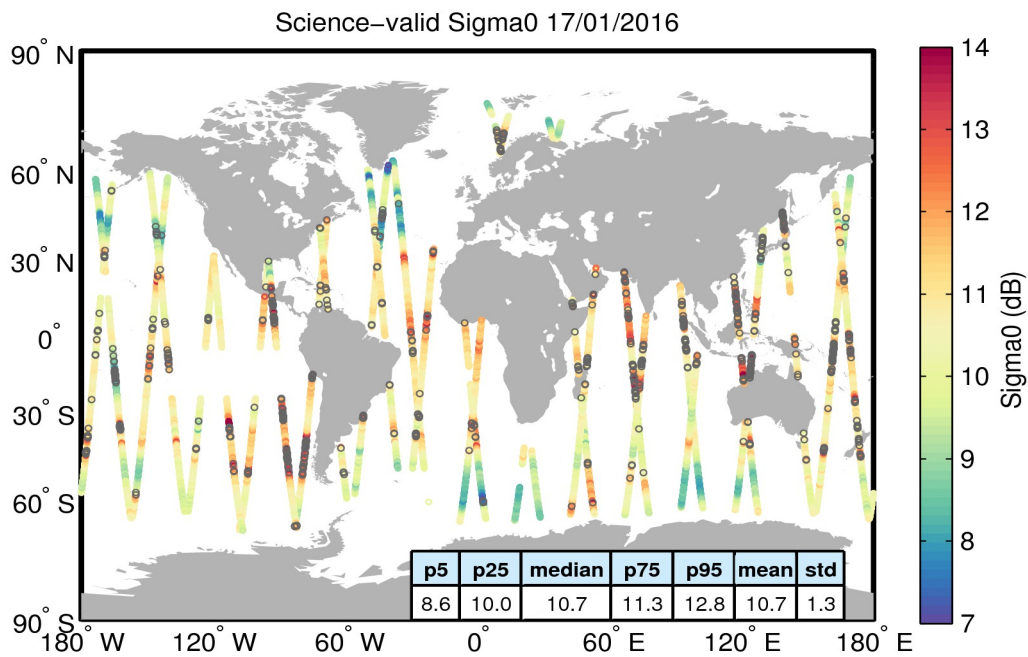
Figure 27. Geographical distribution of science-valid sigma0 data over oceans and lakes for 17/01/2016. The statistical values shown in the table refer to the sigma0 in dB and are calculated over all measurements shown in the figure. Gray circles denote records that have been rejected based on the editing criteria described in Table 4.
