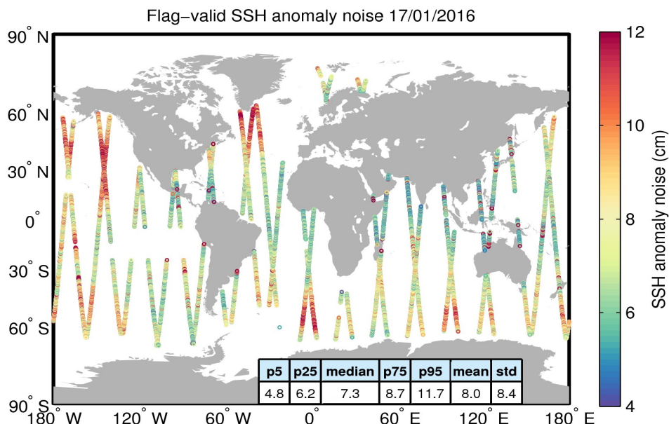
Figure 8. Geographical distribution of flag-valid 20-Hz SSH anomaly measurement noise over oceans and lakes for 17/01/2016. The statistical values shown in the table refer to the SSH anomaly noise and are calculated over all measurements shown in the figure.
