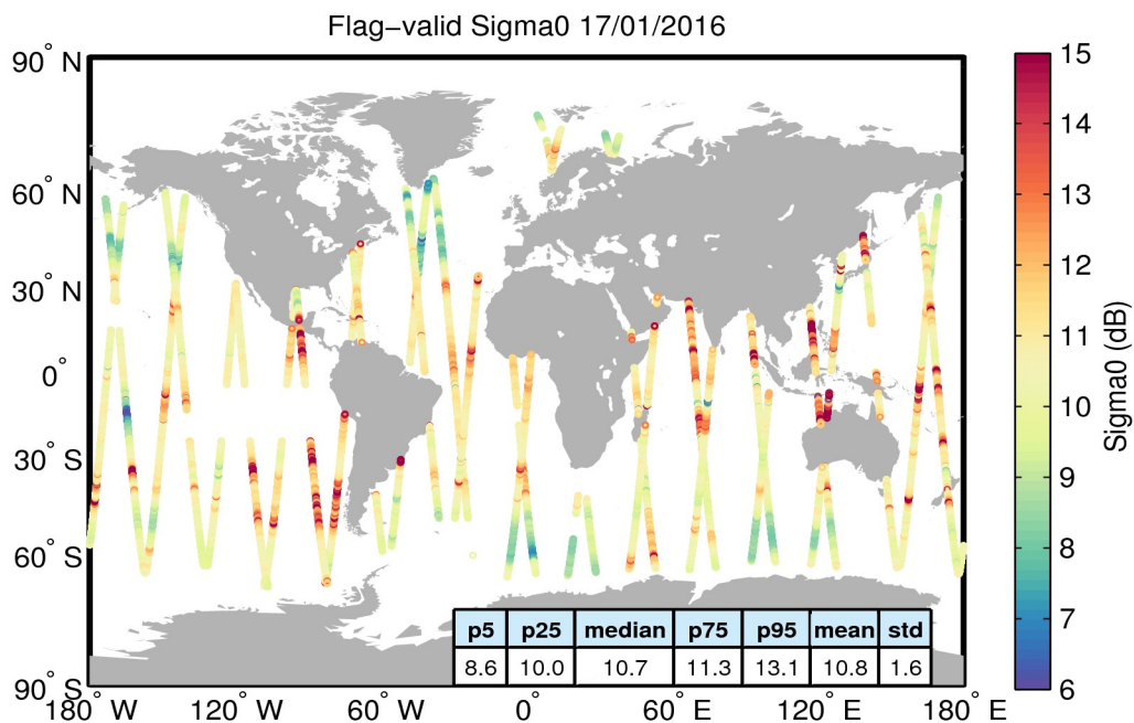
Figure 23. Geographical distribution of flag-valid sigma0 data over oceans and lakes for 17/01/2016. The statistical values shown in the table refer to the sigma0 in dB and are calculated over all measurements shown in the figure.
