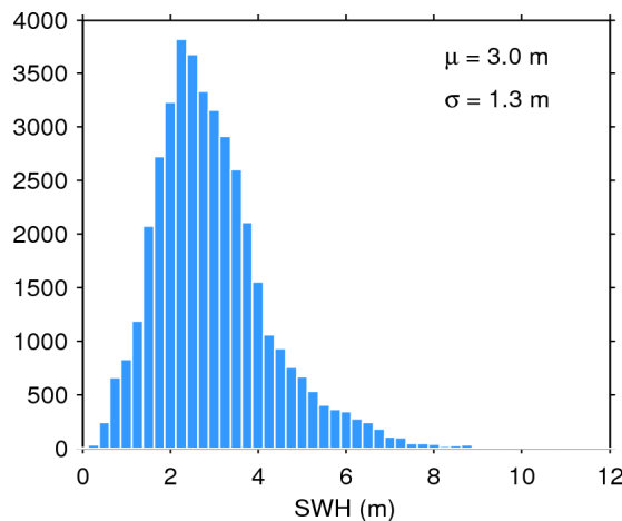
Figure 20. Histogram of science-valid SWH over oceans and lakes for 17/01/2016. The mean ( \mu ) and standard deviation ( \sigma ) are also shown. Note that values larger than 12 m are excluded from the histogram for the sake of readability but not from the computation of \mu and \sigma .
