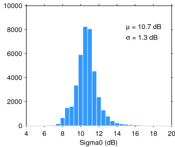
Figure 28. Histogram of science-valid sigma0 over oceans and lakes for 17/01/2016. The mean ( \mu ) and standard deviation ( \sigma ) are also shown. Note that values outside [4 20] dB are excluded from the histogram for the sake of readability but not from the computation of \mu and \sigma .
