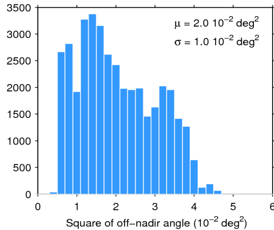
Figure 39. Histogram of flag-valid mispointing over oceans and lakes for 15/01/2016. The mean ( \mu ) and standard deviation ( \sigma ) are also shown. Note that values larger than 6 \cdot 10^{-2} \text{ deg}^2 are excluded from the histogram for the sake of readability but not from the computation of \mu and \sigma .
