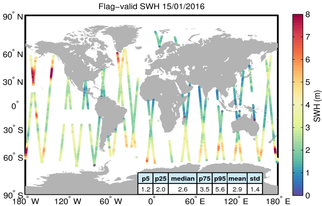
Figure 15. Geographical distribution of flag-valid SWH data over oceans and lakes for 15/01/2016. The statistical values shown in the table refer to the SWH in m and are calculated over all measurements shown in the figure.
