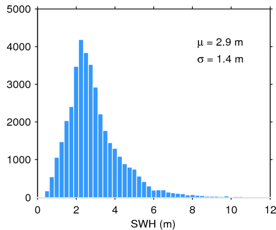
Figure 17. Histogram of flag-valid SWH over oceans and lakes for 15/01/2016. The mean ( \mu ) and standard deviation ( \sigma ) are also shown. Note that values larger than 12 m are excluded from the histogram for the sake of readability but not from the computation of \mu and \sigma .
