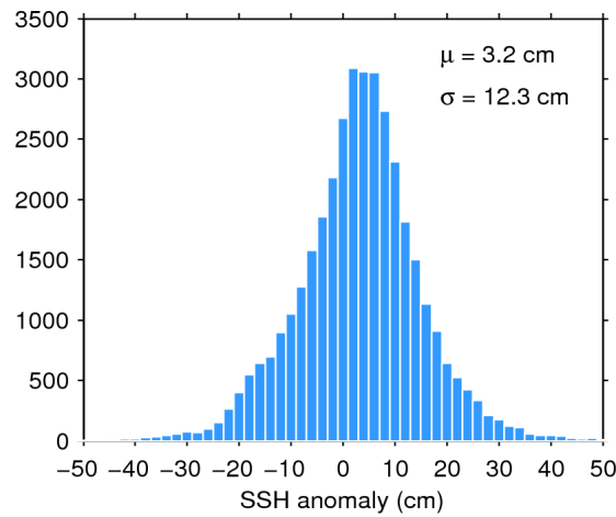
Figure 11. Histogram of science-valid SSH anomaly over oceans and lakes for 15/01/2016. The mean ( \mu ) and standard deviation ( \sigma ) are also shown. Note that values outside [-50 50] cm are excluded from the histogram for the sake of readability but not from the computation of \mu and \sigma .
