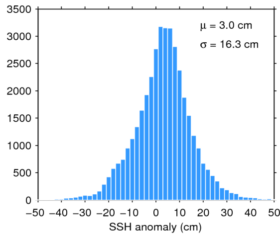
Figure 7. Histogram of flag-valid SSH anomaly over oceans and lakes for 15/01/2016. The mean ( \mu ) and standard deviation ( \sigma ) are also shown. Note that values outside [-50\ 50] cm are excluded from the histogram for the sake of readability but not from the computation of \mu and \sigma .
