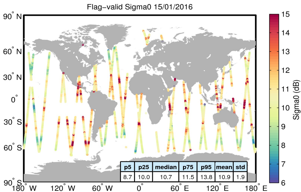
Figure 23. Geographical distribution of flag-valid sigma0 data over oceans and lakes for 15/01/2016. The statistical values shown in the table refer to the sigma0 in dB and are calculated over all measurements shown in the figure.
