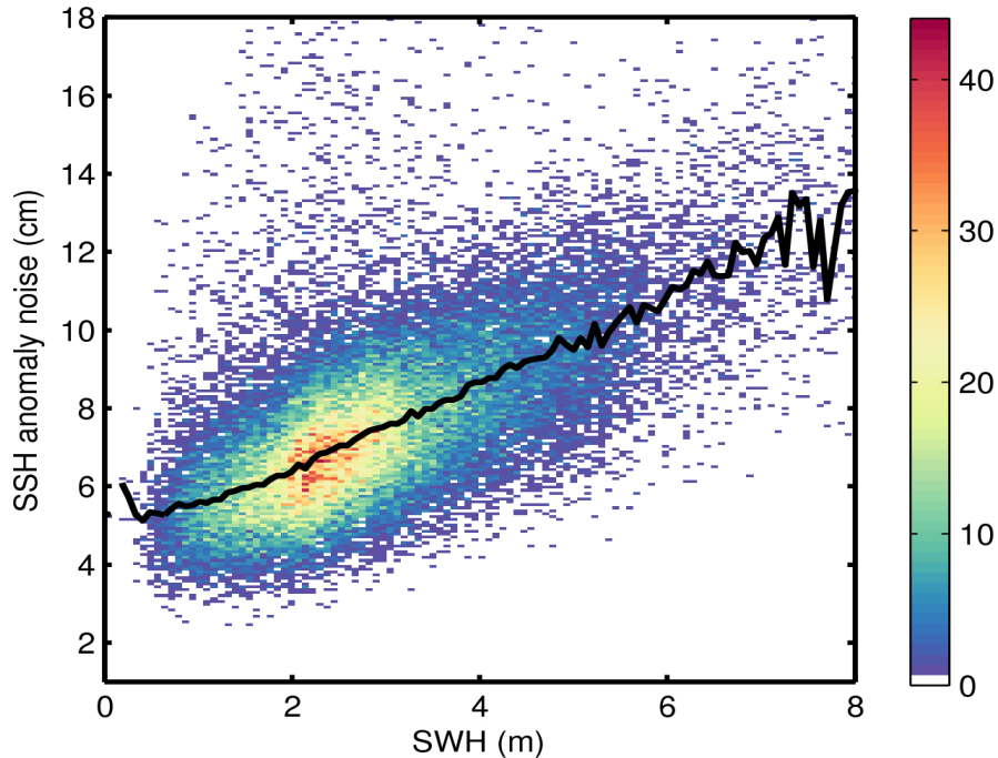
Figure 9. 2D histogram showing flag-valid SSH anomaly noise as a function of SWH for 15/01/2016. The black line denotes the median SSH anomaly noise as a function of SWH.
