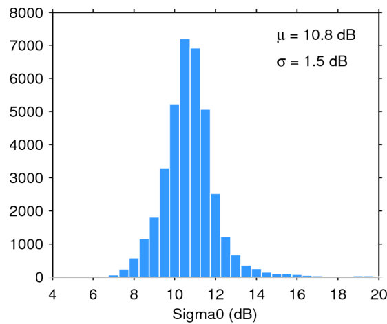
Figure 28. Histogram of science-valid sigma0 over oceans and lakes for 15/01/2016. The mean ( \mu ) and standard deviation ( \sigma ) are also shown. Note that values outside [4 20] dB are excluded from the histogram for the sake of readability but not from the computation of \mu and \sigma .
