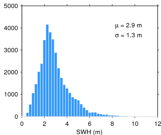
Figure 20. Histogram of science-valid SWH over oceans and lakes for 15/01/2016. The mean ( \mu ) and standard deviation ( \sigma ) are also shown. Note that values larger than 12 m are excluded from the histogram for the sake of readability but not from the computation of \mu and \sigma .
