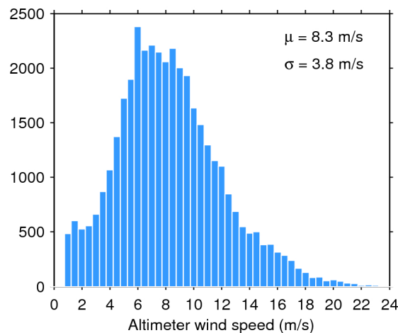
Figure 35. Histogram of science-valid wind over oceans and lakes for 15/01/2016. The mean ( \mu ) and standard deviation ( \sigma ) are also shown. Note that values larger than 24 m/s are excluded from the histogram for the sake of readability but not from the computation of \mu and \sigma .
