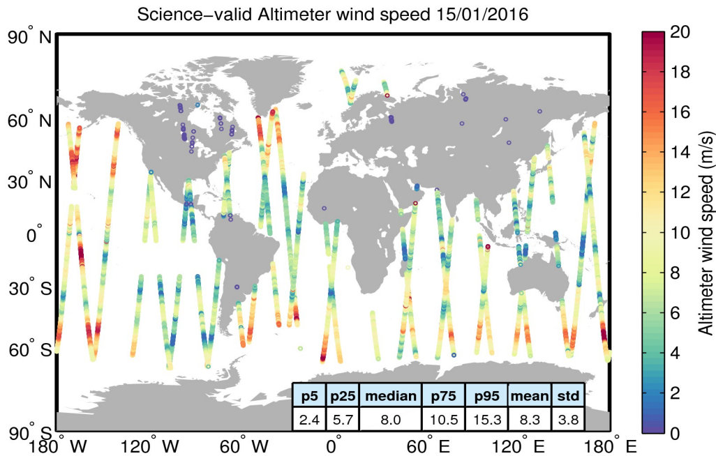
Figure 34. Geographical distribution of science-valid wind data over oceans and lakes for 15/01/2016. The statistical values shown in the table refer to the wind in m/s and are calculated over all measurements shown in the figure. Gray circles denote records that have been rejected based on the editing criteria described in Table 5.
