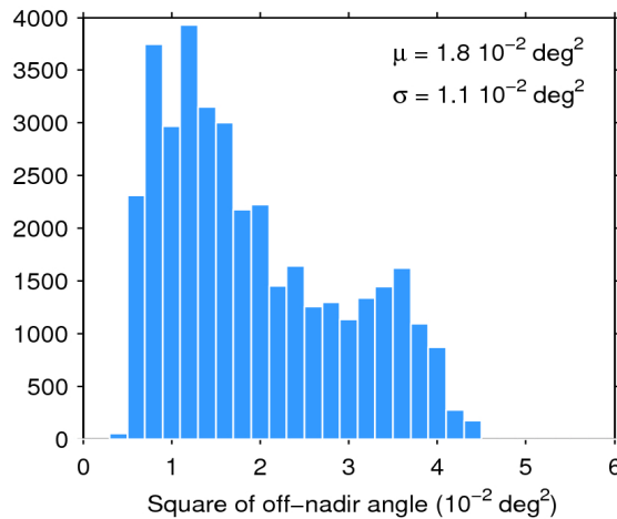
Figure 39. Histogram of flag-valid mispointing over oceans and lakes for 14/01/2016. The mean ( \mu ) and standard deviation ( \sigma ) are also shown. Note that values larger than 6 \cdot 10^{-2} \text{ deg}^2 are excluded from the histogram for the sake of readability but not from the computation of \mu and \sigma .
