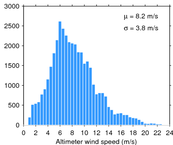
Figure 35. Histogram of science-valid wind over oceans and lakes for 14/01/2016. The mean ( \mu ) and standard deviation ( \sigma ) are also shown. Note that values larger than 24 m/s are excluded from the histogram for the sake of readability but not from the computation of \mu and \sigma .
