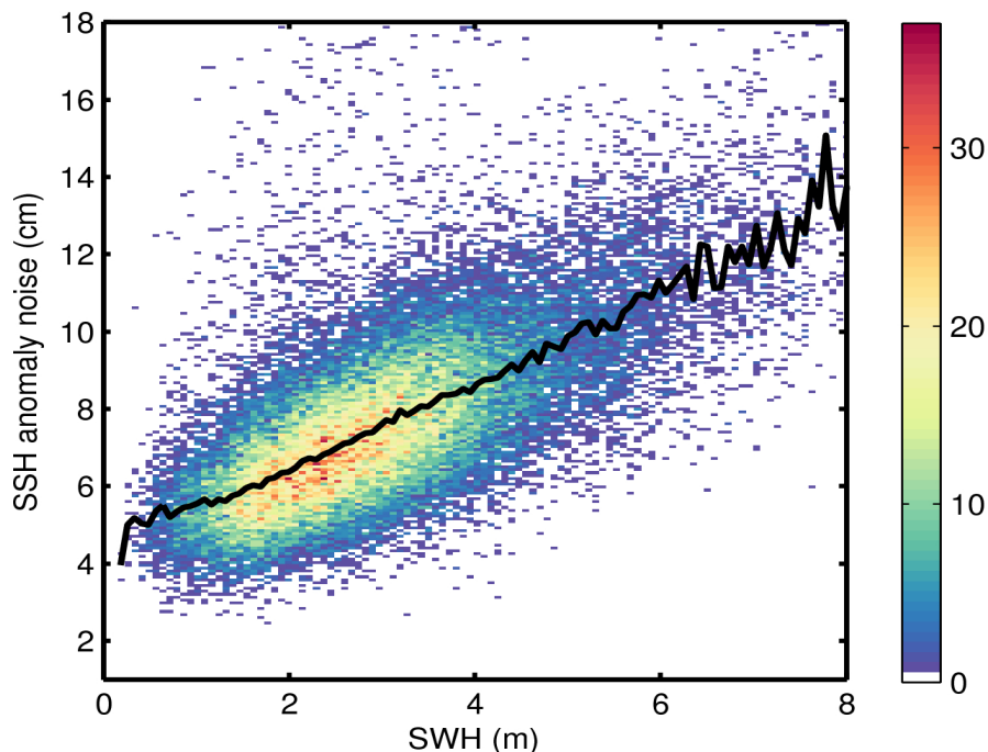
Figure 9. 2D histogram showing flag-valid SSH anomaly noise as a function of SWH for 14/01/2016. The black line denotes the median SSH anomaly noise as a function of SWH.
