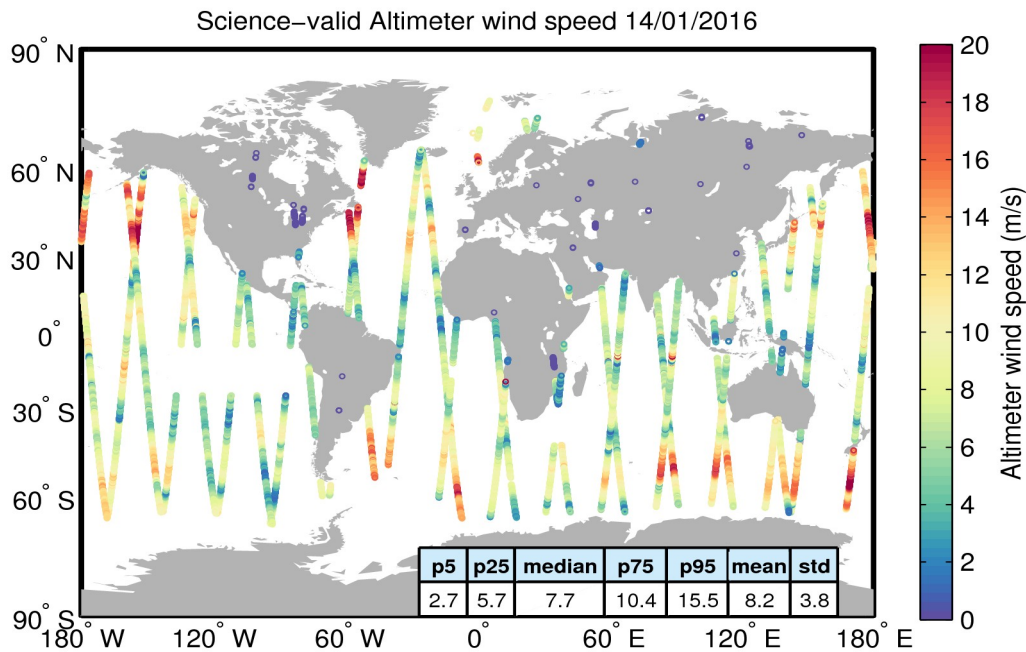
Figure 34. Geographical distribution of science-valid wind data over oceans and lakes for 14/01/2016. The statistical values shown in the table refer to the wind in m/s and are calculated over all measurements shown in the figure. Gray circles denote records that have been rejected based on the editing criteria described in Table 5.
