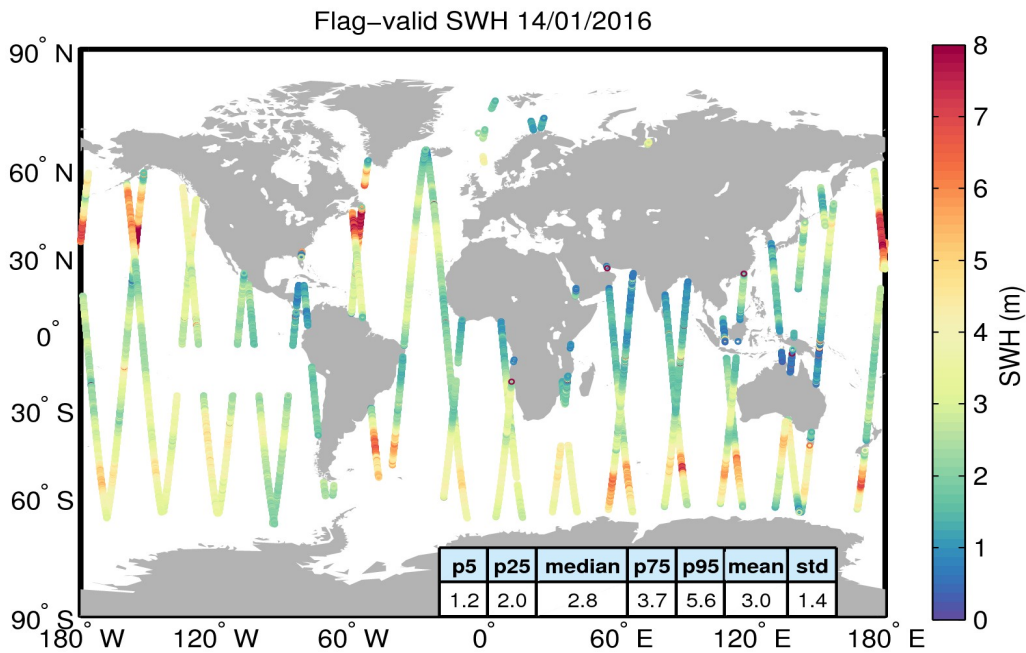
Figure 15. Geographical distribution of flag-valid SWH data over oceans and lakes for 14/01/2016. The statistical values shown in the table refer to the SWH in m and are calculated over all measurements shown in the figure.
