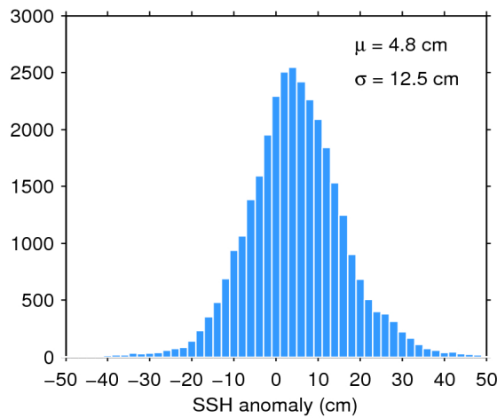
Figure 11. Histogram of science-valid SSH anomaly over oceans and lakes for 14/01/2016. The mean ( \mu ) and standard deviation ( \sigma ) are also shown. Note that values outside [-50 50] cm are excluded from the histogram for the sake of readability but not from the computation of \mu and \sigma .
