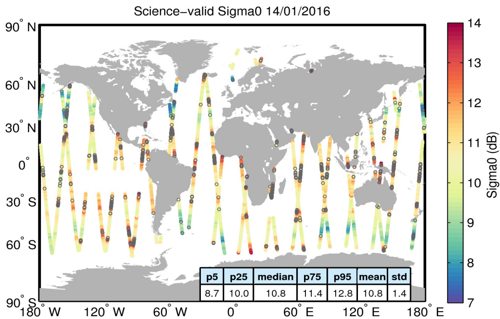
Figure 27. Geographical distribution of science-valid sigma0 data over oceans and lakes for 14/01/2016. The statistical values shown in the table refer to the sigma0 in dB and are calculated over all measurements shown in the figure. Gray circles denote records that have been rejected based on the editing criteria described in Table 4.
