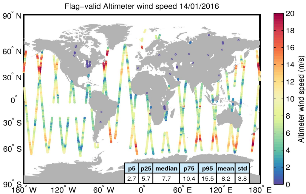
Figure 31. Geographical distribution of flag-valid wind data over oceans and lakes for 14/01/2016. The statistical values shown in the table refer to the wind in m/s and are calculated over all measurements shown in the figure.
