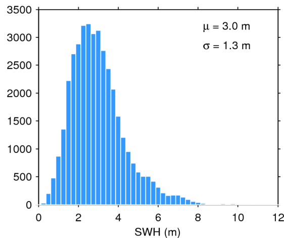
Figure 20. Histogram of science-valid SWH over oceans and lakes for 14/01/2016. The mean ( \mu ) and standard deviation ( \sigma ) are also shown. Note that values larger than 12 m are excluded from the histogram for the sake of readability but not from the computation of \mu and \sigma .
