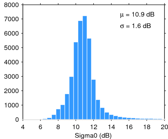
Figure 25. Histogram of flag-valid sigma0 over oceans and lakes for 14/01/2016. The mean ( \mu ) and standard deviation ( \sigma ) are also shown. Note that values outside [4 20] dB are excluded from the histogram for the sake of readability but not from the computation of \mu and \sigma .
