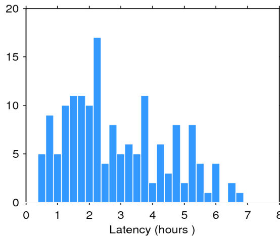
Figure 2. Histogram of the data latency for 14/01/2016. The y-axis denotes the number of files that are made available with a delay of x-hours with respect to the mean time of the records stored in the file.
