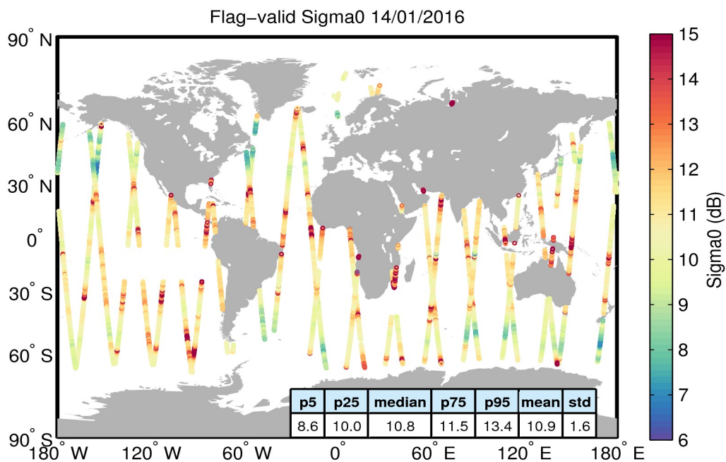
Figure 23. Geographical distribution of flag-valid sigma0 data over oceans and lakes for 14/01/2016. The statistical values shown in the table refer to the sigma0 in dB and are calculated over all measurements shown in the figure.
