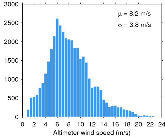
Figure 33. Histogram of flag-valid wind over oceans and lakes for 14/01/2016. The mean ( \mu ) and standard deviation ( \sigma ) are also shown. Note that values larger than 24 m/s are excluded from the histogram for the sake of readability but not from the computation of \mu and \sigma .
