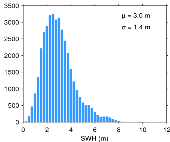
Figure 17. Histogram of flag-valid SWH over oceans and lakes for 14/01/2016. The mean ( \mu ) and standard deviation ( \sigma ) are also shown. Note that values larger than 12 m are excluded from the histogram for the sake of readability but not from the computation of \mu and \sigma .
